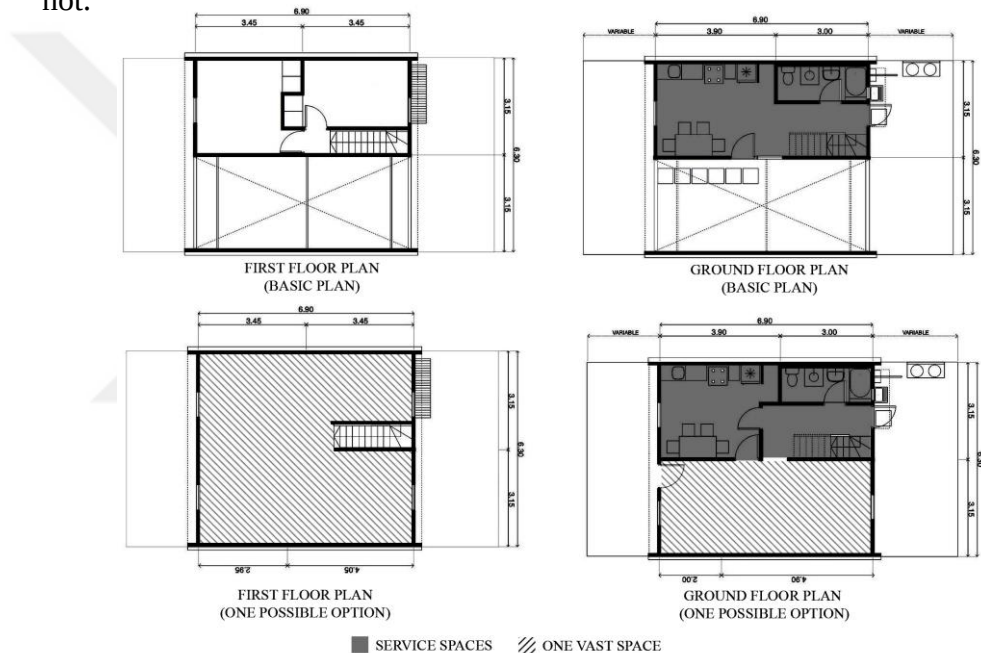
Figure 4.8. Service and post-created vast spaces in Villa Verde Housing (Elemental, 2013)
