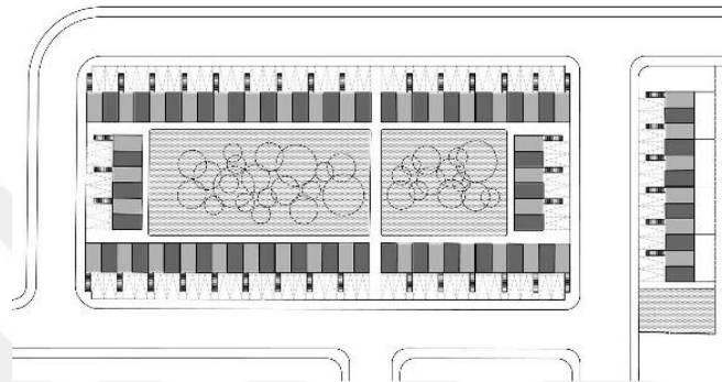
Figure 3.28. Site plan of Monterrey Housing (Elemental, 2010)
