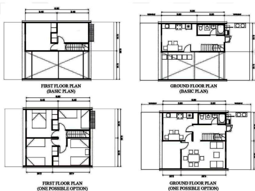
Figure 4.6. Basic and possible plans for dwellings in Villa Verde (Elemental, 2013)
