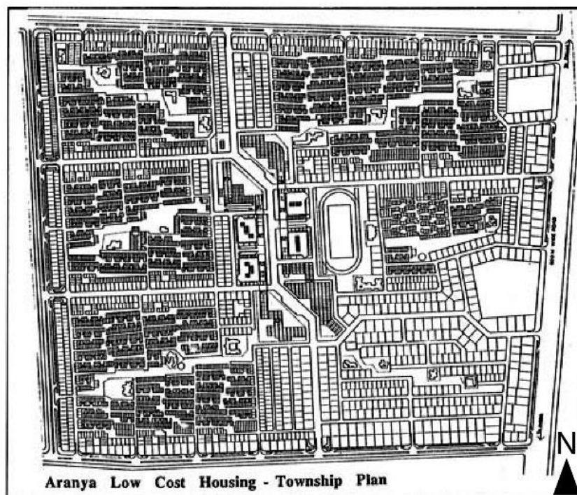
Figure 3.19. Aranya Low-Cost Housing, Doshi, 1982 (Ekram, 1995, p. 83)
