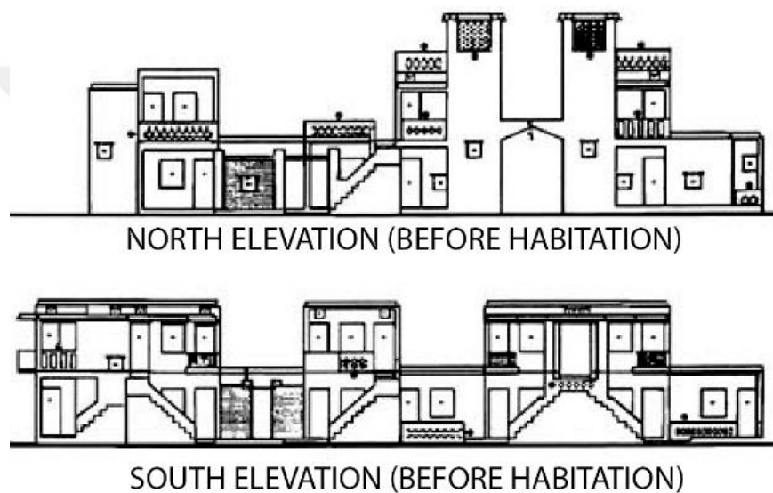
Figure 3.20. Elevations of Aranya Low-Cost Housing before habitation (Ekram, 1995)
