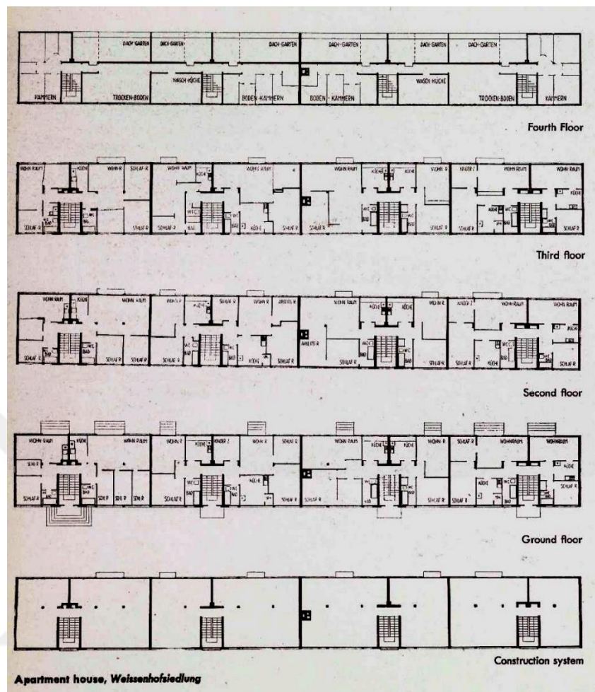
Figure 3.3. Floor plans of Weissenhofsiedlung from Mies' block (Johnson, 1978, pp. 44-45).
