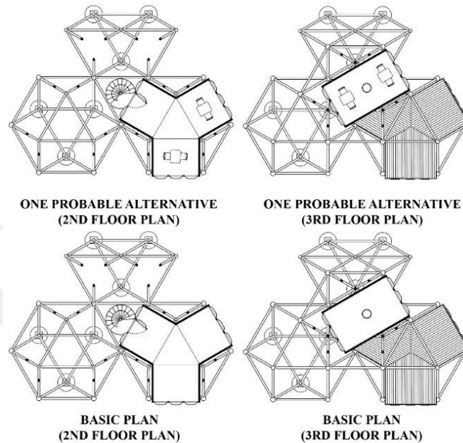
Figure 4.20. Basic and possible plan options in Plugin Tower (People's Architecture Office, 2016)
