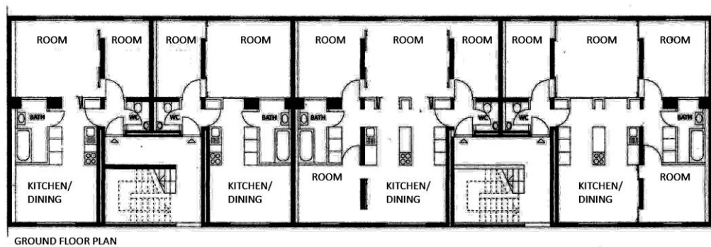
Figure 2.8. Housing Graz-Straßgang by Riegler Rieue Architekten (Riewe, 1994)
