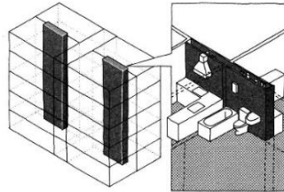
Figure 2.13. Vertical service distribution (Schneider & Till, 2007, p. 198)
