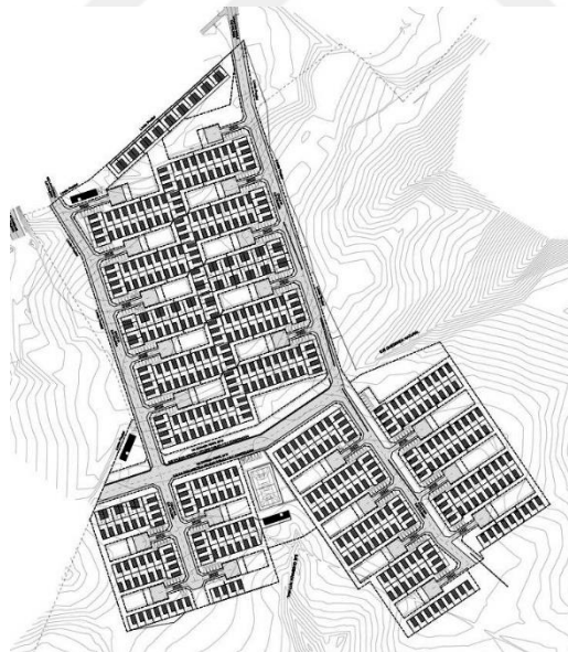
Figure 4.1. Site plan of Villa Verde Housing (Elemental, 2013)
