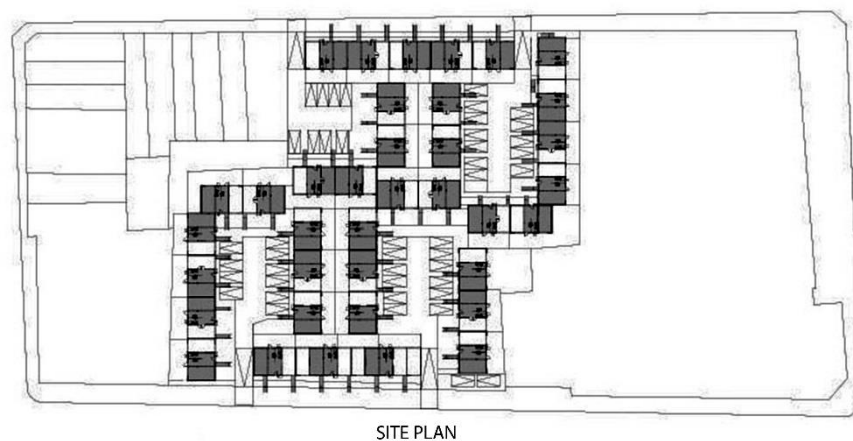
Figure 3.25. Quinta Monroy Housing, Elemental, 2004 (Aravena, Montero, Cortese, de la Cerda & Iacobelli, 2004, p. 30).
