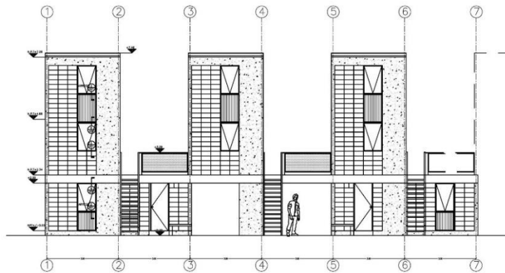
Figure 3.26. Front Elevation of Quinta Monroy Housing (Aravena, Montero, Cortese, de la Cerda & Iacobelli, 2004, p. 30).
