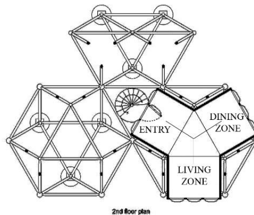
Figure 4.21. Direct contact between zones in Plugin Tower (People's Architecture Office, 2016)
