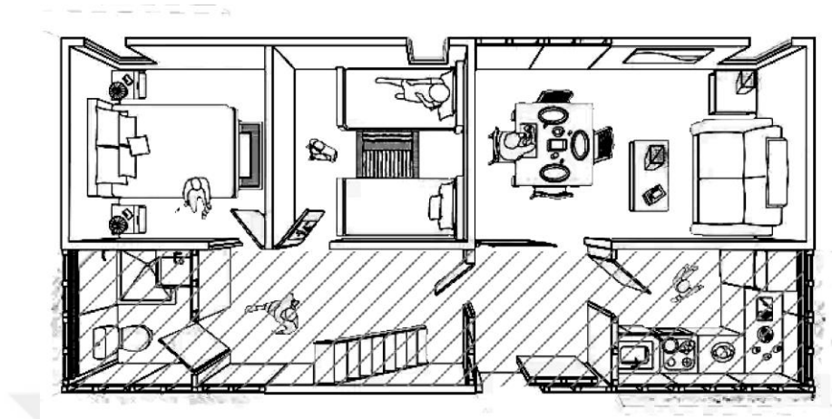
Figure 4.15. Ground floor in Sustainable Housing (Cruz, 2015)
