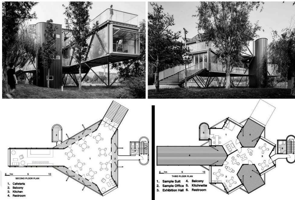
Figure 4.17. Lakeside Plugin Tower (People's Architecture Office, 2019)
