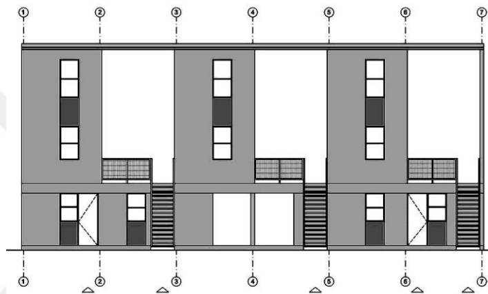
Figure 3.29. Front Facade of Monterrey Housing (Elemental, 2010)
