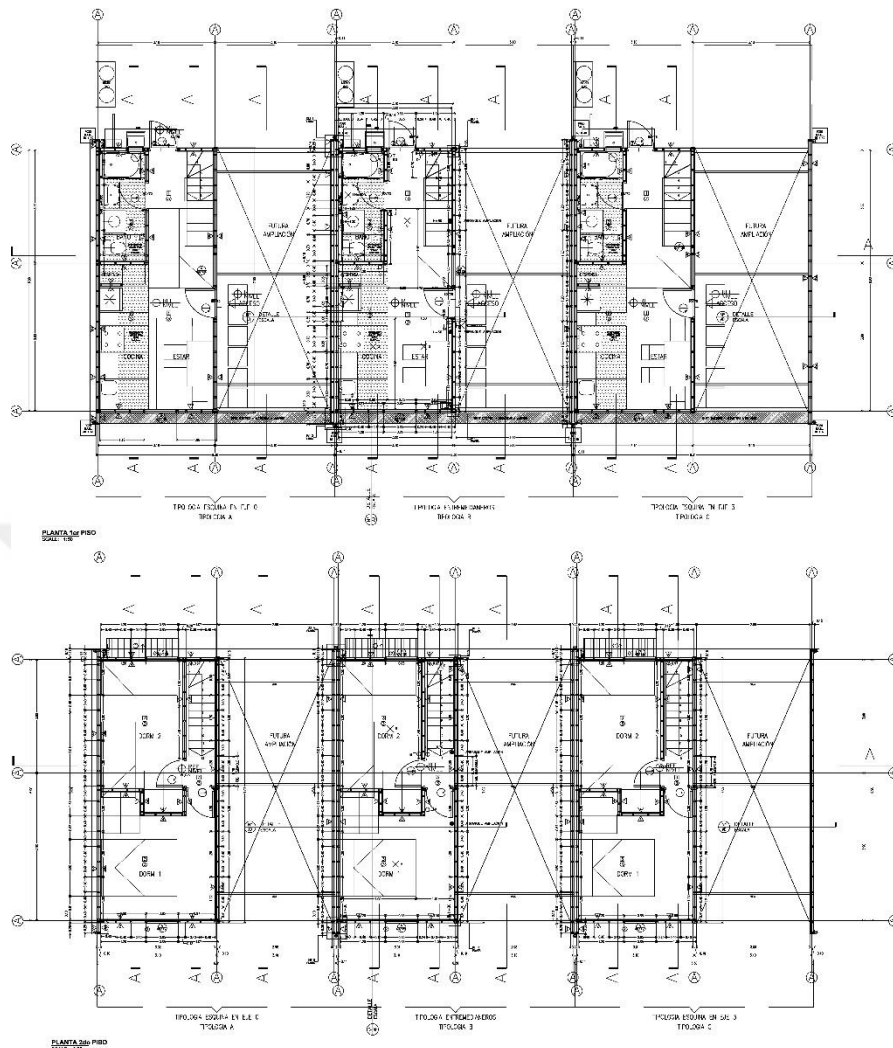
Figure 4.7. Ground floor (top) and first floor (bottom) plans of Villa Verde Housing (Elemental, 2010)
