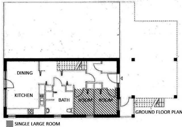
Figure 2.12. London Flexhouse of Nouvelle Development Corporation (CMHC, 1999, p. 52)
