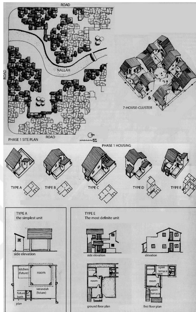
Figure 3.22.. Belapur Incremental Housing, Correa, 1984-1986 (Khan, 1987)
