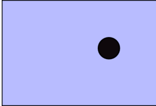
Figure 2.2: The object (black circle) is more salient than background and it attracts more attention.
