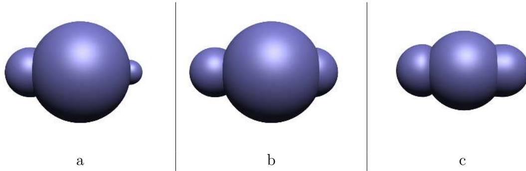
Figure 2.5: Saliency by parts: larger size, larger protrusion, and stronger boundaries (having higher crease angles) increase saliency of the part [53].
