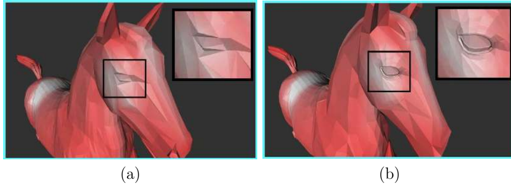
Figure 3.6: The animated horse model is simplified using quadric error metrics (a) and using our saliency-based simplification method (b). Both of the models have 4600 faces. (From [21]. ©2010 ACM, reprinted with permission.)
