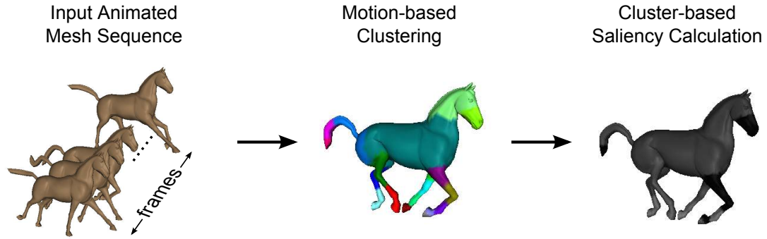
Figure 3.15: Overview of the cluster-based saliency calculation model.
