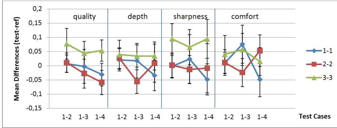
Figure 5.16: Experimental results for texture resampling method (Error bars show the 95% confidence interval of the mean). (From [20]. ©2010 Elsevier, reprinted with permission.)
