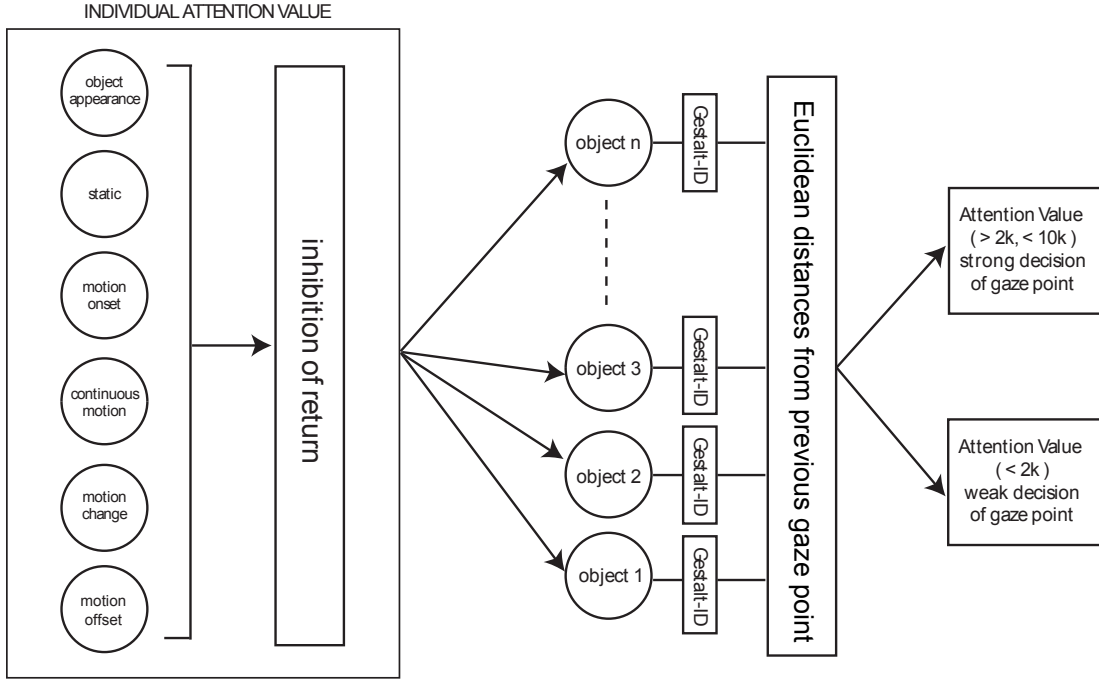
Figure 3.13: Overview of the POS model. (From [11]. ©2011 Springer, reprinted with permission.)
