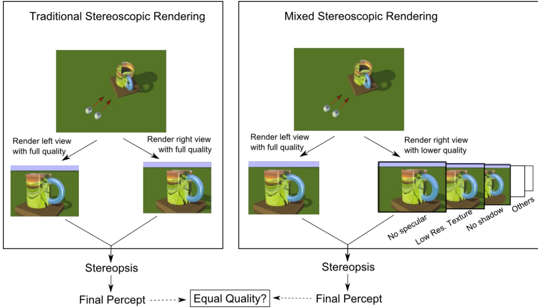
Figure 4.1: Left: Traditional stereoscopic rendering approach, Right: Our rendering approach for optimization. On the upper images, the object space is illustrated along with the viewpoint. The images below show the corresponding left and right eye views of the above scene. The right view on the mixed stereoscopic rendering approach is generated with lower quality caused by simplifying a set of modeling and rendering features. (From [20]. ©2010 Elsevier, reprinted with permission.)
