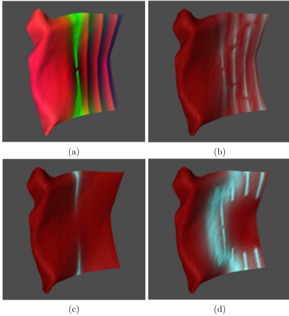
Figure 3.4: The animated cloth model (a). The calculated saliencies based on hue, color opponency, and intensity are shown in (b), (c), and (d), respectively. Light-colored areas show the salient regions and are emphasized for illustration purposes. (From [21]. ©2010 ACM, reprinted with permission.)
