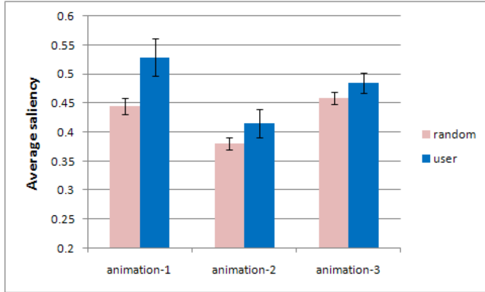
Figure 5.3: Comparison between the calculated average saliencies of the regions that are looked at by the actual users, and the randomly generated virtual users. Error bars indicate 95% confidence intervals. (From [21]. ©2010 ACM, reprinted with permission.)
