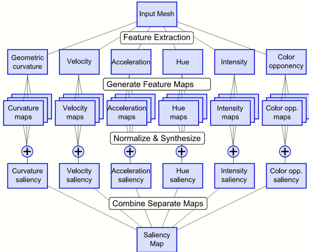
Figure 3.1: The proposed saliency computation framework. (From [21]. ©2010 ACM, reprinted with permission.)
