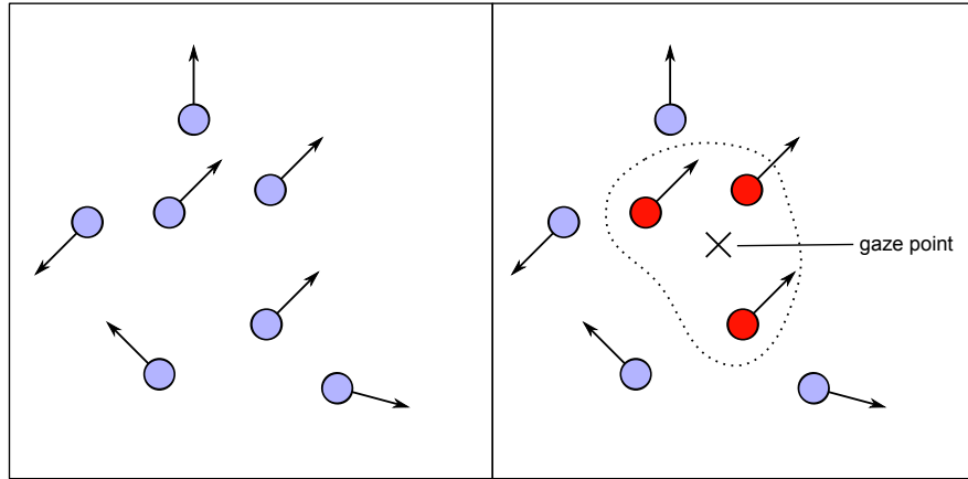
Figure 2.16: Left: arrows represent motion directions of the separate units. Right: According to Gestalt psychology, the units with the same motion behavior are united and perceived as a single unit. In such a case, viewers look at somewhere inbetween the group members instead of focusing on one of them.
