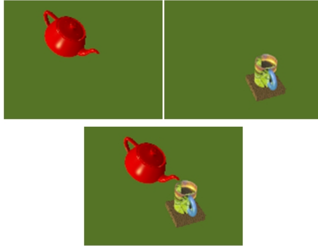
Figure 2.15: Binocular rivalry mechanism. When the left-eye (top-left) and right-eye (top-right) views are shown, the combined view (bottom) merges the dominant regions from the two views. (From [20]. ©2010 Elsevier, reprinted with permission.)
