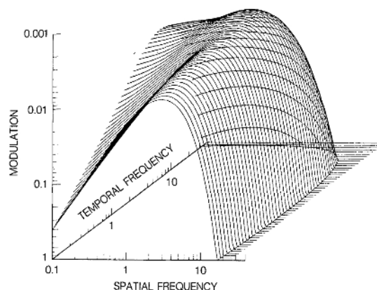
Figure 2.9: Spatiotemporal sensitivity formula derived by Kelly. (From [65]. ©1979 Optical Society of America, reprinted with permission.)
