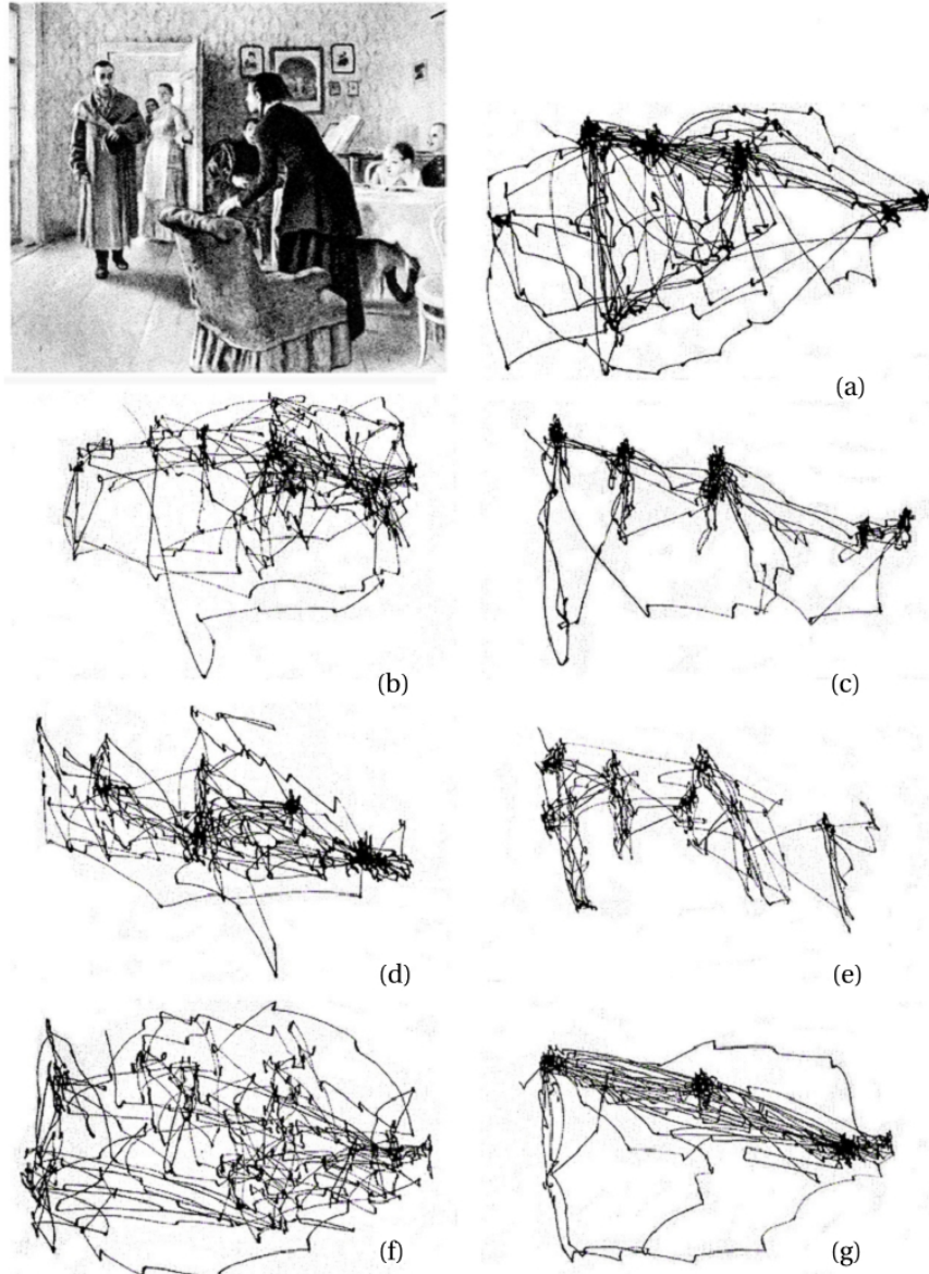
Figure 2.6: Repin's picture was examined by subjects with different instructions; (a) Free examination. (b) Estimate the material circumstances of the family in the picture. (c) Give the ages of the people. (d) Surmise what the family had been doing before the arrival of the 'unexpected visitor'. (e) Remember the clothes worn by the people. (f) Remember the position of the people and objects in the room. (g) Estimate how long the unexpected visitor had been away from the family. (From [115]. ©Benjamin W. Tatler, Nicholas J. Wade, Hoi Kwan, John M. Findlay, and Boris M. Velichkovsky; reprinted with permission. )
