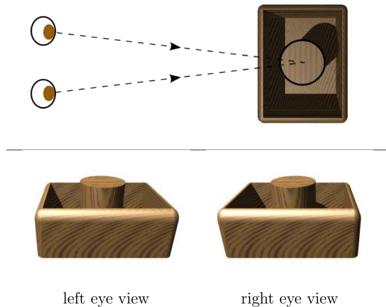
Figure 2.14: Visual system uses the difference of images viewed by left and right eyes to extract depth information.
