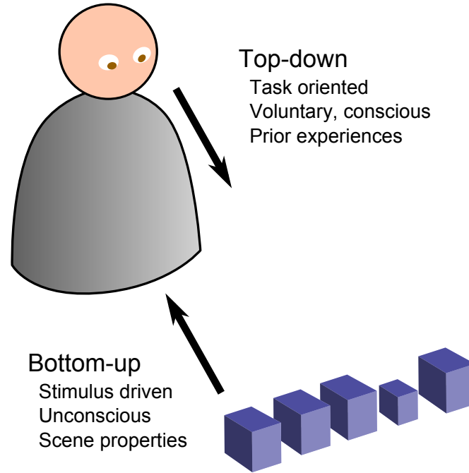
Figure 2.1: Two components of visual attention
