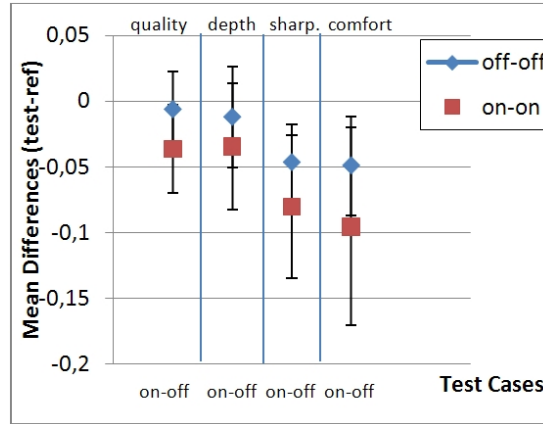
Figure 5.17: Experimental results for mixed shadowing method (Error bars show the 95% confidence interval of the mean). (From [20]. ©2010 Elsevier, reprinted with permission.)
