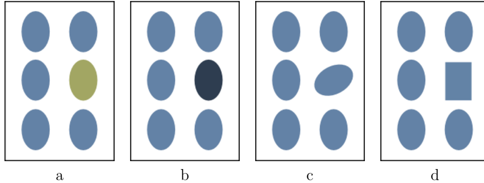
Figure 2.4: Difference in various properties affects saliency. Here, differing properties are hue (a), luminance (b), orientation (c), and shape (d).
