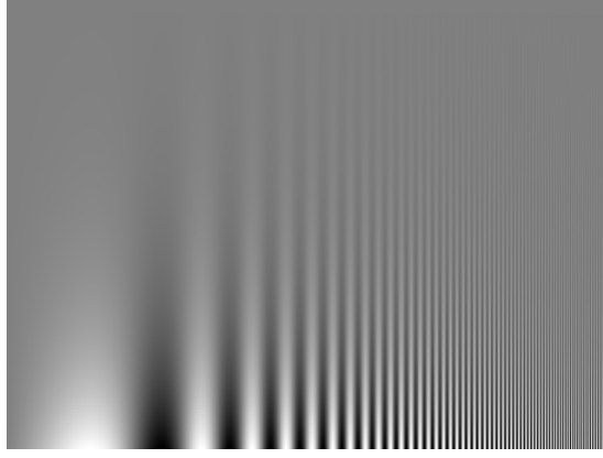
Figure 2.8: Campbell-Robson Contrast sensitivity function chart [22]. The frequency increases from left to right and contrast decreases from bottom to top. (Image from [94]. Courtesy of Izumi Ohzawa, reprinted with permission.)
