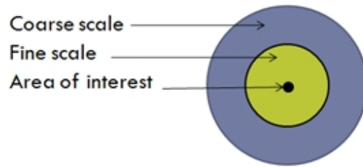
Figure 2.3: Center-surround mechanism, saliency of interested area is related to difference of fine and coarse scales in terms of different properties such as luminance, velocity, orientation, etc.
