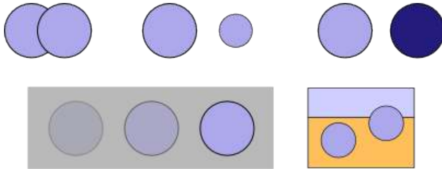
Figure 2.13: Several monocular depth cues including: occlusion, relative size, relative brightness, atmosphere, and distance to horizon.
