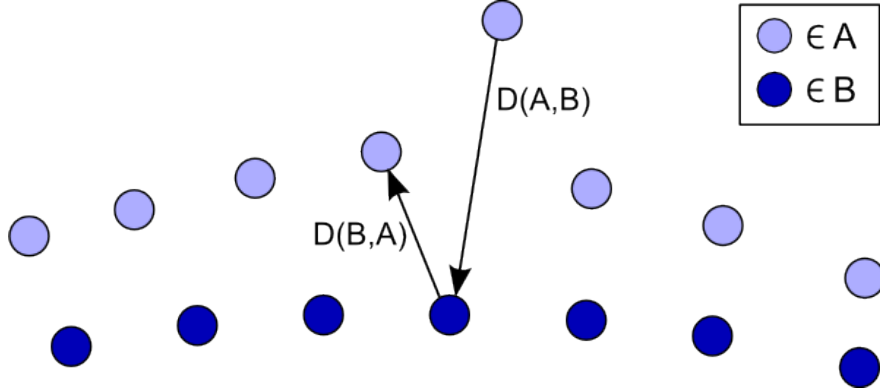
Figure 2.18: The Hausdorff distance between two surfaces. The two-sided Hausdorff distance is H(A, B) = \max(D(A, B), D(B, A)) . (From [19]. ©2011 IEEE, reprinted with permission.)
