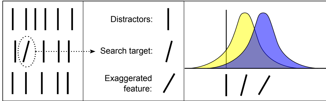
Figure 2.7: Human visual system is tuned to the exaggerated feature, which is a better discriminator, to optimize the search process.
