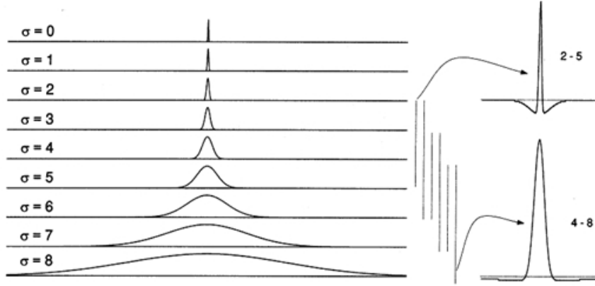
Figure 4.2: Gaussian pixel widths for the nine scales used in the intensity contrast calculation. Scale \sigma = 0 corresponds to the original image, and each subsequent scale is coarser by a factor 2. On the right, two examples of the six center-surround DoG filters are shown, for scale pairs 2-5 and 4-8. (From [60]. ©1998 Elsevier, reprinted with permission.)
