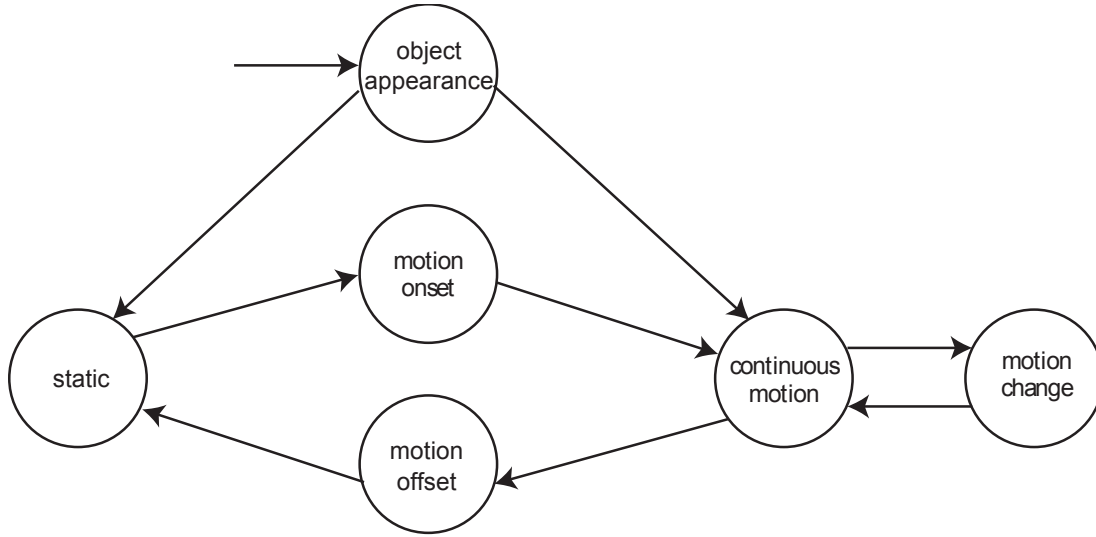
Figure 3.10: Motion cycle of an object in an animation. Perceptually distinct phases are indicated as six states. Object appearance is the initial state for each object. (From [11]. ©2011 Springer, reprinted with permission.)
