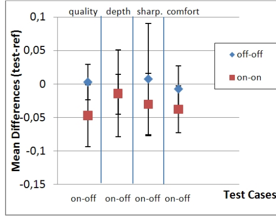
Figure 5.12: Experimental results for mixed-level antialiasing method (Error bars show the 95% confidence interval of the mean). (From [20]. ©2010 Elsevier, reprinted with permission.)
