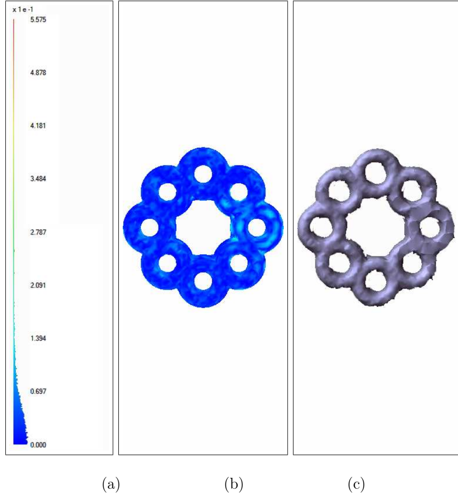
Figure 3.21: 9 Handle Torus model compressed with JPEG2000 to 14.6 KB (12.4 bpv). (a) The histogram of the error on the original model. (b) The original model. Color levels indicate the distortion between the original and the reconstructed model. Blue is the lowest distortion level. As the distortion increases the color index goes from blue to green and then red. Red is the highest distortion level. (c) The reconstructed model.
