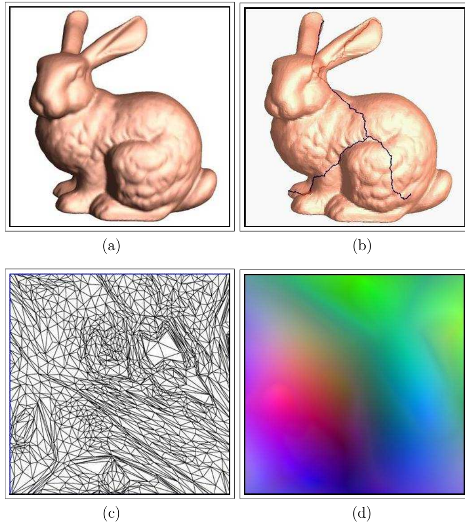
Figure 1.12: Geometry images. (a) The original model. (b) Cut on the mesh model. (c) Parameterized mesh model. (d) Geometry image of the original model. (Reprinted from [5] Data Courtesy Hugues Hoppe)
