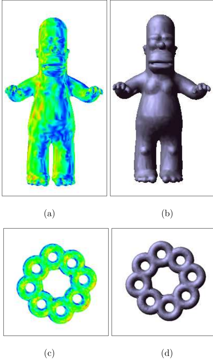
Figure 3.18: Homer and 9 Handle Torus models compressed using MPEG-3DGC. The compressed data sizes are 41.8 KB and 82.8 KB respectively. Figures on the left side show the error of the reconstructed model with respect to the original one. Reconstructed models are shown on the right side.
