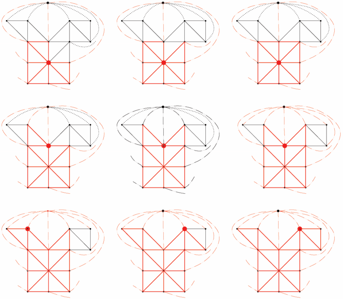
Figure 1.7: TG Encoding of the same mesh as EdgeBreaker. The resulting codeword will be [ 8,6,6,4,4,4,4,4,6,4,5,Dummy 13,3,3 ].
