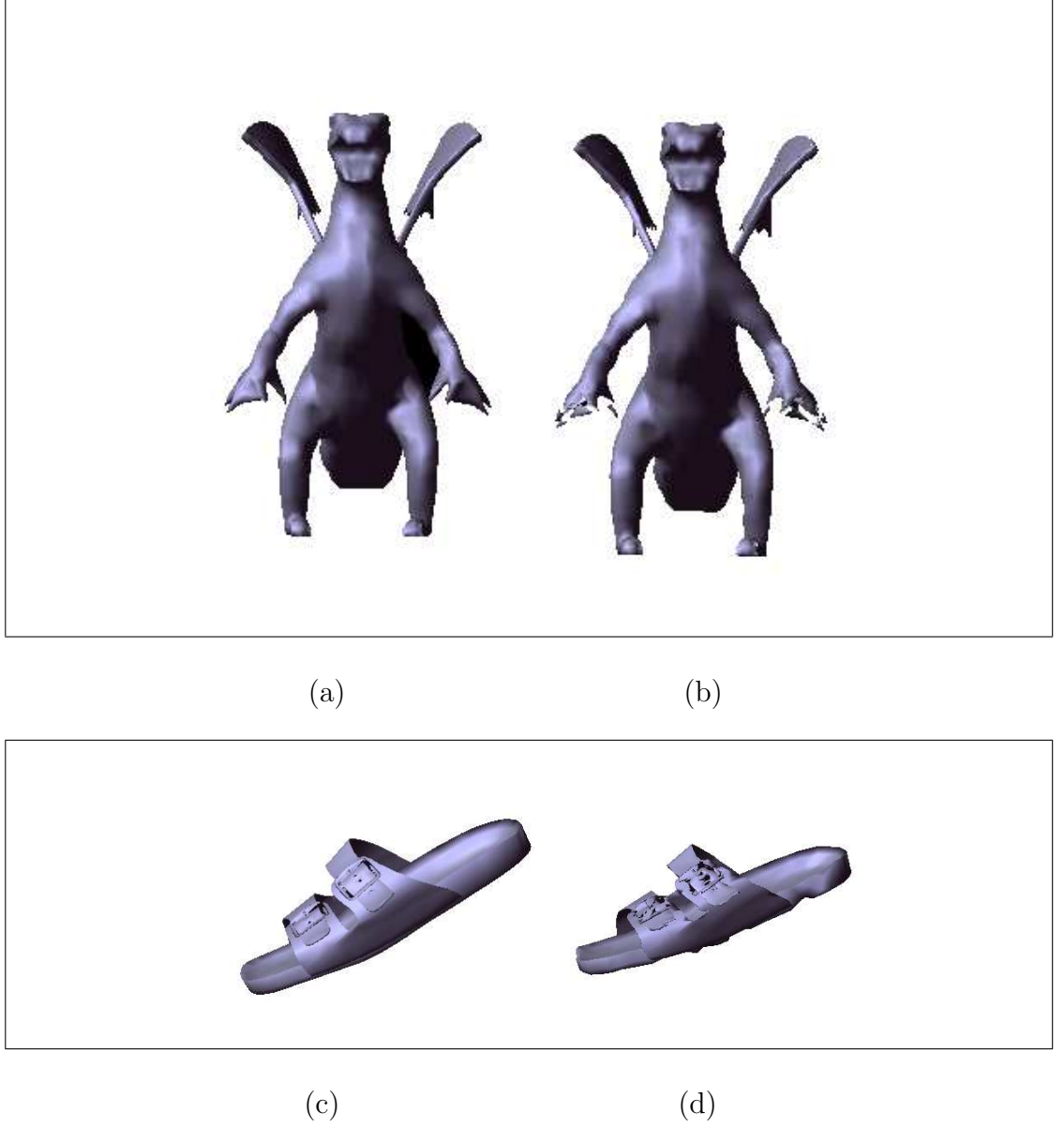
Figure 3.20: (a) Dragon (5213 vertices) and (c) Sandal (2636 vertices) models compressed using MPEG-3DGC. (b) Dragon (5213 vertices) and (d) Sandal (2636 vertices) models compressed using The proposed SPIHT coder. Compressed data size are 43.1 KB and 10.4 KB, respectively for Dragon model and 22.7 KB and 2.77 KB respectively for Sandal model.
