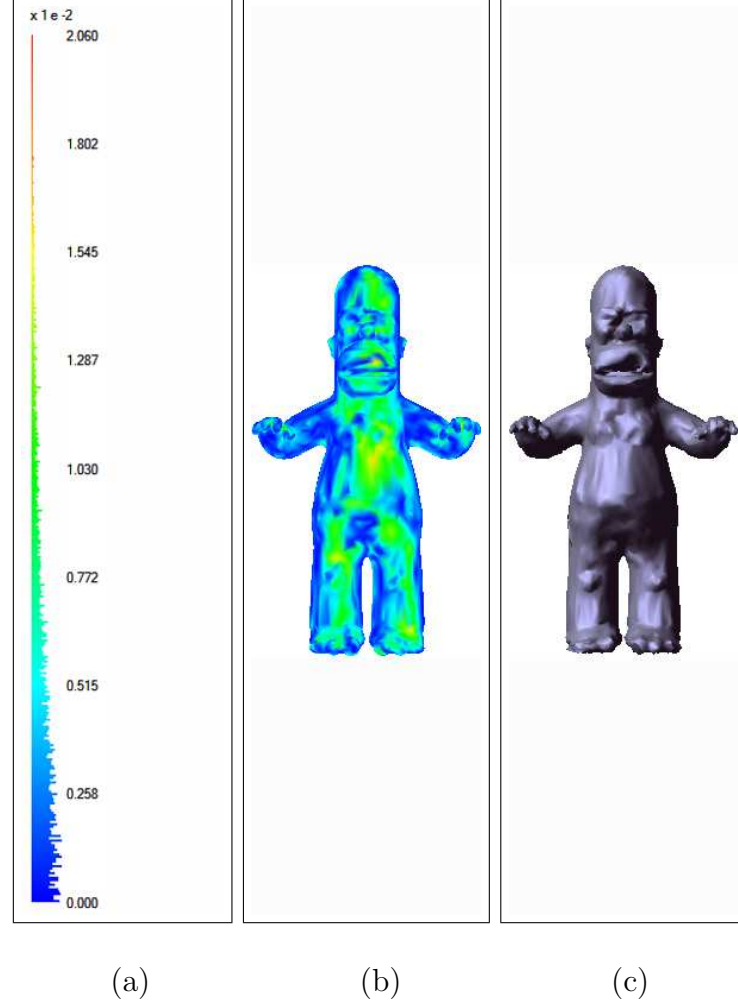
Figure 3.3: Homer Simpson model compressed with JPEG2000 to 6.58 KB (10.7 bpv). (a) The histogram of the error on the original model. (b) The original model. Color levels indicate the distortion between the original and the reconstructed model. Blue is the lowest distortion level. As the distortion increases the color index goes from blue to green and then red. Red is the highest distortion level. (c) The reconstructed model.
