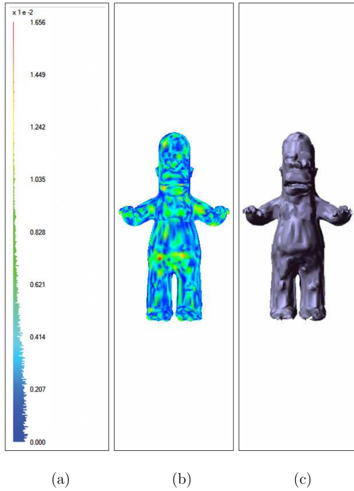
Figure 3.9: Homer Simpson model compressed with SPIHT to 4.67 KB (7.6 bpv).
