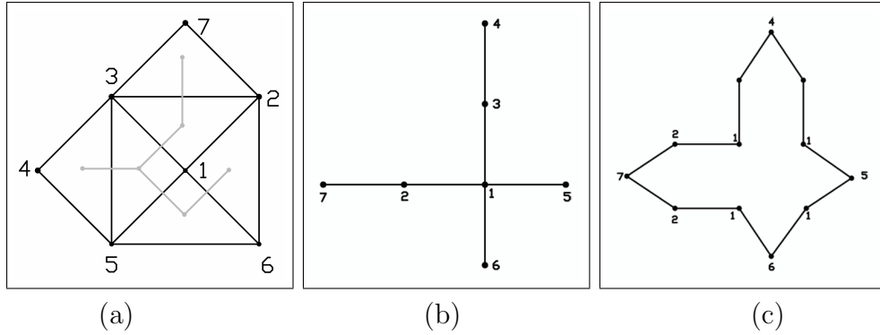
Figure 1.3: Spanning trees in the triangular mesh strip method. (a) Triangle spanning tree, (b) vertex spanning tree, (c) vertex spanning tree with doubled edge.
