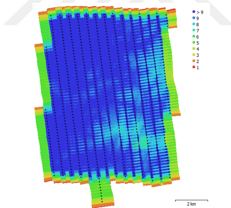
Figure A.6 Camera locations and image overlaps of block 6
