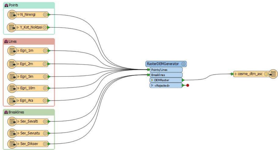
Figure 4.6 FME workbench for raster DTM generation
