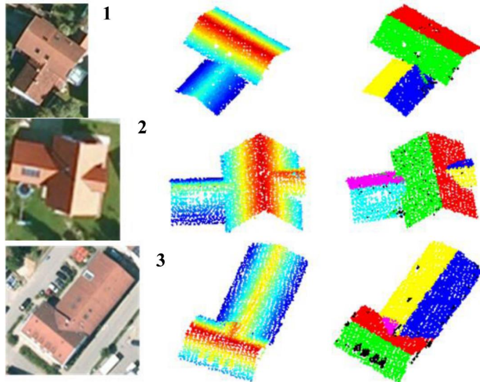
Figure 2.10 Segmented roofs: Aerial photo (left), point cloud sorted by height (middle) and point cloud segmented (right) Fan et al. [49]
