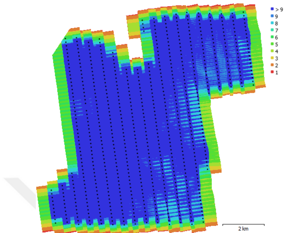
Figure A.5 Camera locations and image overlaps of block 5
