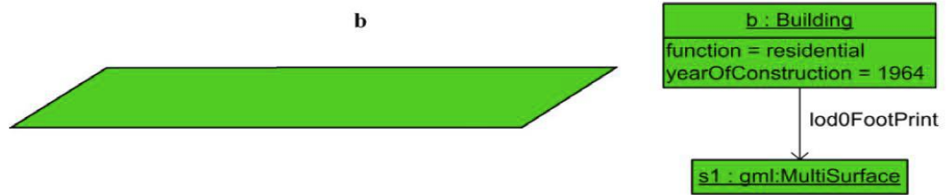
Figure 2.3 LoD0 building (left) and UML diagram (right) by Gröger and Plümer [21].
