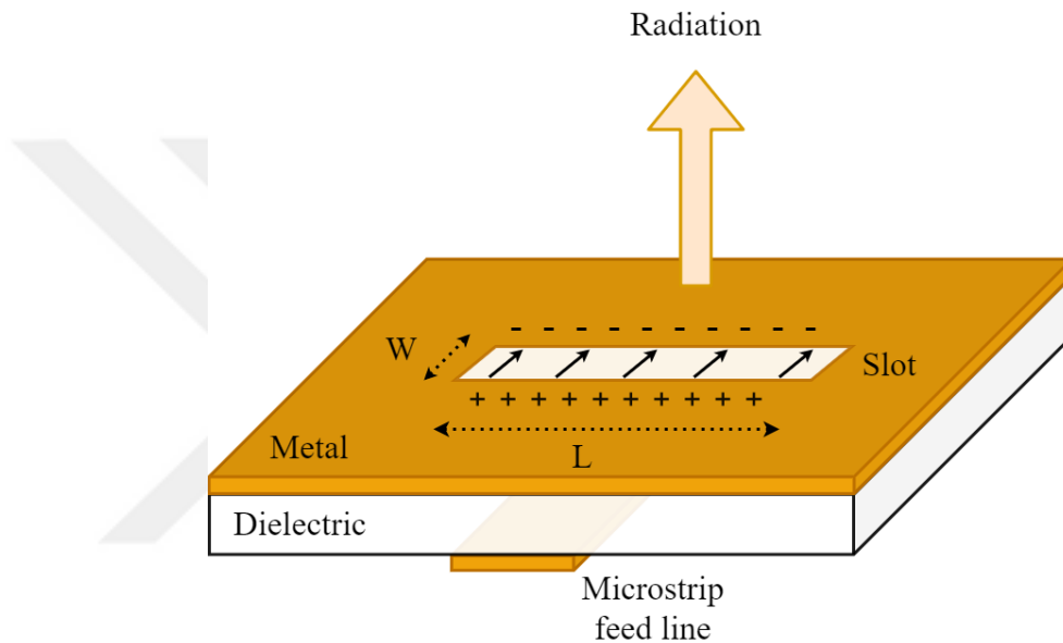
Figure 3.16. A microstrip fed slot antenna model.
