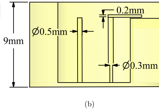
Figure 3.6. The biohybrid implant dimensions (a) top view. (b) side view with lower outer wall.
