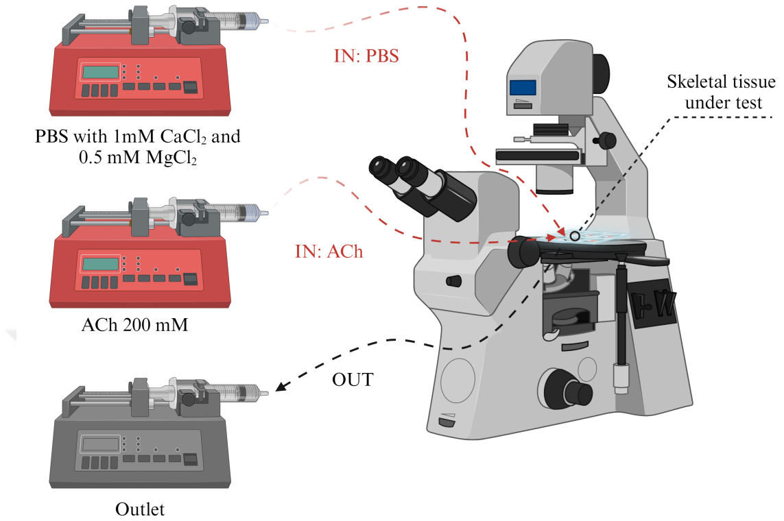
Figure 3.4. The ACh test setup.
