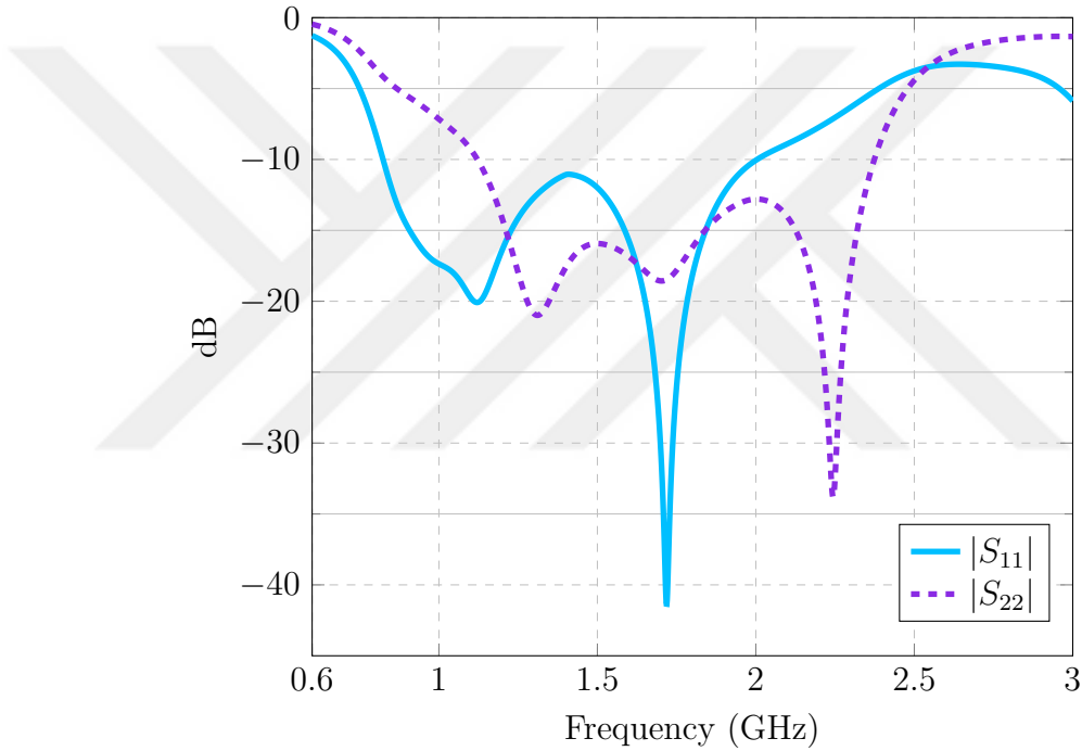
Figure 4.4. dB versus frequency graph for |S_{11}| and |S_{22}| of the optimized antenna located on the electromagnetic simulation setup.
