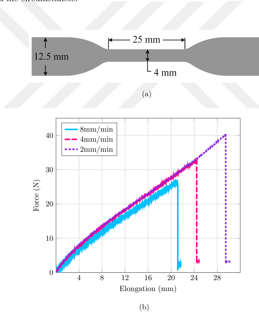
Figure 3.8. (a) The dog-bone specimen used for the ASTM638 tensile test. (b) Force versus elongation curve for three pulling speeds.
