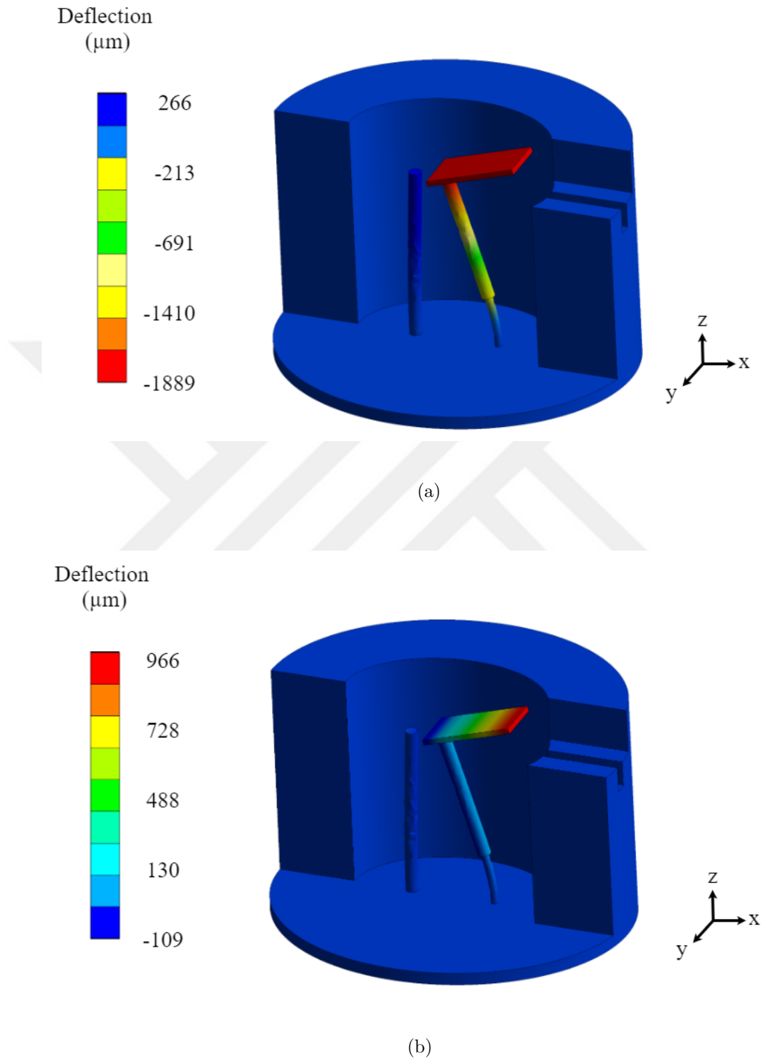
Figure 4.1. Mechanical deflection analysis of the flexible scaffold. (a) Deflection in x-direction. (b) Deflection in z-direction.
