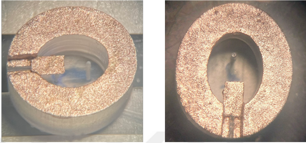
Figure 3.15. Fabricated prototype views of implant antenna.
