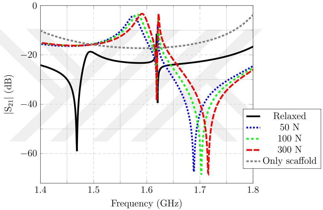
Figure 3.12. The transmission coefficient magnitude of the waveguide for different muscle contraction cases.
