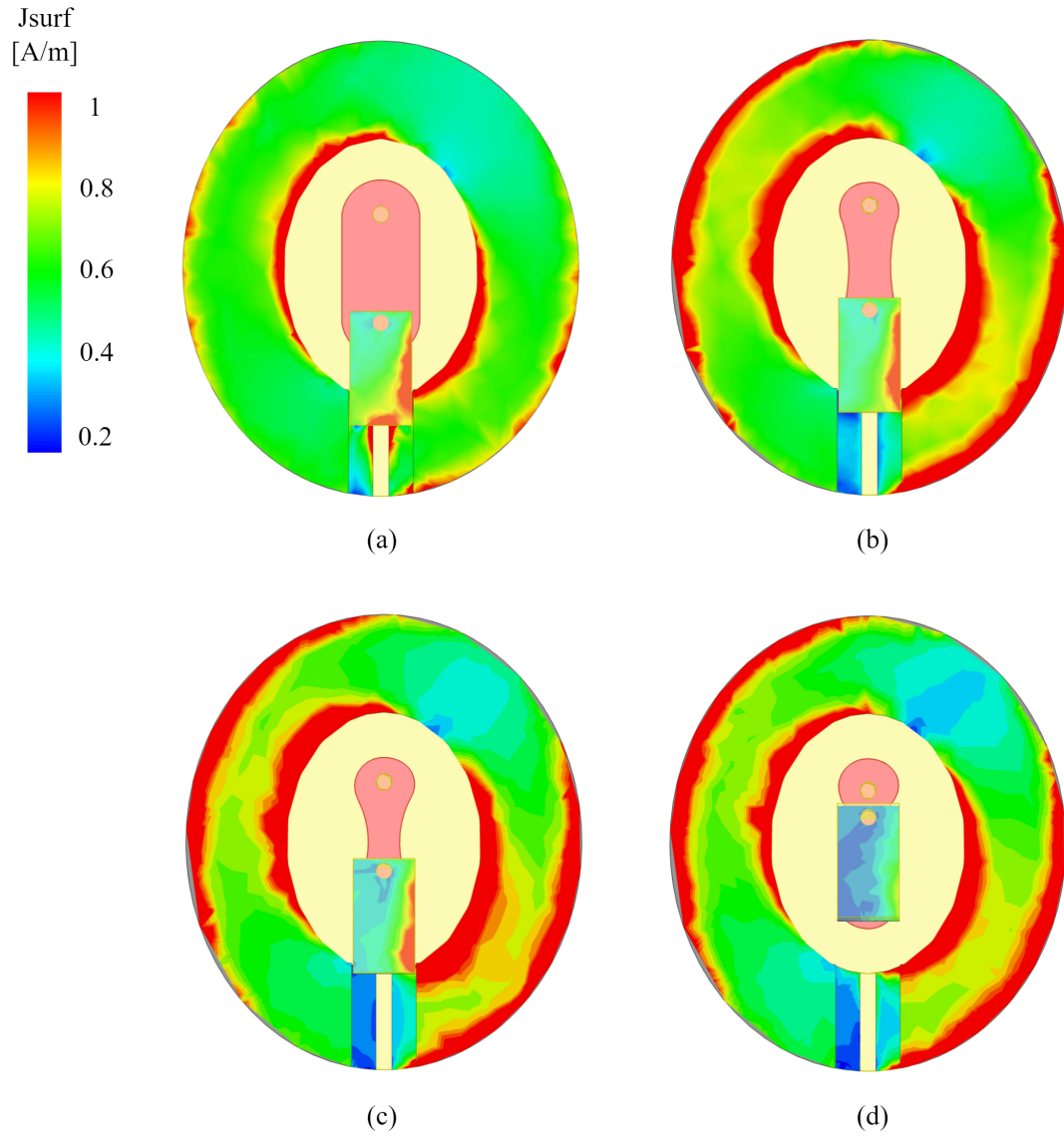
Figure 4.8. Surface current density for the (a) Relaxed case at 1.48 GHz (b) 50 \mu N case at 1.57 GHz (c) 100 \mu N at 1.59 GHz (d) 300 \mu N case at 1.62 GHz.
