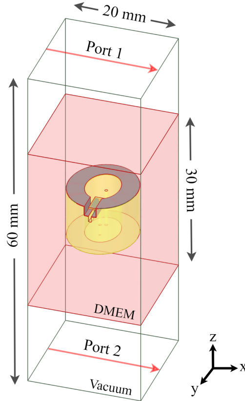
Figure 3.11. Waveguide simulation setup and dimensions.
