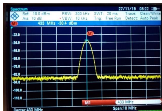
Figure 3.29 Signal level at the output of down-converter block after optimizations
