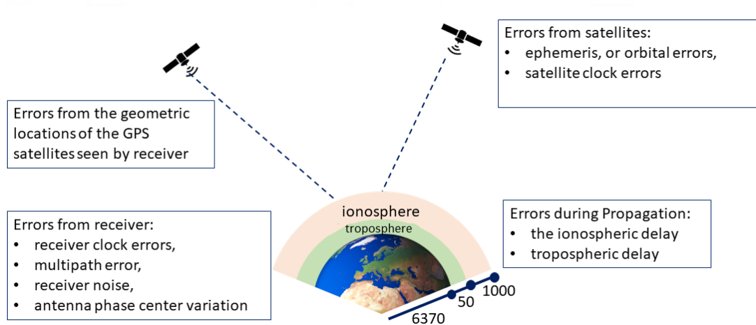
Figure 2.4 GPS Errors [72]
