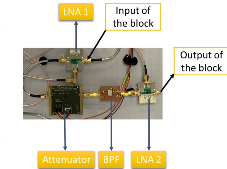
Figure 3.31 Realized signal power conditioner and filter block
