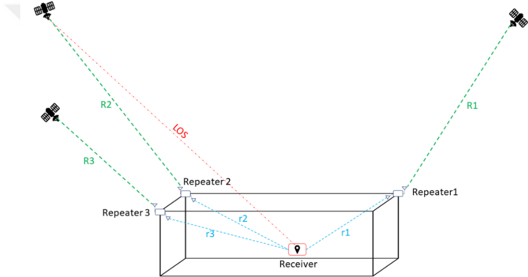
Figure 2.5 Overview of 2D Indoor Positioning Based on GPS
