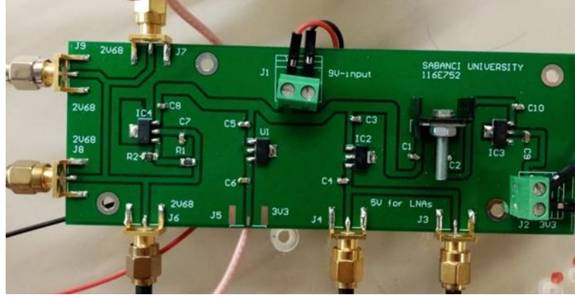
Figure 4.23 Voltage regulator for receiver hardware
