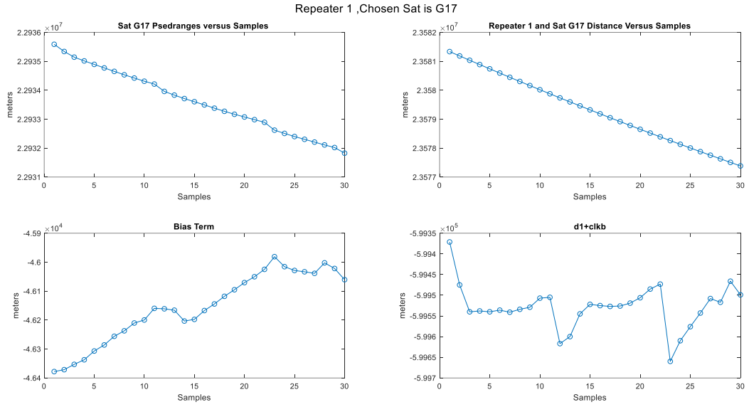
Figure 5.23 PR1, clkb, dst, and d1+clkb terms when G17 is selected from repeater 1
