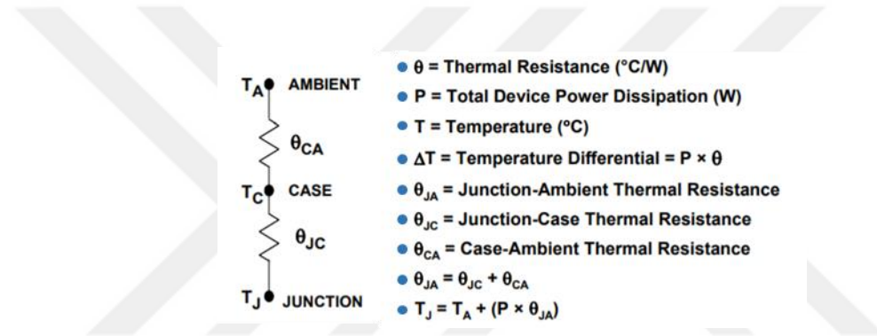
Figure A.1 Thermal design terms and equations [92]
