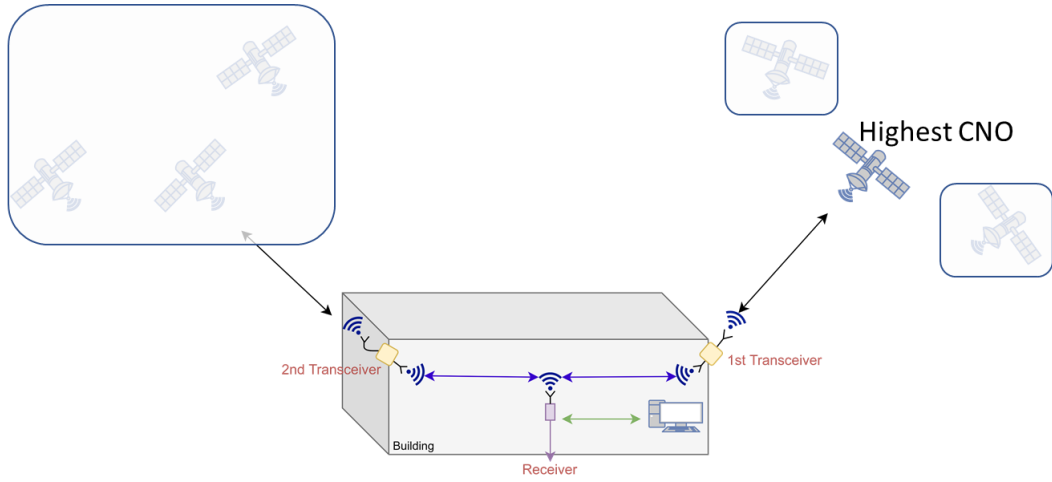
Figure 5.13 Satellite represented with the highest CNO in the directional antenna's angle of view
