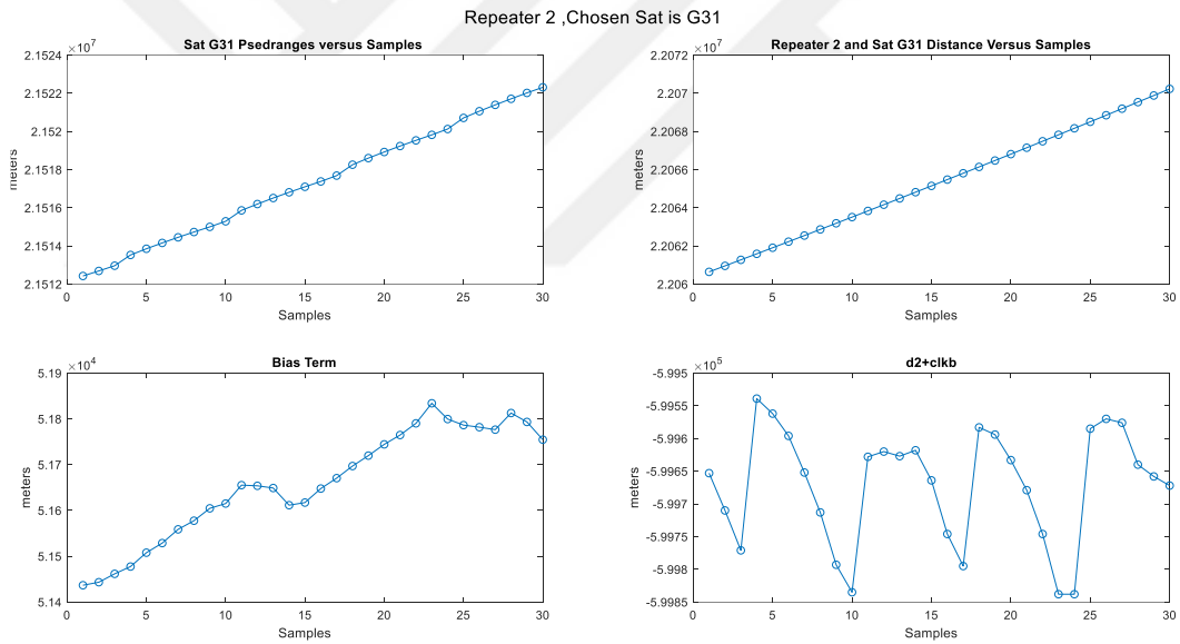
Figure 5.24 PR2, clkb, dst, and d2+clkb terms when G31 is selected from repeater 2
