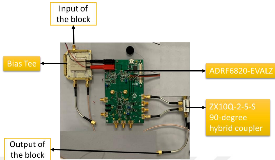
Figure 3.13 Down-converter block formed with the modules presented
