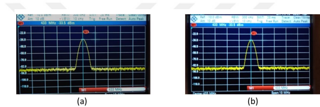
Figure 3.28 Signal levels at the output of I+ in (a) and Q+ in (b) after optimizations
