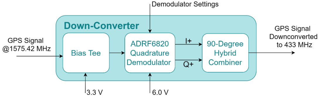
Figure 3.11 Modules in the down-converter block
