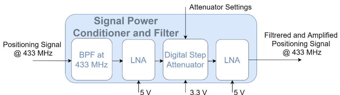
Figure 4.4 Modules in the signal power conditioner and filter block
