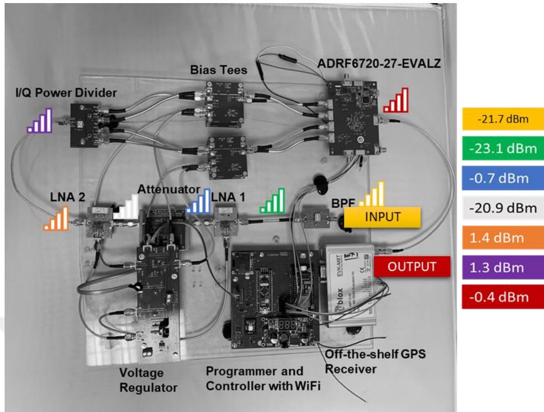
Figure 5.2 Signal power levels between modules of the receiver
