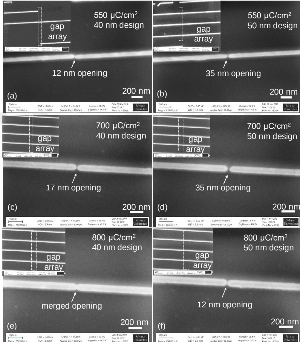
Figure 5.5 SEM images of the gap nanostructures fabricated the same developing time and type for predefined 40 nm and 50 gaps with various exposed dose values respectively; a) and b) 550 \mu\text{C cm}^{-2} , c) and d) 700 \mu\text{C cm}^{-2} , e) and f) 800 \mu\text{C cm}^{-2} for substrate of silicon
