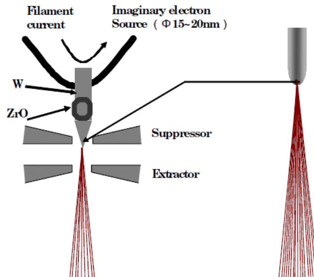
Figure 3.7 Electron gun with a thermal field emission gun [11].
