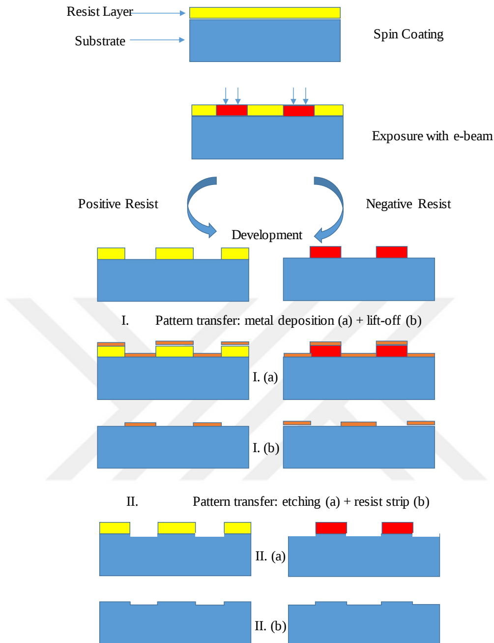
Figure 3.1 Schematic for positive and negative resists [9]
