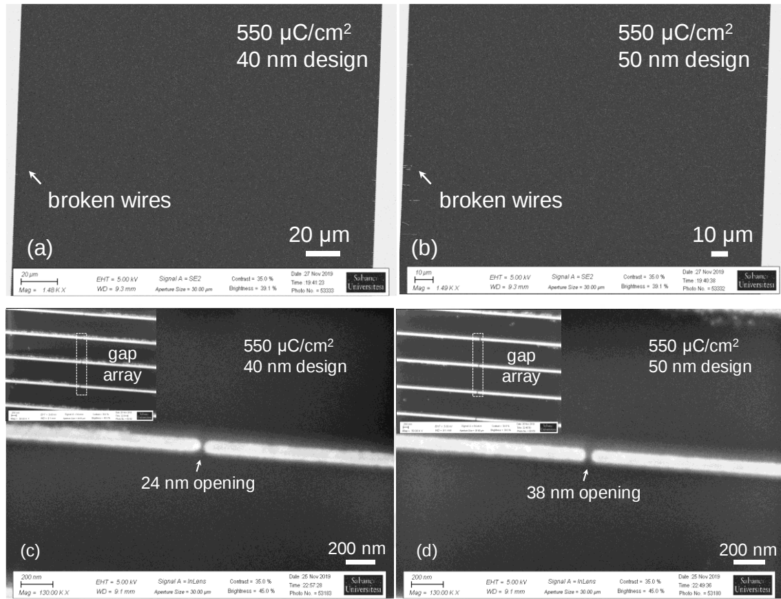
Figure 5.13 SEM images of PEC on gap nanostructures when the exposure dose (550 \mu\text{C cm}^{-2} ), developer type (MIBK:IPA (1:3)) and (MIBK:IPA (1:1)) and develop time are kept constant for a) and b) no PEC , c) and d) PEC for silicon substrate.
