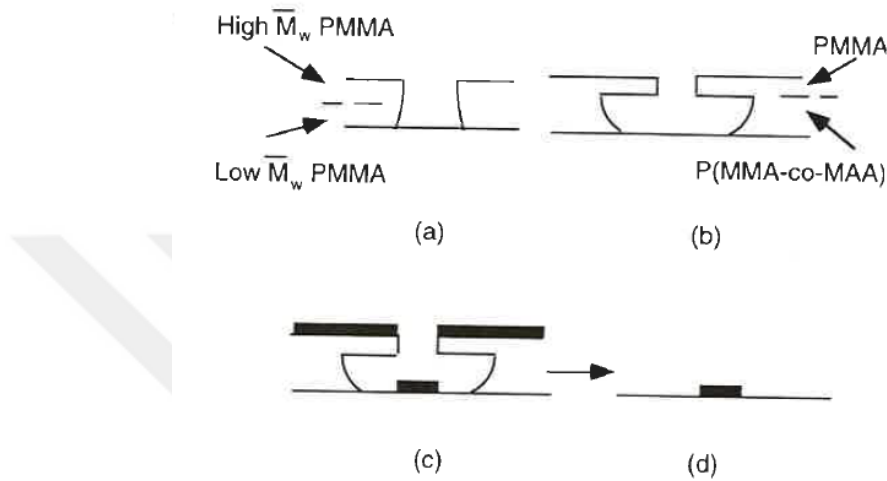
Figure 3.14 Two bilayer e-beam resist structure a) High MW PMMA / Low MW PMMA b) PMMA /Copolymer c) The resist is then removed in the solvent. d) Final structure after dissolving resist [32].
