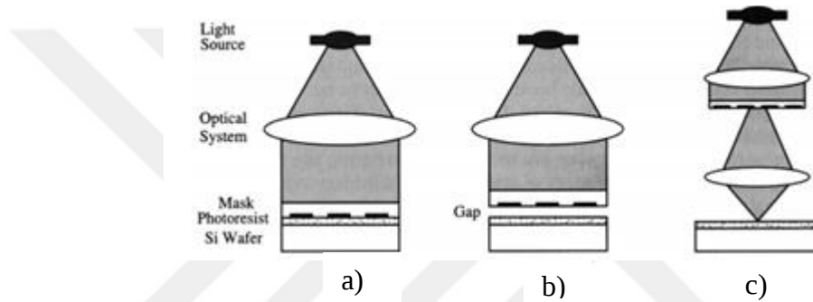
Figure 2.1 Patterning techniques; a) Contact Printing, b) Proximity Printing, c) Projection Printing [30]
