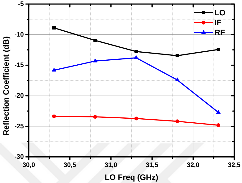
Figure 68: The RF, LO and IF return losses of the designed upconverter
