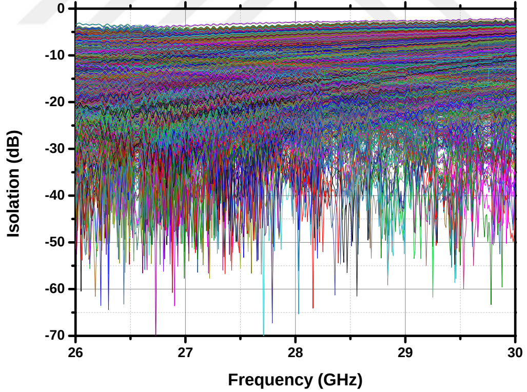
Figure 50: The isolation for every state of the impedance tuner
