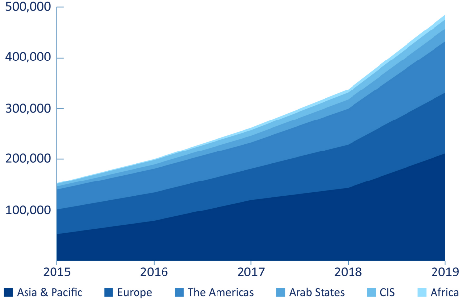
Figure 2: Bandwidth usage by region between in Gbps 2015 - 2019 [5]
