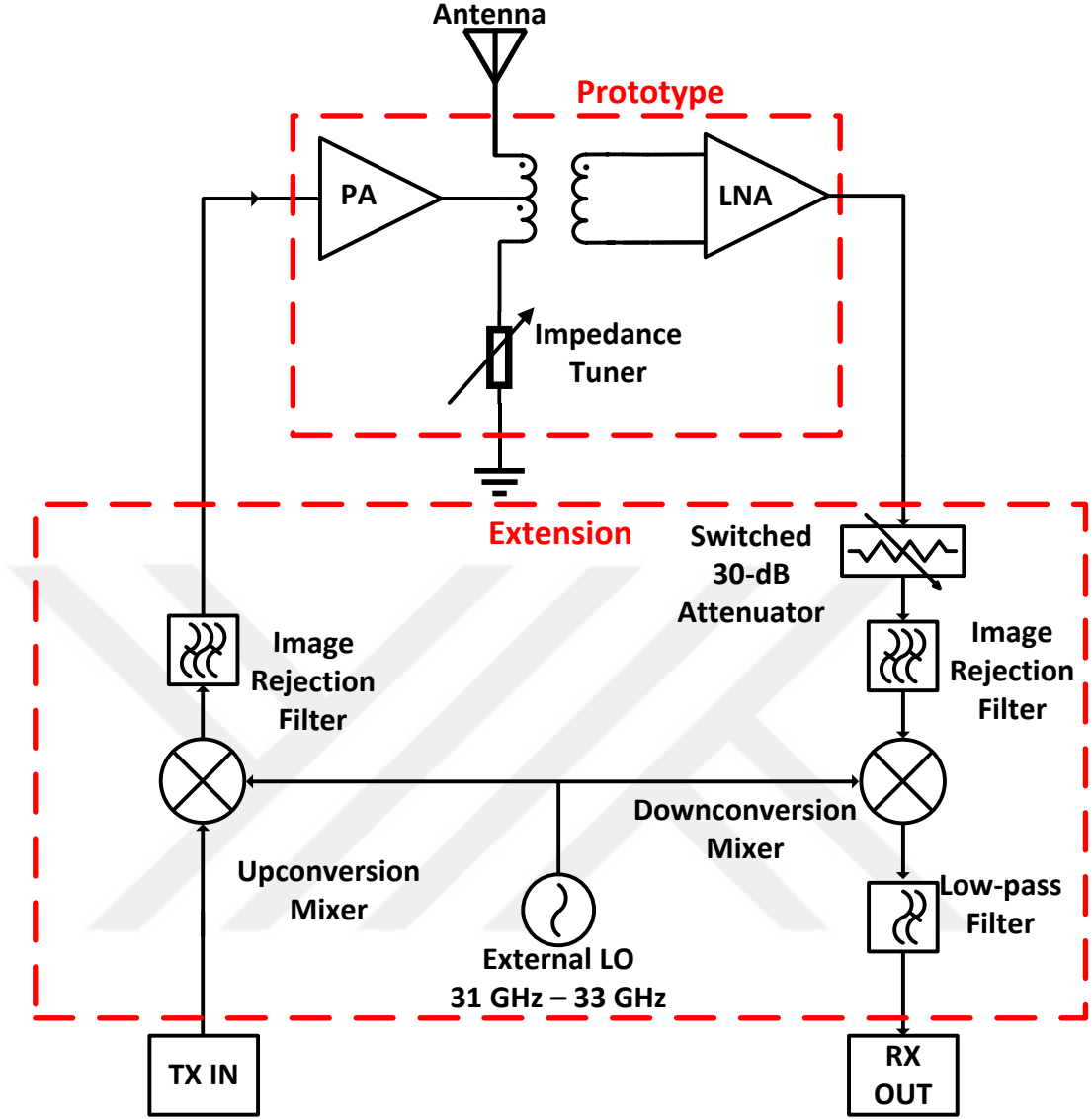
Figure 17: The block diagram of the system
