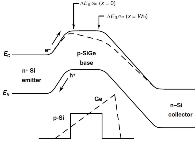
Figure 7: The representation of the energy band diagram of SiGe HBT (top) and Si BJT (bottom) [9]
