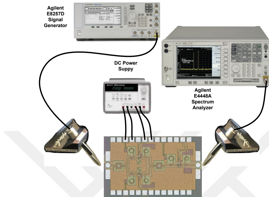
Figure 37: Linearity measurement setup
