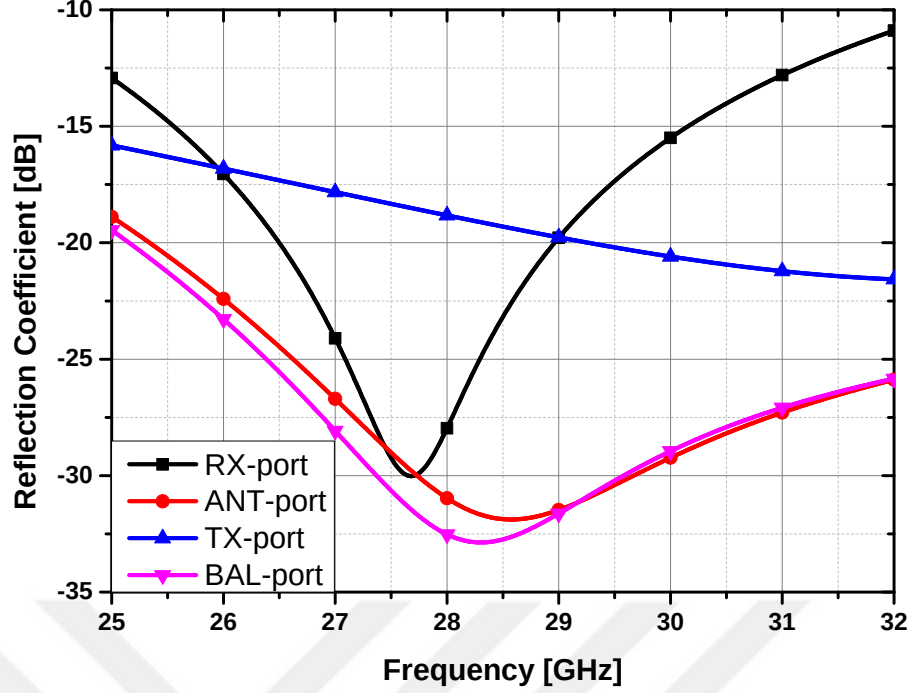
Figure 22: The reflection coefficients at each port of the designed hybrid transformer
