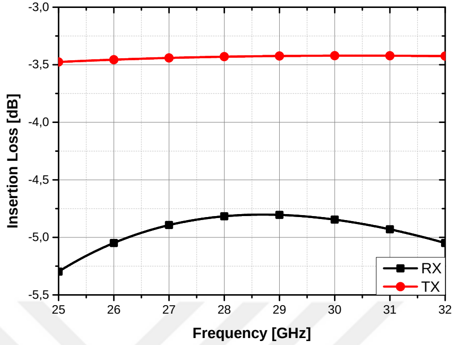
Figure 23: The insertion loss of the designed hybrid transformer in RX and TX paths
