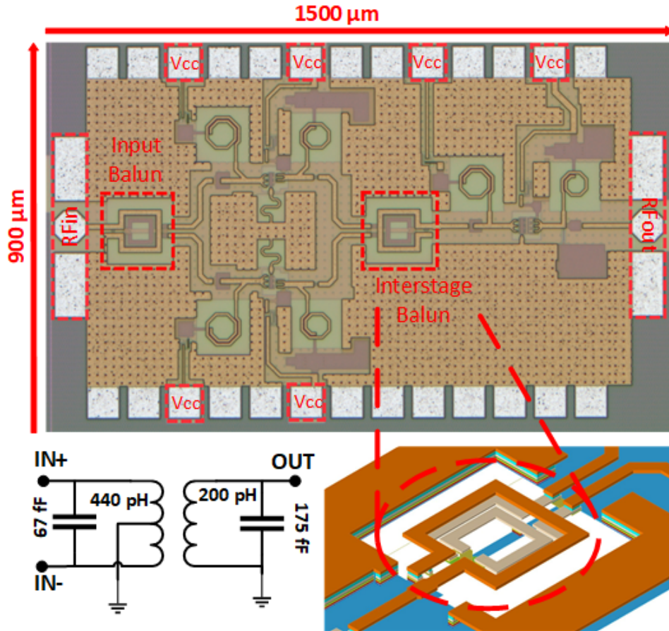
Figure 35: Chip photo of the measured LNA and schematic and 3D view of the interstage balun
