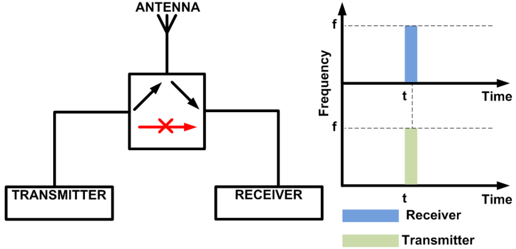
Figure 11: The block diagram and illustration of in-band full-duplex communication
