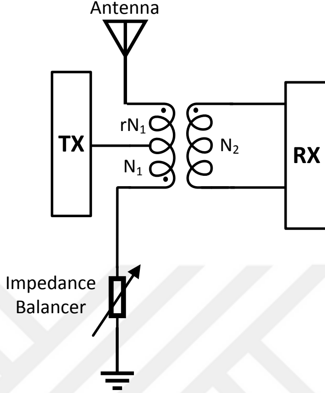
Figure 13: The block diagram of a typical EBD constructed with hybrid transformers
