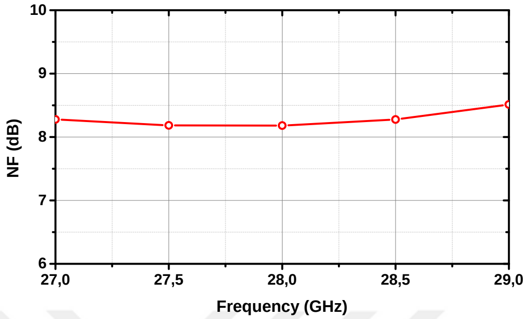
Figure 74: The NF of the receiver of the designed system
