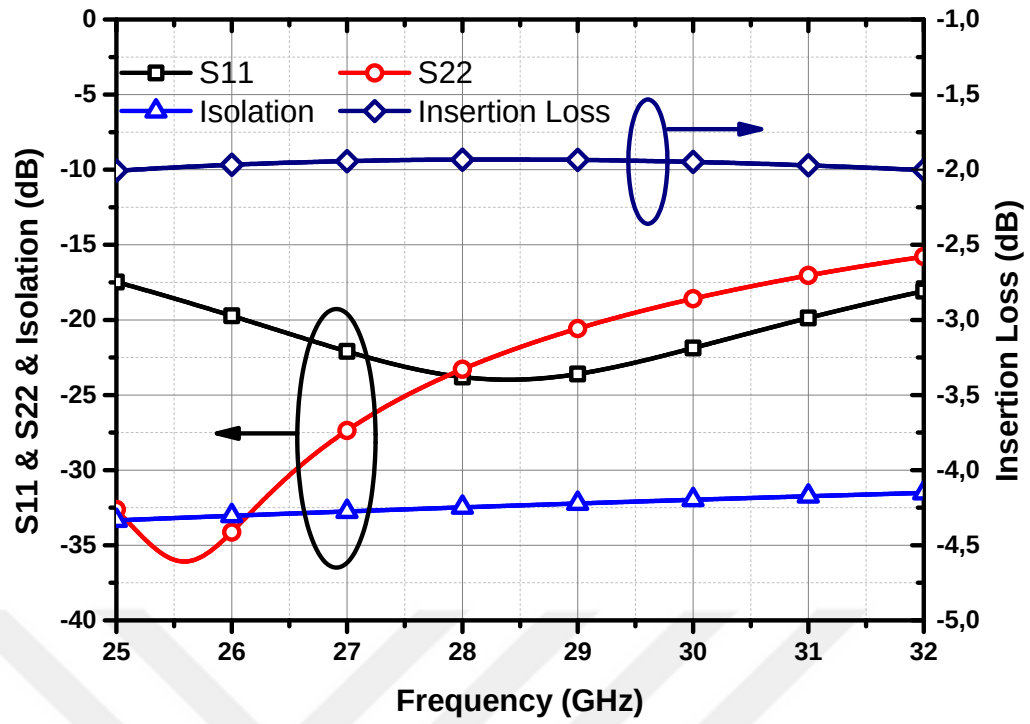
Figure 58: The S11 and S22, insertion loss and isolation of the designed SPDT
