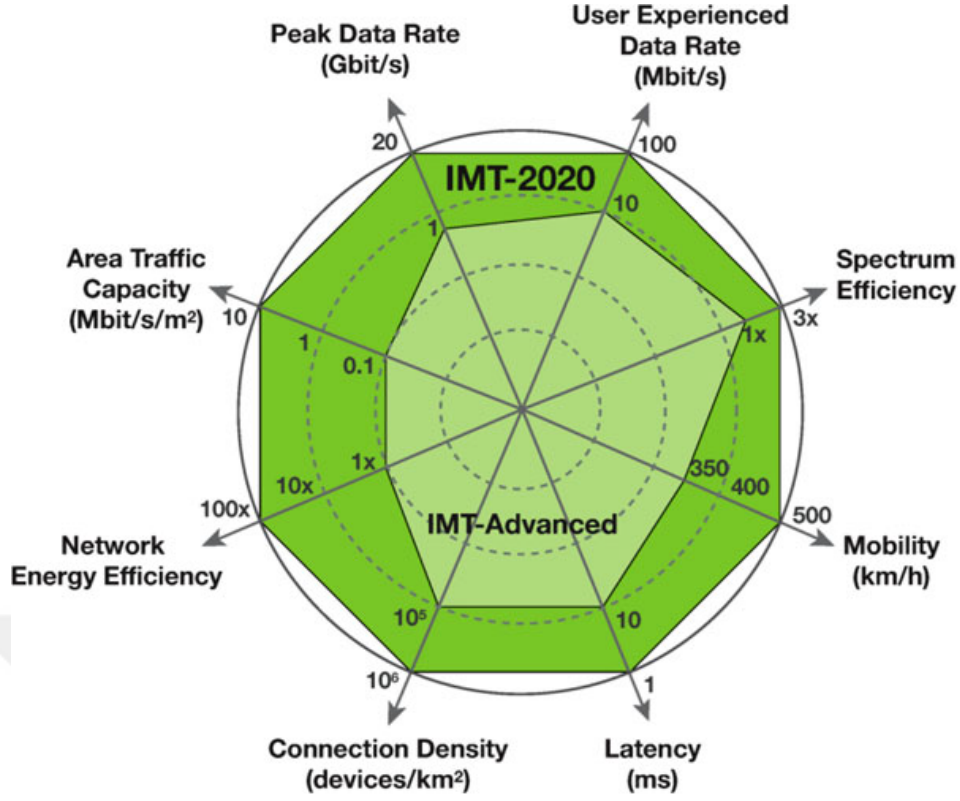
Figure 6: Improvements of significant features from IMT-Advanced to IMT-2020 [7]
