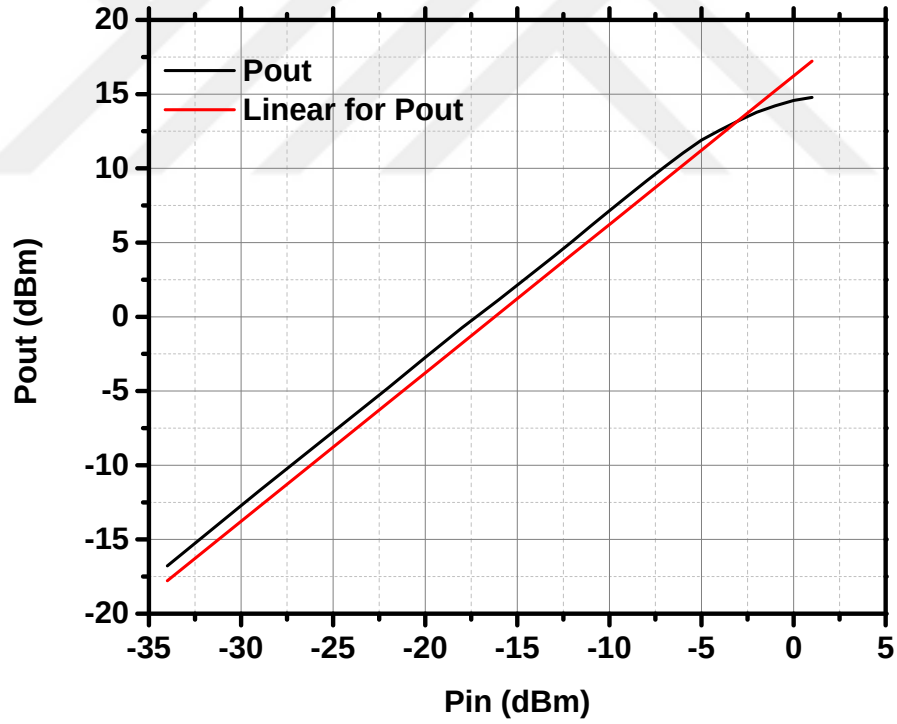
Figure 52: P_{out} vs P_{in} of the receiver
