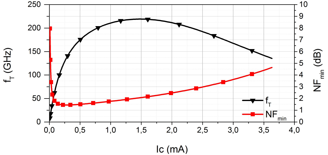
Figure 33: NF_{min} and f_T with respect to the collector current
