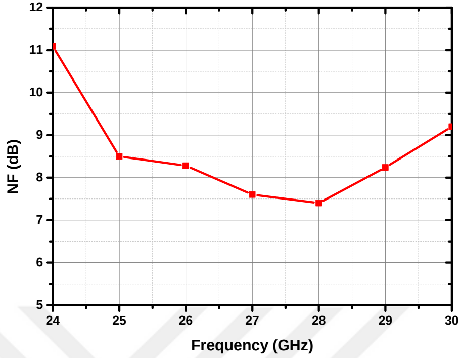
Figure 51: The NF of the receiver
