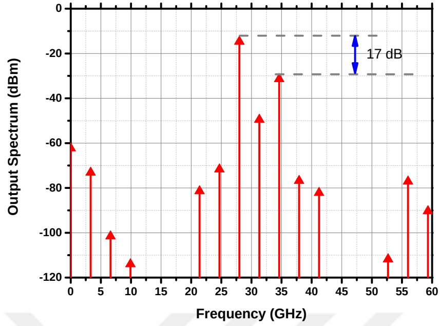
Figure 71: The output spectrum of the designed upconverter
