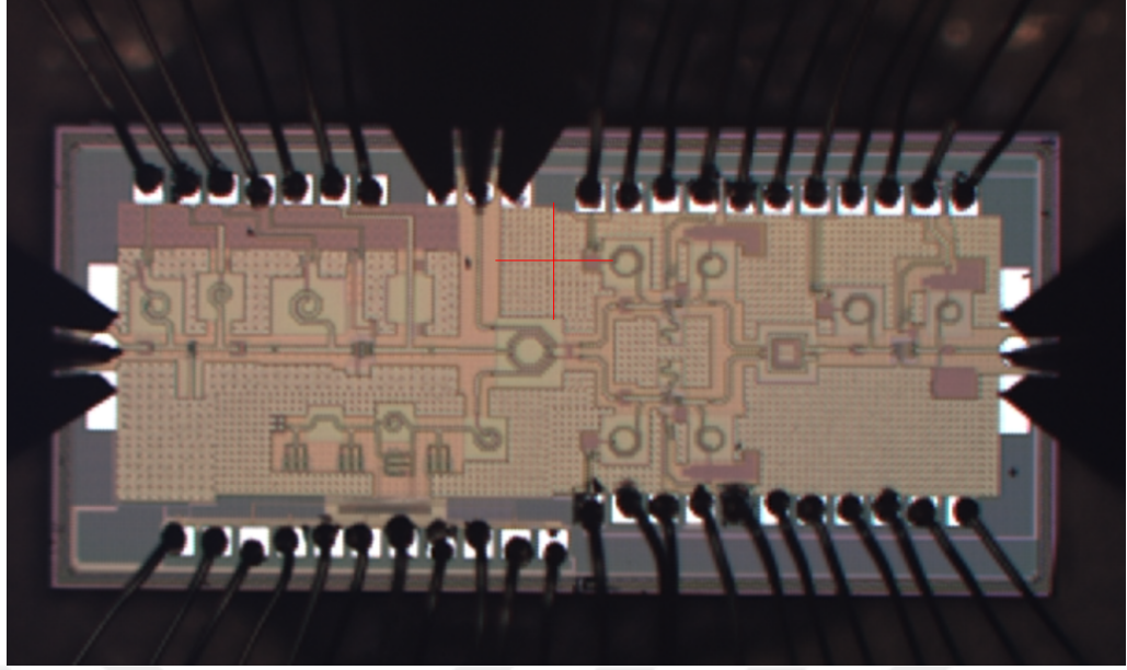
Figure 46: The chip photo of the fabricated prototype
