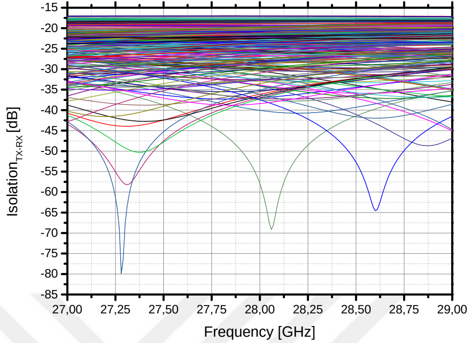
Figure 31: The isolation results for the combination of the hybrid transformer and impedance tuner ( Z_{ANT} = 50 \Omega )
