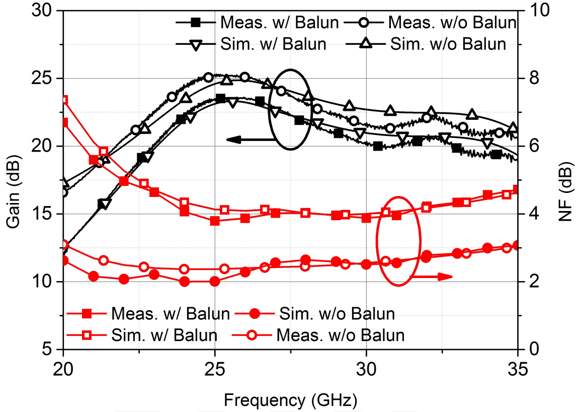
Figure 39: Measured and simulated gain and NF of the designed LNA
