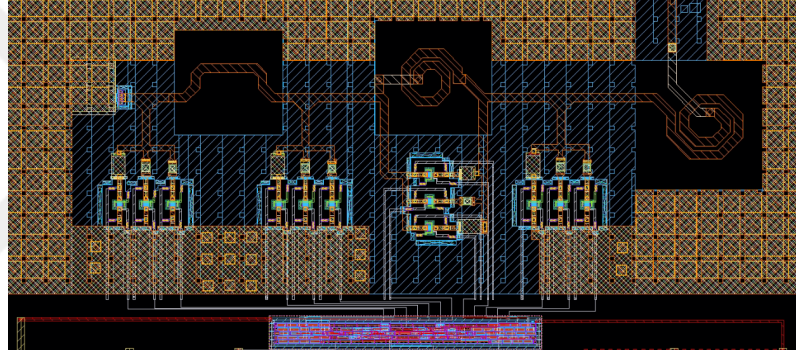
Figure 29: The layout of the designed impedance tuner with digital control circuit
