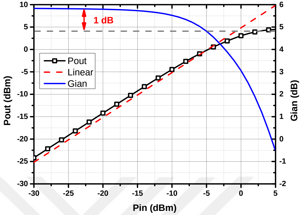
Figure 76: The RX output power and gain of the designed system with respect to the input power
