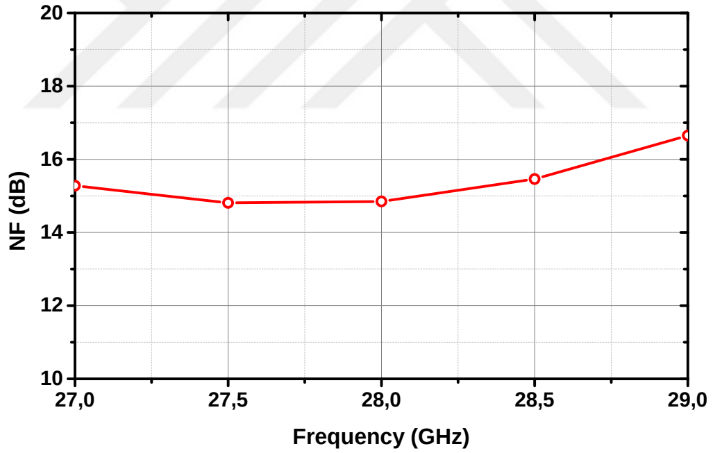
Figure 64: The SSB NF of the designed downconverter
