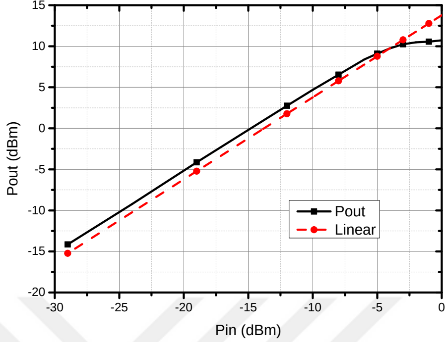
Figure 53: P_{out} vs P_{in} of the transmitter
