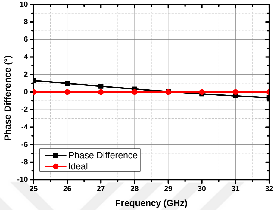
Figure 25: The phase difference between RX ports
