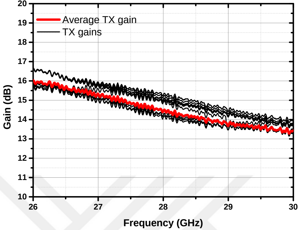
Figure 48: Sampled ten TX-gains with the average of all the TX gains of the prototype
