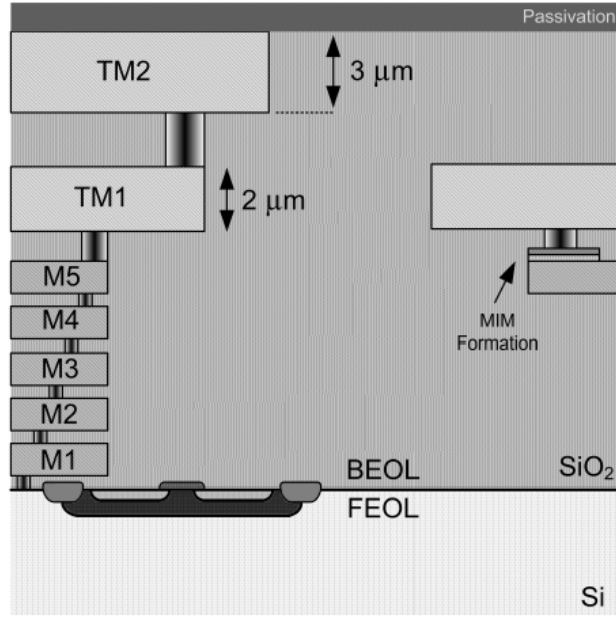
Figure 8: The cross-section of IHP's 0.13 \mu\text{m} SiGe BiCMOS SG13S technology [10]
