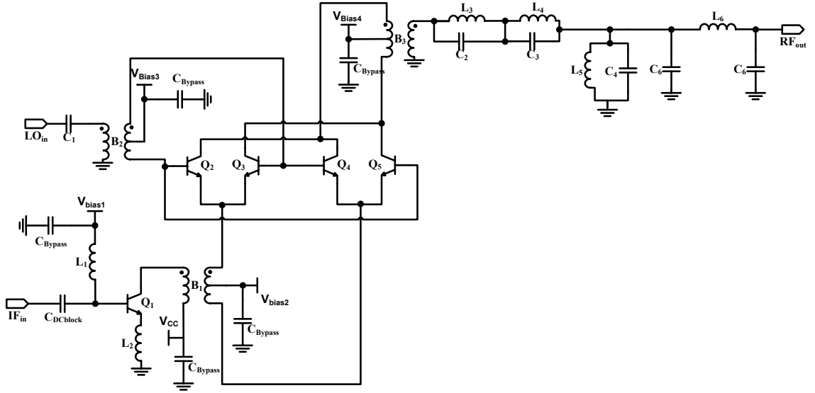
Figure 66: The schematic of the designed upconverter
