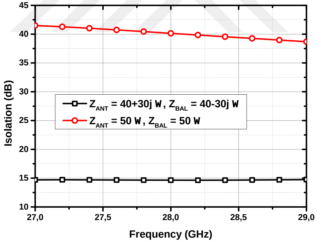
Figure 77: The isolation between the TX and RX ports of the designed system
