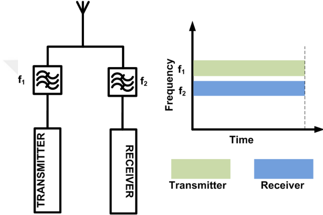
Figure 10: The block diagram and illustration of full-duplex communication
