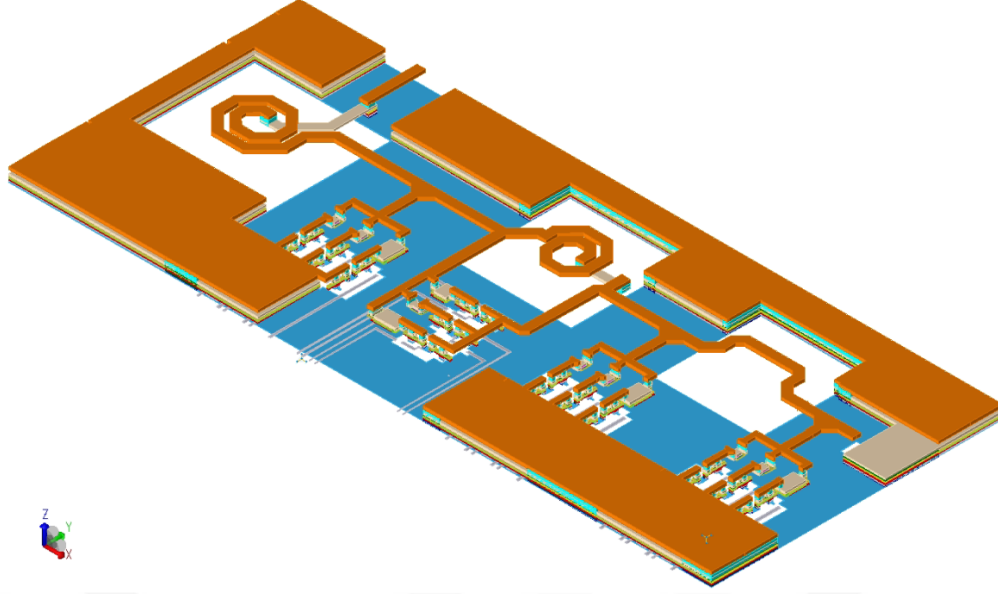
Figure 28: The 3D view of the designed impedance tuner
