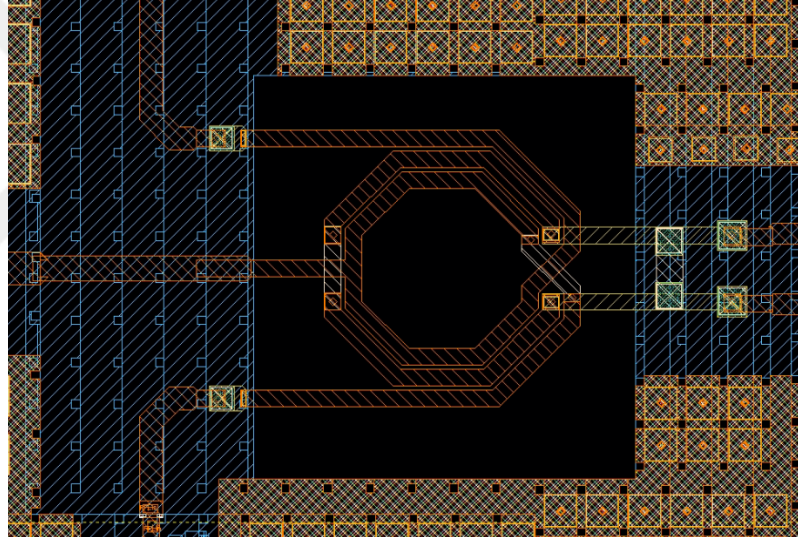
Figure 21: The layout of the designed hybrid transformer
