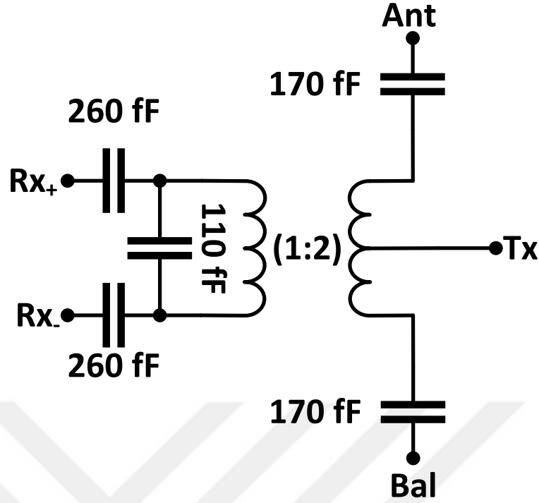
Figure 19: The schematic of the designed hybrid transformer
