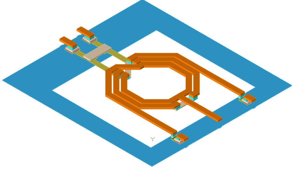
Figure 20: The 3D view of the designed hybrid transformer
