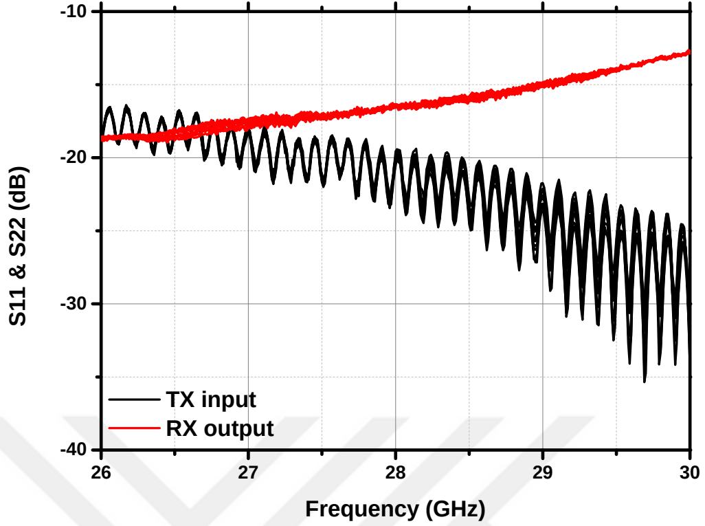
Figure 47: The return losses of TX-input and RX-output of the prototype
