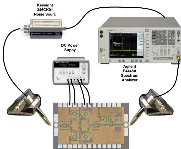
Figure 36: Noise measurement setup
