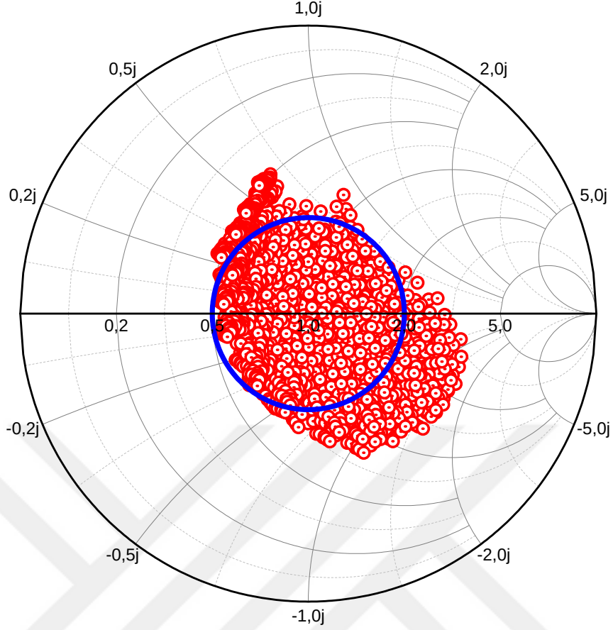
Figure 30: The impedances covered by the impedance tuner at 28 GHz
