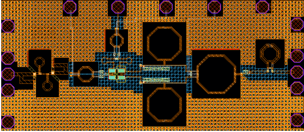
Figure 61: The layout of the designed downconverter
