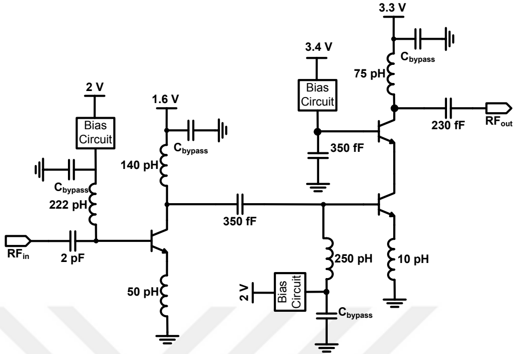
Figure 41: The schematic of the designed PA
