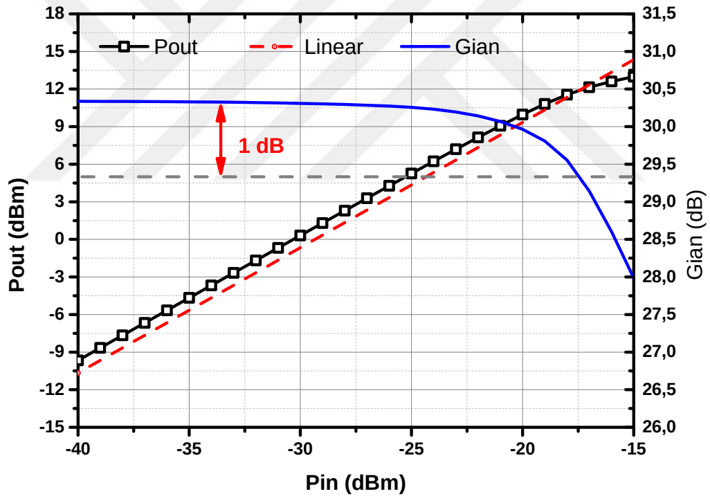
Figure 75: The TX output power and gain of the designed system with respect to the input power
