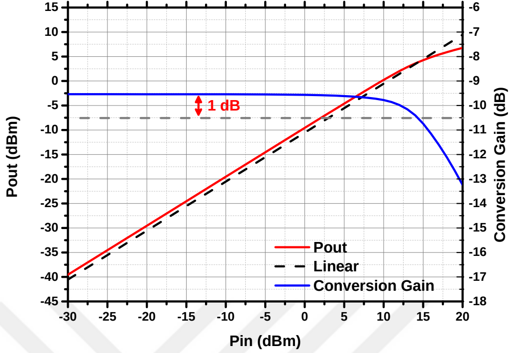
Figure 65: P_{out} vs P_{in} of the designed downconverter
