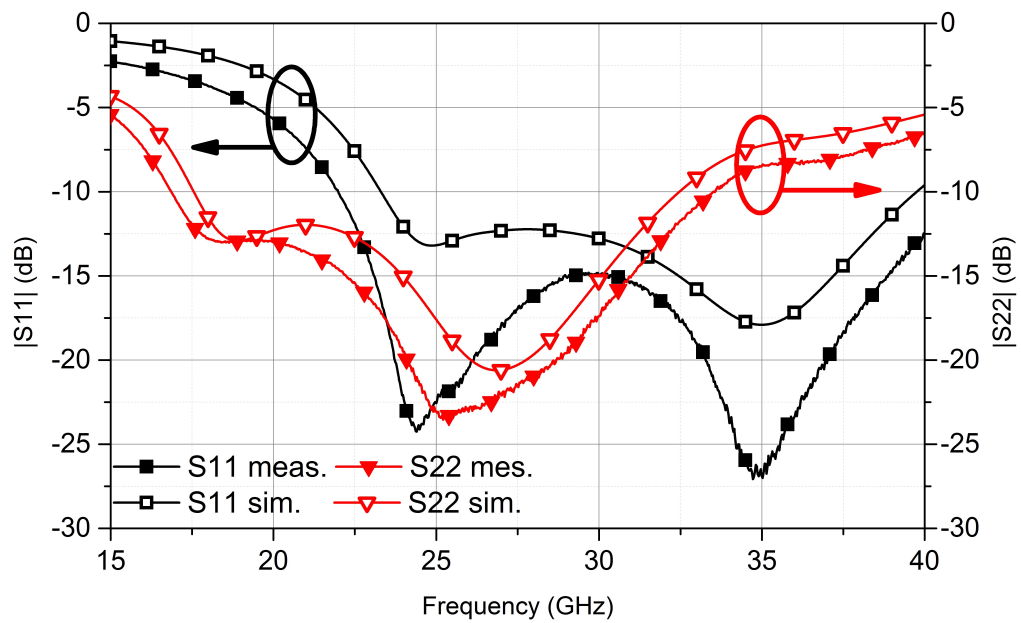
Figure 38: Input and output matchings of the designed LNA
