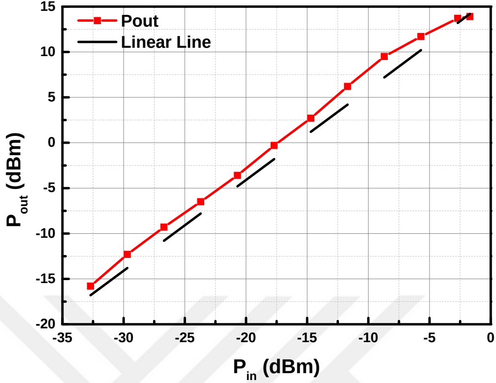
Figure 45: P_{out} vs P_{in} of the designed PA
