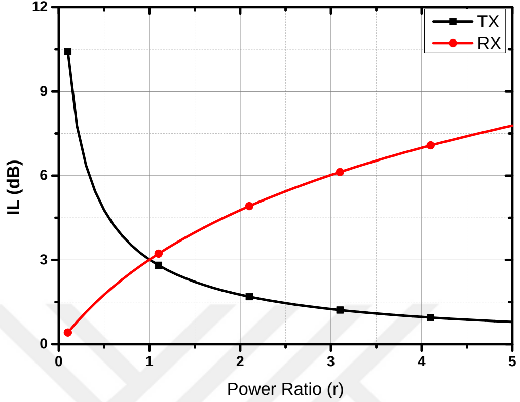
Figure 14: The insertion loss of the hybrid transformer in TX and RX path with respect to the power ratio
