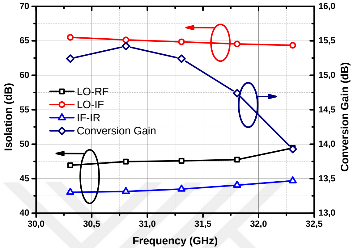
Figure 69: The port isolations and convergence gain of the designed up-converter
