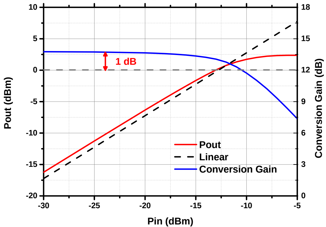
Figure 70: P_{out} vs P_{in} of the designed upconverter
