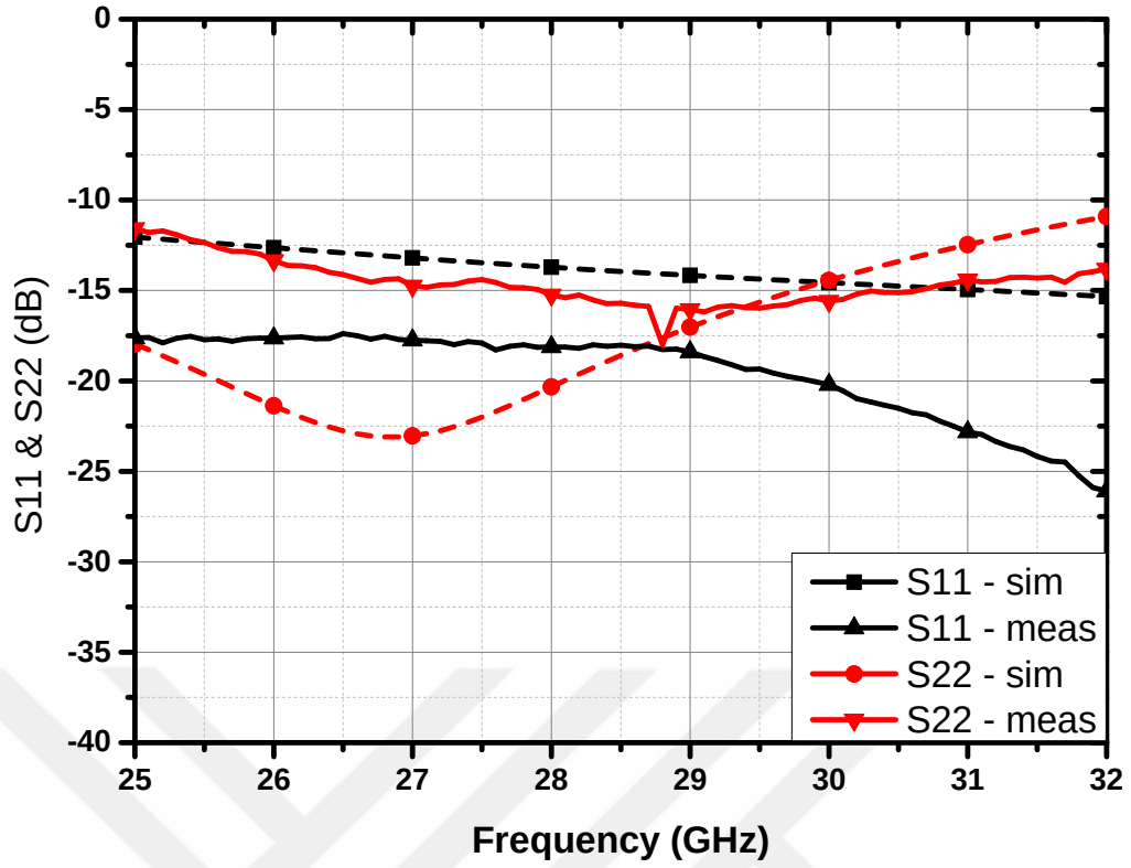
Figure 43: The return losses of the designed PA
