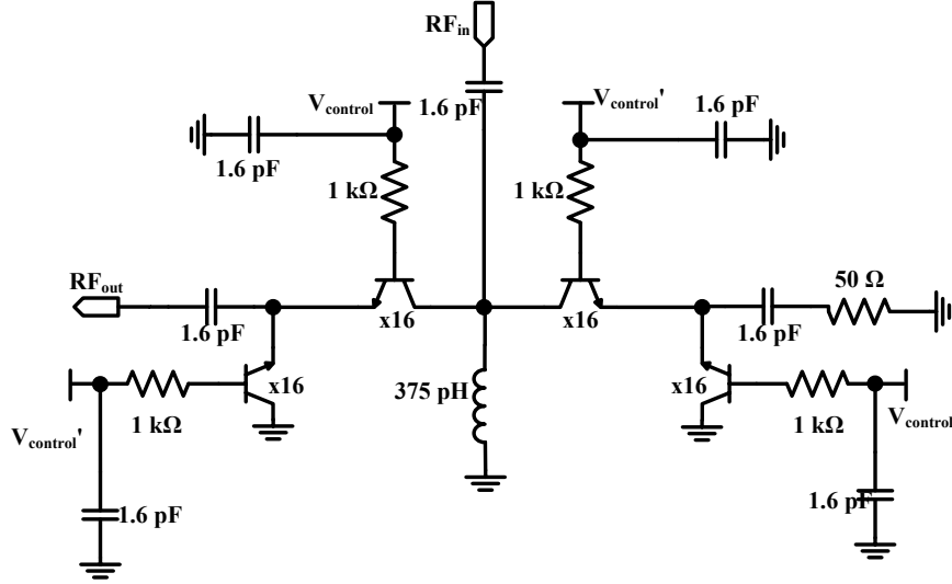
Figure 56: The schematic of the designed SPDT
