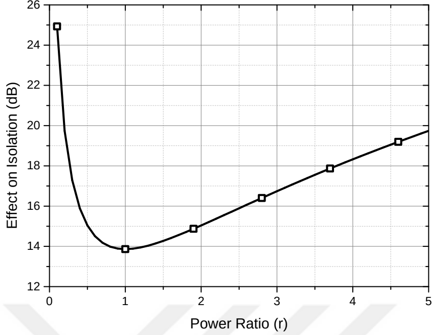
Figure 18: The effect of the power ratio on the isolation
