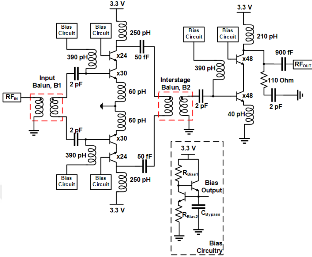
Figure 32: The schematic of LNA
