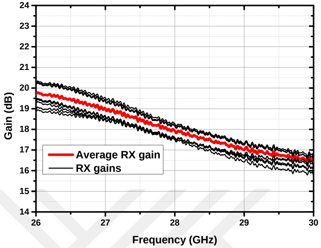
Figure 49: Sampled ten RX-gains with the average of all the RX gains of the prototype
