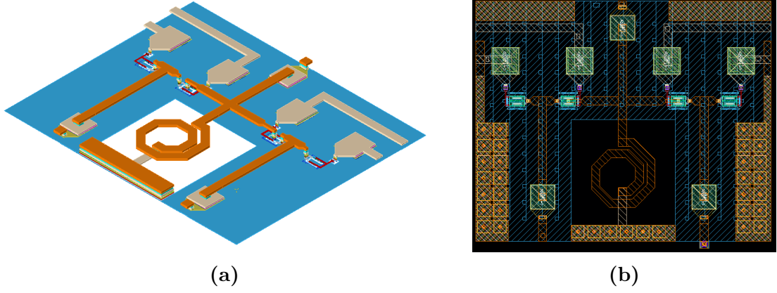
Figure 57: The 3D view (a) and layout (b) view of the designed SPDT
