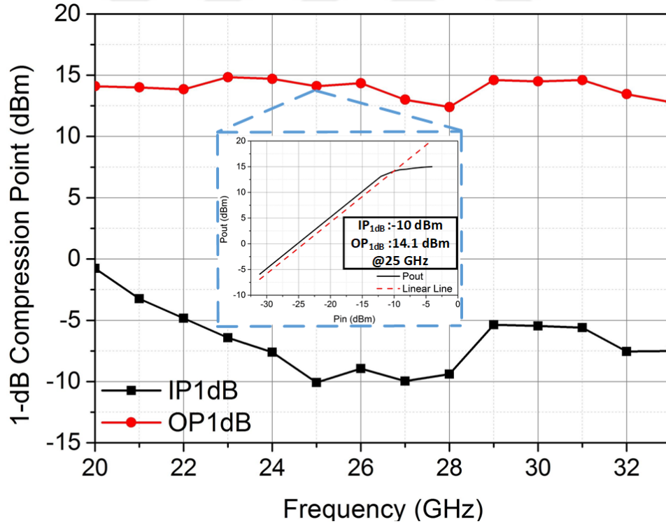
Figure 40: The measured IP 1dB and OP 1dB of the LNA
