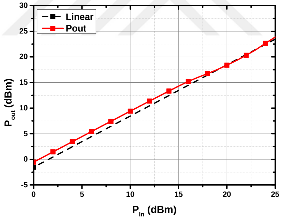
Figure 59: P_{out} vs P_{in} of the SPDT
