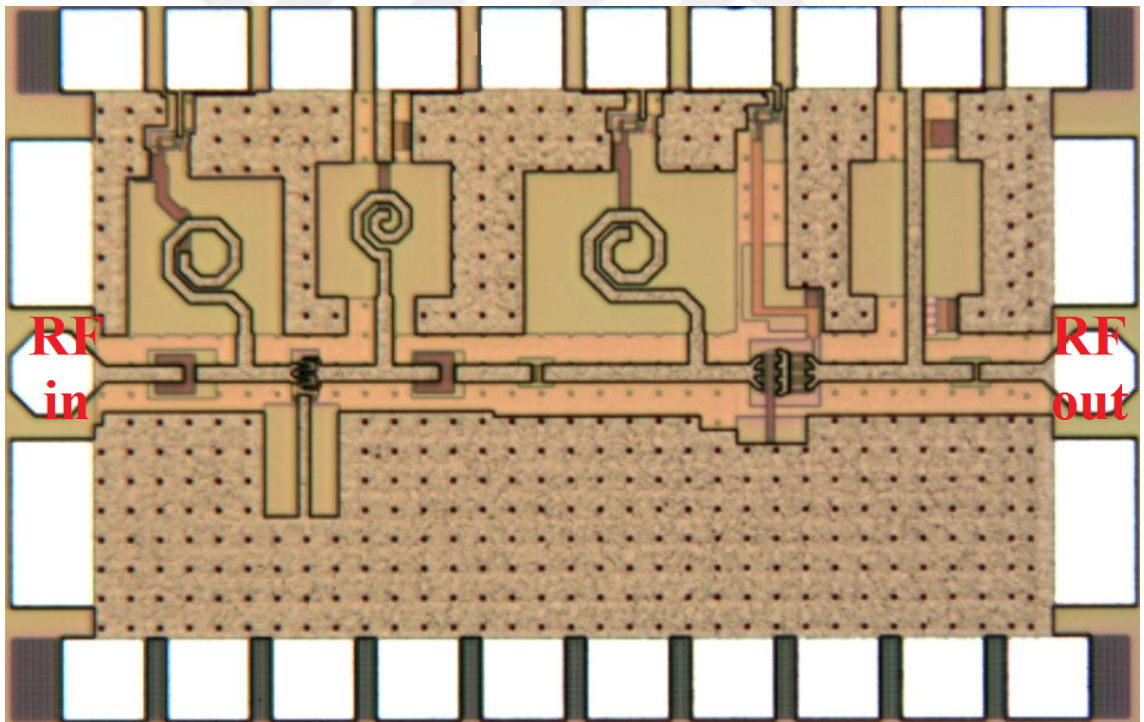
Figure 42: The chip photo of the designed PA
