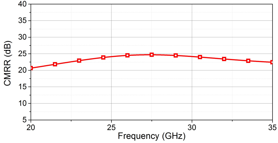
Figure 34: The simulated common-mode rejection ratio of LNA
