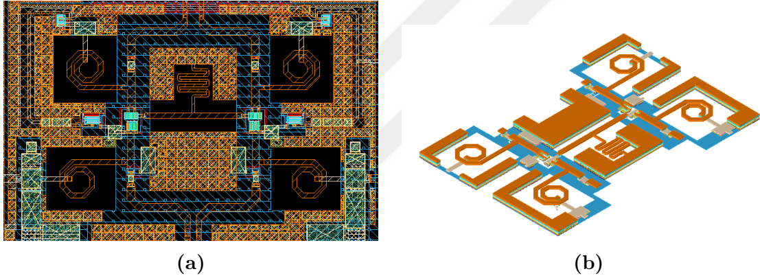
Figure 55: The layout (a) and 3D view (b) of the first stage of the updated LNA
