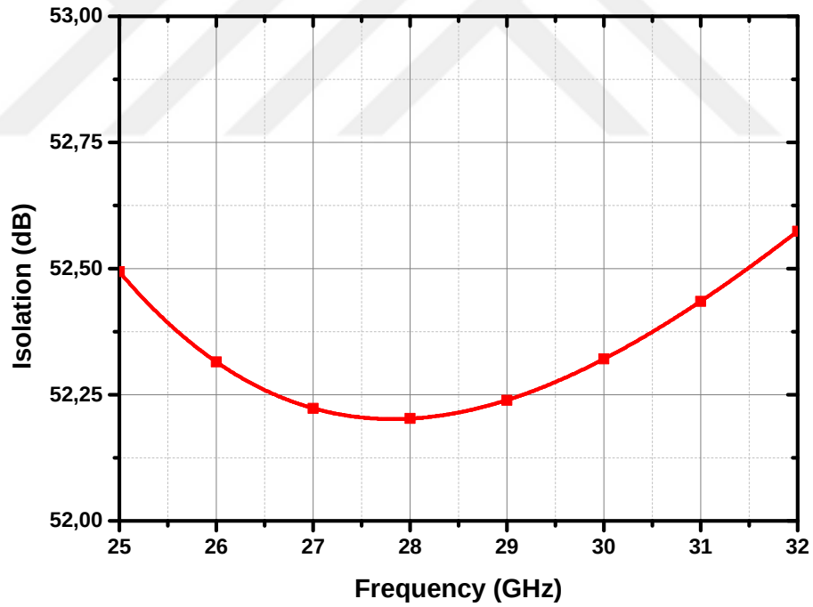
Figure 24: The isolation between of the designed hybrid transformer TX and RX ports
