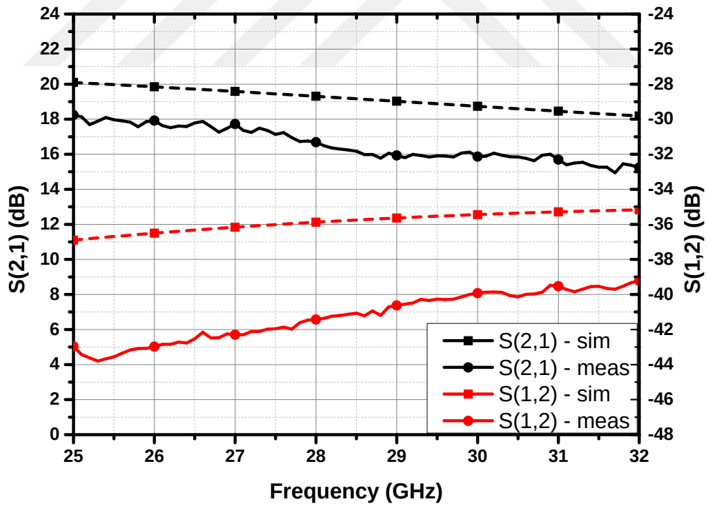
Figure 44: The forward and reverse gain of the designed PA
