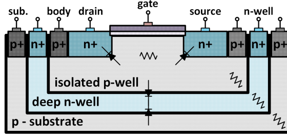
Figure 27: The cross-section view of the isolated NMOS [23]
