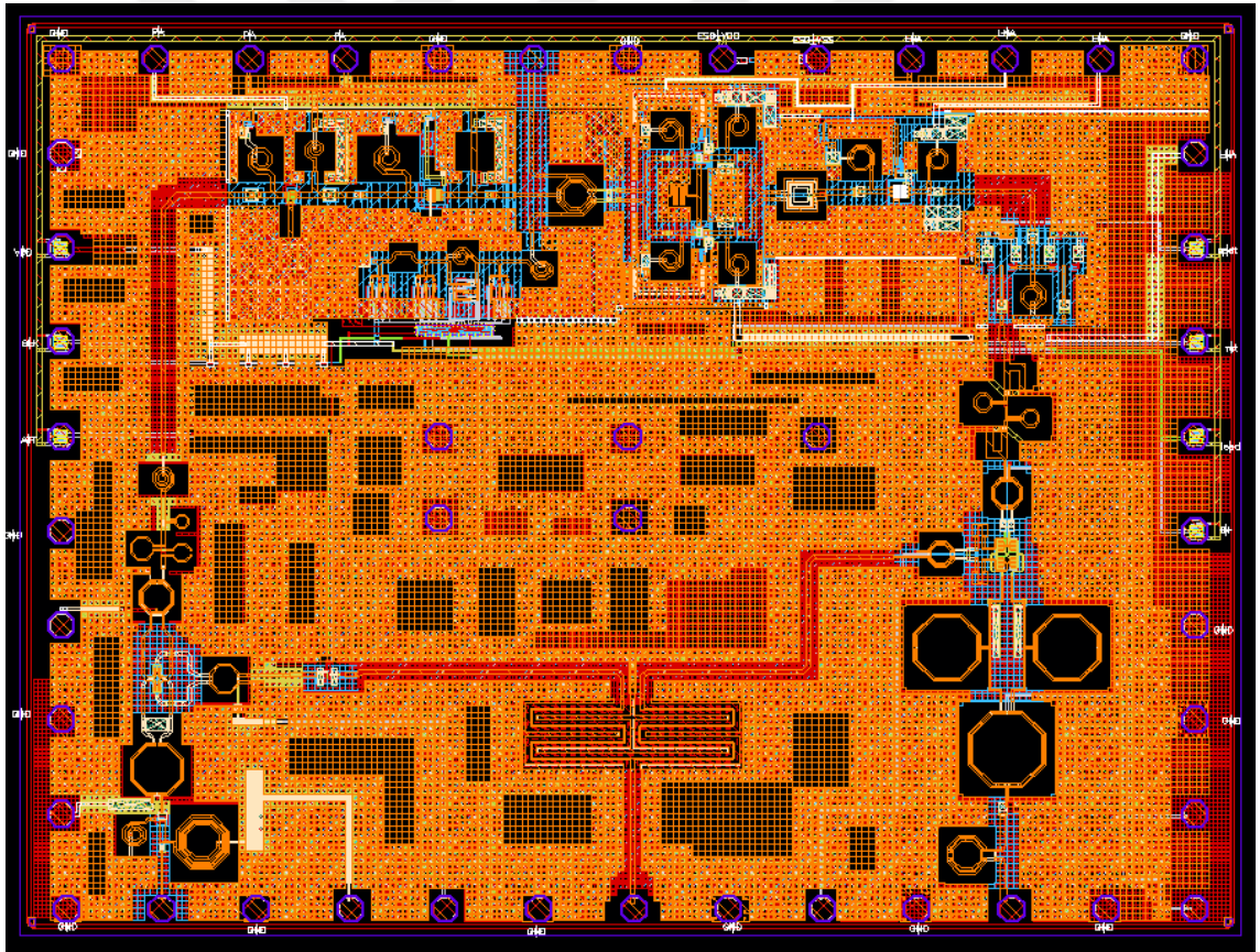
Figure 72: The layout of the designed system
