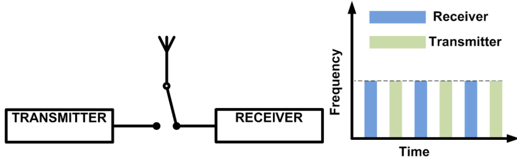
Figure 9: The block diagram and illustration of half-duplex communication
