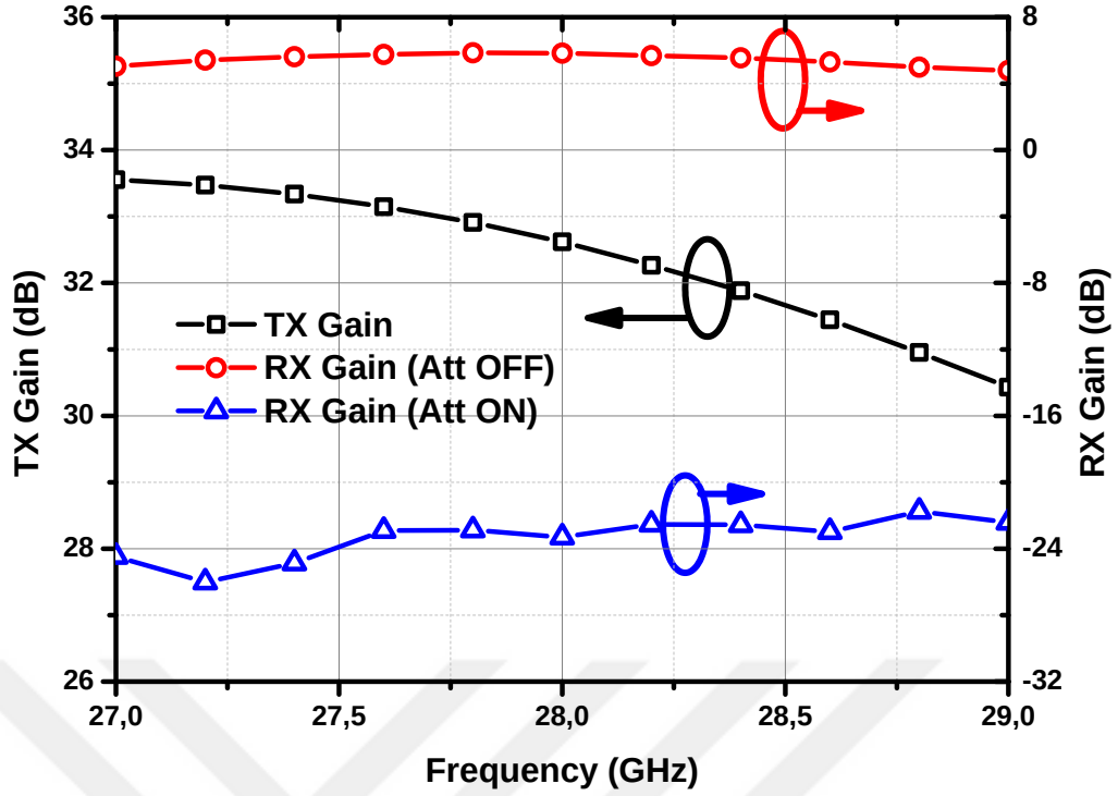
Figure 73: The TX and RX gain performances of the designed system
