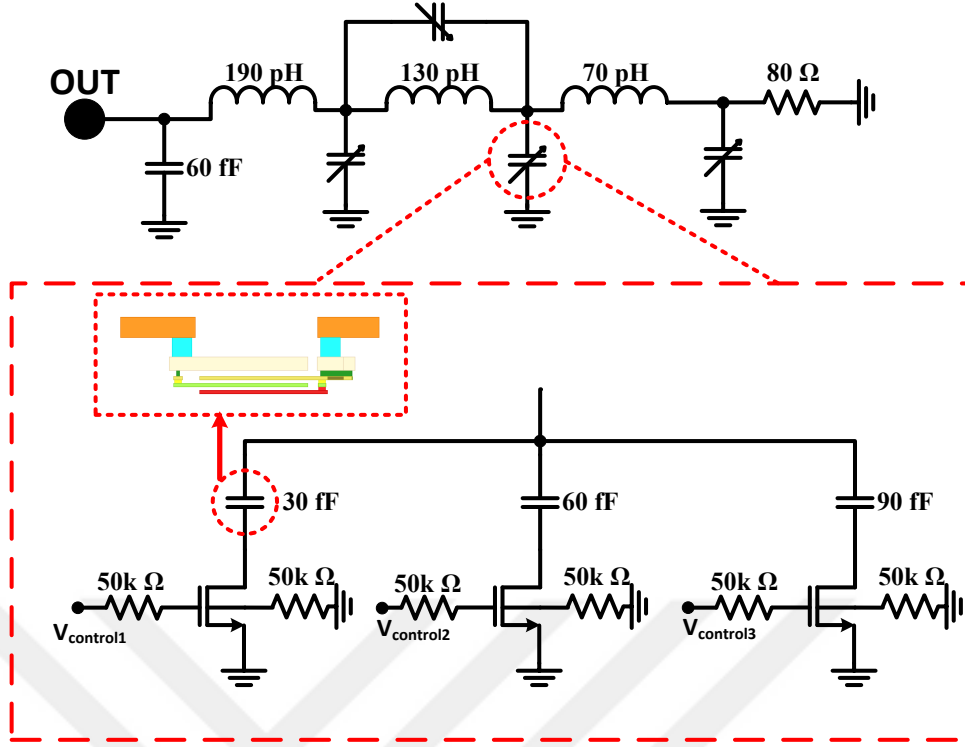
Figure 26: The schematic of the designed impedance tuner
