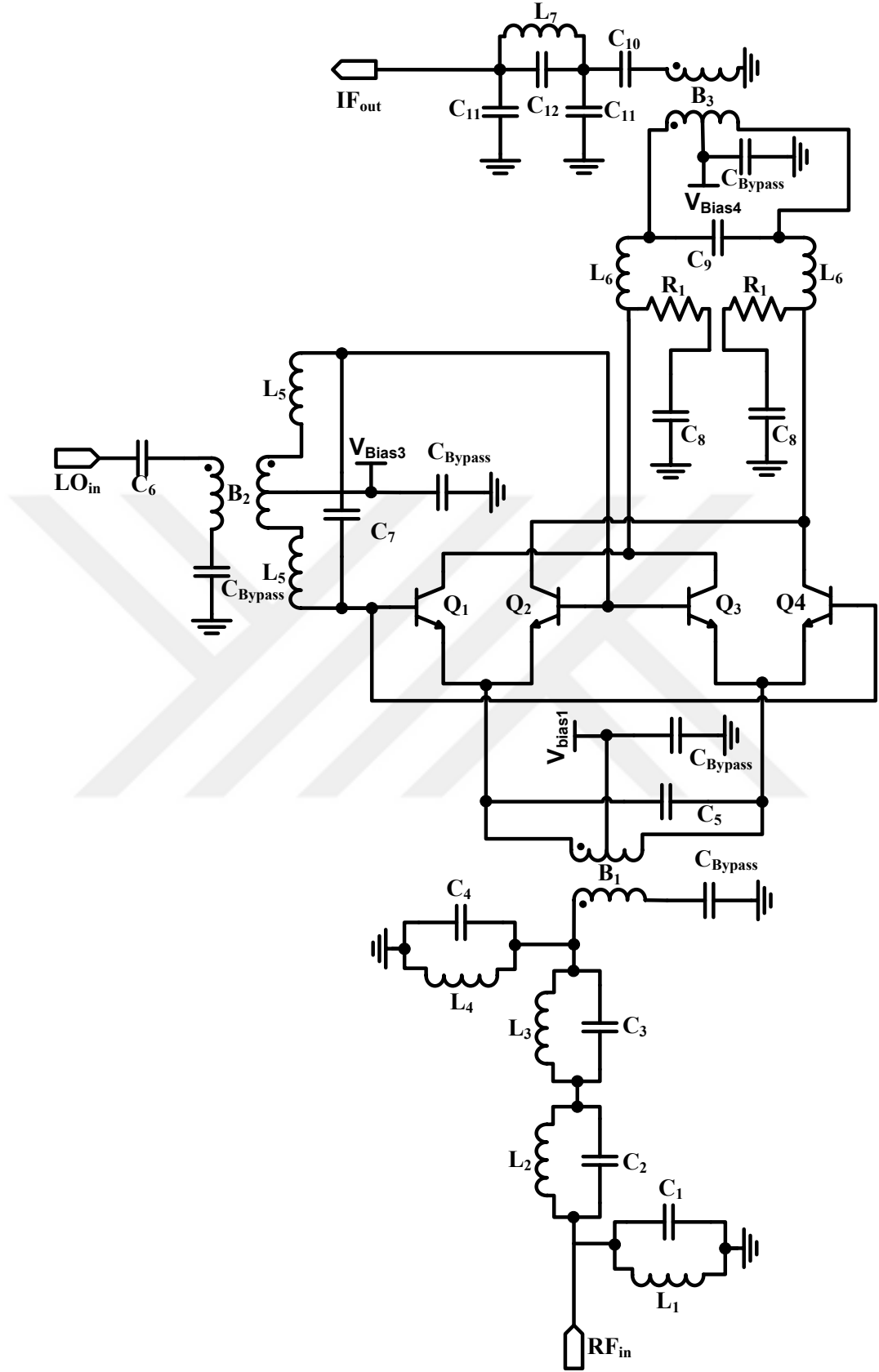
Figure 60: The schematic of the designed downconverter
