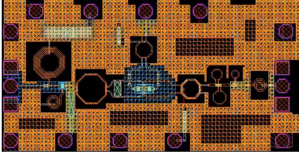
Figure 67: The layout of the designed upconverter
