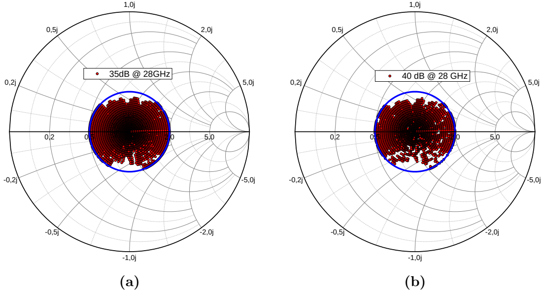
Figure 54: The antenna impedances that 35 dB (a) and 40 dB (b) of isolation is obtained
