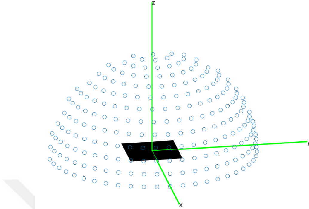
Figure 2.5: Far-field points (blue) on a quarter sphere.
