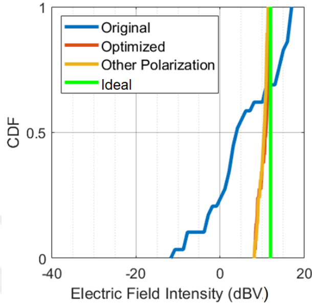
Figure 3.10: Sensitivity of the optimized surface to polarization in terms of the CDF.
