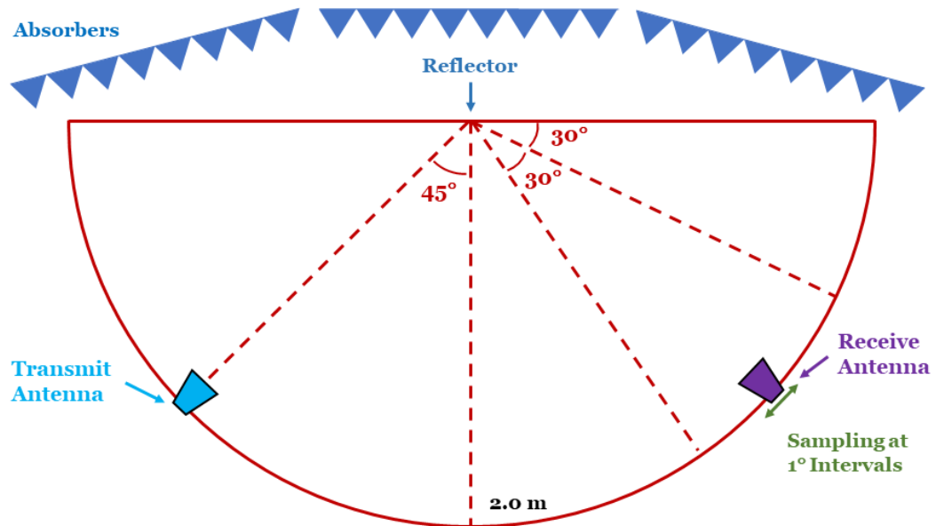
Figure 4.15: A schematic diagram of the free-space measurement setup.
