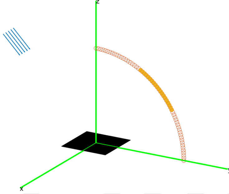
Figure 3.3: Optimization setup for redirecting incident fields towards a set of directions in a single cut.
