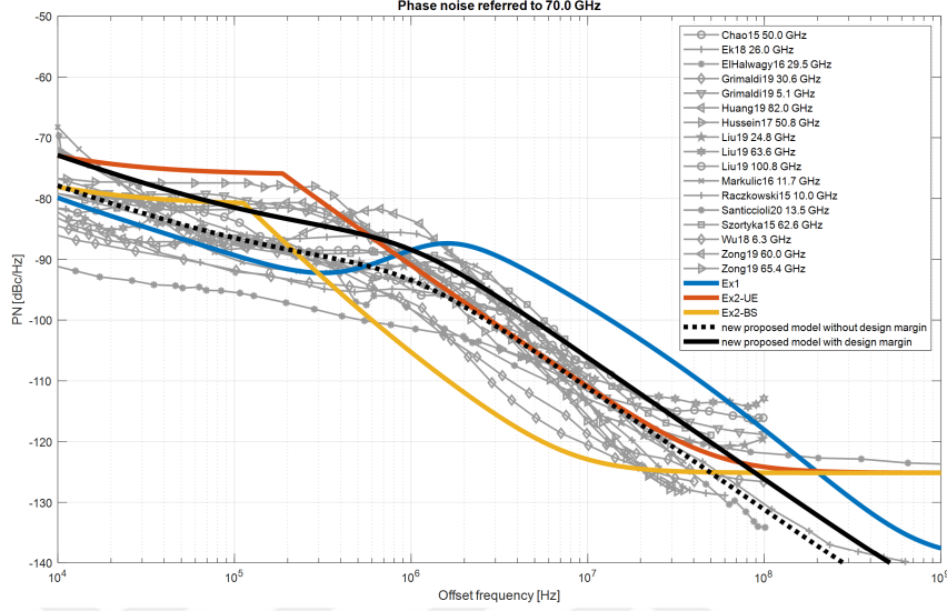
Figure 2.2: Phase Noise PSD models [4].
