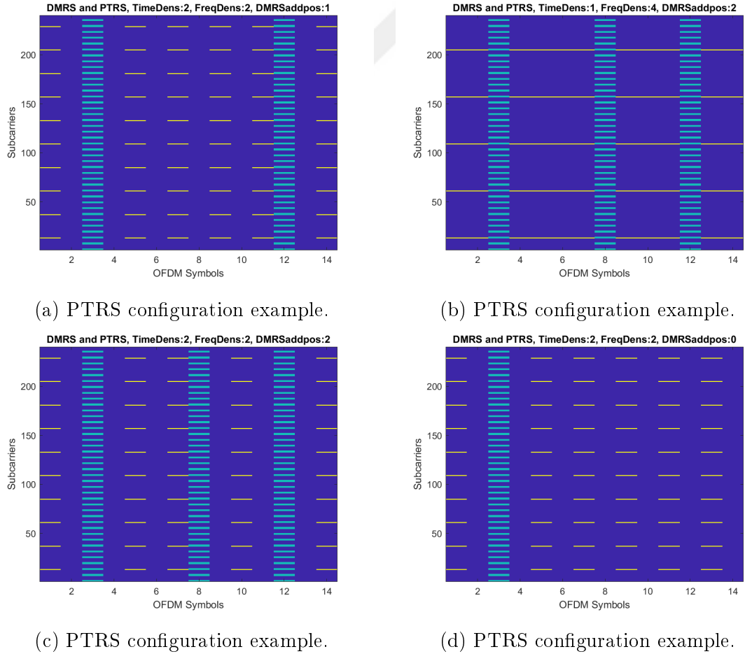
Figure 1.5: OFDM grid generation examples in MATLAB for different PTRS time density and additional DMRS position parameters.
