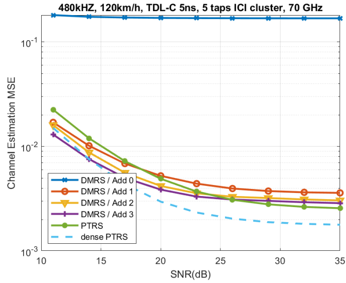
Figure 4.11: Channel estimation MSE for TDL-C channel with 5 ns of delay spread for 120 km/h user speed.
