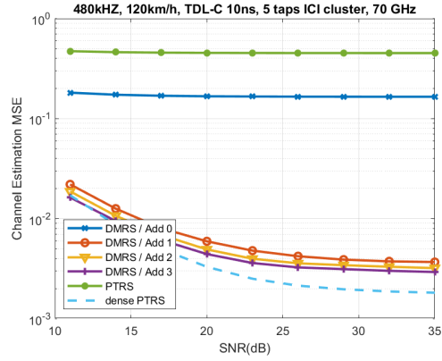
(c) Channel estimation MSE for 120 km/h.
