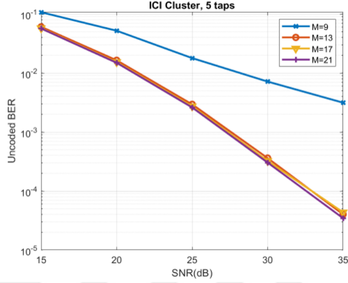
Figure 4.3: Performance results for ICIclust algorithm with ICI filter length of 5 for changing M .
