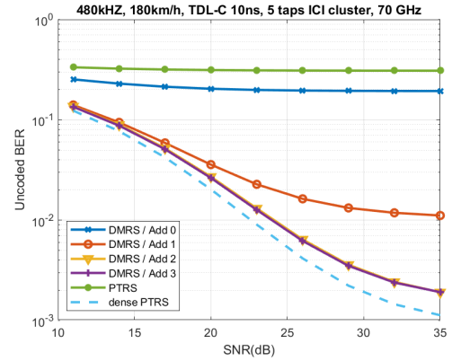
(f) Uncoded BER for 180 km/h.
