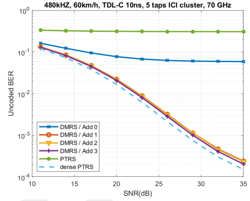
(b) Uncoded BER for 60 km/h.
