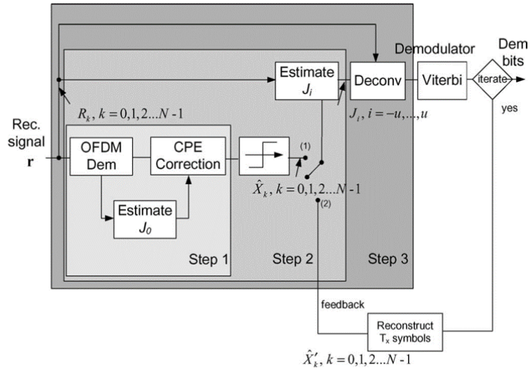
Figure 3.2: Data-aided ICI filter approximation algorithm [5].
