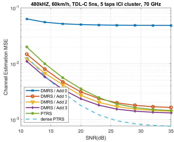
Figure 4.10: Channel estimation MSE for TDL-C channel with 5 ns of delay spread for 60 km/h user speed.
