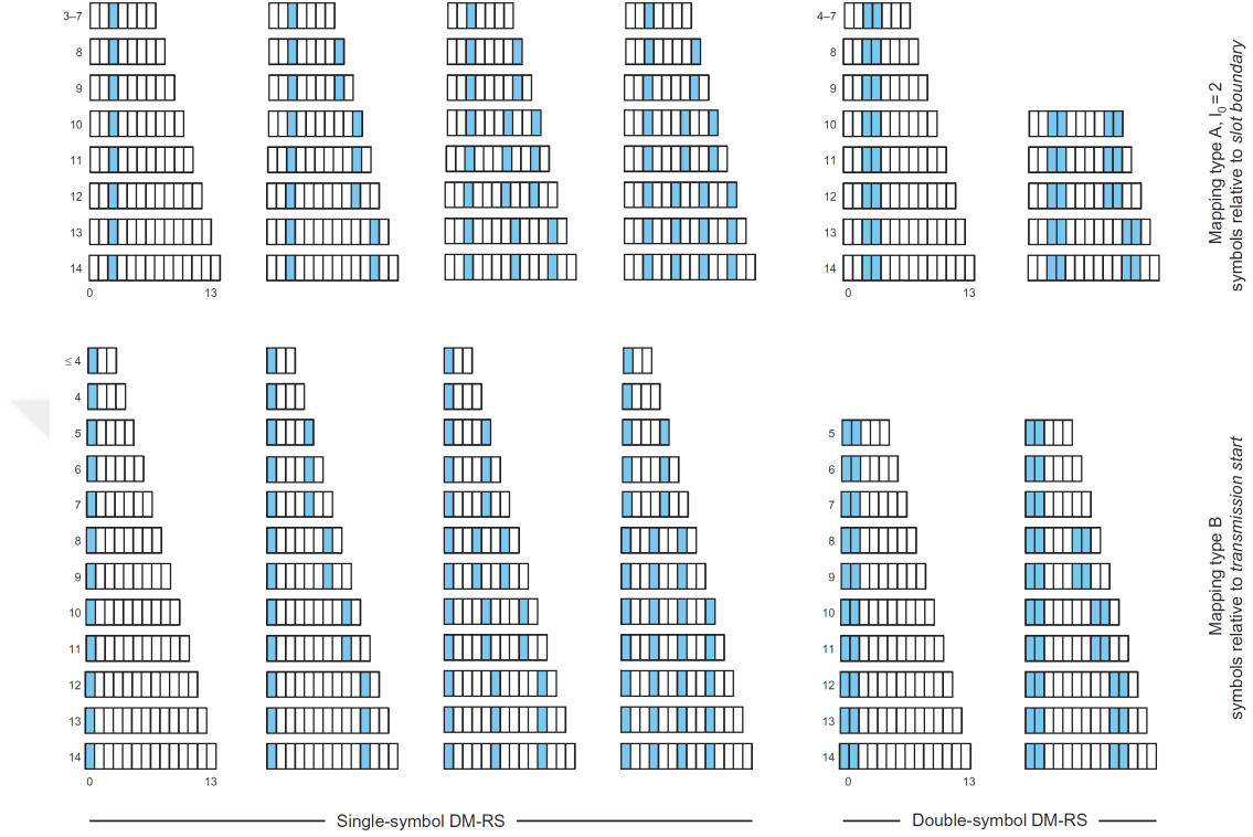
Figure 1.4: DMRS time locations for different configuration parameters [2].
