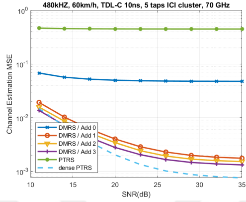
(a) Channel estimation MSE for 60 km/h.
