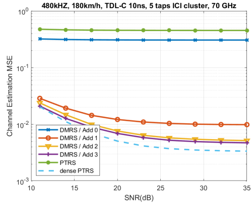
(e) Channel estimation MSE for 180 km/h.
