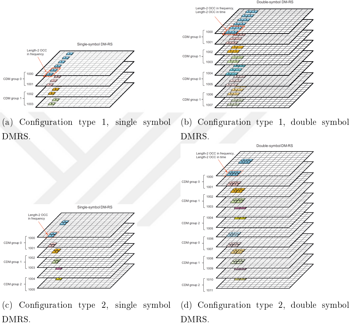
Figure 1.3: DMRS locations in slot for different configuration parameters [2].
