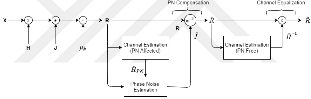
Figure 3.1: System model diagram.
