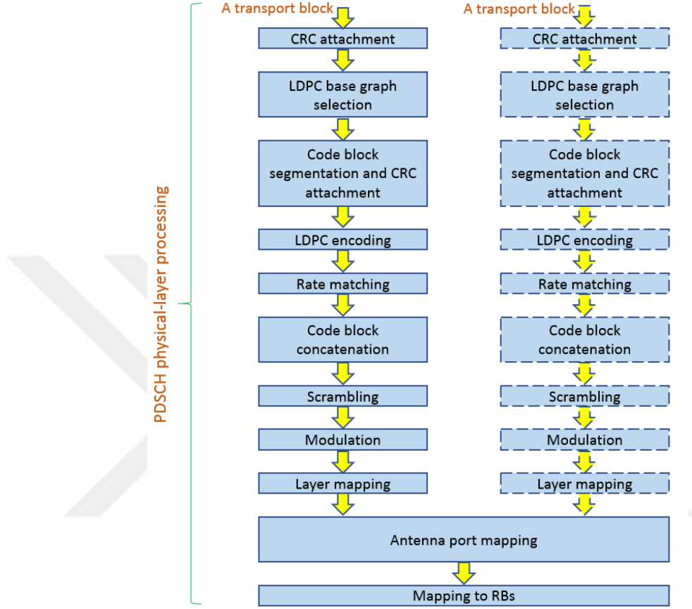
Figure 1.2: 5G PDSCH physical layer processing [1].
