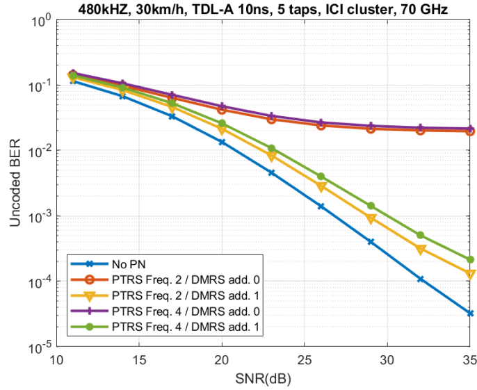
Figure 4.6: The effect of N_{\text{add}}^{\text{DMRS}} and d_{\text{freq}}^{\text{PTRS}} for 30 km/h user speed.
