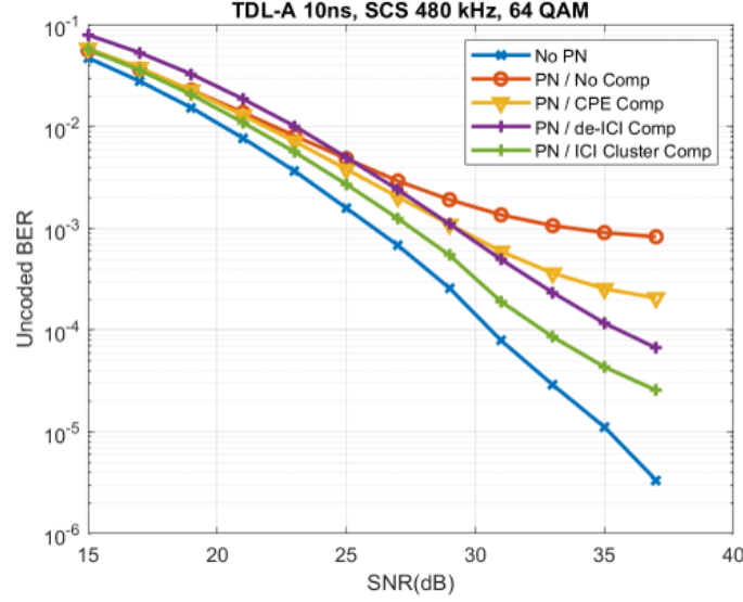
Figure 4.1: General comparison of the algorithms.
