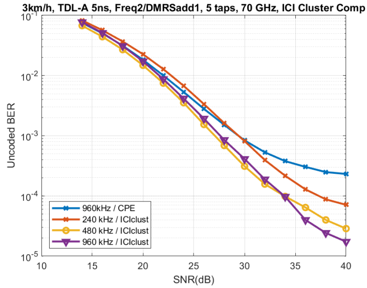
Figure 4.8: Performance results of different subcarrier spacing for ICI filter approximation algorithm.
