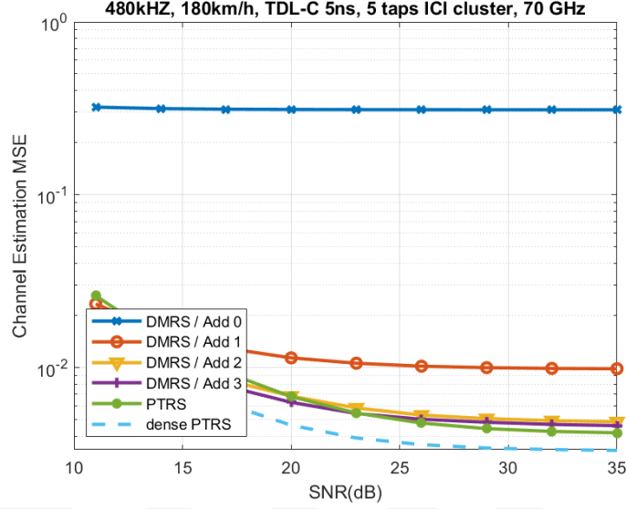
Figure 4.12: Channel estimation MSE for TDL-C channel with 5 ns of delay spread for 180 km/h user speed.
