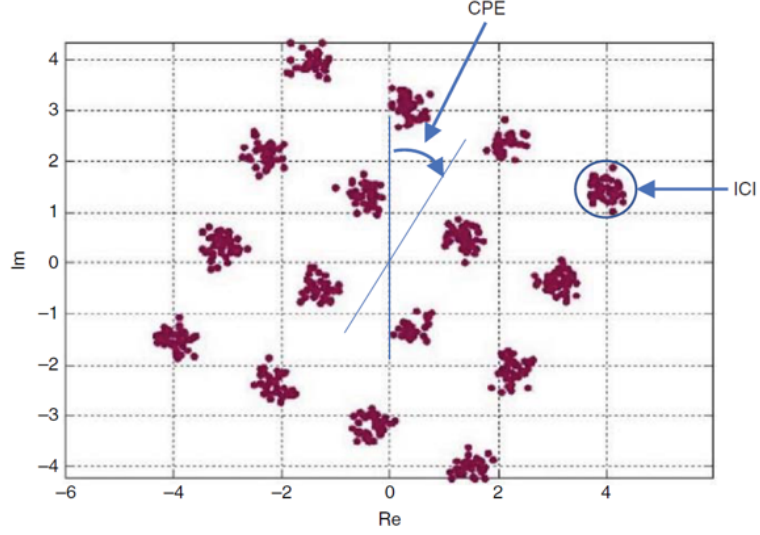
Figure 1.6: CPE and ICI effects on the received constellation [3].
