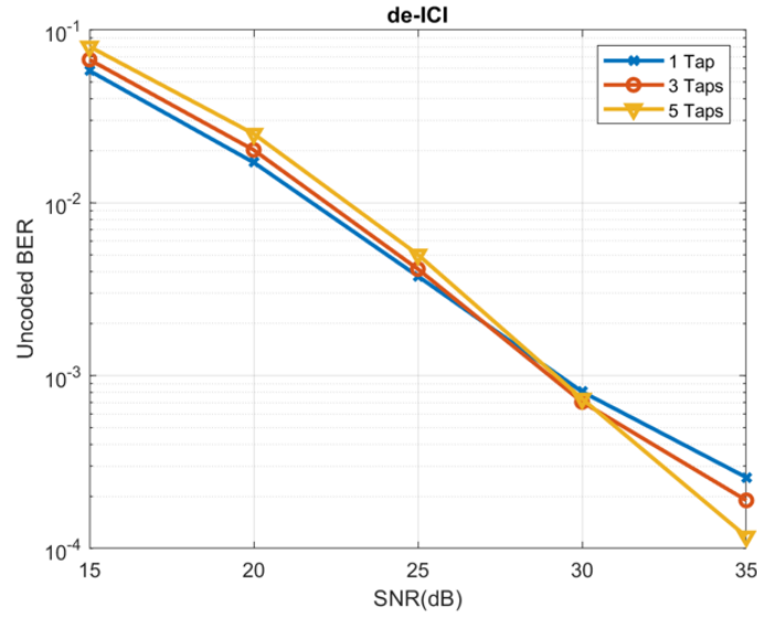
Figure 4.4: Performance results for de-ICI algorithm for changing ICI filter length.
