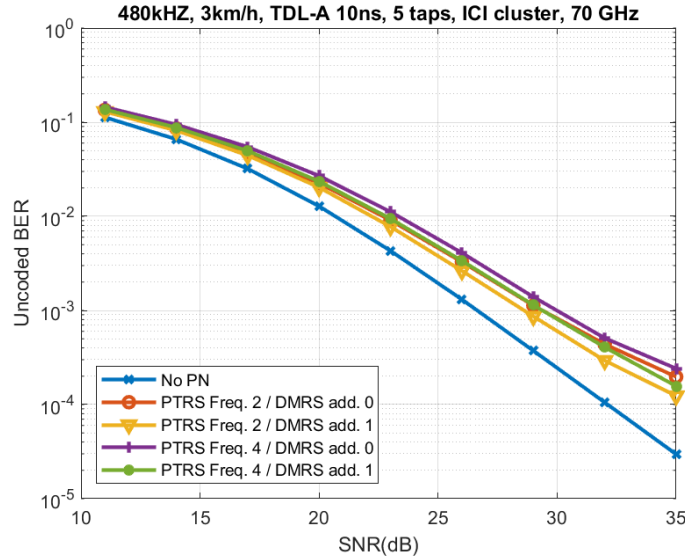
Figure 4.5: The effect of N_{\text{add}}^{\text{DMRS}} and d_{\text{freq}}^{\text{PTRS}} for 3 km/h user speed.
