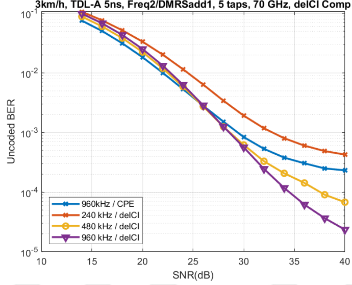
Figure 4.7: Performance results of different subcarrier spacing for direct de-ICI filtering algorithm.
