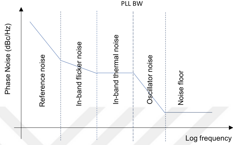
Figure 2.1: PLL phase noise model for different frequency offsets [4].
