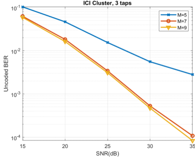
Figure 4.2: Performance results for ICIclust algorithm with ICI filter length of 3 for changing M.
