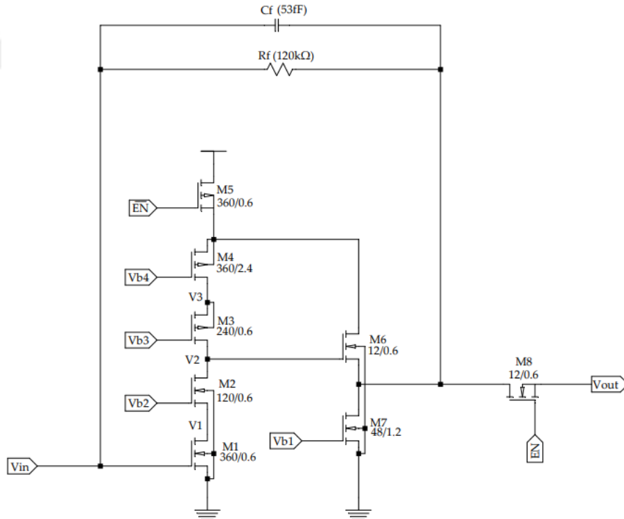
Figure 3.3: Cascode Common Source Amplifier Multiplexer Topology
