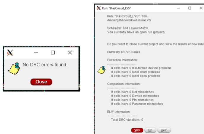
Figure 4.1: DRC and LVS
