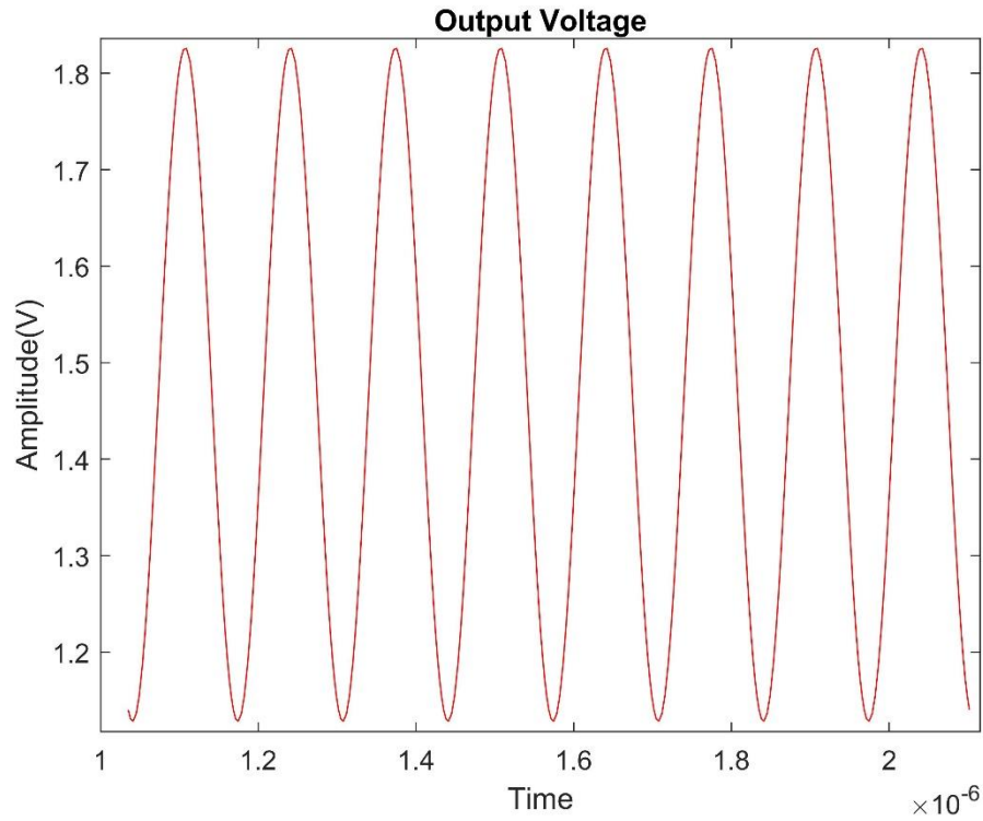
Figure 4.9: TIA output voltage to 3\mu A input current
