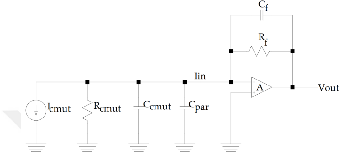
Figure 3.1: Resistive Feedback Transimpedance Amplifier
