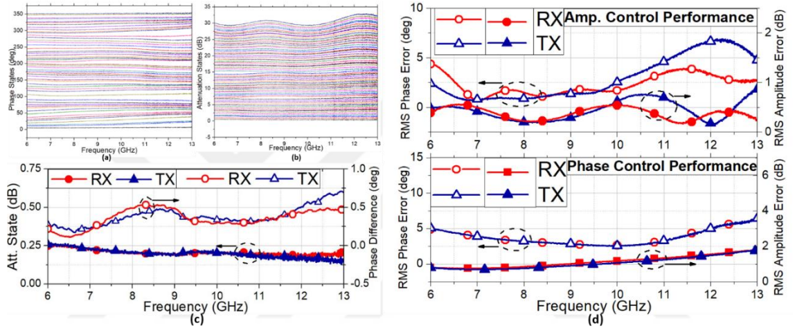
Figure 1. 12 The measured (a) phase states, (b) attenuation states, (c) optional attenuation bit, and (d) RMS phase and amplitude errors of the core-chip.
