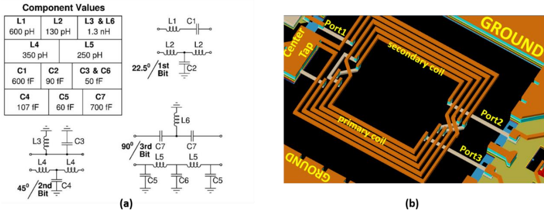
Figure 2. 22 (a) The block diagram of the filter networks with their component values. (b) The top view of the transformer.
