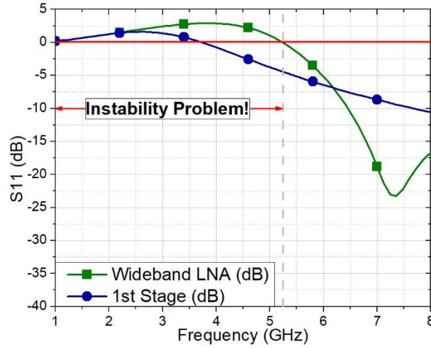
Figure 2. 47 The S11 of the CE stage and wideband LNA at low frequencies.
