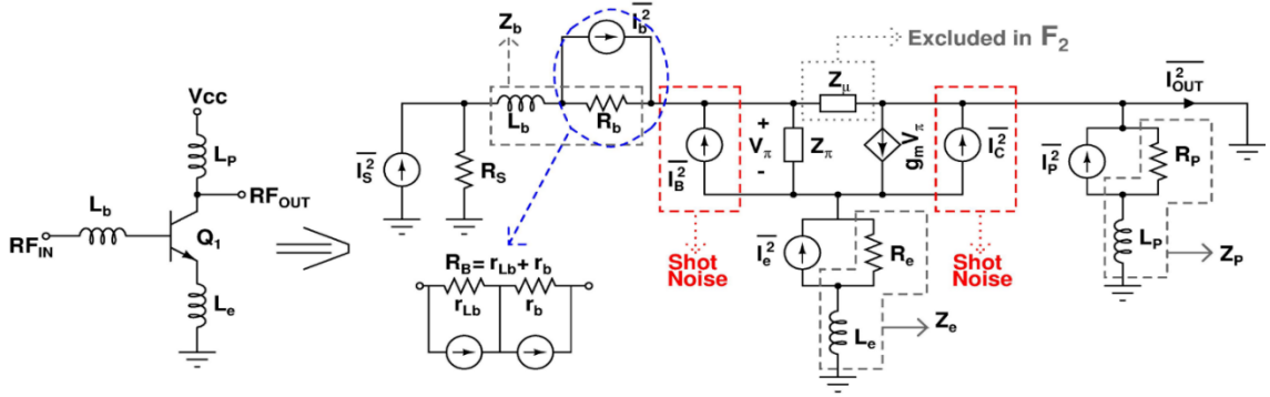
Figure 2. 37 Small signal model of the CE amplifier with noise sources.
