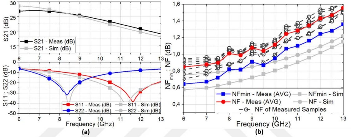
Figure 2. 41 The sub-1dB LNA's (a) S-parameters, (b) NF_{\min} and NF.
