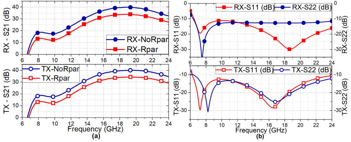
Figure 2.52 The reference mode (a) gain, and (b) return loss for RX and TX.
