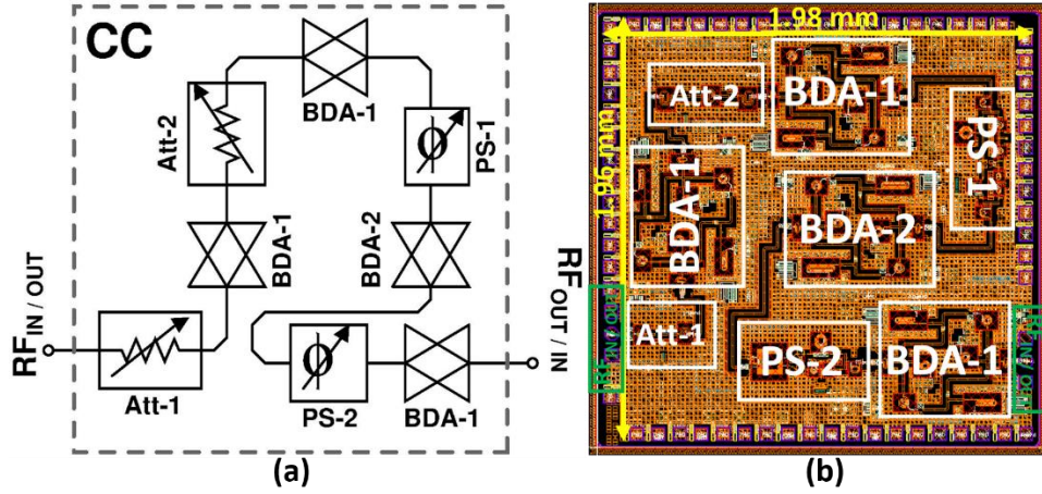
Figure 2. 28 (a) The block diagram of the CC. (b) The view of the CC.
