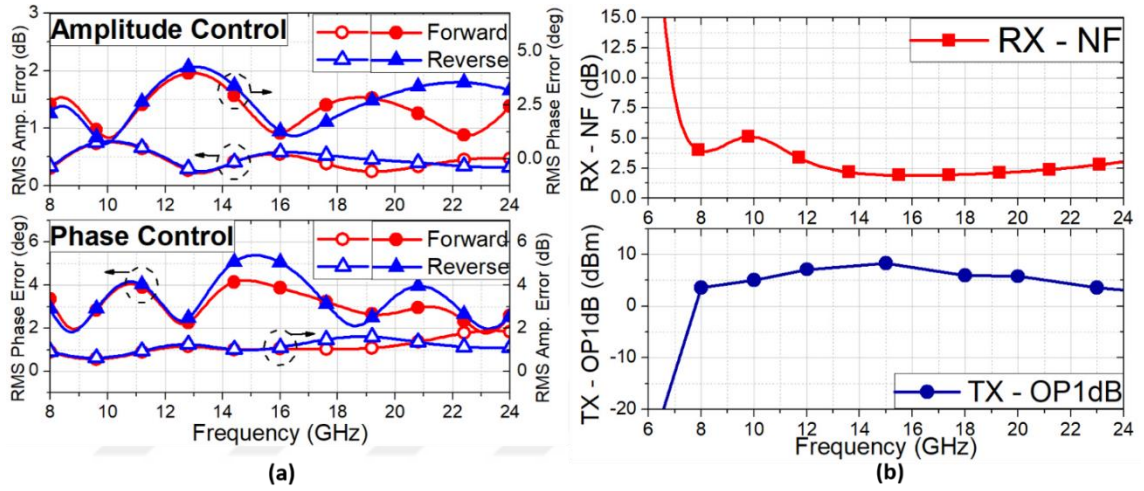
Figure 2.53 (a) The RMS phase and amplitude errors of the core-chip during amplitude and phase control, (b) RX NF and TX OP1dB during reference mode of operation.
