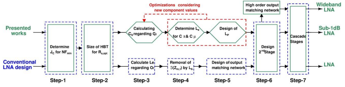
Figure 2. 39 The design flows for the described and conventional methods.
