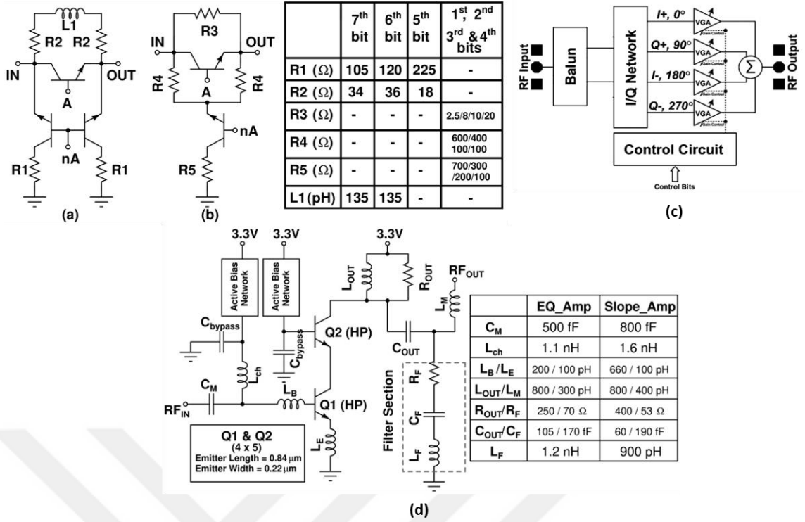
Figure 1. 9 The block diagrams of (a) \pi -type attenuator bit, (b) T-type attenuator bit, (c) PS, (d) the EQ_Amp and Slope_Amp .
