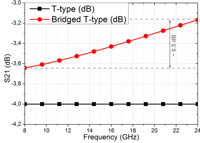
Figure 2. 15 Comparison of an ideal and a bridged T-type 4-dB attenuators.
