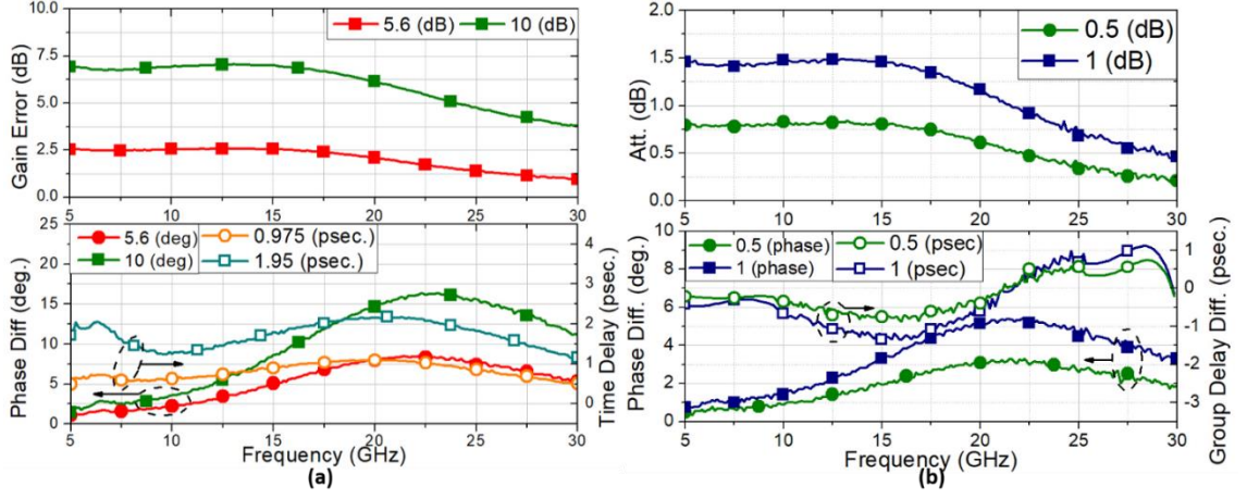
Figure 2. 12 (a) 5.6^\circ and 10^\circ of phase shift, 0.975 psec. and 1.95 psec. of time delays obtained from BDA including their gain error. (b) BDA with 0.5 dB and 1 dB of gain steps, including their phase and group delay difference.
