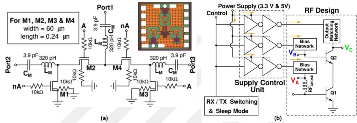
Figure 1. 7 (a) The block diagram of the SPDT switch. (b) The block diagram of the SCU with a basic amplifier.
