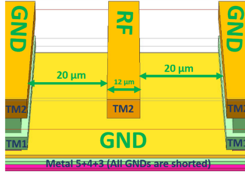
Figure 2. 5 The cross-section of the guided microstrip transmission line.
