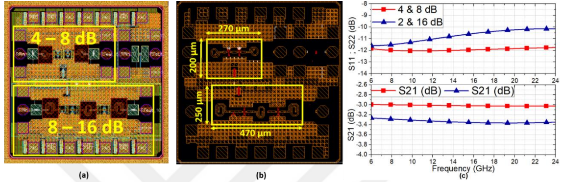
Figure 2. 18 (a) Top view of the attenuator. (b) The dimensions of the sections excluding pads. (c) Impedance terminations and S21 of the sections.
