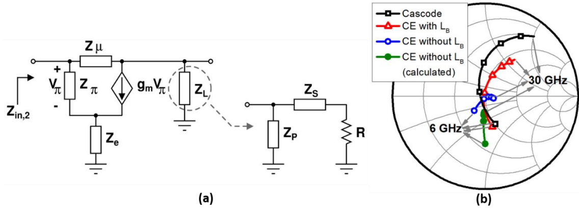
Figure 2. 36 (a) The small signal model of a CE amplifier. (b) The input impedance comparison of the three different amplifier topologies and calculated Z_{in,2} .
