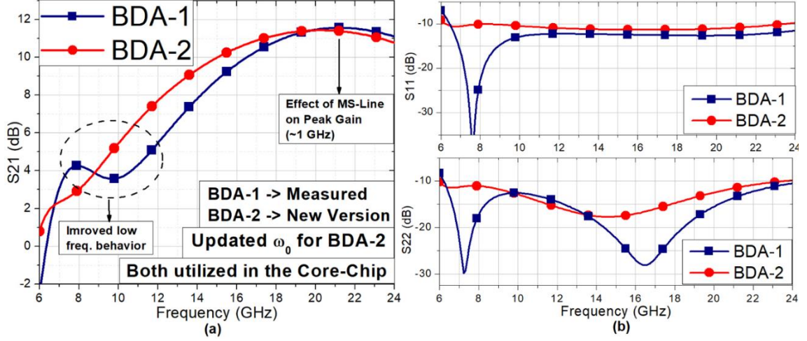
Figure 2. 13 The difference between two BDA version in terms of (a) S21, and (b) impedance matching performance.
