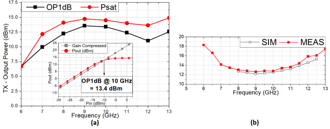
Figure 1. 11 The measured (a) OP1dB of the TX, (b) NF of the RX.
