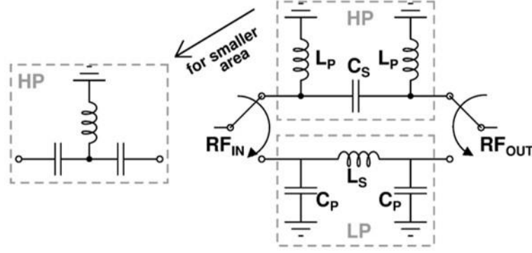
Figure 2. 21 Schematic view of a HP-LP type PS.
