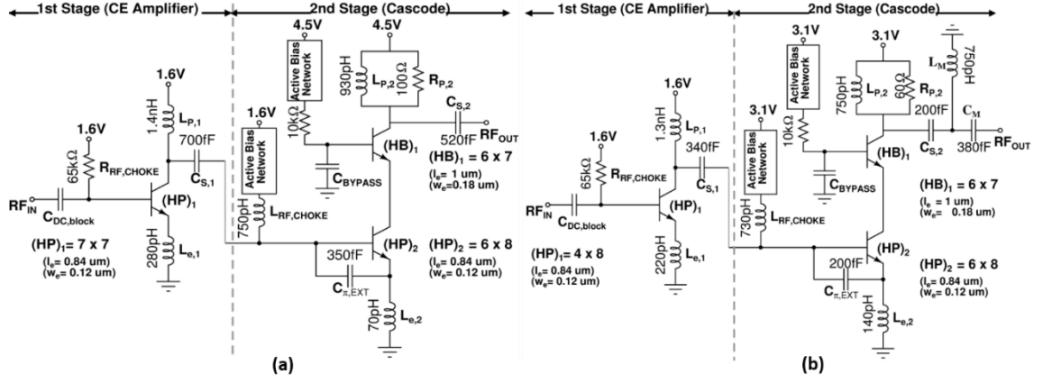
Figure 2. 40 The schematic views of (a) the sub-1dB, and (b) the wideband LNAs.
