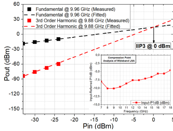
Figure 2. 43 The wideband LNA's measured IIP3 and IP1dB performances.
