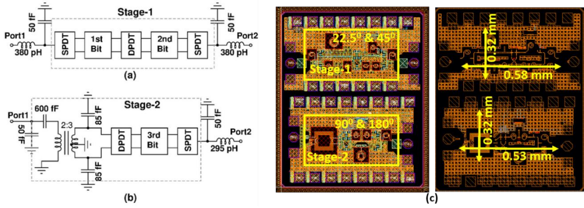
Figure 2. 24 The block diagram of the PS's (a) Stage-1, (b) Stage-2, (c) top-view.
