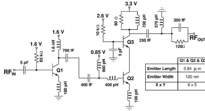
Figure 2. 44 The schematic view of the new wideband two-stage LNA.
