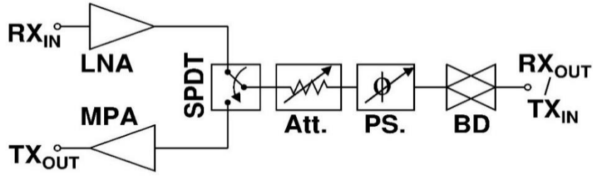
Figure 2. 1 Block diagram of the 8-to-24 GHz SiGe BiCMOS T/R module core-chip.
