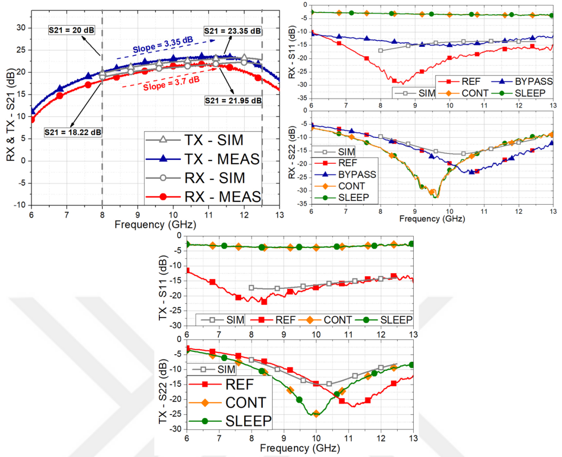
Figure 1. 10 The measured S-parameters of the X-Band core-chip for RX and TX.
