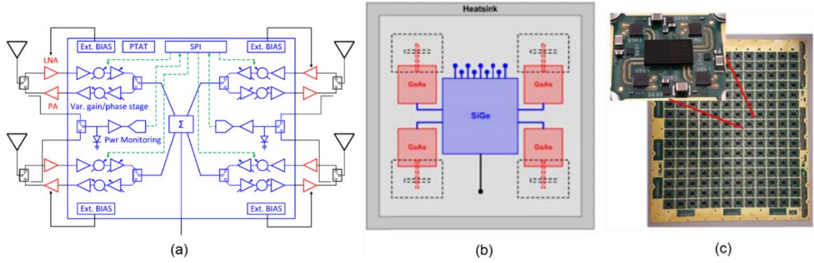
Figure 1. 4 a) Block diagram of core-chip and RF front-end b) SiGe and GaAs chips in the phased array c) X-Band 768-element phased array (Rebeiz et al 2017).
