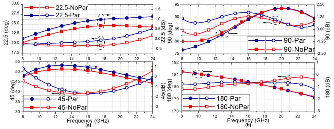
Figure 2. 26 The simulated major phase states and their amplitude errors (a) for Stage-1, and (b) for Stage-2, with (Par) and without (NoPar) the parasitic resistance.
