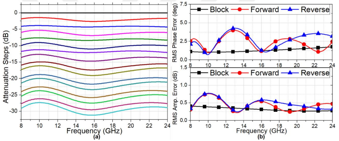
Figure 2. 34 (a) The relative attenuation states of the CC during forward mode. (b) The RMS phase and amplitude errors obtained during amplitude control of the CC for both signal direction, compared with block level performance.
