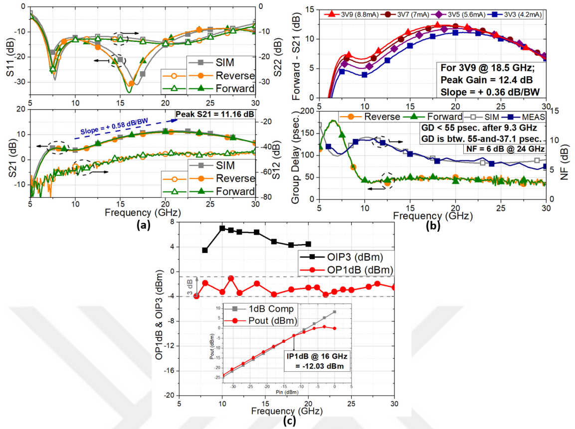
Figure 2. 11 (a) Simulated and measured S-parameters of the BDA. (b) Measured forward-mode gain for various collector currents, GD and NF of the BDA. (c) The OP1dB and OIP3 of the BDA for the defined frequency range.
