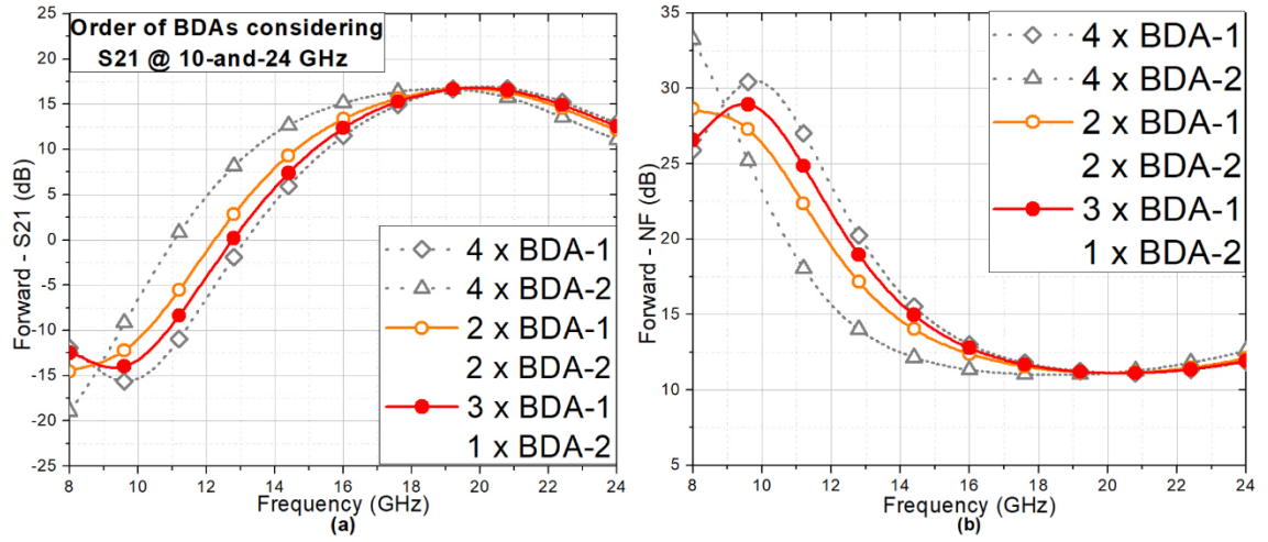
Figure 2. 29 The effect of various BDA-1 and BDA-2 combinations on (a) Forward-Mode S21, and (b) Forward-Mode NF.
