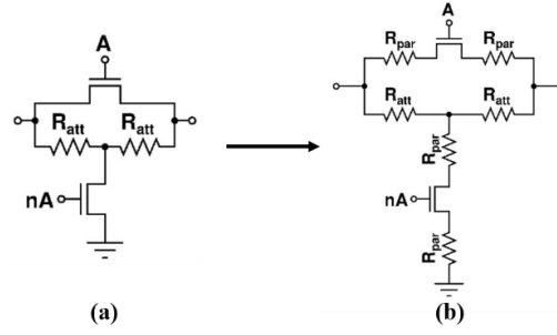
Figure 2. 17 R_{par} is added to the device ports. The schematic in (a) is converted to (b).
