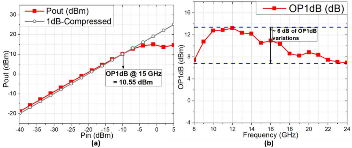
Figure 2. 46 OP1dB of the LNA (a) at 15 GHz, (b) at various frequencies.
