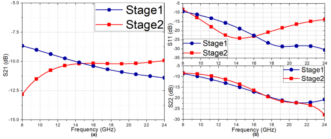
Figure 2. 25 The simulated (a) S21, and (b) S11-S22 of the PS stages.
