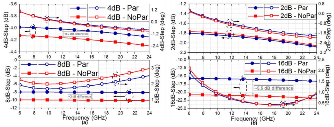
Figure 2. 19 The attenuation and phase differences of each individual bit.
