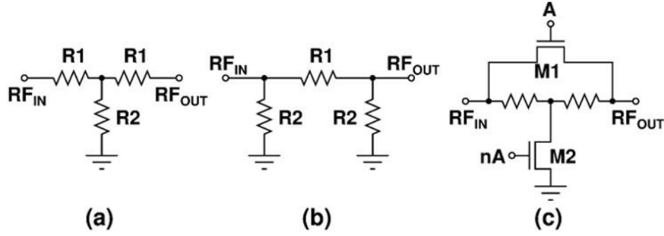
Figure 2. 14 Schematic view of a) T-type, b) \pi -type, c) Bridged T-type attenuators.
