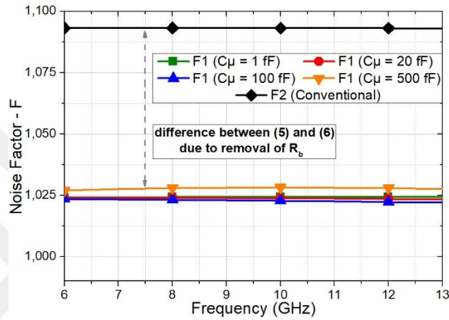
Figure 2. 38 Calculated F_1 and F_2 in (5) and (6) for various Z_\mu values.
