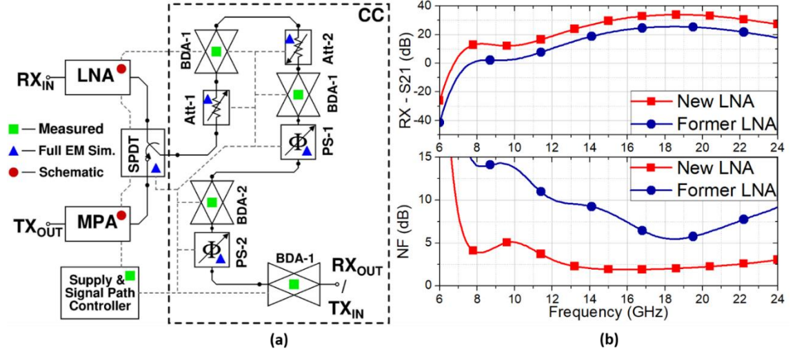
Figure 2.48 (a) The block diagram of the X-to-K Band T/R module core chip. (b) RX gain and NF with Former and New LNA.
