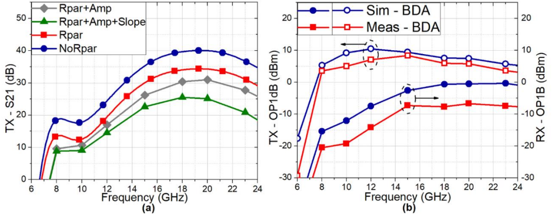
Figure 2. 51 (a) TX gain for different added parasitic scenarios. (b) TX and RX OP1B performance for the simulated and measured BDA.
