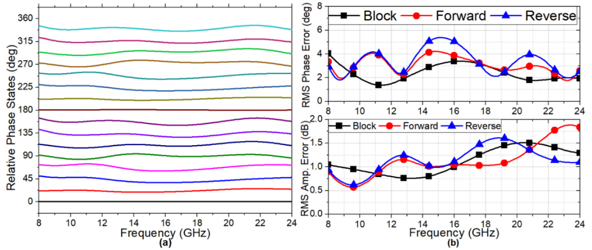
Figure 2. 33 (a) The relative phase states of the CC during forward mode. (b) The RMS phase and amplitude errors obtained during phase control of the CC for both signal direction, compared with block level performance.
