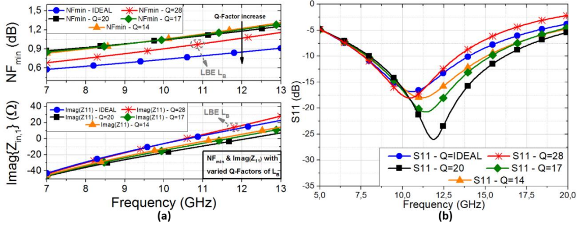
Figure 2. 35 The effect of the L_b on (a) NF_{min} and \text{Imag} \{Z_{in,1}\} , (b) S_{11} of a conventional amplifier, (with various Q-factors).
