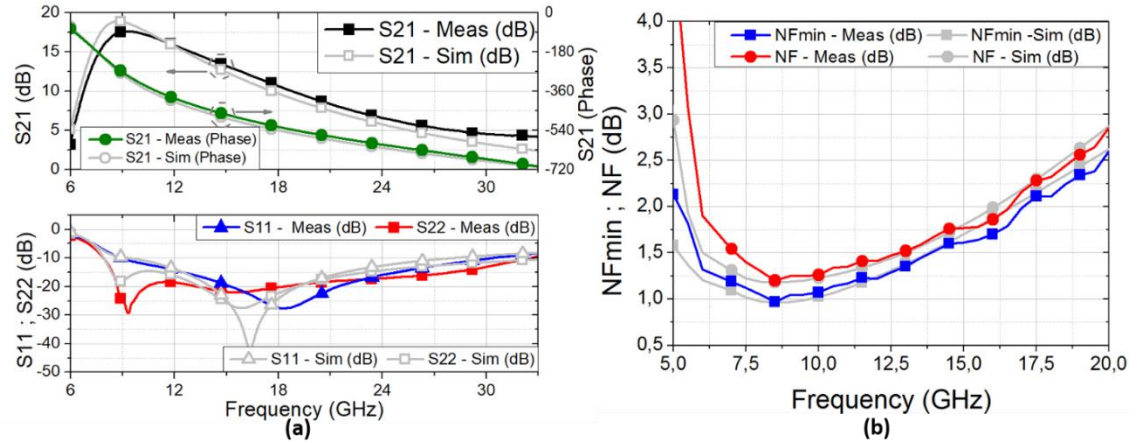
Figure 2. 42 The wideband LNA's (a) S-parameters, (b) NF_{\min} and NF.
