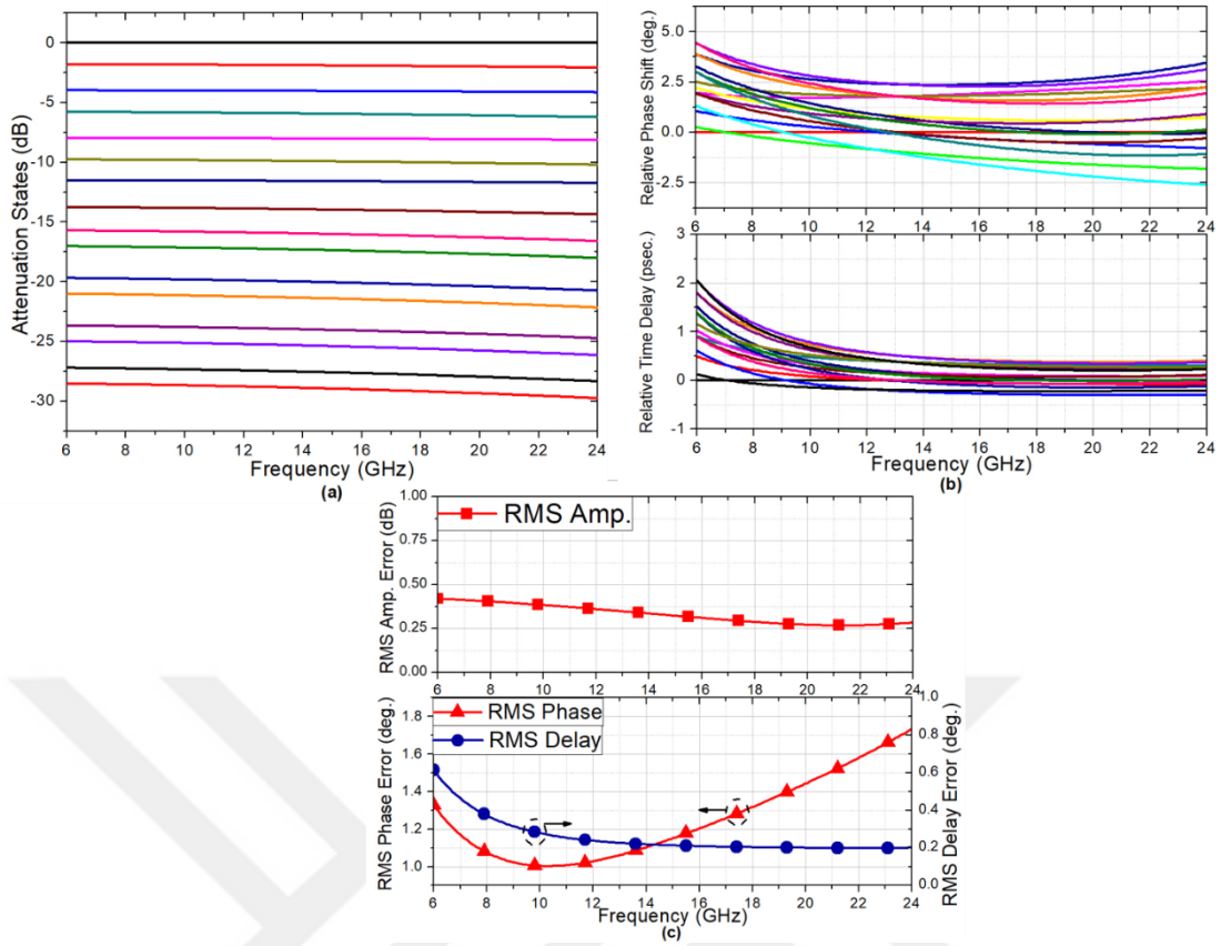
Figure 2. 20 The 16 a) attenuation states, b) relative phase and time delay states, and c) calculated RMS amplitude, phase and delay errors of the 4-bit attenuator.
