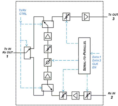
Figure 1. 5 Common-path based core-chip example with separated attenuator range (Bentini et al 2014).
