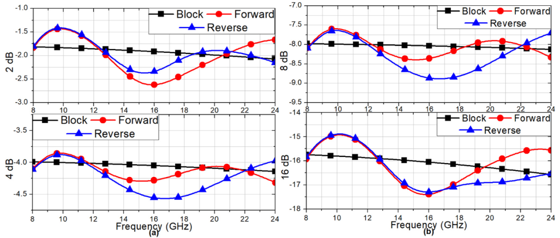
Figure 2.31 Comparing the block level and the CC forward-reverse mode performances of (a) 2-and-4 dB, (b) 8-and-16 dB attenuations.
