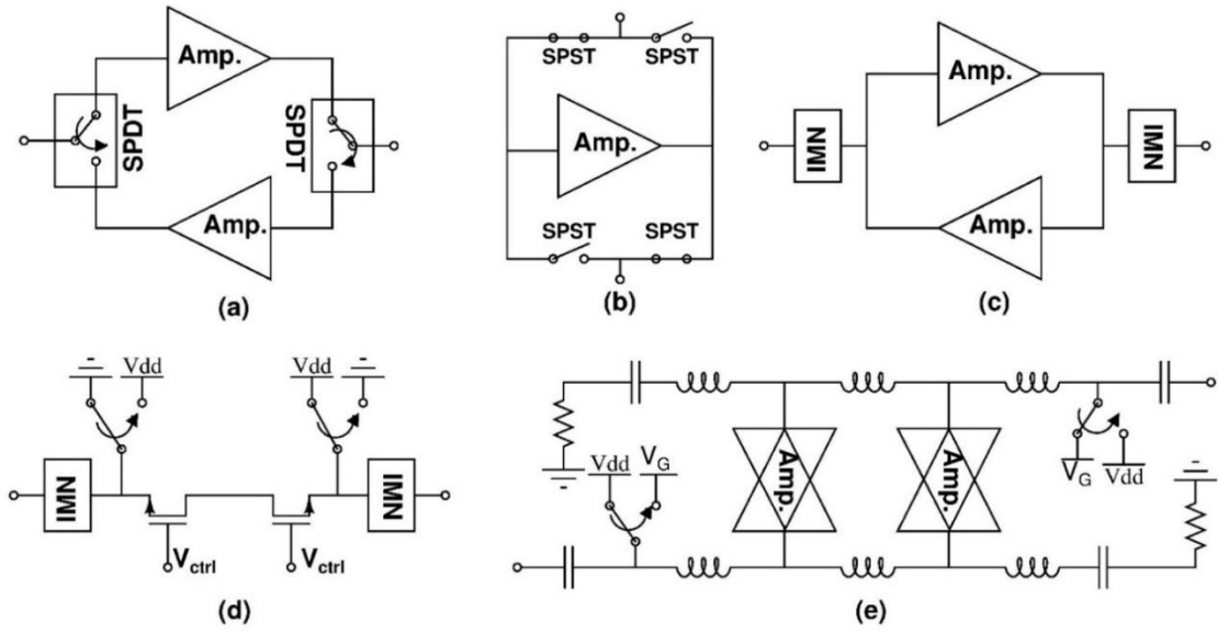
Figure 2. 8 Various methods for bidirectionality in an amplifier; (a) switching between two amplifiers, (b) single amplifier with four switches, (c) Common IMN topology, (d) Common IMN with a single amplifier, (e) the distributed BDA.
