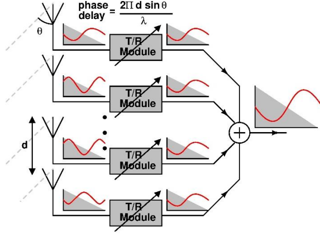
Figure 1. 1 A phased array example with several elements.
