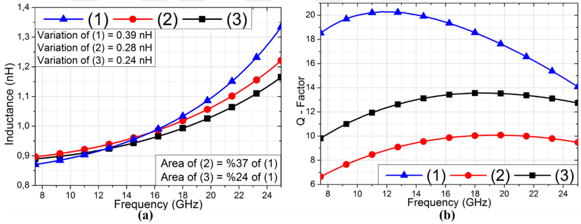
Figure 2. 4 Comparison of different inductor designs; a) Inductance variation and total box size variation b) Q-factor comparison of three inductors.
