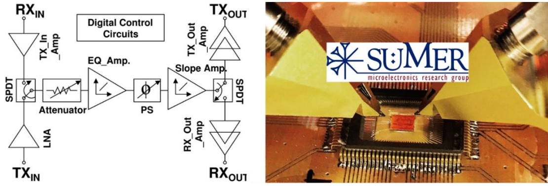
Figure 1. 6 The block diagram and the top-view of the measured positively sloped X-Band 6-bit core-chip.
