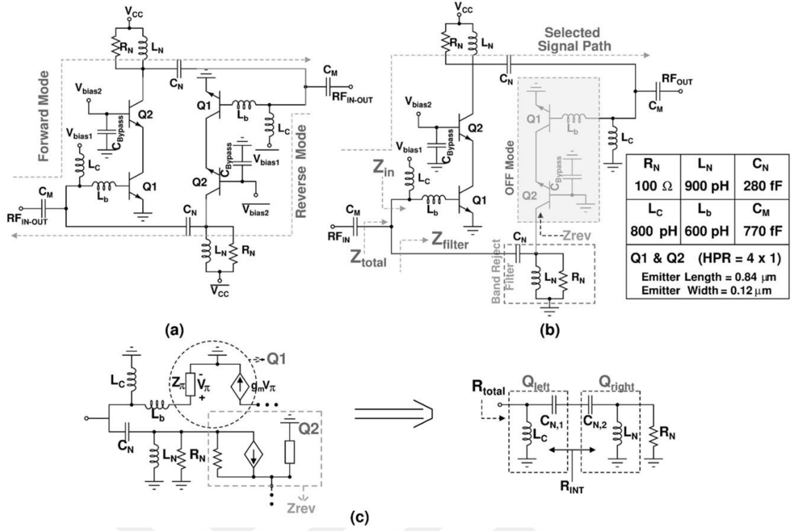
Figure 2. 9 a) Schematic of the BDA. b) Signal flow of the BDA during forward-mode. c) The small-signal model of Q1.
