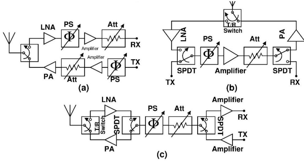
Figure 1. 2 Various T/R module architectures; (a) the separated architecture, (b) the combined path, (c) the bidirectional common-chain.
