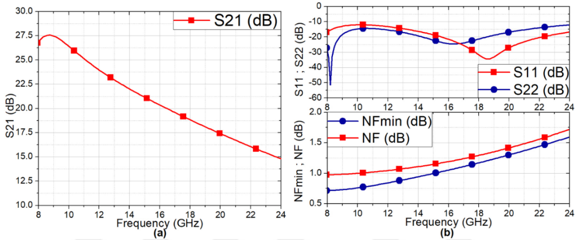
Figure 2. 45 a) The S21, (b) Input-output matching and NF of the LNA.
