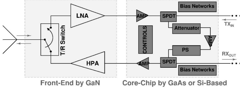
Figure 1. 3 Block diagram of a T/R module with multiple technologies.
