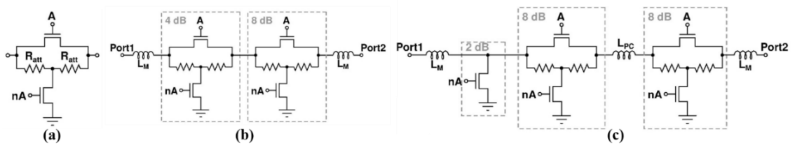
Figure 2. 16 The schematic views of the a) single T-type attenuator, b) 4-and-8 dB attenuation section, c) 2-and-16 dB attenuation section.
