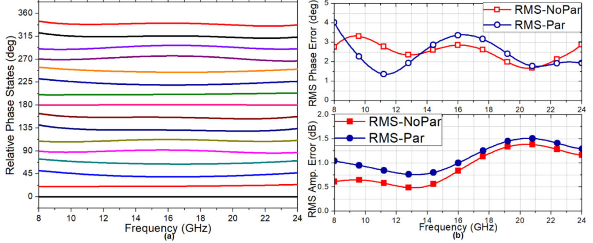
Figure 2. 27 The simulated (a) 16 phase states, and (b) Calculated RMS phase and amplitude errors of the PS.
