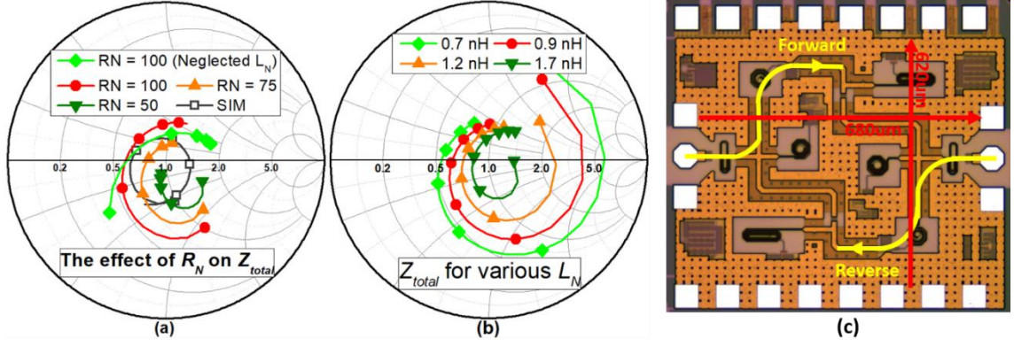
Figure 2. 10 The effects of (a) R_N , (b) L_N on Z_{total} . (c) Top-view of the BDA.
