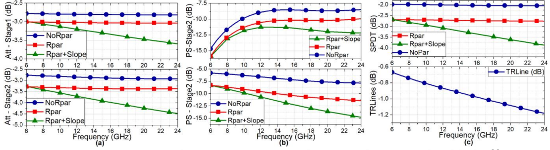
Figure 2. 49 (a) Attenuator, (b) PS, (c) SPDT and TRLine losses with added effects.
