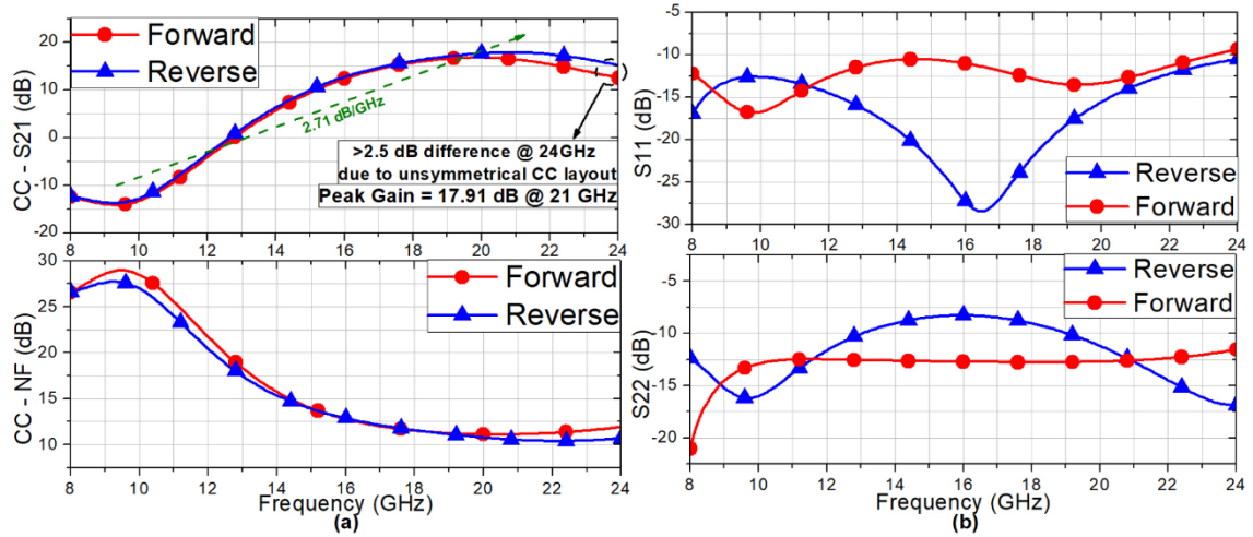
Figure 2. 30 (a) The forward-and-reverse mode S21 and NF performances of the CC. (b) The impedance matching performances of the CC for both signal directions.
