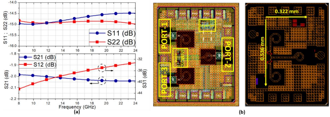
Figure 2. 7 (a) The post-layout S-parameters, (b) The top view of the SPDT switch.
