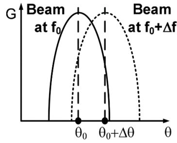
Figure 2. 2 An antenna pattern representation including the effect of beam squint (Garakoui et al 2011).
