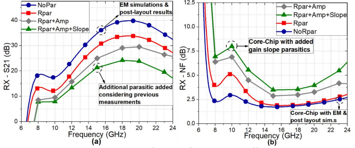
Figure 2. 50 RX (a) gain, and (b) NF for the defined parasitic effect scenarios.
