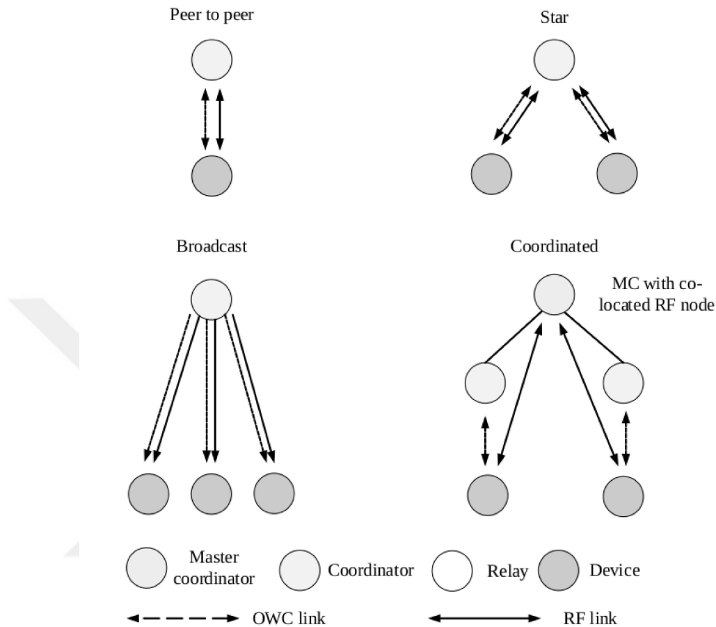
Figure 5: 802.15.13 Supported Topologies.
