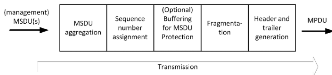
Figure 10: The MAC Transmit Process.
