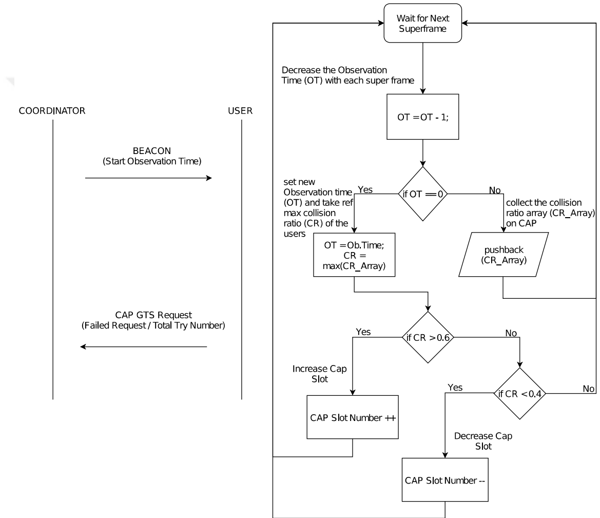
Figure 28: Proposed Algorithm.
