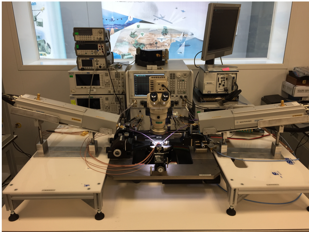
Figure 4.5: 94 GHz setup
