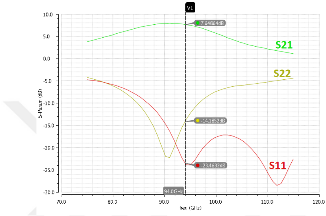
Figure 4.7: Simulation results of core PI-VGA
