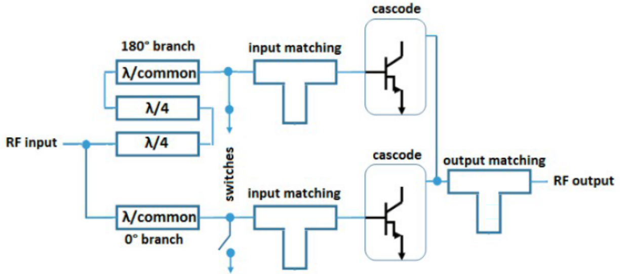
Figure 3.16: Block diagram of phase inverter-variable gain amplifier
