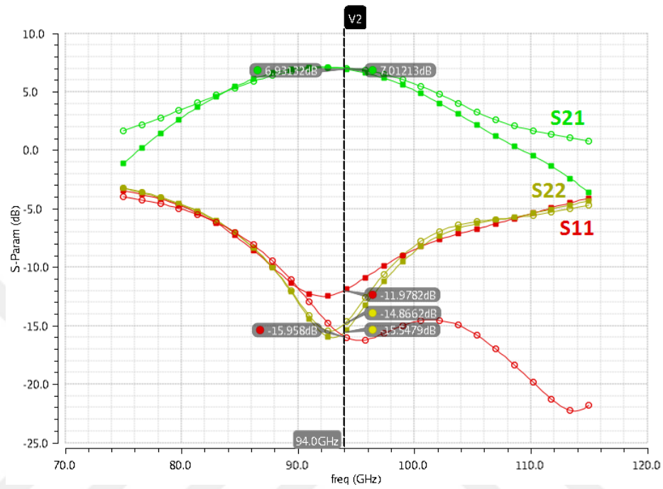
Figure 3.23: Fast corner, min. gain setting, s-parameters
