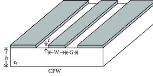
Figure 2.2: A CPW line
