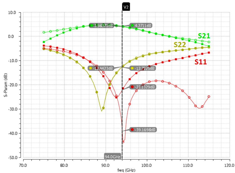
Figure 3.22: Slow corner, max. gain setting, s-parameters
