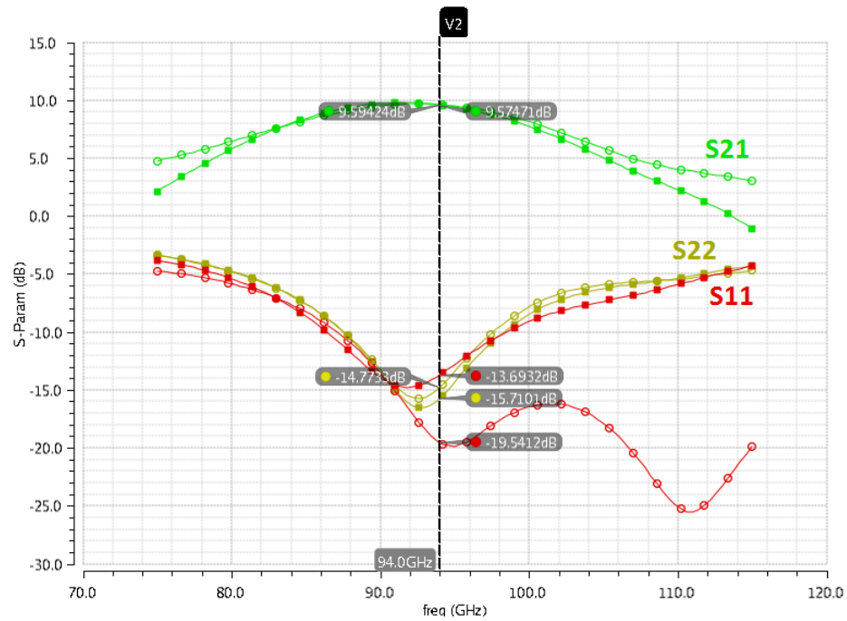
Figure 3.24: Fast corner, max. gain setting, s-parameters
