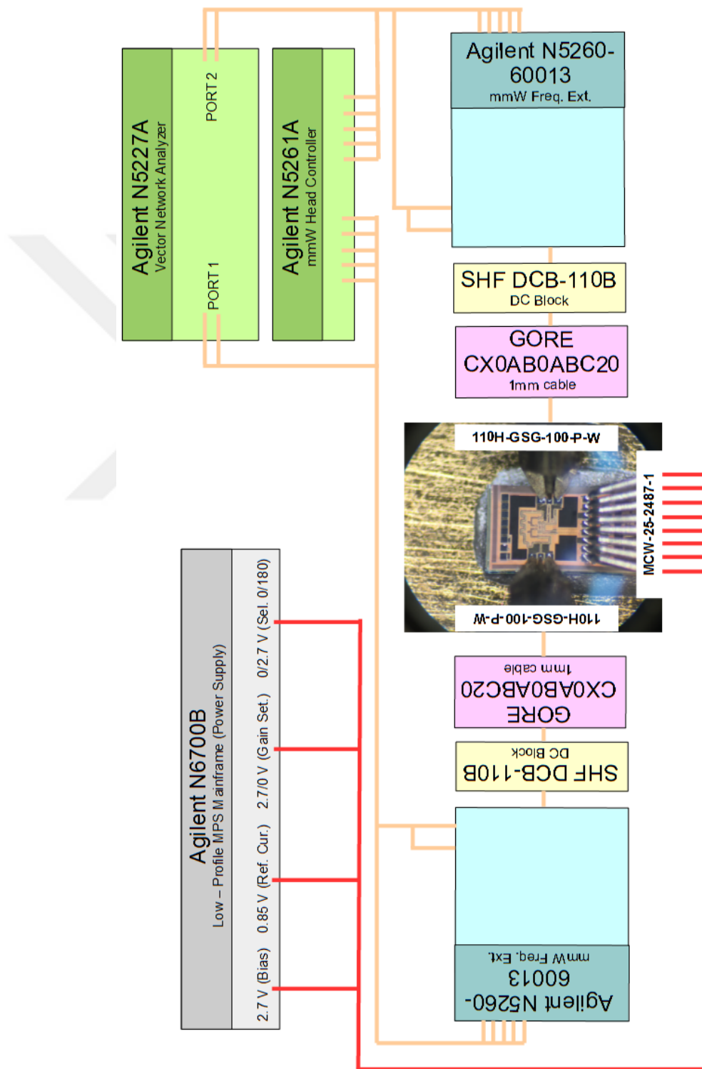
Figure 4.1: Block diagram of measurement setup
