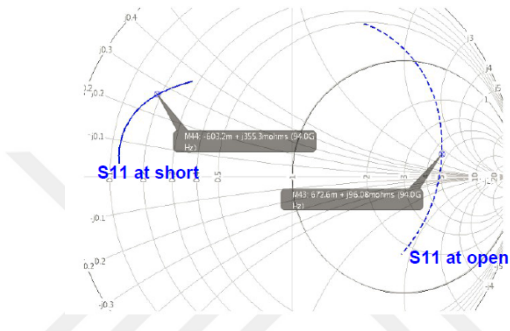
Figure 3.6: Short and improved open characteristics of 0^\circ branch
