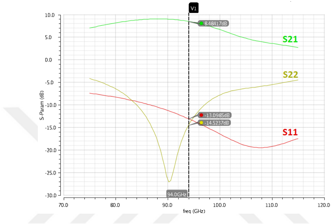
Figure 3.9: s_{11} , s_{21} and s_{22} plots of cascode gain amplifier at rectangular plot in dB
