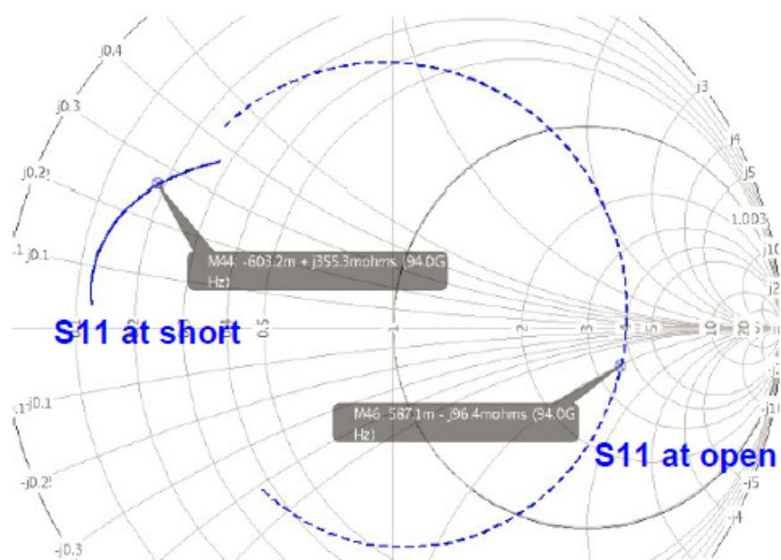
Figure 3.7: Short and improved open characteristics of 180^\circ branch
