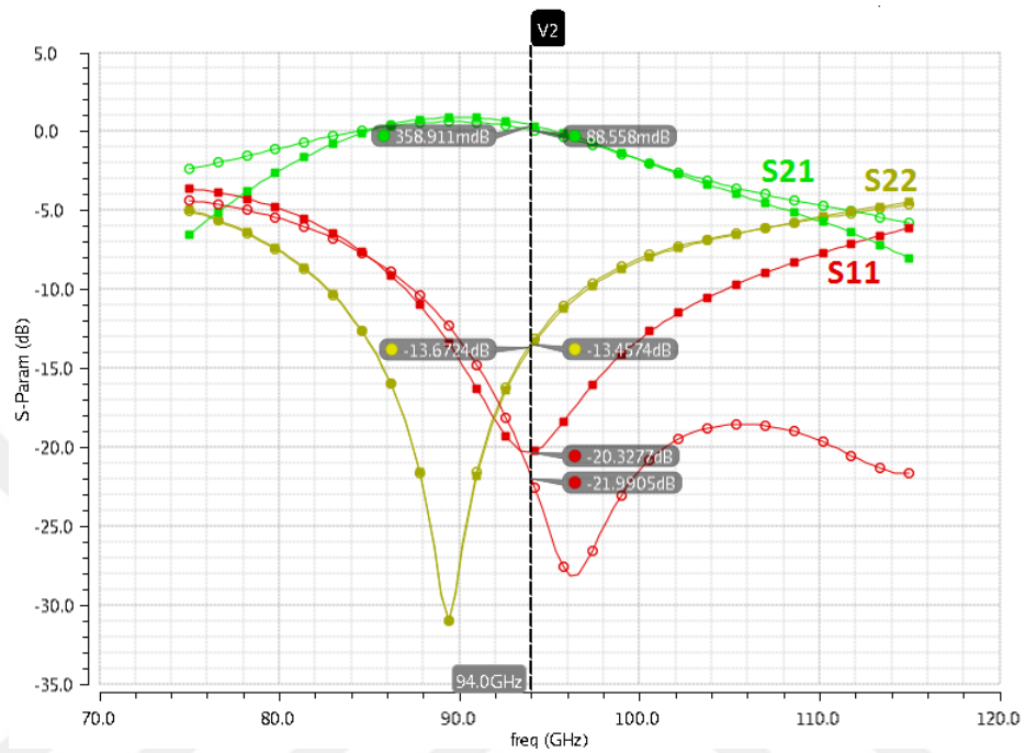
Figure 3.21: Slow corner, min. gain setting, s-parameters
