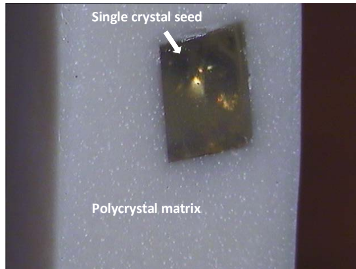
Figure 9.11. Stereo microscope image of single crystal seed material embedded in polycrystalline matrix
