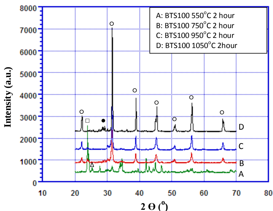
Figure 7.10. XRD pattern of BTS100 coded powders, calcined at 550-750-950-1050°C for 2 hours, with the ratio of Ti/Ba=1 (○BaTiO 3 ●Ba 2 TiO 4 ▲Rutile TiO 2 △Anatase TiO 2 □BaCO 3 )
