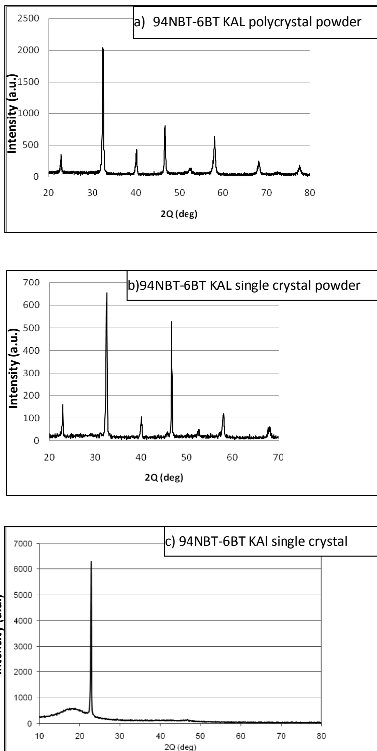
Figure 8.11. XRD pattern for polycrystal powder (a) single crystal powder from a single crystal structure (b) and the bulk single crystal (c) with a composition of 94NBT-6BT KAL
