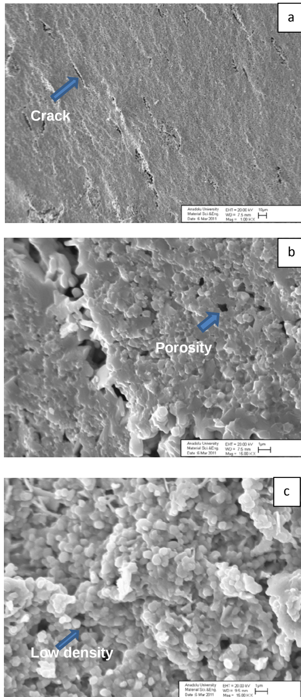
Figure 9.8. The microstructure images of the NBT based sample after SPS sintering under 30MPa; (a) 1000X, (b) 15000X, (c) 15000X
