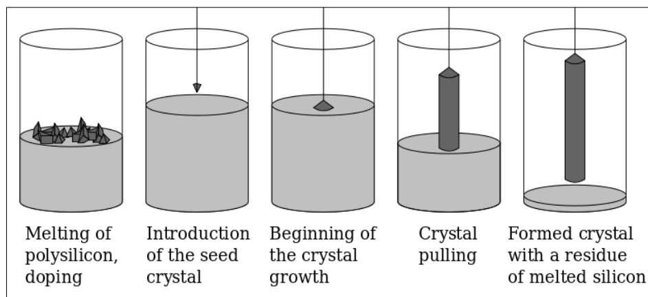
Figure 4.6. Single crystal production stages in Czochralski method
