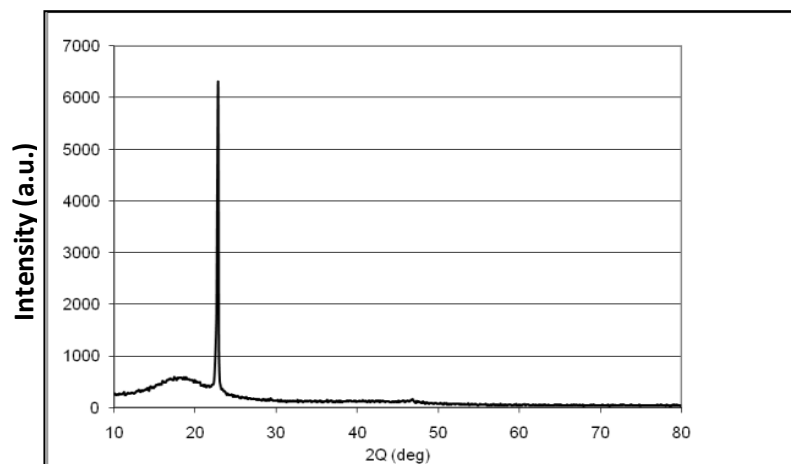
Figure 8.14. XRD pattern of oriented 94NBFT-6BT based single crystal
