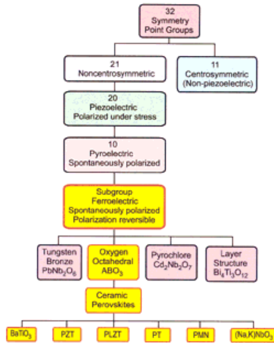
Figure 2.5. The symmetry point groups and electrical properties of sub-groups depending on symmetry [11]
