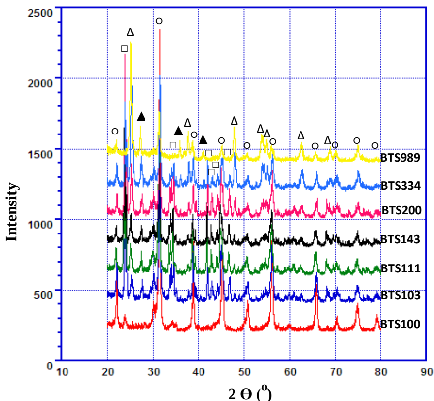
Figure 7.9. XRD pattern of BTS coded powders, calcined at 750^\circ\text{C} for 2 hours, with the ratio of different Ti/Ba ( \circ \text{BaTiO}_3 \blacktriangle Rutile \text{TiO}_2 \triangle Anatase \text{TiO}_2 \square \text{BaCO}_3 )
