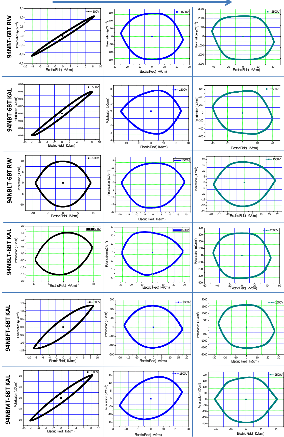
Figure 10.8. The electric field dependent hysteresis loop for 94NBT-6BT-based single crystals
