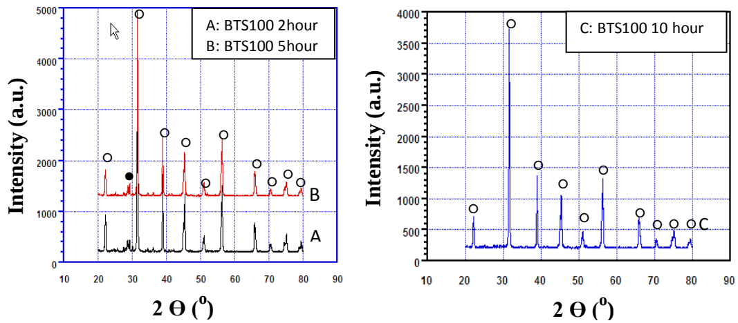
Figure 7.11. XRD pattern of BTS100 coded powders, calcined at 1050°C for 2-5-10 hours, with the ratio of Ti/Ba=1 (○BaTiO 3 ●Ba 2 TiO 4 )
