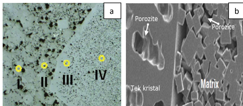
Figure 9.2. Grown NBT-BT (a) and KNN (b) single crystals with SSCG method [77,98]
