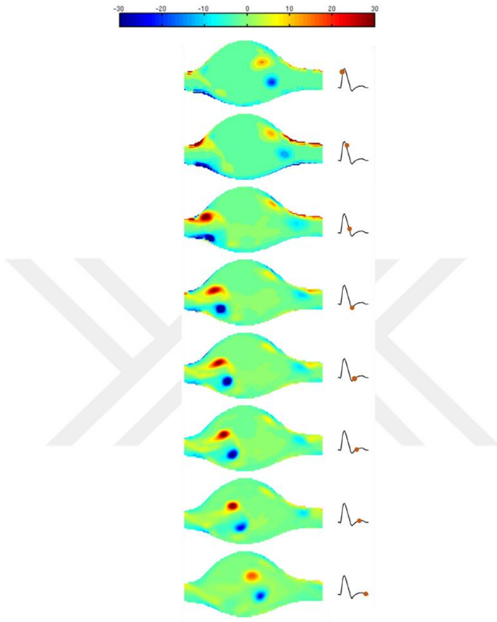
Figure 2.13: Temporal evolution of vorticity for different phases of a physiological flow pattern [33]
