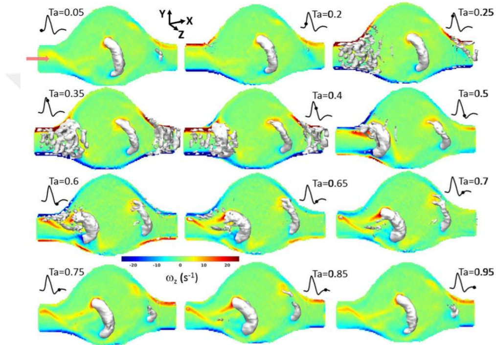
Figure 2.14: Temporal evolution of vorticity and swirling strength for different phases of a physiological flow pattern [34]
