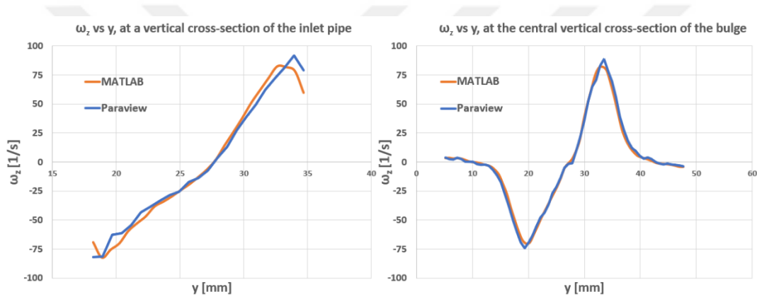
Figure 4.6: Comparison of vorticity in the out of plane direction for the used code and Paraview; at a vertical cross-section of the entrance pipe at left, and at the central vertical cross-section of the bulge at right
