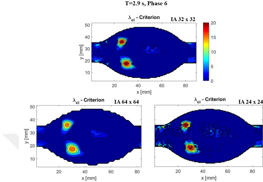
Figure 4.23: \lambda_{ci} contours of different interrogation area sizes applied at the sixth phase of T=2.9 s, 32 x32 at top, 64 x 64 at left-down and 24 x 24 at right-down
