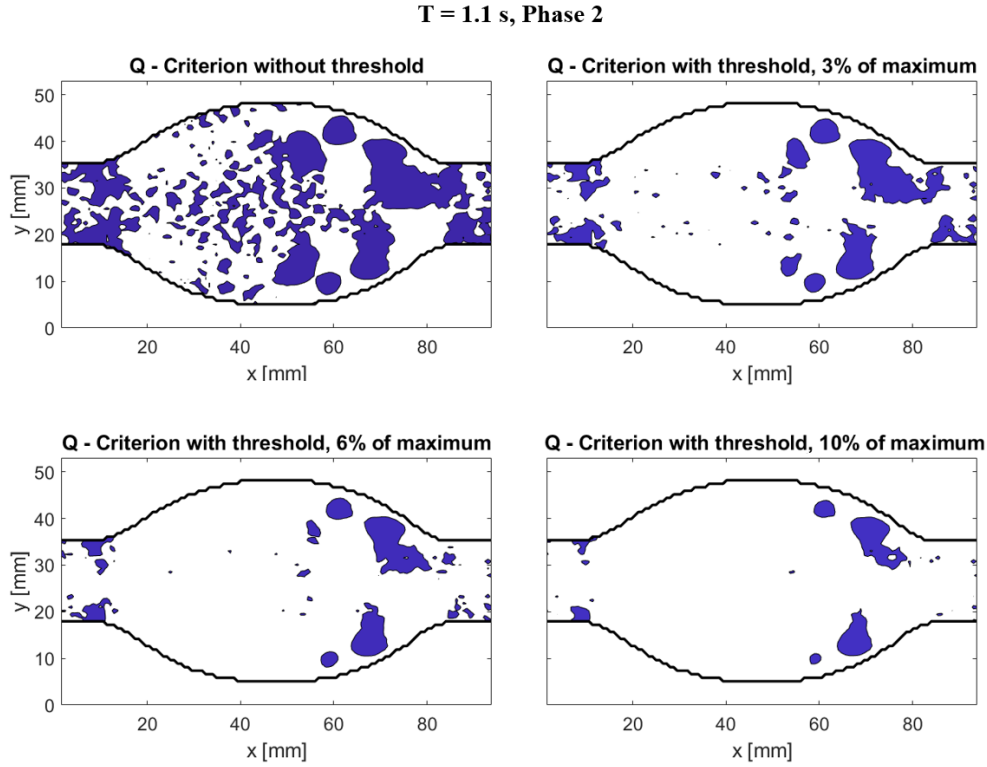
Figure 4.28: Vortex locations identified by different thresholds of Q-criterion at the second phase of T=1.1 s
