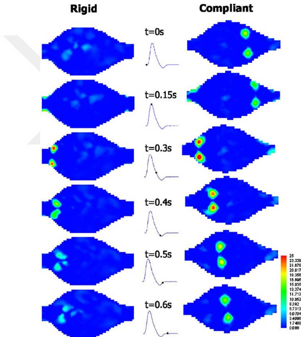
Figure 2.16: Swirling strength distribution for rigid and compliant models in a typical physiological flow pattern [32]
