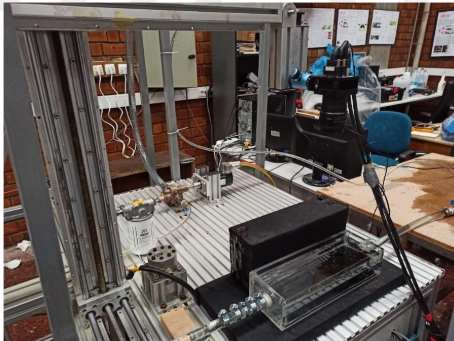
Figure 3.4: Picture of the pump, filter, and the aneurysm model
