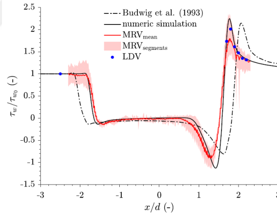
Figure 2.17: Experimental and numerical normalized WSS results with Budwig et al. (1993) comparison [67]
