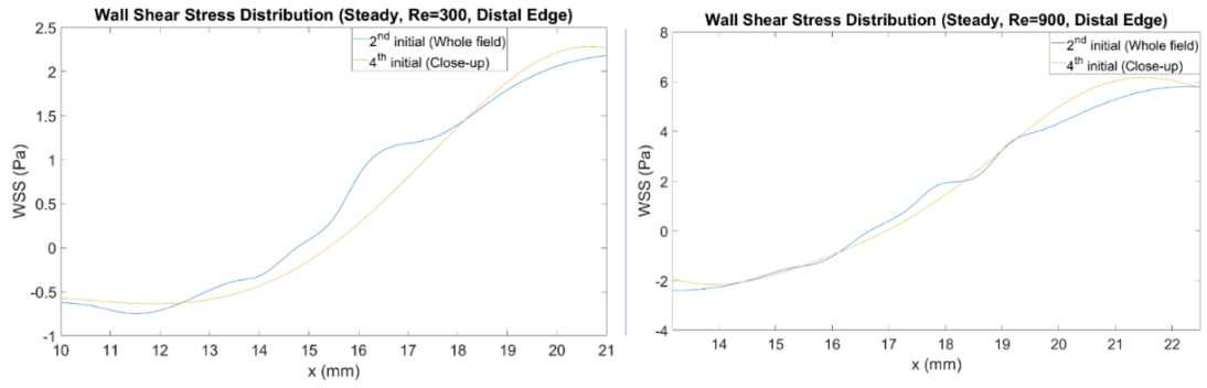
Figure 4.8: WSS distributions for close-up (4 th initial) and whole field (2 nd initial) at the distal edge (Re=300, Re=900)
