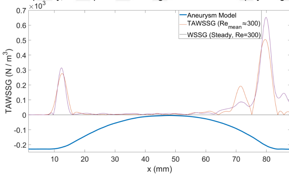
WSSG (Steady, Re=300) and Time Average WSSG Distribution (Physiological)
