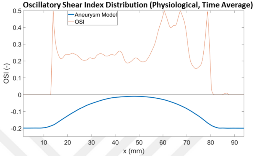
Figure 4.21: OSI distribution of the physiological pattern
