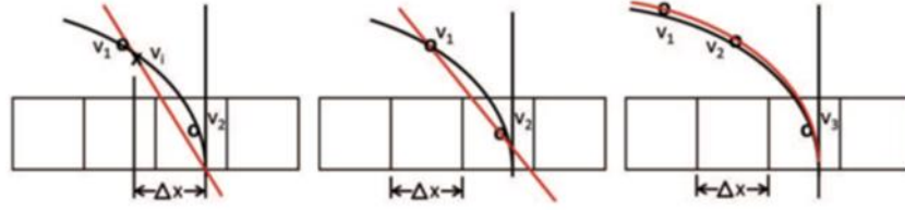
Figure 2.12: Overview schematics of the WSS estimation profiles (Left to right: Vel-Wall method, Vel-LE method, Vel-Parabolic) [52]
