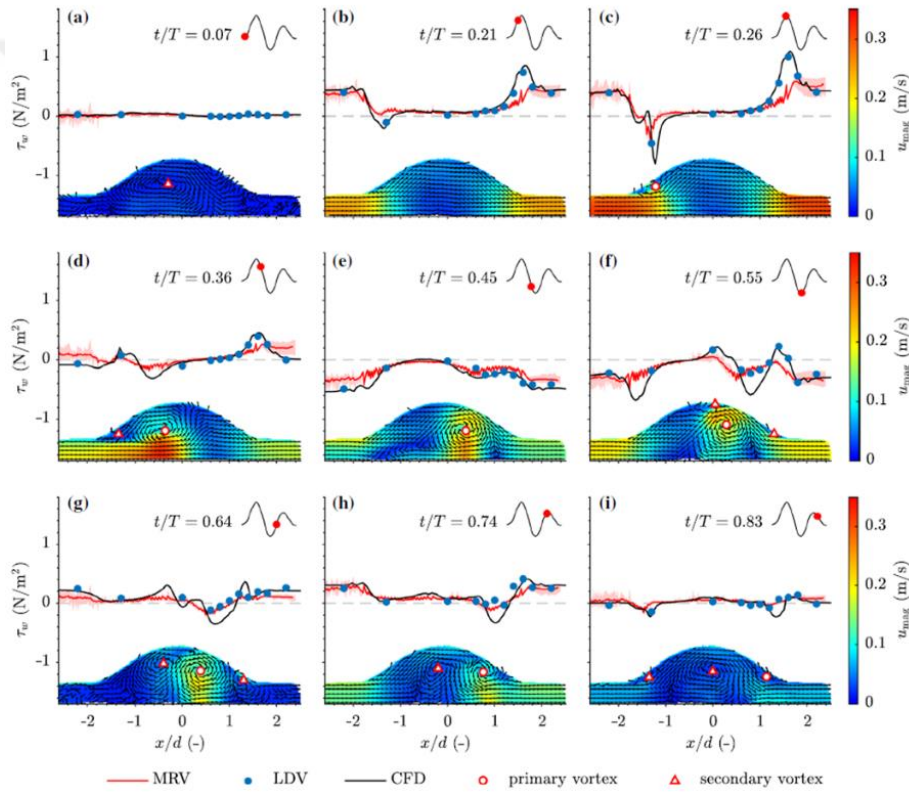
Figure 2.18: WSS variation for different time points with MRV, LDV, and CFD results [75]
