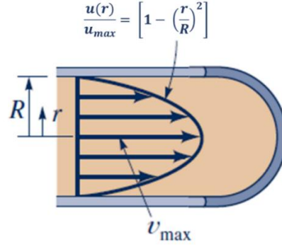
Figure 4.2: Schematic of Hagen-Poiseuille flow [78]
