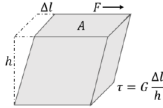
Figure 2.10: Shear stress applied to an elastic material [31]
