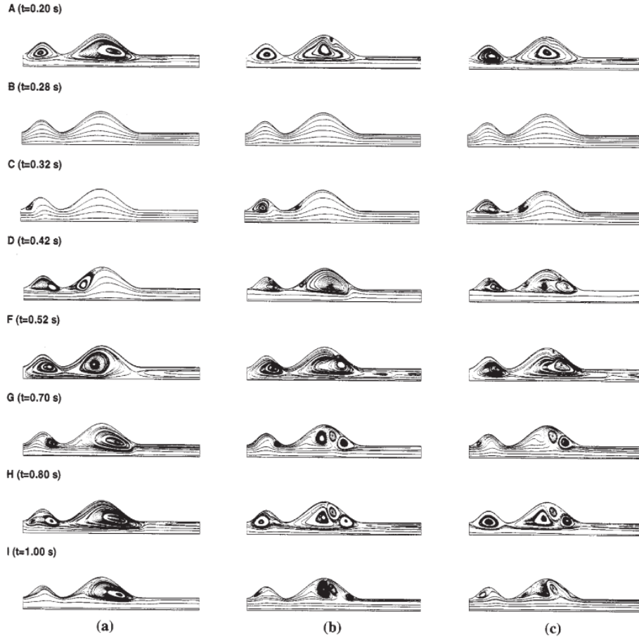
Figure 2.15: Pulsatile flow streamlines (a: Re_{mean} = 100 , b: Re_{mean} = 200 , c: Re_{mean} = 300 ) [66]
