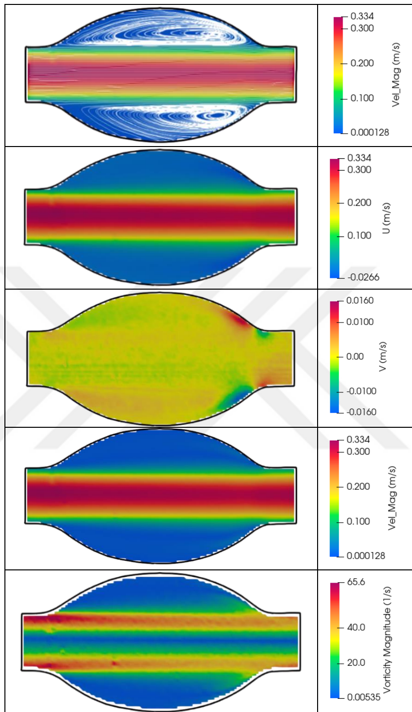
Figure 4.5: Streamline and contours of “u,” “v,” “vel_mag,” and “vorticity magnitude” for Re=300 , Steady case
