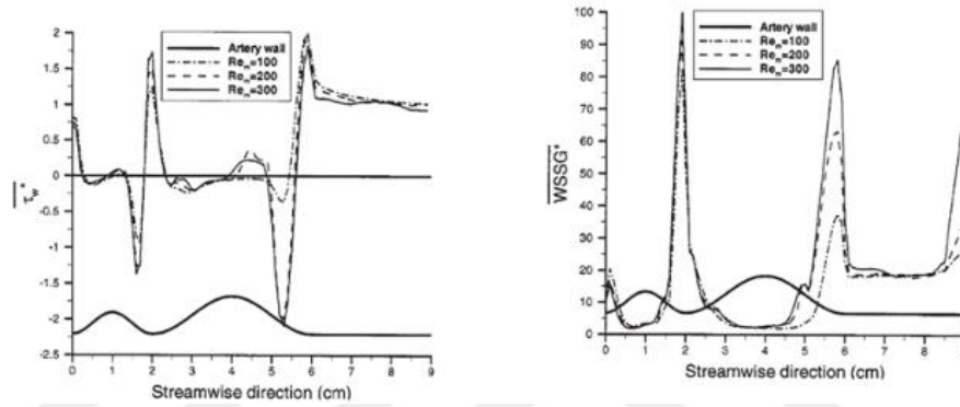
Figure 2.16: Time average WSS and time average WSSG distribution for physiological, selected mean Reynolds numbers [66]
