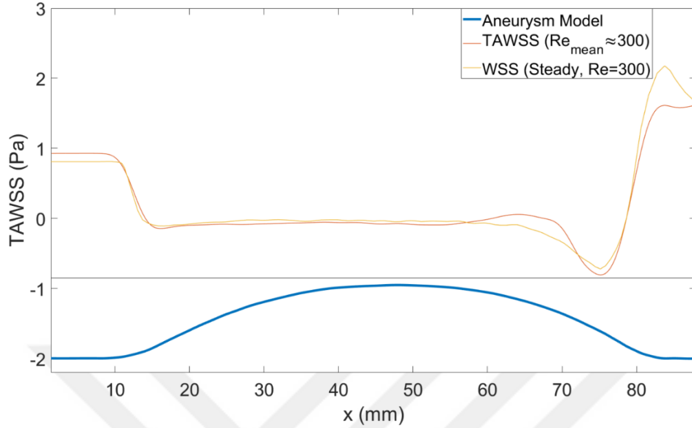
WSS (Steady, Re=300) and Time Average WSS Distribution (Physiological)
