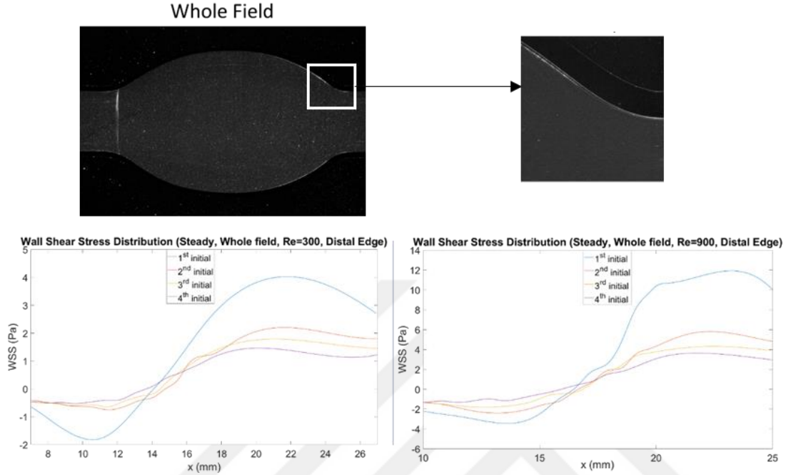
Figure 4.7: WSS distributions for the whole field at the distal edge ( Re=300 , Re=900 , Different initial data points)
