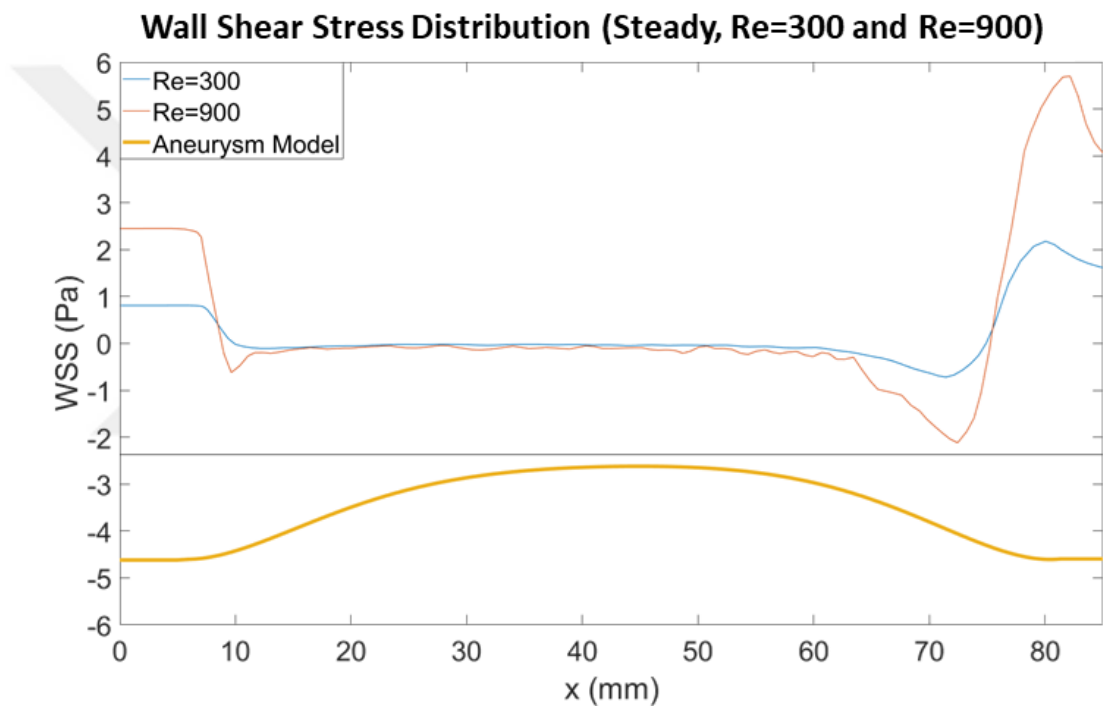
Figure 4.11: WSS distribution for Re=300 and Re=900 under the steady flow
