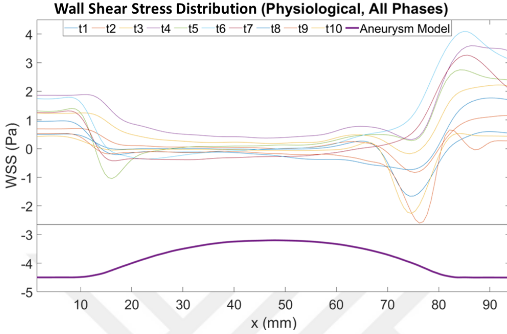
Figure 4.17: WSS distribution for all phases of the physiological pattern
