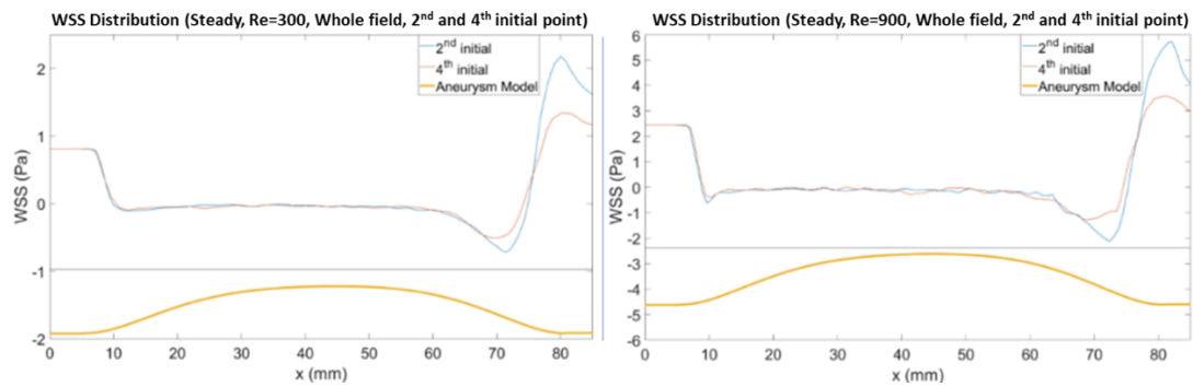
Figure 4.10: WSS distributions for the whole field with 2 nd and 4 th initial data points (Re=300, Re 900)
