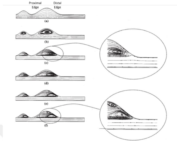
Figure 2.13: Laminar steady flow streamlines (a: Re=10, b: Re=100, c: Re=500, d: Re=1000, e: Re=1750, f: Re=2265) [65]
