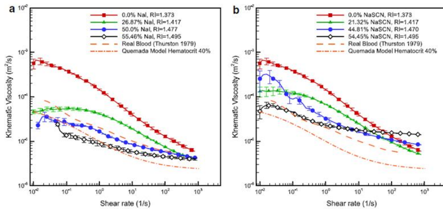
Figure 2.9: Xanthan Gum–Glycerin–Distilled Water - (NaI and NaSCN) mixture's steady shear viscosity properties for different refractive index adjustments (a: NaI, b: NaSCN) [40]
