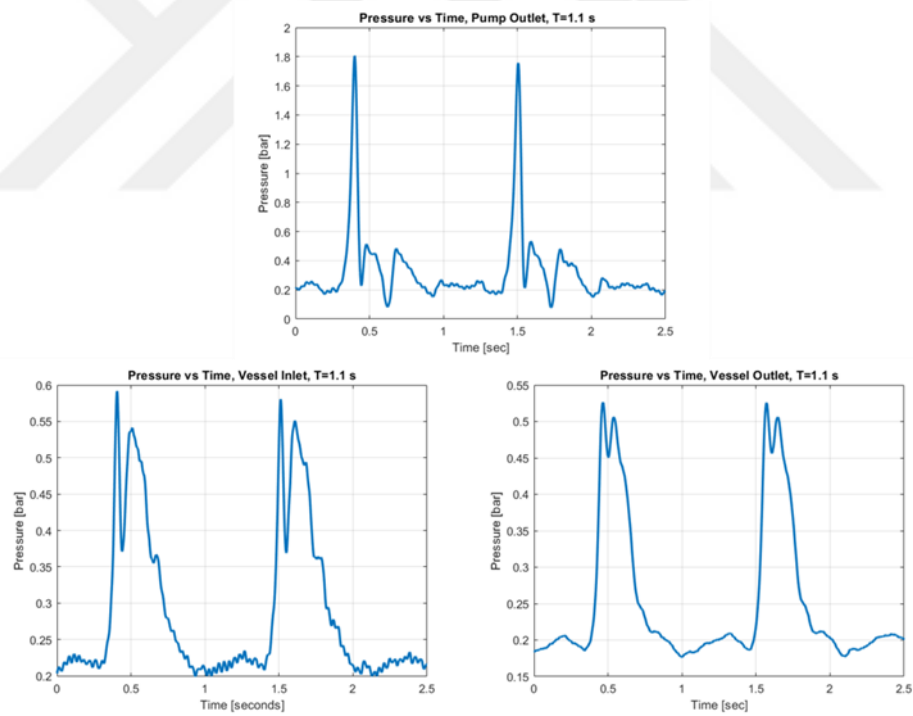
Figure 4.14: Pressure vs. time graph (Up: PT1, Left: PT2, Right: PT3)
