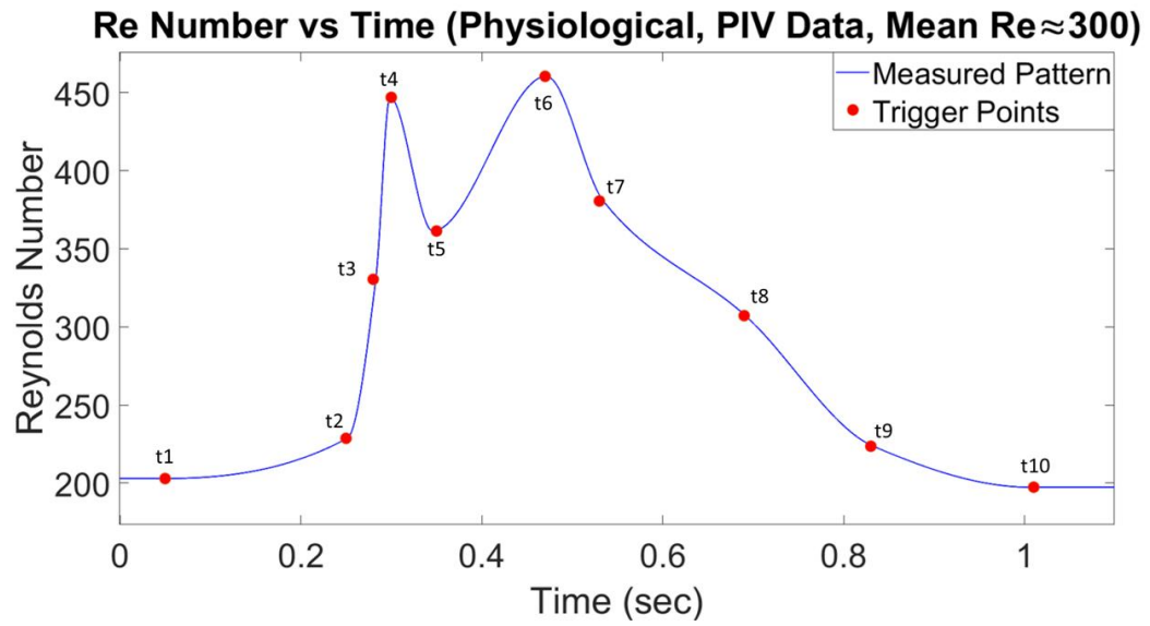
Figure 4.13: Physiological pattern obtained from PIV measurements ( Re_{\text{mean}} \approx 300 )
