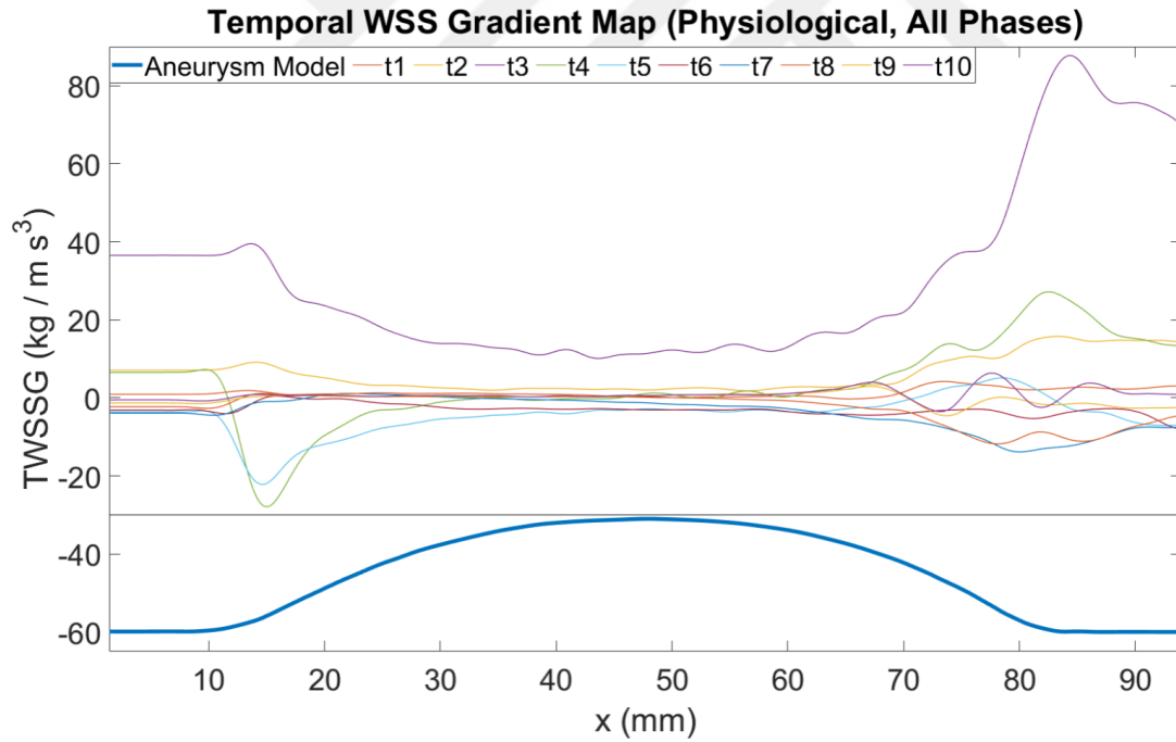
Figure 4.22: TWSSG distribution of all phases in physiological pattern
