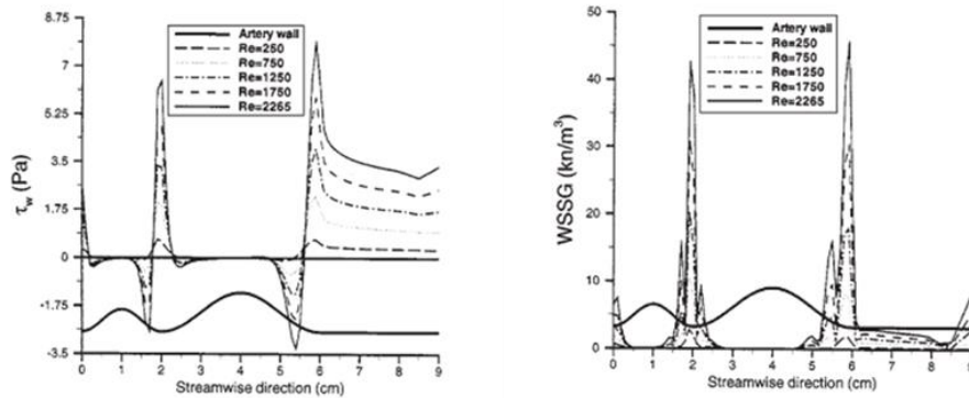
Figure 2.14: WSS and WSSG distribution for steady, selected Reynolds numbers [65]
