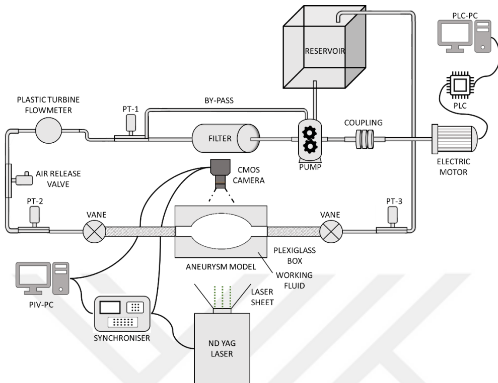
Figure 3.1: Schematics of the experimental set-up used in the present study
