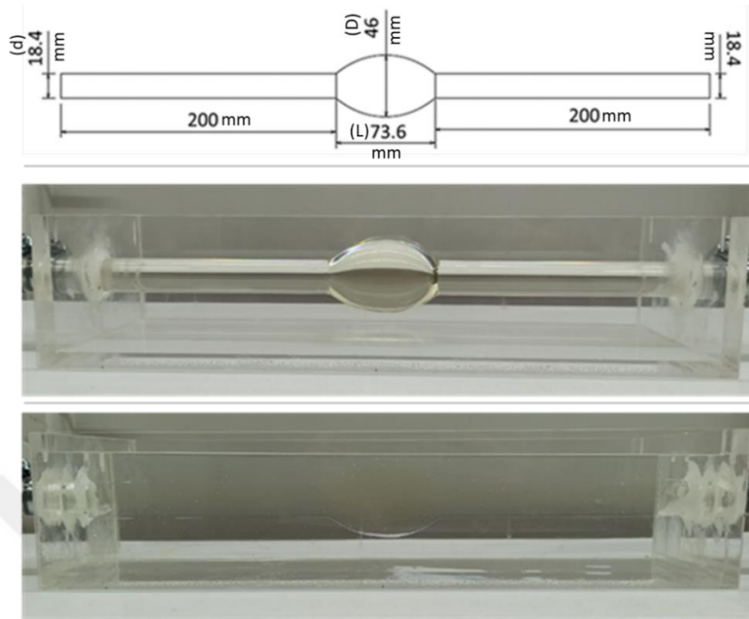
Figure 3.5: Aneurysm model - Above: Schematic of the model, Middle: Image of the model (Empty box), Below: Image of the model (The box full of working fluid)
