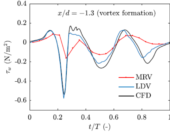
Figure 2.19: WSS variation at x/d = -1.3 with MRV, LDV and CFD results [75]
