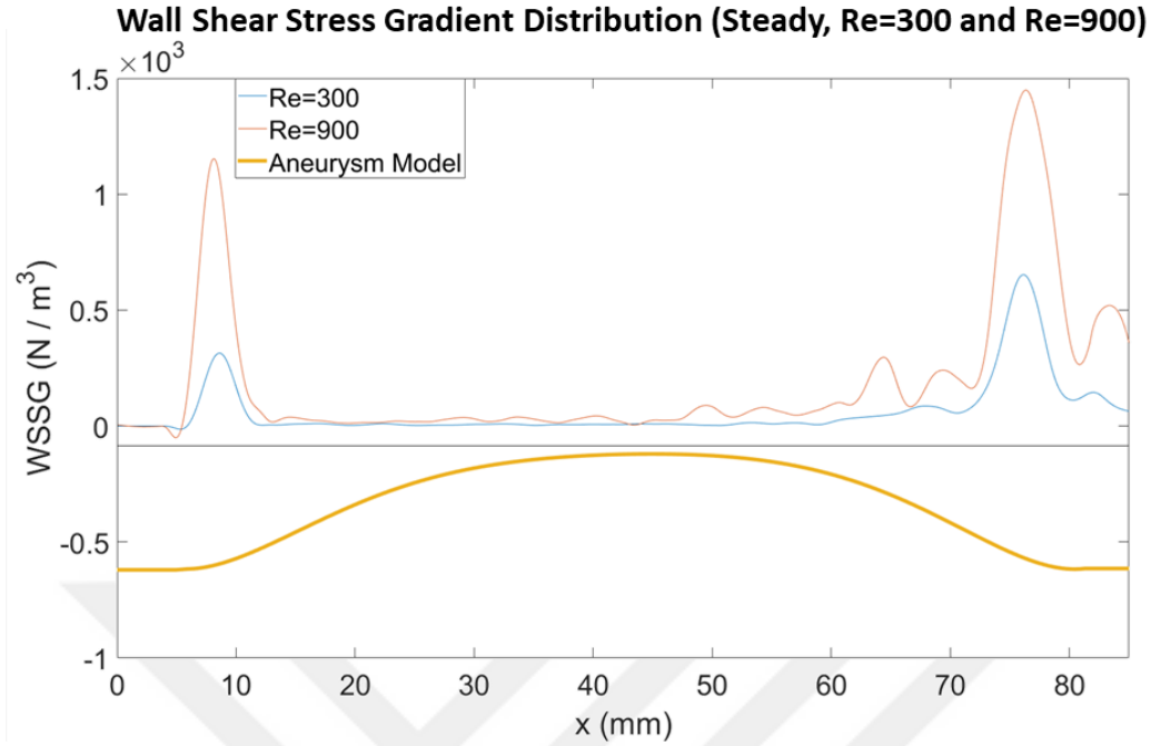
Figure 4.12: WSSG distribution for Re=300 and Re=900 under the steady flow (Absolute)
