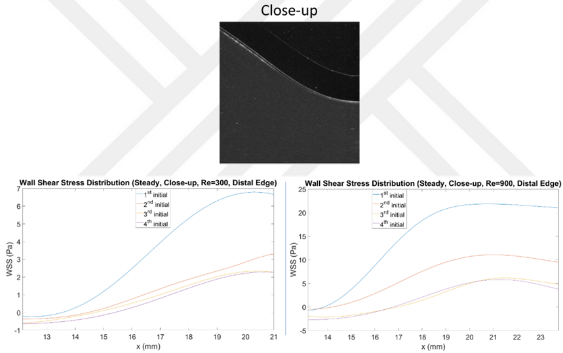
Figure 4.6: WSS distributions for close-up at distal edge ( Re=300 , Re=900 , Different initial data points)
