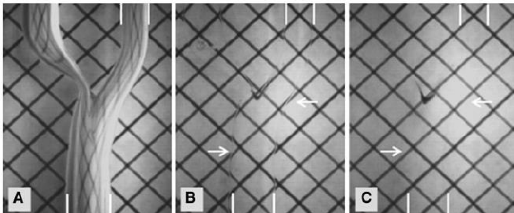
Figure 2.8: Presentation of the effect of the refractive index match between fluid and phantom model (Left to right filled with: Air – Nearly Matched RI – Optimally Matched RI) [39]
