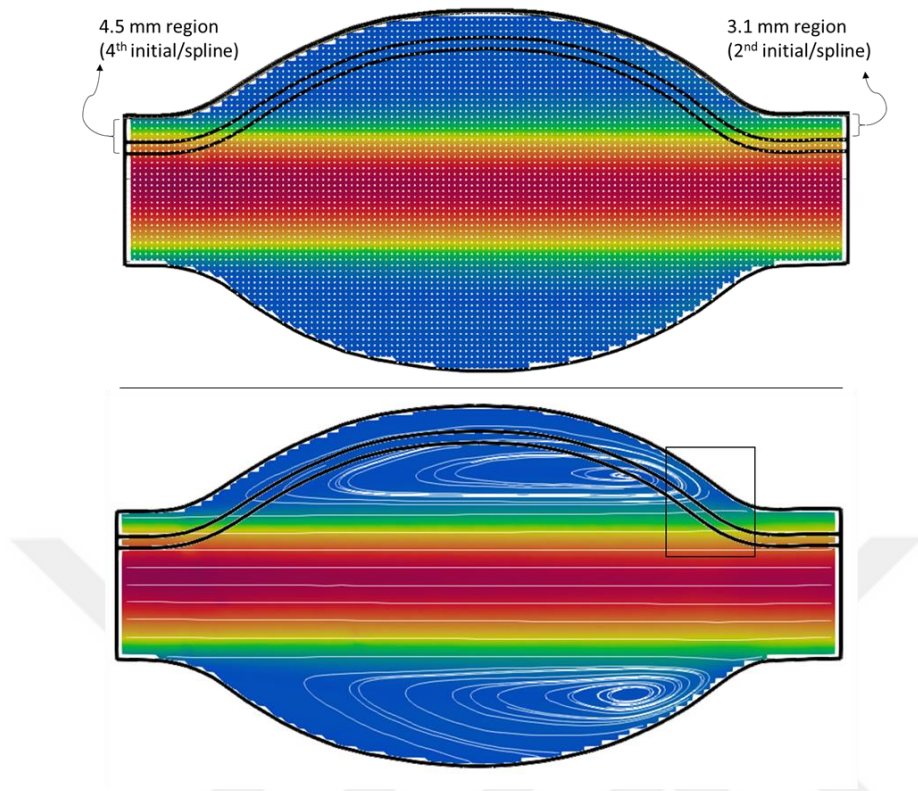
Figure 4.9: Presentation of data regions for different initial data points (Above: Data points, Below: Streamlines)
