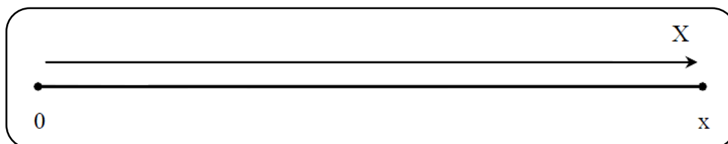
Figure 2.9 The random lifetime
