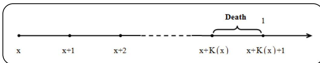
Figure 2.14 Death age and payment diagram for discrete whole life insurance
