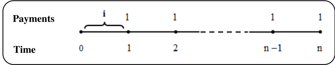
Figure 2.1 Time and payments diagram for the annuity-immediate
