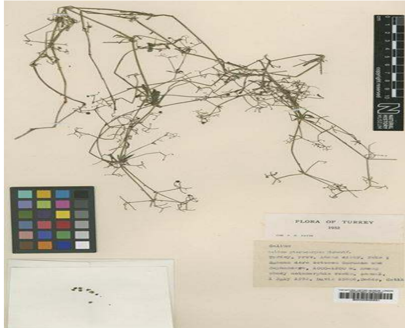
Şekil 3.4 Galium pterocarpum Ehrend. ( http://plants.jstor.org/specimen/bm000945631 )
