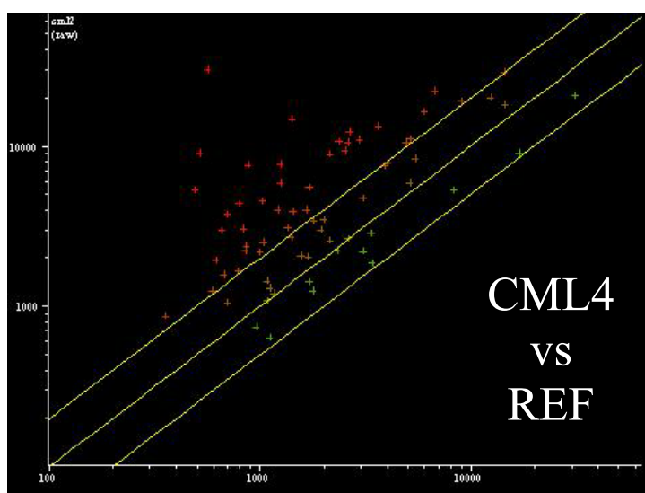
Figure 25: Scatter plot of 58 risk group indicator genes in CML 4. These genes were found to be expressed at least 3-fold higher in high-risk samples. In this figure, CML 4 is on the y-axis and the reference is on the x-axis.
