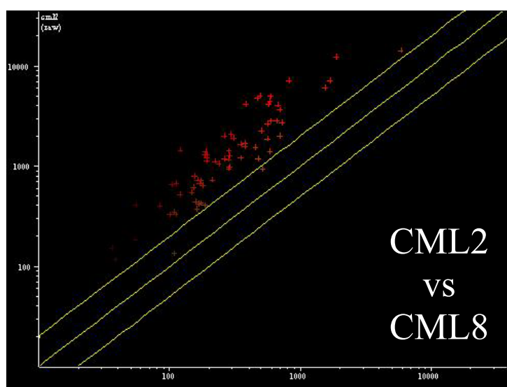
Figure 28: Scatter plot of CML 2 versus CML 8. CML 2 is on the y-axis and the CML 8 is on the x-axis.
