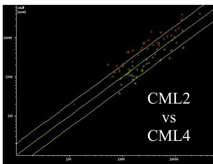
Figure 29: Scatter plot of CML 2 versus CML 4. CML 4 is on the y-axis and the CML 2 is on the x-axis.
