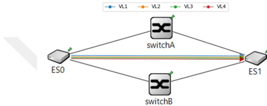
Figure 6.8 Experiment 2 – Topology
