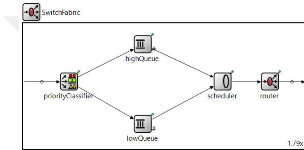
Figure 3.9 Switch Fabric Compound Module – Open Form
