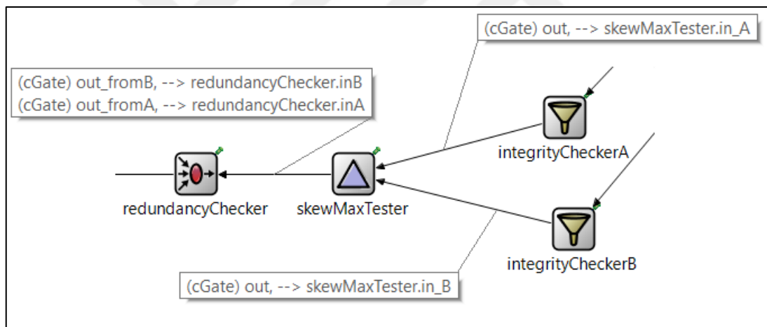
Figure 6.17 Experiment 5 – Skew Max Tester Block in End-System
