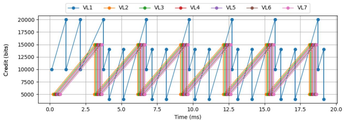
Figure 6.14 Experiment 3 – Change in Credit for Sigma = 20000 bits
