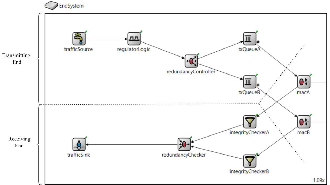
Figure 3.3 End-System Compound Module
