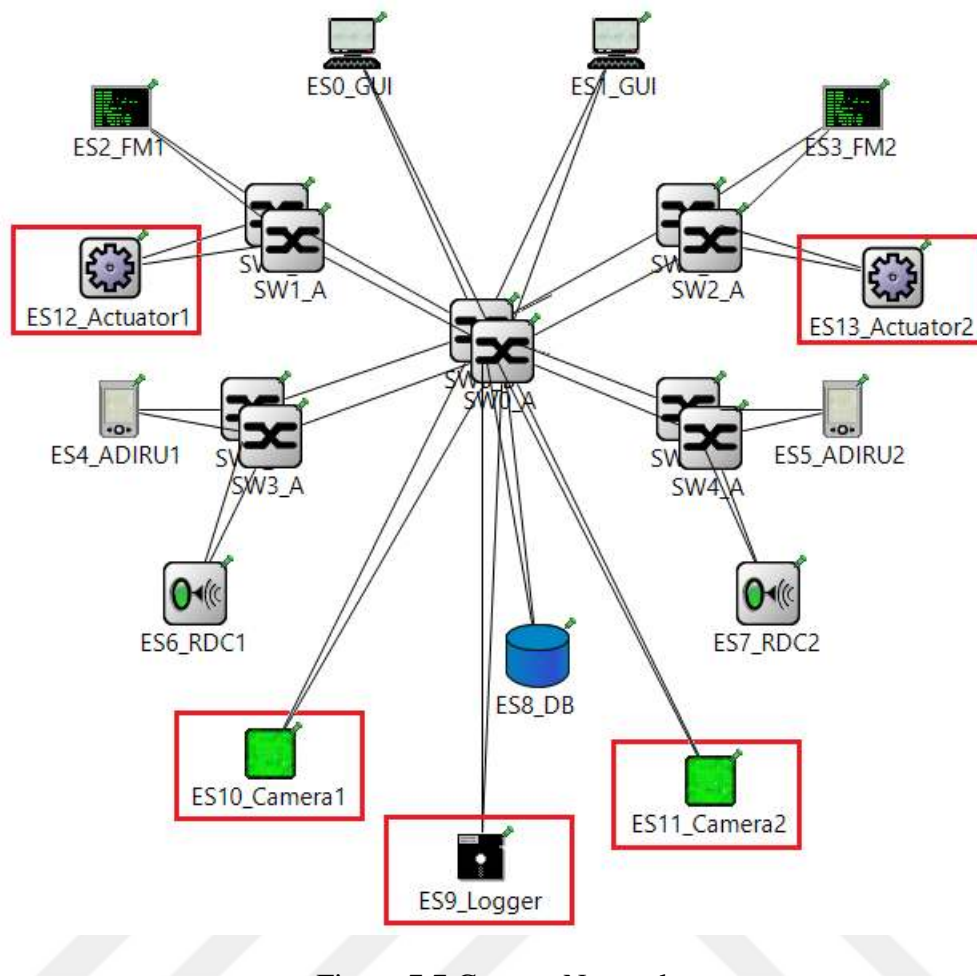
Figure 7.7 Custom Network
