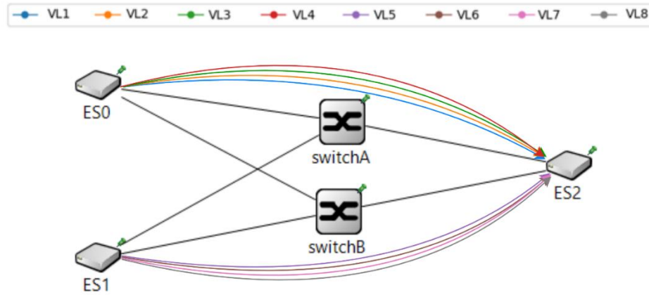
Figure 6.15 Experiment 4 – Topology
