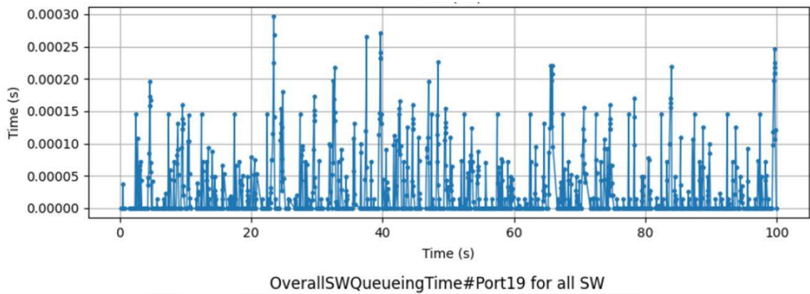
Figure 7.4 Queueing Time for SW0-ES19
