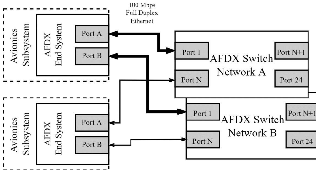
Figure 2.5 Switch – End-System Connections
