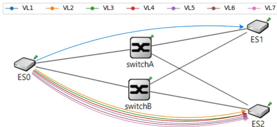
Figure 6.12 Experiment 3 – Topology
