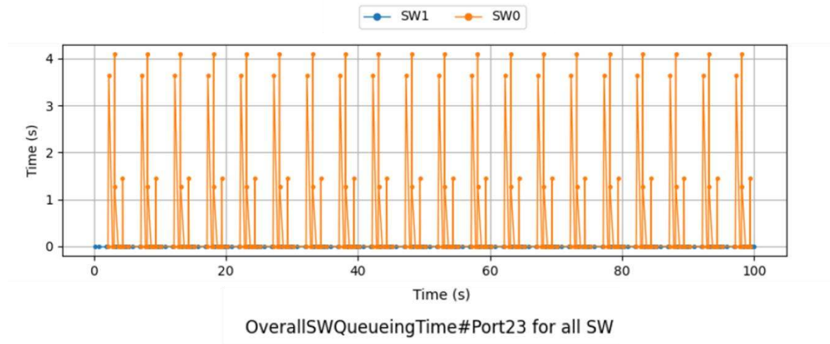
Figure 7.6 Queueing Time for SW0-SW1
