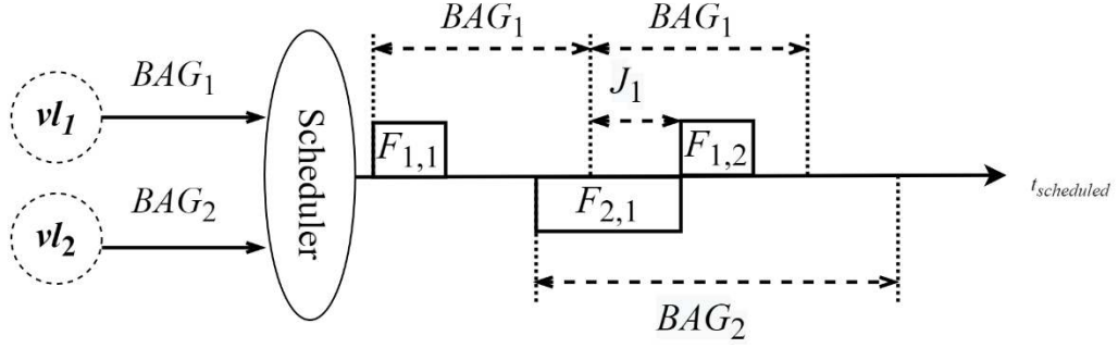
Figure 2.4 End-System Scheduling
