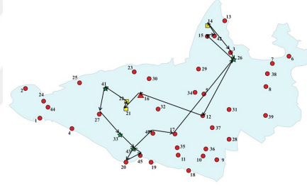
(b) Arc Profit PDARP (Solution a )
