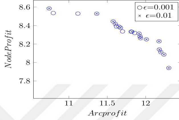
(a) Set Coverage performance: \epsilon=0.001 vs. \epsilon=0.01
