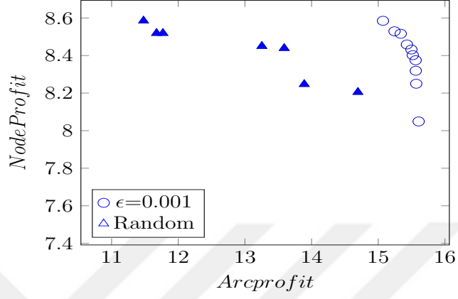
(a) Model Under \epsilon=0.001 vs. Random
