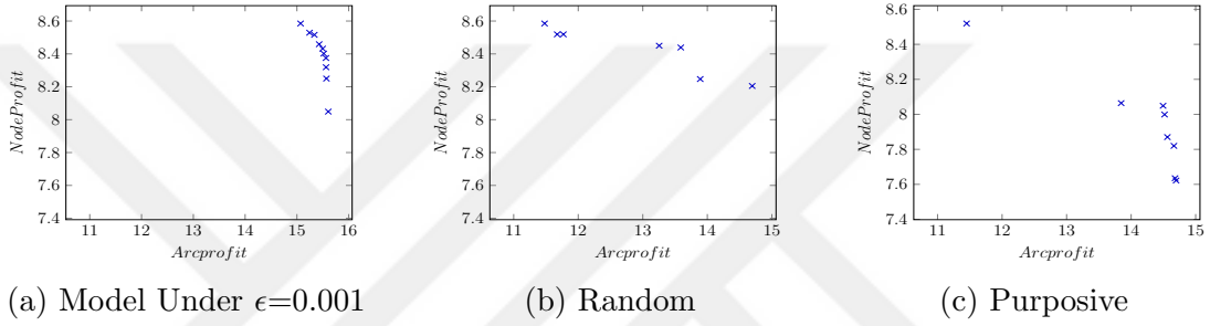
Figure 7.2: Spacing performances of Pareto Fronts of the instance (|D|, |M|)=(1,2) model under \epsilon value 0.001 and random and purposive improvement heuristics
