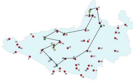
(c) Node profit PDARP (Solution b )
