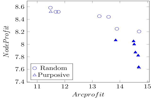
(c) Random vs. Purposive
