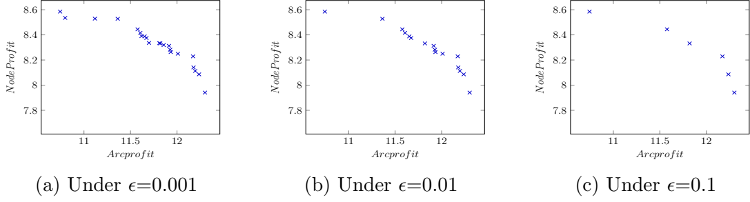
Figure 5.4: Spacing performances of Pareto Fronts of the instance (|D|, |M|)=(1,1) under \epsilon values 0.001, 0.01, 0.1
