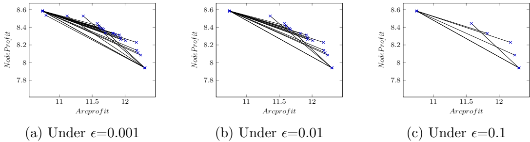
Figure 5.5: Maximum Spread performances of Pareto Fronts of the instance (|D|, |M|)=(1,1) under \epsilon values 0.001, 0.01, 0.1
