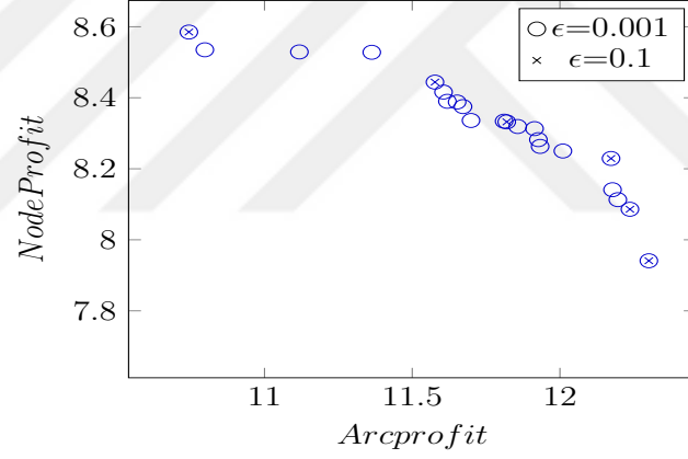
(b) Set Coverage performance: \epsilon=0.001 vs. \epsilon=0.1
