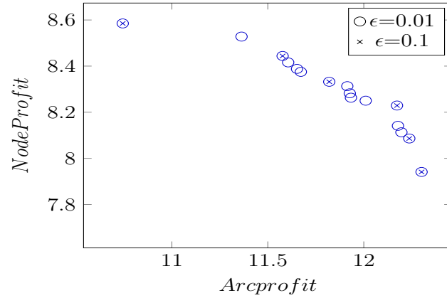
(c) Set Coverage performance: \epsilon=0.01 vs. \epsilon=0.1
