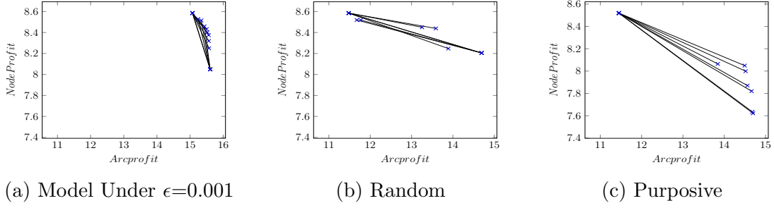
Figure 7.3: Maximum Spread performances of Pareto Fronts of the instance (|D|, |M|)=(1,2) model under \epsilon value 0.001 and random and purposive improvement heuristics
