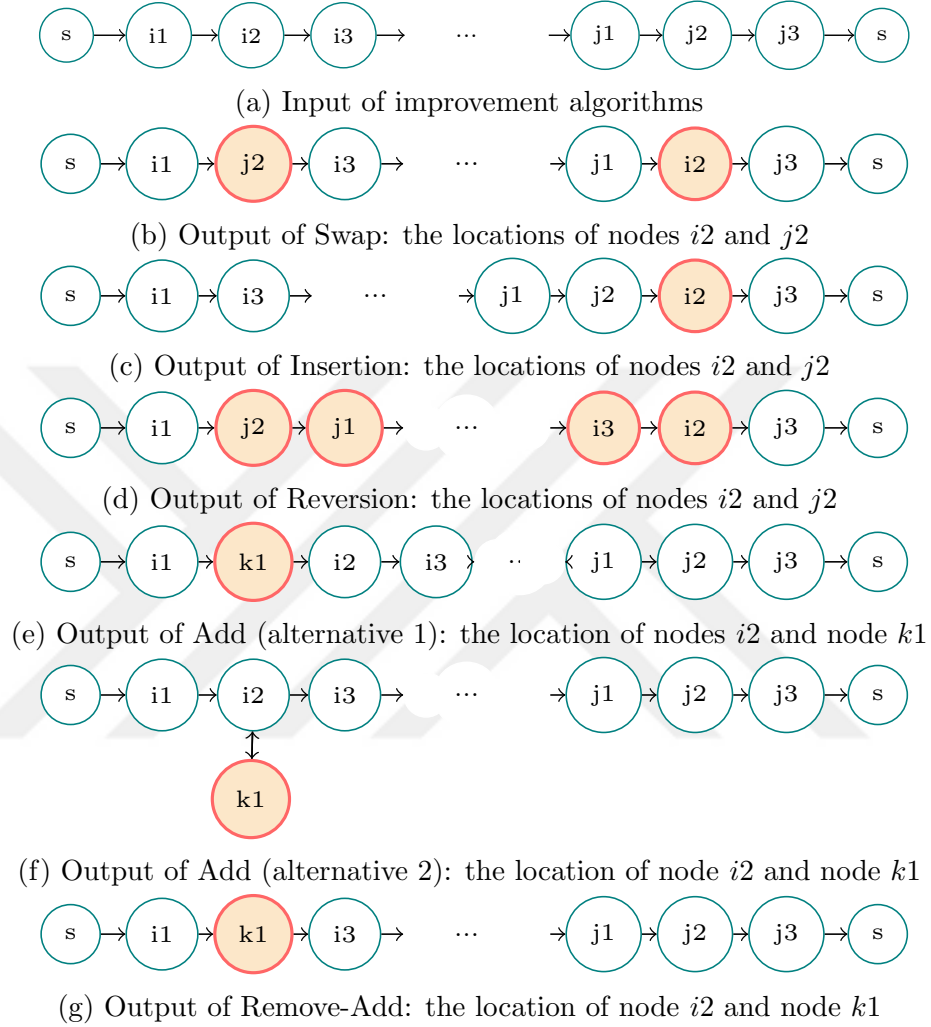
Figure 6.1: Illustrative example of the improvement algorithms.
