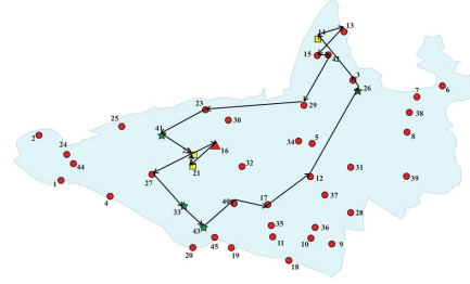
(d) An Example Non-dominated Pareto Solution (Solution c )
