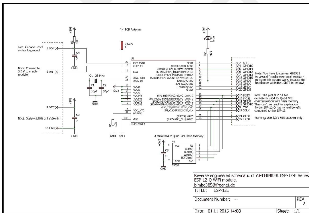
Figure 25 ESP8266 ESP-12 Module Schematic
