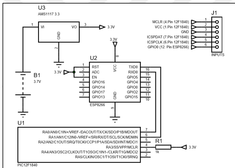
Figure 28 EHU Design
