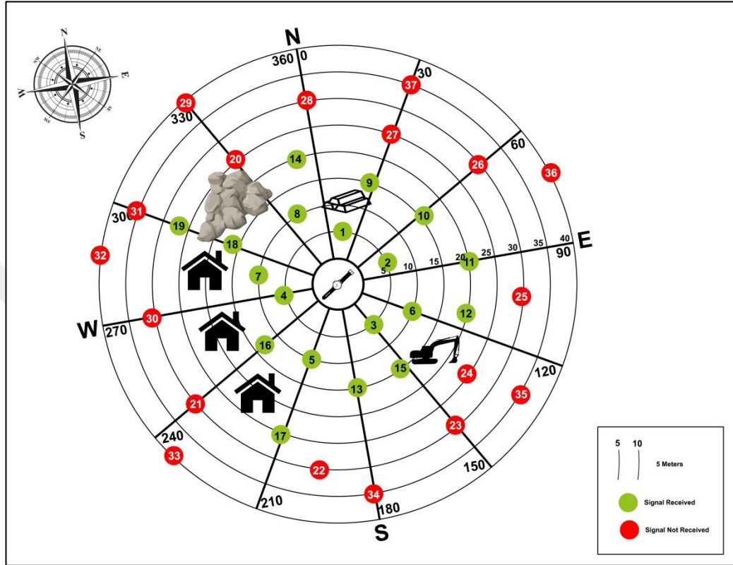
Figure 43 Signal Power From EHU Located in Wreckage (Device II)
