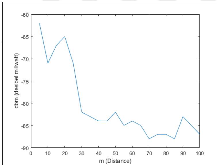
Figure 35 The (Average) Values Received From EHU to EHDU According to the Distance
