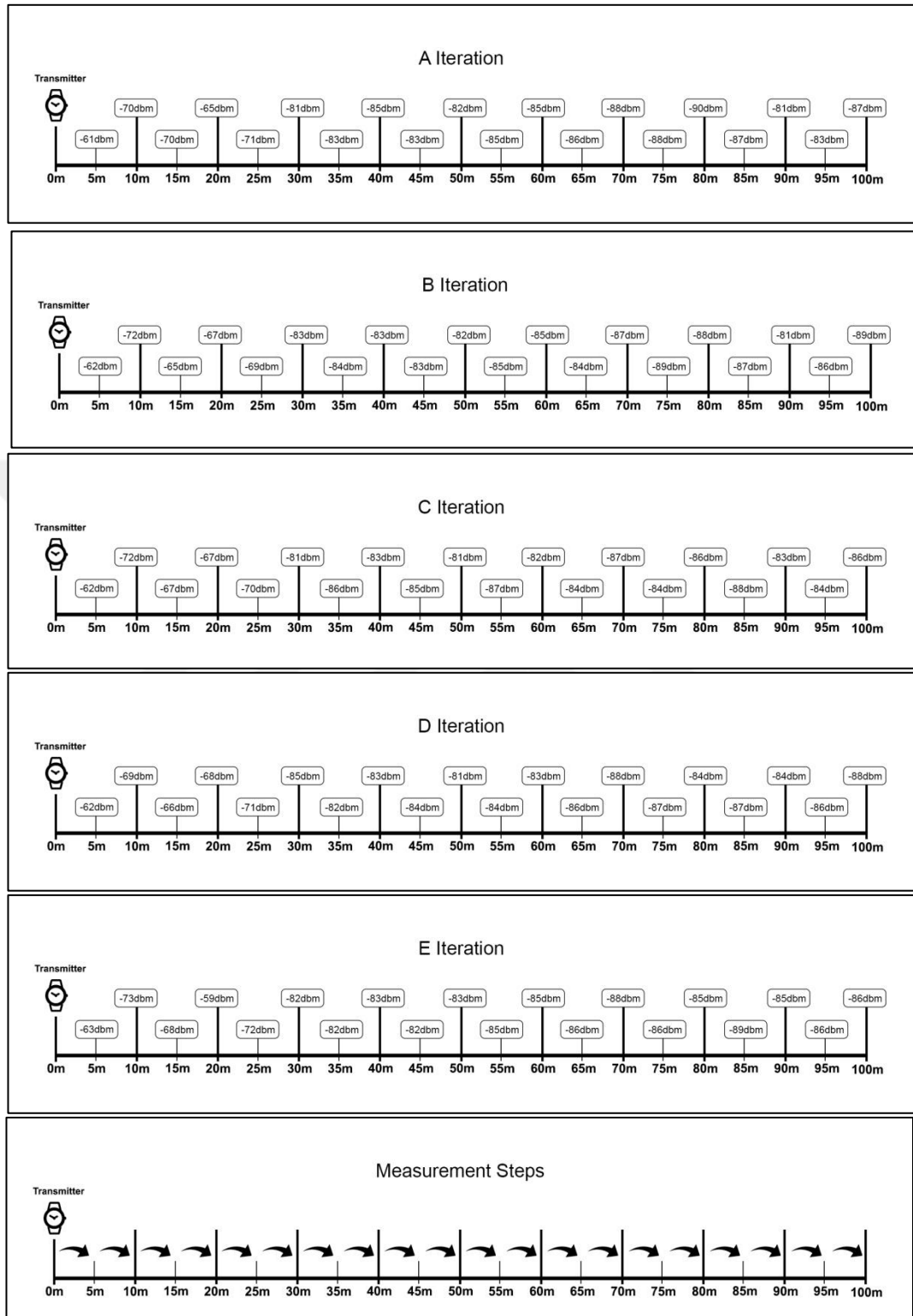
Figure 33 Distance Test Iterations For EHDU
