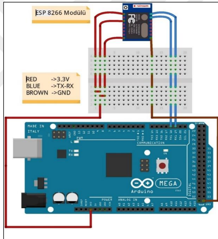
Figure 26 ESP Module And Arduino Mega Connection
