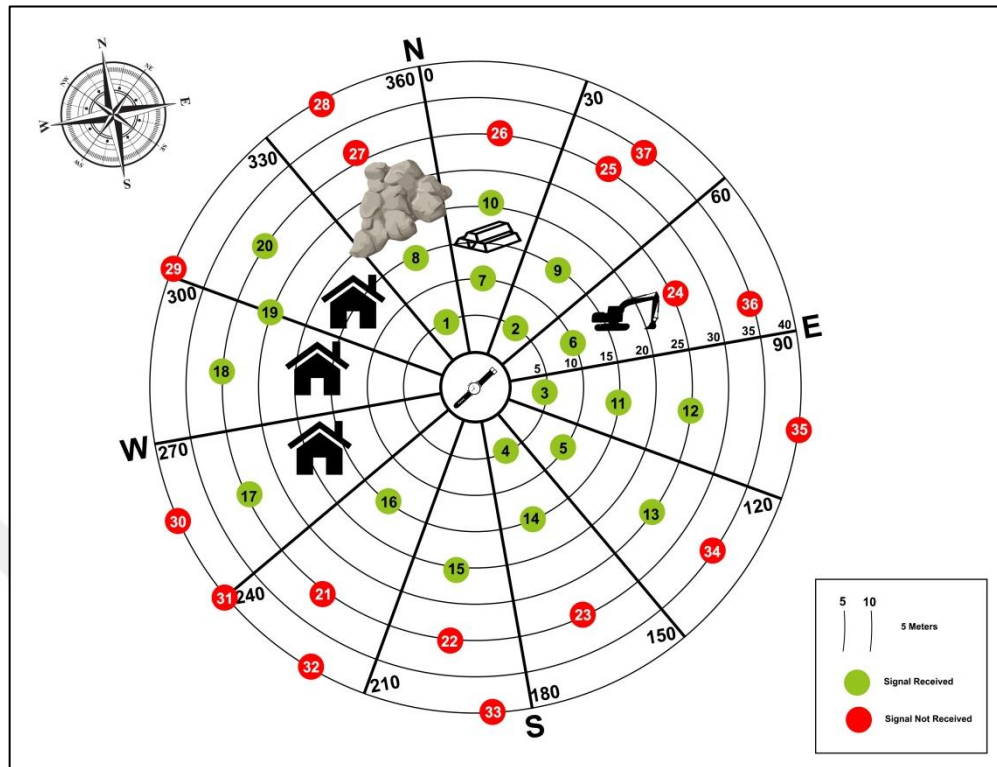
Figure 42 Signal Power From EHU Located in Wreckage (Device I)
