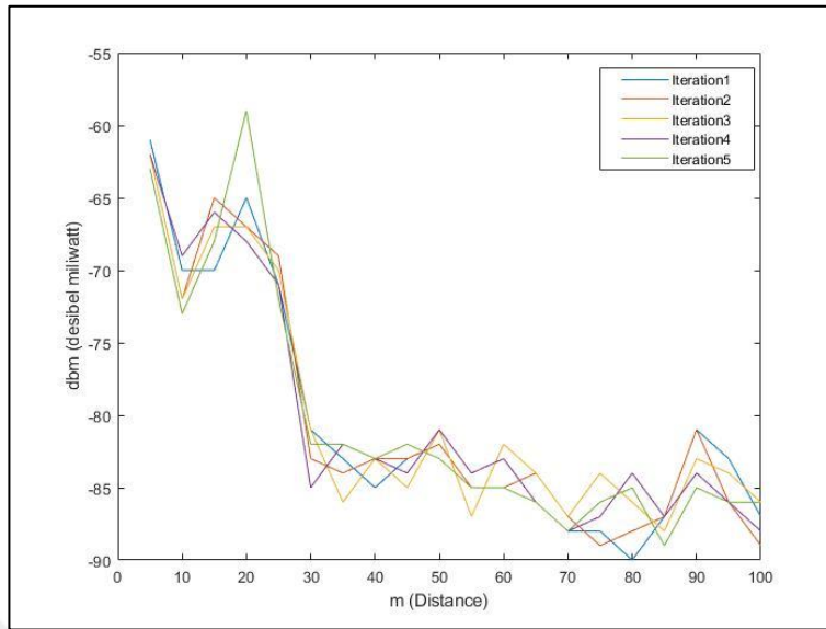
Figure 34 The Values Received From EHU to EHDU (5 iteration)
