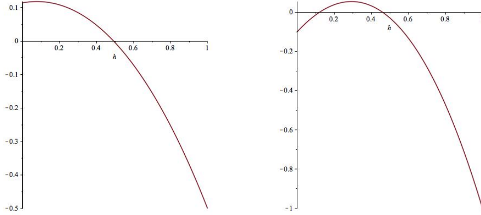
(a) F(h) for low level of cost c = 1
