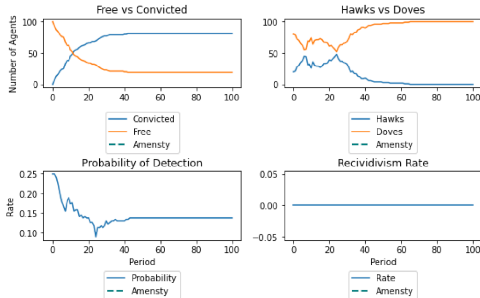
Figure 4.4 – Simulation III ( v = c imprisonment and no amnesty)
