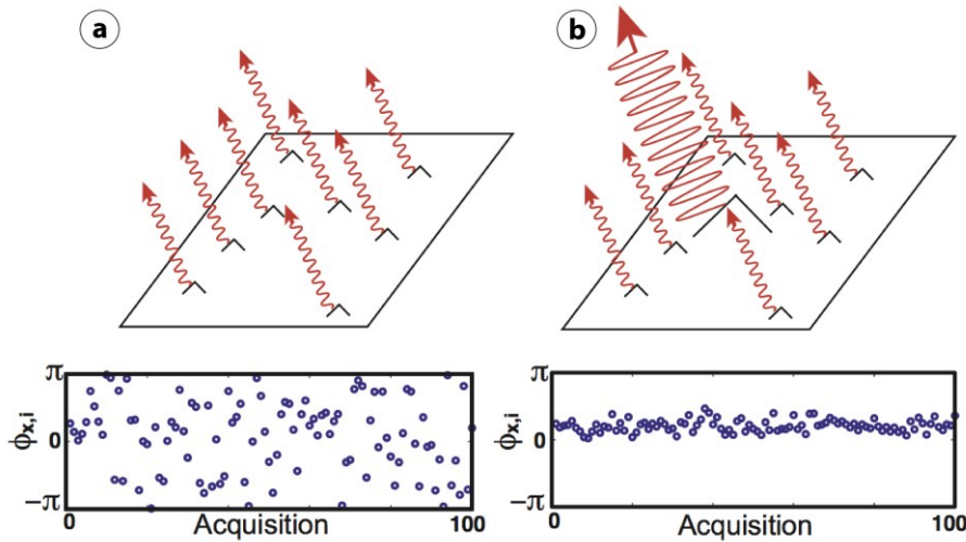
Figure 2.1 : Phase simulations from Hooper et al. (2007) for (a) a distributed scatterer pixel and (b) a persistent scatterer pixel. The cartoons above represent the scatterers contributing to the phase of one pixel in an image and the plots below show simulations of the phase for 100 iterations, with the smaller scatterers moving randomly between each iteration. The brighter scatterer in (b) is three times brighter than the sum of the smaller scatterers.
