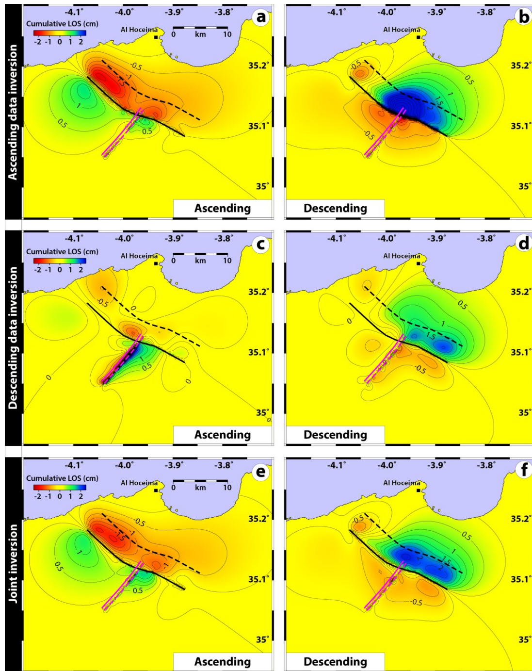
Figure C.6 : Model of 3.3-year cumulative LOS postseismic surface deformation predicted by the two fault rupture inversions according to PS LOS change in the southern section of the fault. Black line shows the main modeled fault. Pink line indicates the fault branch obtained using PS LOS displacement fields.
