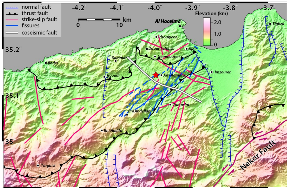
Figure 4.2 : Tectonic map of the Al Hoceima region (compiled from Calvert et al., 1997; Ait Brahim et al., 2004b) with surface cracks and fissures observed after the 2004 event (redrawn from Ait Brahim et al., 2004a). Thick white line is the surface trace of the modeled fault plane.
