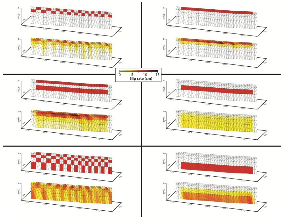
Figure D.4 : Resolution test using checker-box approach with 0.10 m slip at different depths for each cell.
