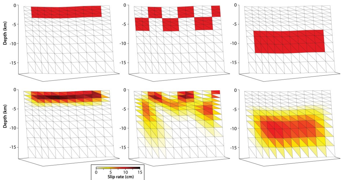
Figure C.8 : Resolution test using checker-box approach with 0.10 m slip at different depths for each cell.
