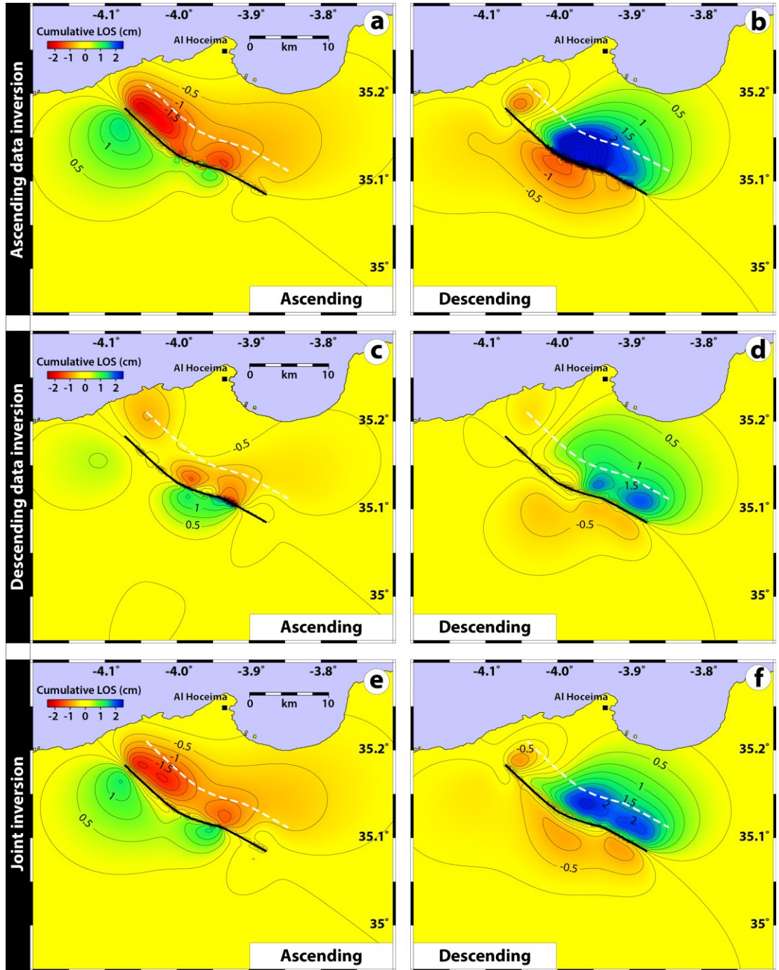
Figure C.3 : Model of 3.3-year cumulative LOS postseismic surface deformation predicted by the modeled slip distribution shown in Figure 4.11. Black lines show the top of the modeled fault. White dashed lines show the bottom of the modeled fault.
