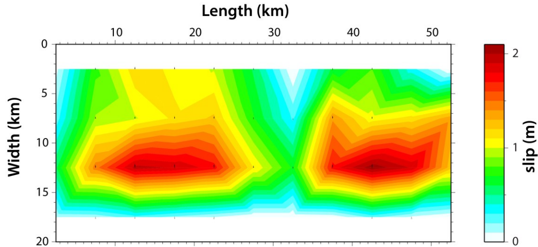
Figure B.1 : Coseismic slip distribution used as an input file for PSCMP, which is simulated on a planar fault by enforcing the slip distribution deduced by Belabbes et al. (2009), is 55-km-long and 20-km-wide offshore thrust fault striking N60°, and dipping 42° SE.
