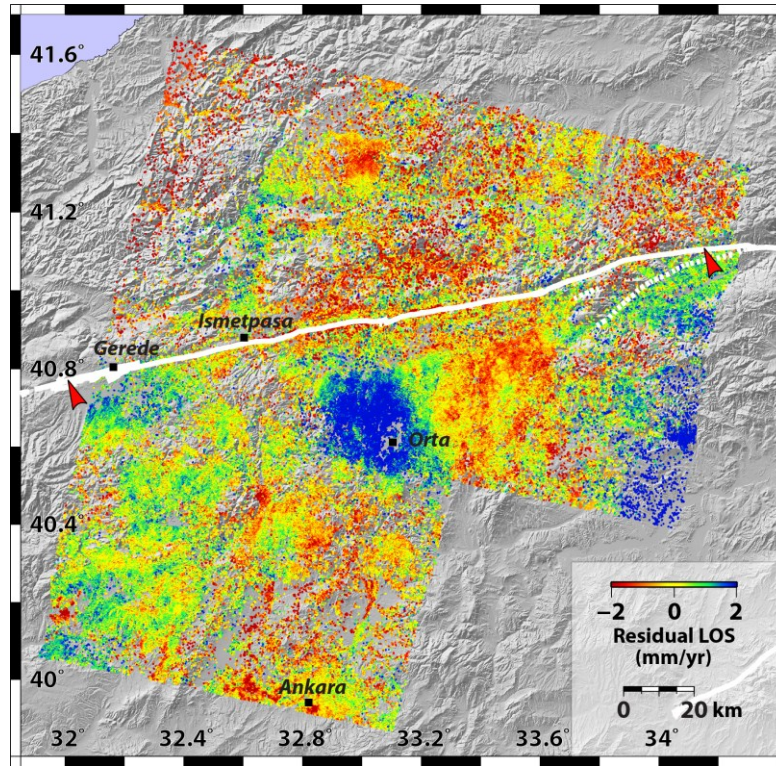
Figure D.3 : Residual LOS velocity field.
