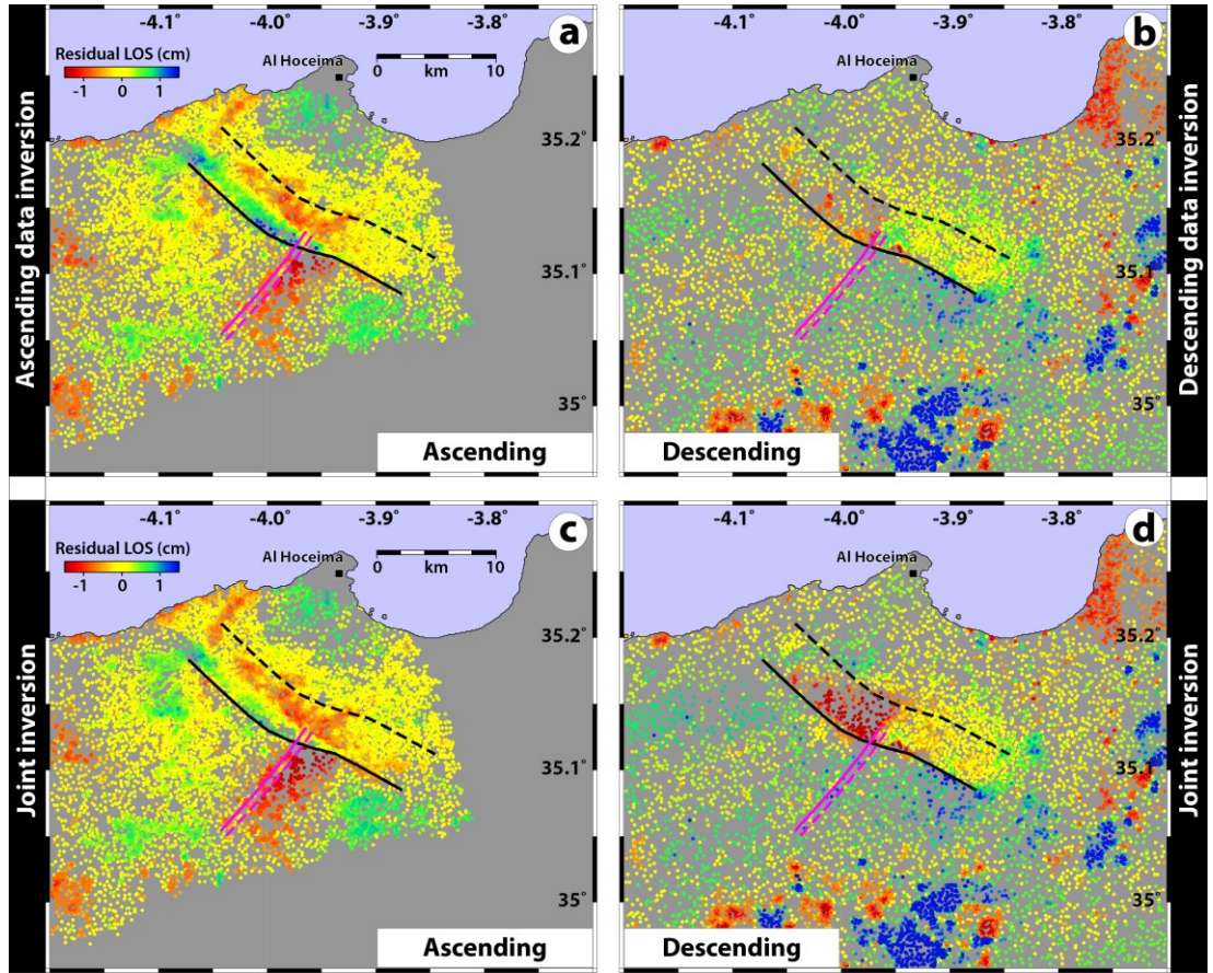
Figure C.7 : Residual maps obtained after subtracting the synthetic InSAR data (Figure C.5) from the observed data (shown in Figure 4.10). Residuals after inversion of (a) the ascending and (b) the descending data alone, and (c, d) jointly with a lower weighting for the descending data. Black line shows the main coseismic model fault, and pink line is the secondary fault branch.
