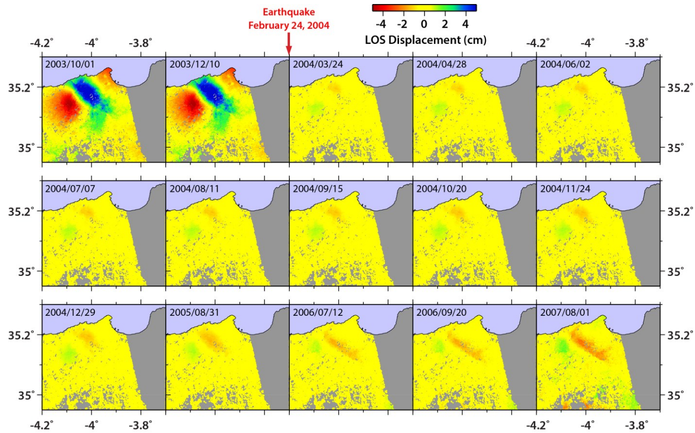
Figure C.2 : Time series of ascending LOS for Al Hoceima region between 2003 and 2007. Each image represents the incremental displacement towards the satellite since the time of the previous image, relative to pixels in the northwest corner.
