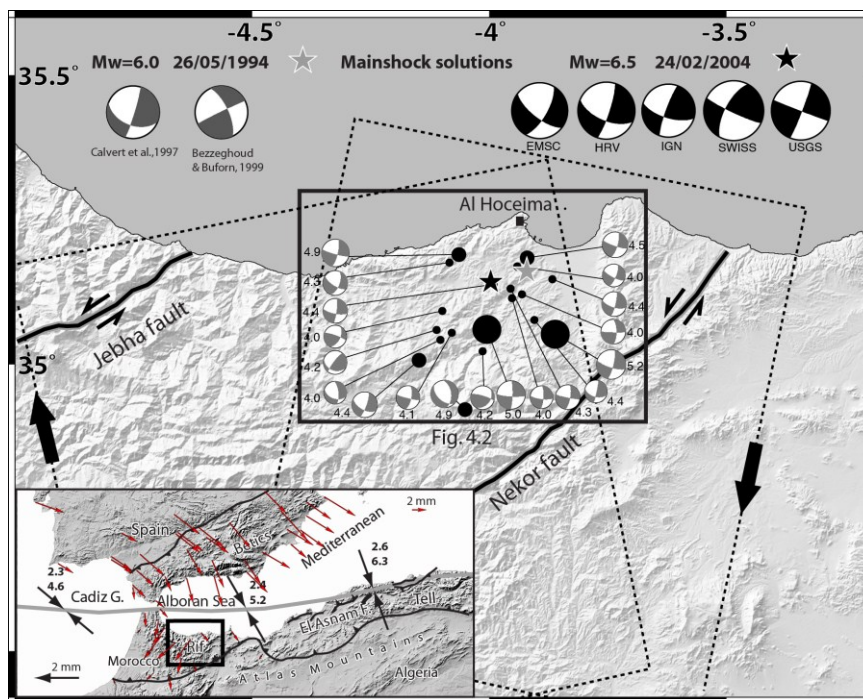
Figure 4.1 : Al Hoceima region of Morocco with shaded relief (SRTM 90m). Large beach balls are focal mechanism solutions of the May 26, 1994 and February 24, 2004 Al Hoceima earthquakes (Calvert et al., 1997; Bezzeghoud and Buform, 1999), whose epicenters are indicated by gray and black stars, respectively. Small black circles are M > 4 aftershocks from IGN with focal mechanism solutions from Buform et al. (2004) and Stich et al. (2005). Dashed rectangles are the frames of the Envisat radar images with arrows showing the flight direction of the satellite. The convergent plate boundary between Africa and Eurasia is depicted with a thick gray line in the inset map with arrows illustrating the direction and estimated rate (min. and max.) of convergence (Nocquet and Calais, 2004). Red arrows indicate the recent GPS measurements (Koulali et al., 2011).
