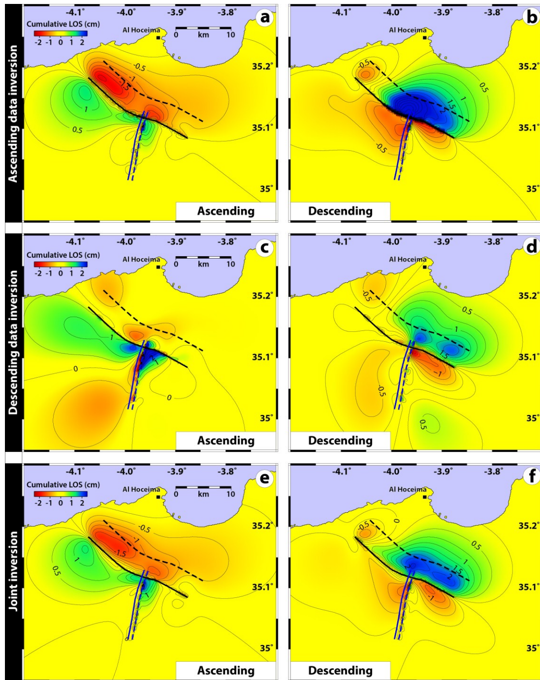
Figure C.4 : Model of 3.3-year cumulative LOS postseismic surface deformation predicted by the two fault rupture inversions according to aftershocks distribution. Black line shows the main modeled fault. Blue line indicates the fault branch obtained using aftershocks distribution.
