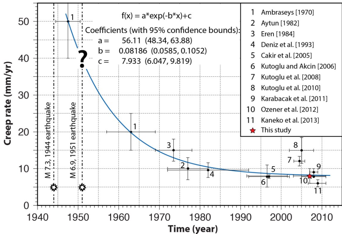
Figure 5.11 : Time history of surface creep at Ismetpaşa as reported by various studies following the 1944 earthquake (after Cakir et al., (2005)). Horizontal and vertical bars are the time window and error range of measurements, respectively. The question mark corresponds to the unknown effect of the 1951 earthquake on creep rate. Curve shows the fit of the exponential relaxation function to the change of the creep rate with time (Savage, 2005).
