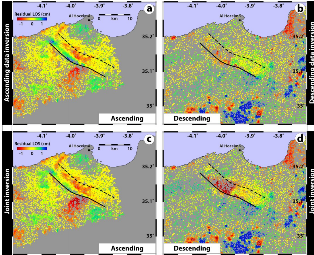
Figure 4.12 : Residual maps obtained after subtracting the synthetic InSAR data (Figure C.2) from the observed data (shown in Figure 4.10). Residuals after inversion of (a) the ascending and (b) the descending data alone, and (c, d) jointly with a lower weighting for the descending data. Black line is the top of the coseismic model fault, and the dashed black line is the bottom of the coseismic model fault.
