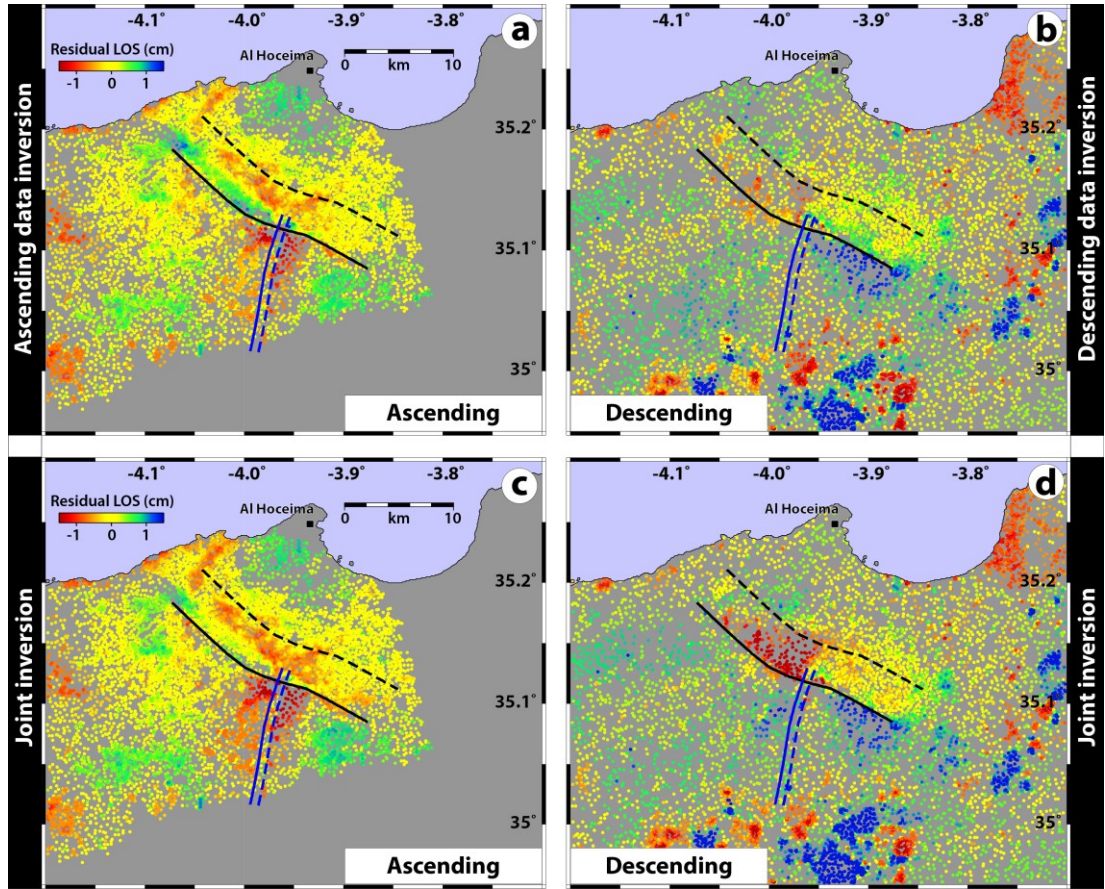
Figure C.5 : Residual maps obtained after subtracting the synthetic InSAR data (Figure C.3) from the observed data (shown in Figure 4.10). Residuals after inversion of (a) the ascending and (b) the descending data alone, and (c, d) jointly with a lower weighting for the descending data. Black line shows the main coseismic model fault, and blue line is the secondary fault branch.
