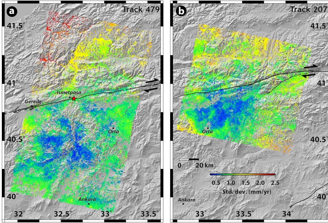
Figure D.1 : Velocity standard deviation maps calculated by StaMPS using bootstrapping.
