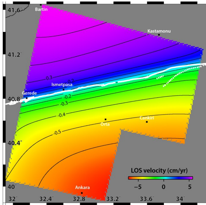
Figure D.2 : Variable interseismic slip model using multiple fault patches to flatten the far field velocity field.
