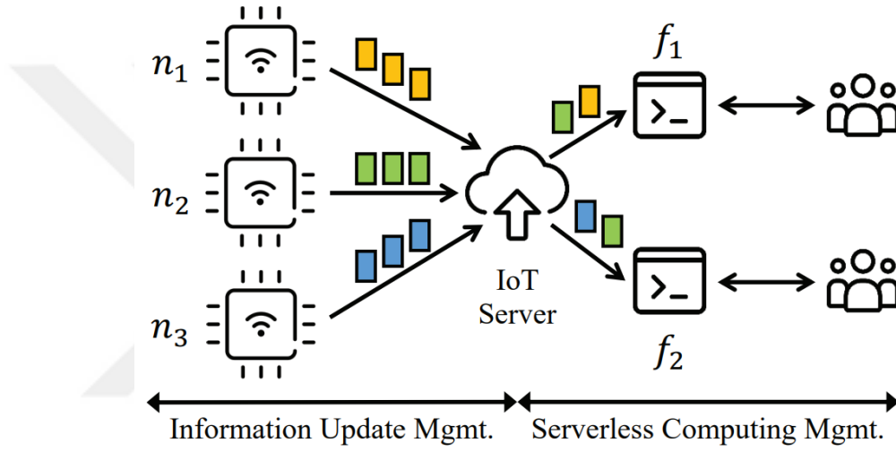
Figure 3.9. An IoT system with three IoT devices and two serverless functions [126],
