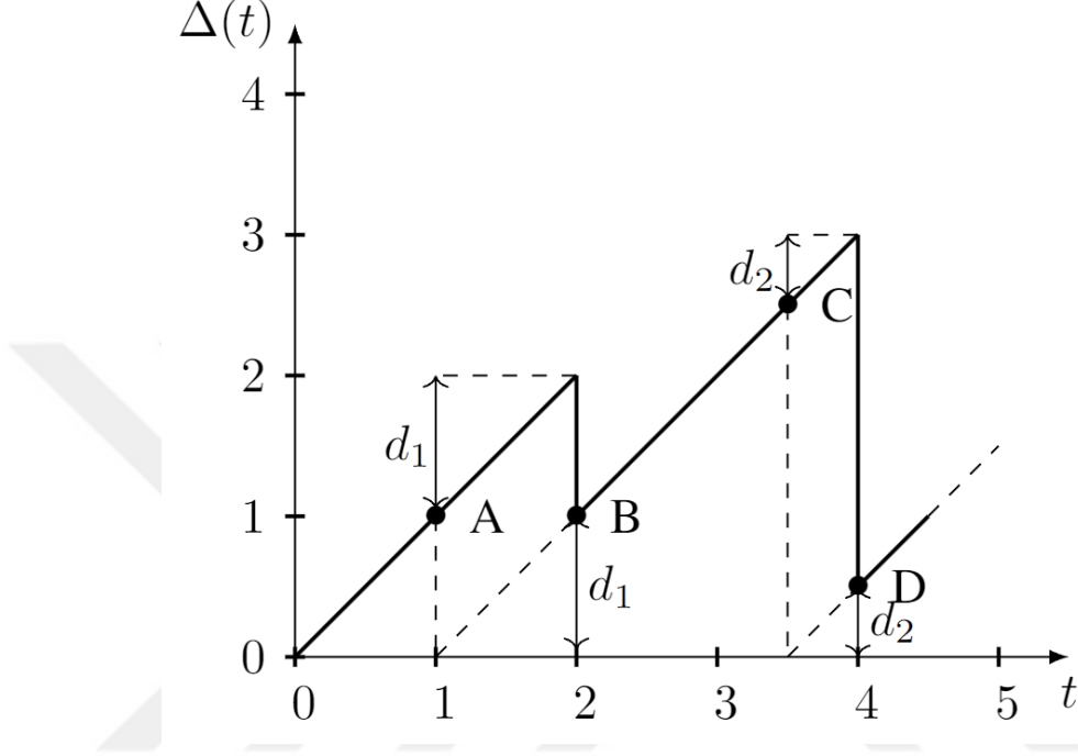
Figure 2.1. An example graph for the age of information at a receiver.
