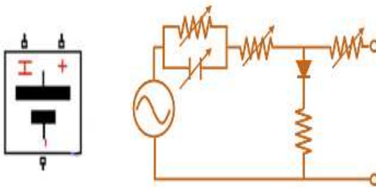
Figure 3.5. Battery cell equivalent of a discharge circuit.
