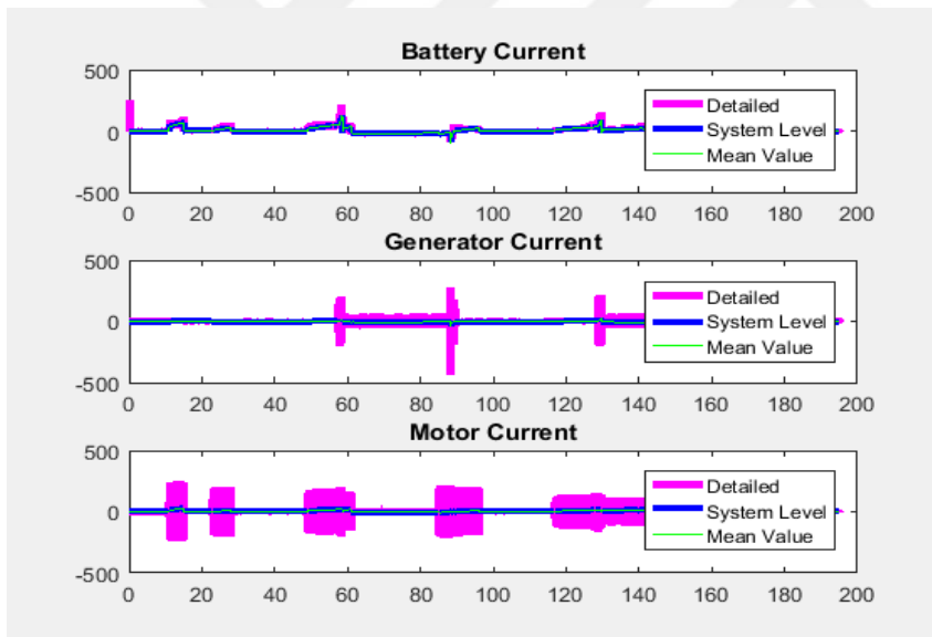
Figure 4.4. Currents obtained from urban driving cycle.
