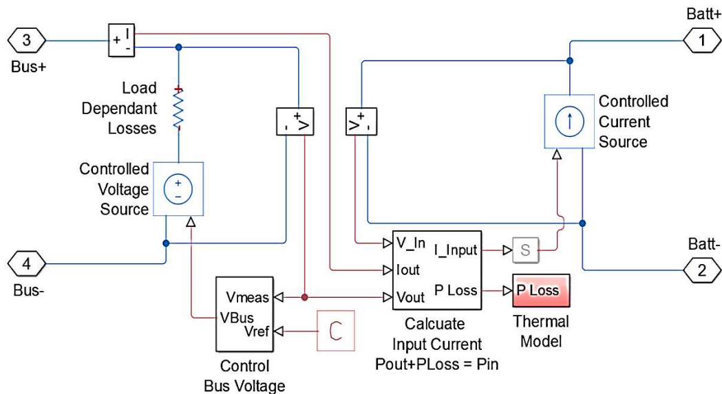
Figure 3.7. DC-DC-Convertor system.
