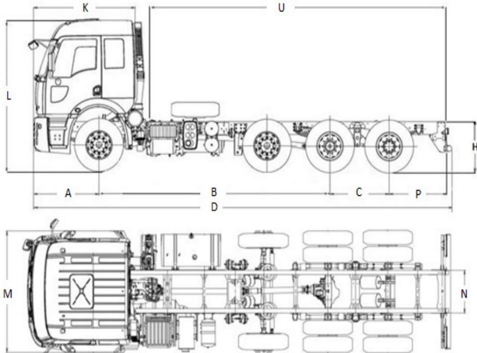
Figure 4.1 : Dimensions of the Vehicle 1 [29].
