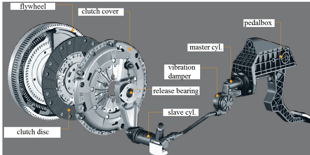
Figure 2.3 : Overview of the clutch and clutch actuation system [8].
