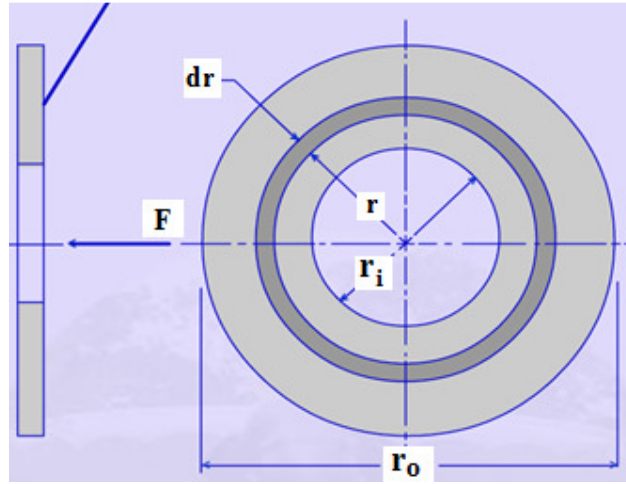
Figure 3.1 : Single surface axial disc clutch [27].
