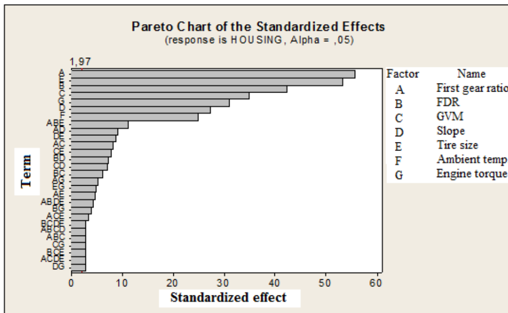
Figure 6.2 : Pareto chart for the clutch housing temperature.
