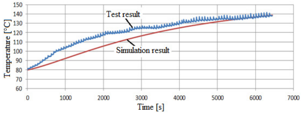
Figure 5.9 : Clutch housing temperature vs time – Vehicle 3.
