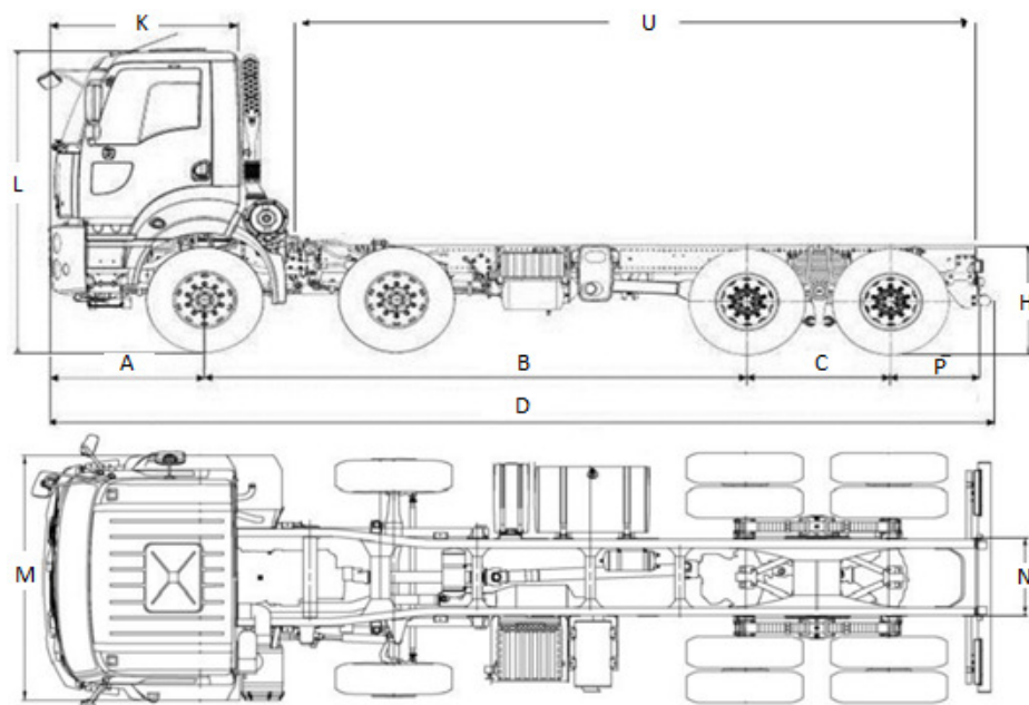
Figure 4.3 : Dimensions of the Vehicle 2 [30].
