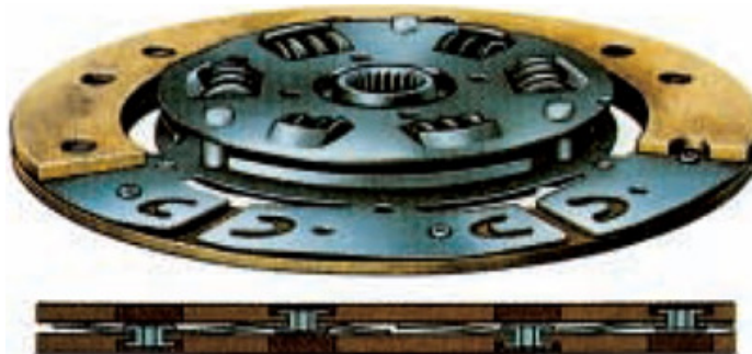
Figure 2.14 : Cushion disc [9].
