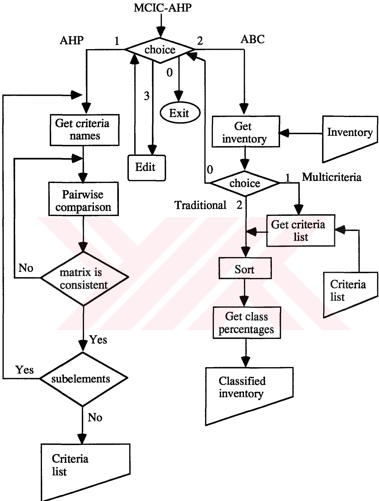
Fig. A.1. Flow-chart of MCIC-AHP.
