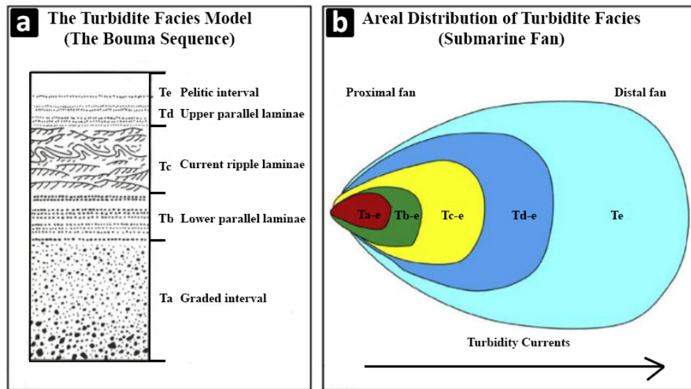
Figure 2.1. Schematic representation of the Bouma sequence. a) Columnar section view and b) Map view of a typical turbidite in the Bouma sequence (From Shanmugam, 2016).
