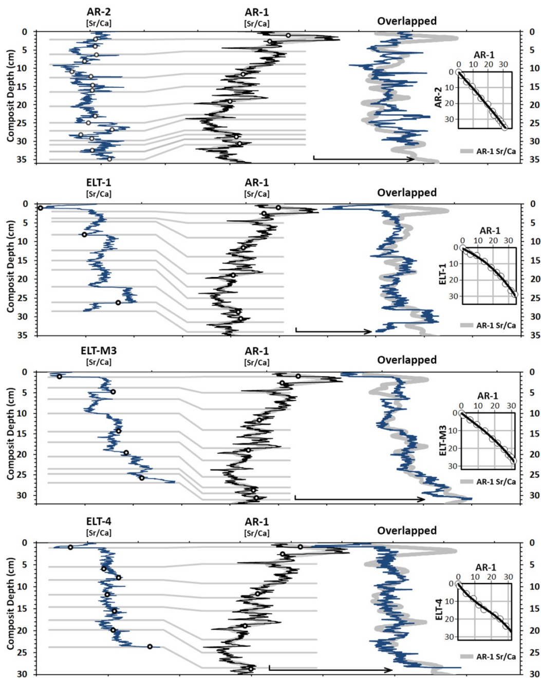
Figure 5.6. The correlation between the cores taken from the north of the AR-1 core-site. (Northern cores are AR-2, ELT-1, ELT-M3, and ELT-4). Small insets in the right of the graphs are transfer functions representing depth adjustments.
