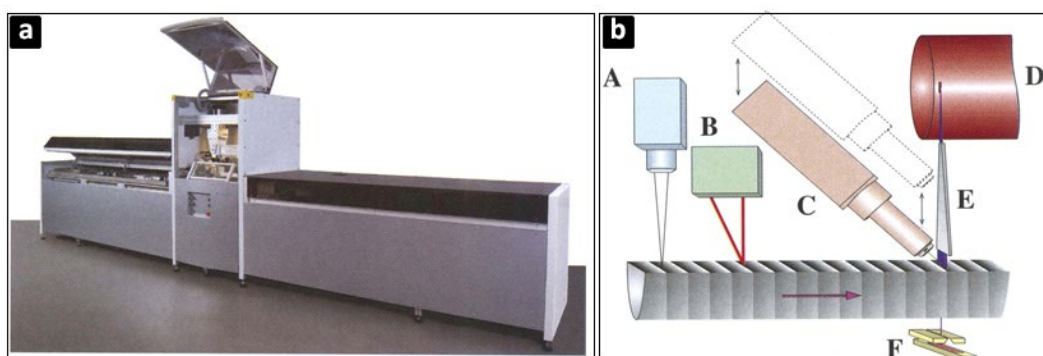
Figure 3.8. a) A photo from the ITRAX Micro XRF core scanning device. b) Parts included in the ITRAX Micro XRF system (Croudace et al., 2006). A - optical-line camera, B - laser triangulation system, C - motorized XRF Si-drift chamber detector, D - 3 kW X-ray tube, E - flat-beam X-ray waveguide, and F - X-ray line camera.
