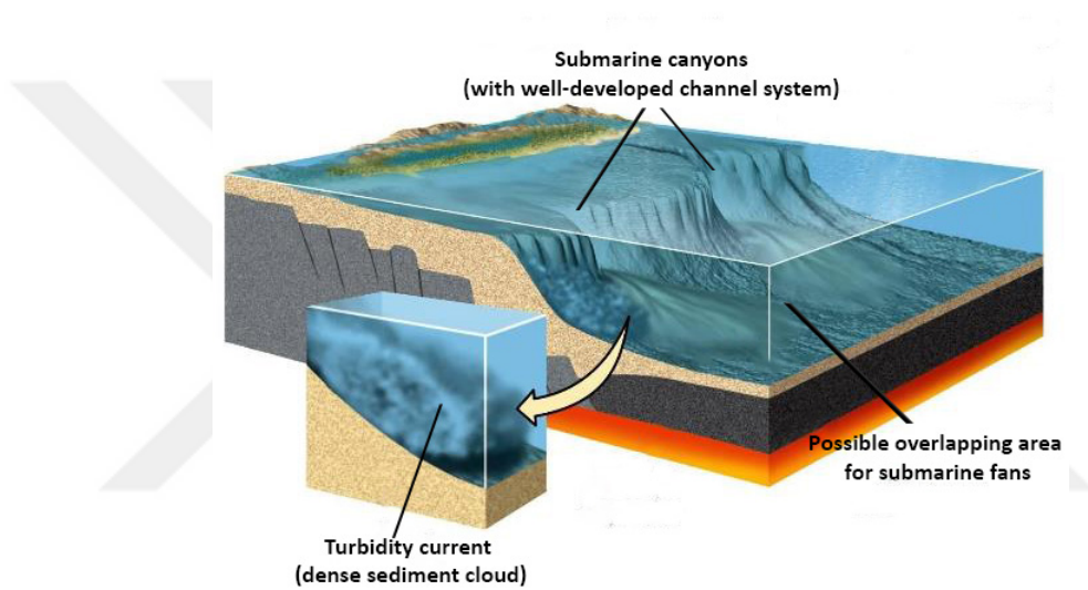
Figure 2.3. Schematic diagram of submarine canyons with well-developed channel system (Modified from Grotzinger & Jordan, 2010).
