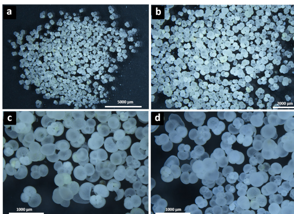
Figure 3.10. Photographs of planktonic foraminifera samples extracted from sediment cores. The photographs were taken under a binocular microscope with different magnifications.
