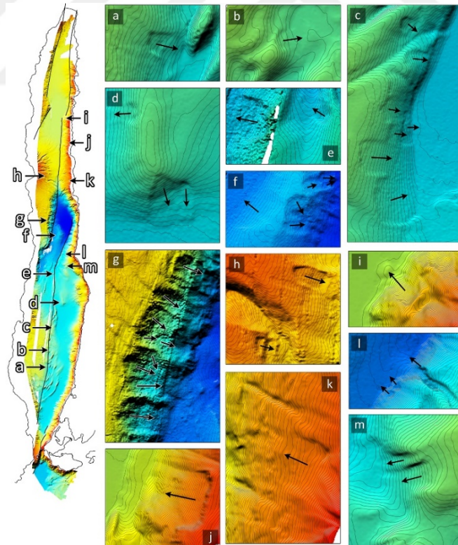
Figure 4.1. Noticeably well-imaged landslides in the close bathymetry of the Gulf of Aqaba. Arrows indicate the flow directions.
