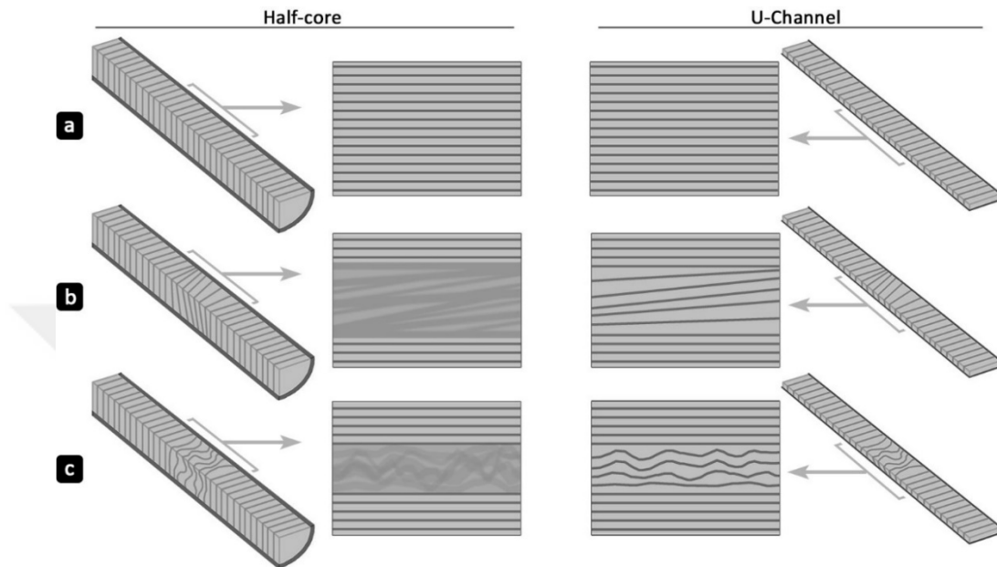
Figure 3.7. Sketches illustrating possible radiographic images taken from half core and u-channel for different types of sediment deformation. a) Undisturbed horizontal lamination. b) Intercalation of inclined laminae. c) Intercalation of undulated soft sediment.
