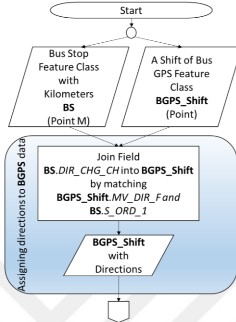
Figure A.6.10 Flowchart of the GIS Preprocessing of Bus Trajectory Data Page 1
