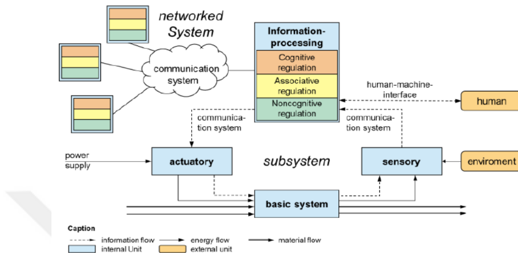
Figure 2.8. Technological concept – from intelligent subsystems to networked, cyber-physical systems
