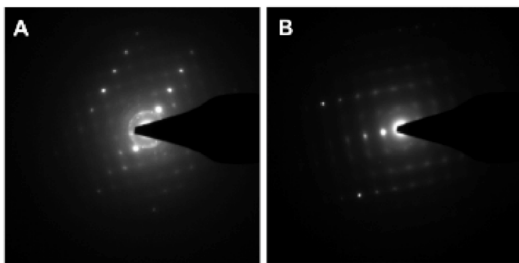
Figure 6.7 – TEM Diffraction patterns of (A) silica synthesis without peptide mediation and (B) with peptide mediation.
