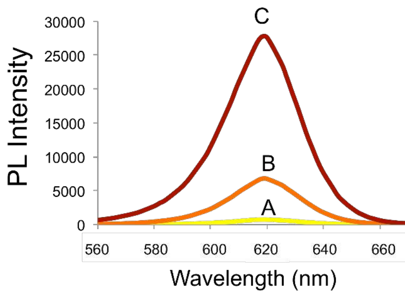
Figure 6.14 – Photoluminescence intensity of three-layered red emitting hybrid nanoassemblies. (A) The first layer of bio-QBP1-SA-Q-Dot, (B) the second layer of bio-QBP1-SA-Q-Dot, and finally in (C) the third layer of bio-QBP1-SA-Q-Dot.
