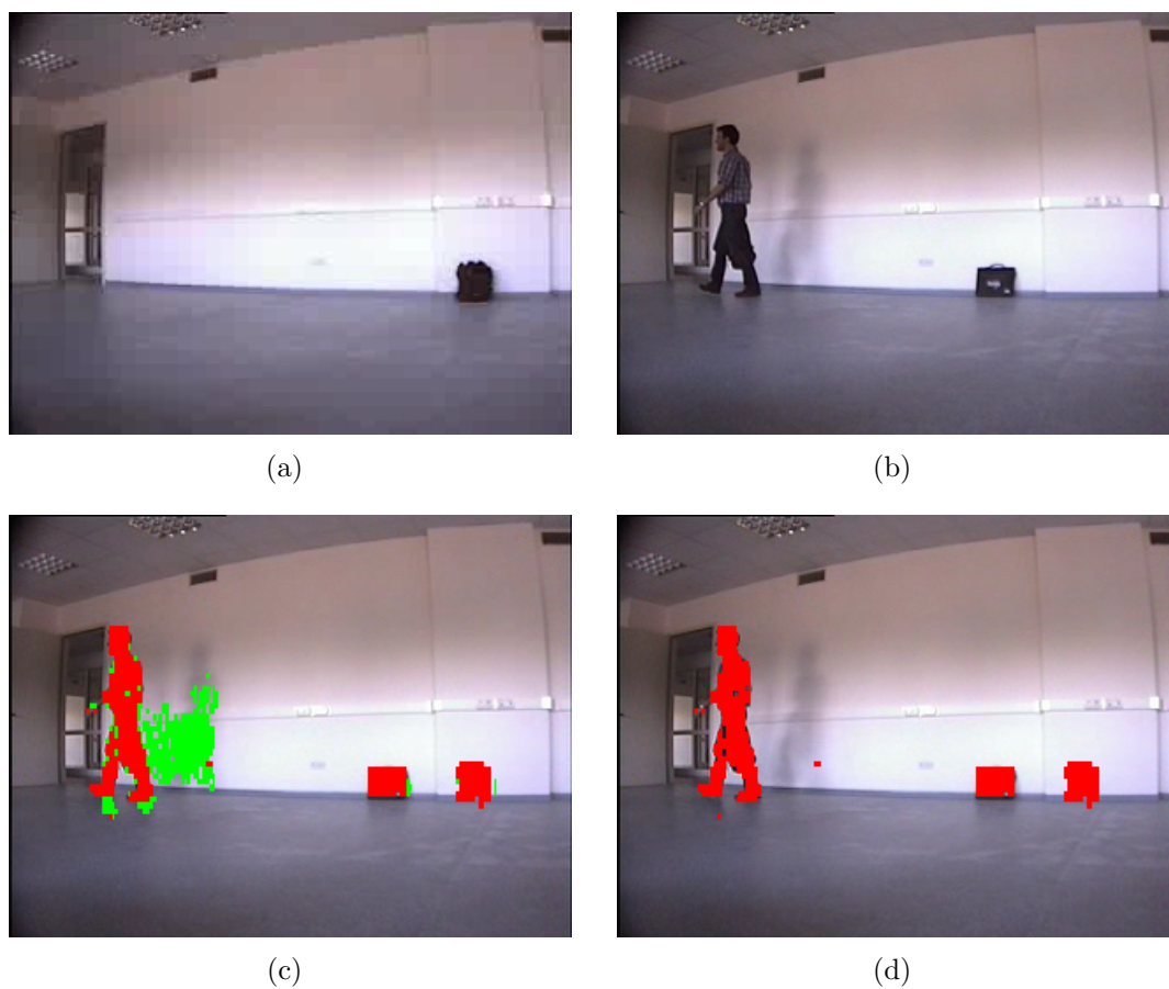
Figure 3.7: Shadow removal sample. (a) Estimated background (b) Current image (c) Detected foreground pixels (shown as red) and shadow pixels (shown as green) (d) Foreground pixels after shadow pixels are removed
