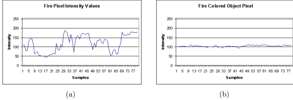
Figure 5.3: Temporal variance of the intensity of fire colored pixels. (a) A pixel in true fire region (b) A pixel of a fire colored object
