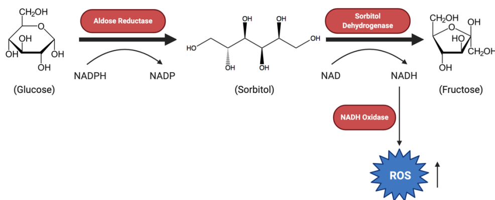
Figure 5. Polyol pathway
