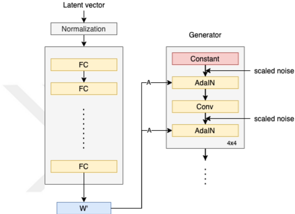
Figure 1.7: StyleGAN generator architecture [49]
