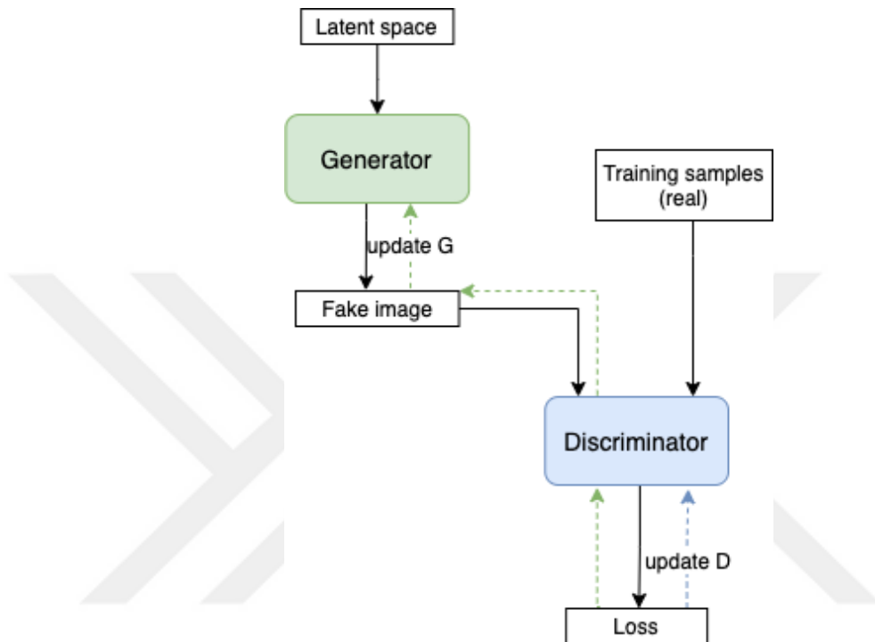
Figure 1.2: Overview of generative adversarial network training
