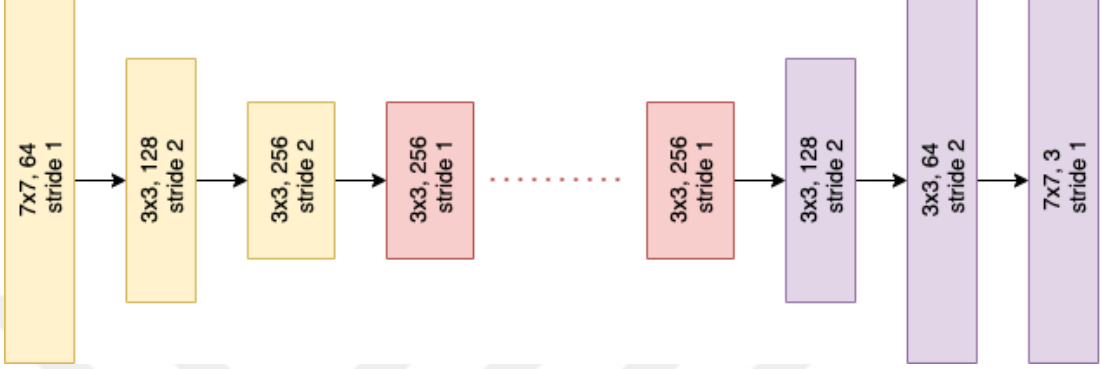
Figure 1.6: CycleGAN generator architecture [51]
