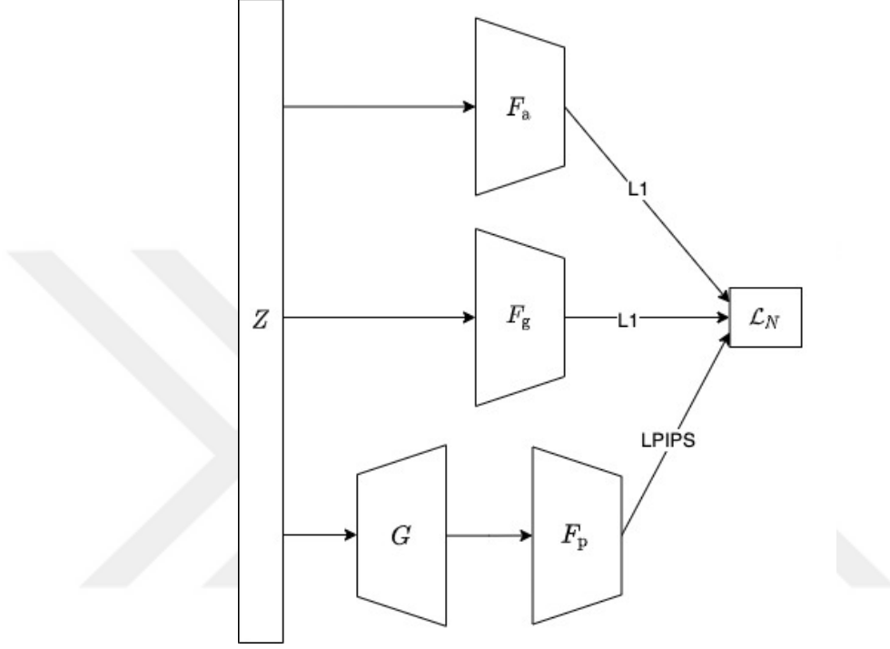
Figure 2.10: Sample-specific latent representation optimization using age and gender feedback in latent space
