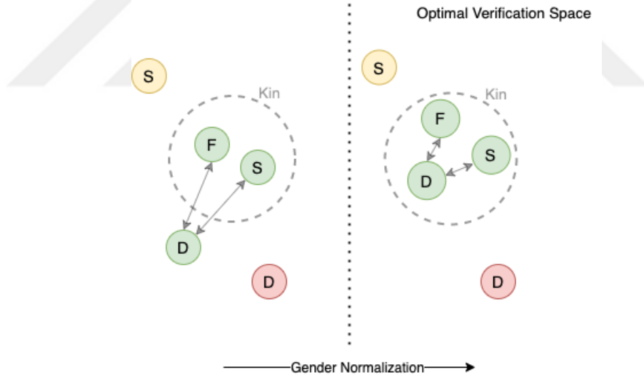
Figure 1.9: Gender normalized latent space in kinship verification
