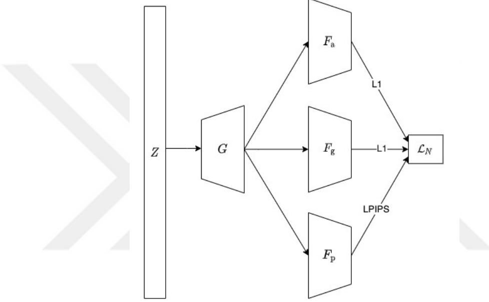
Figure 2.9: Sample-specific latent representation optimization using age and gender feedback in image space
