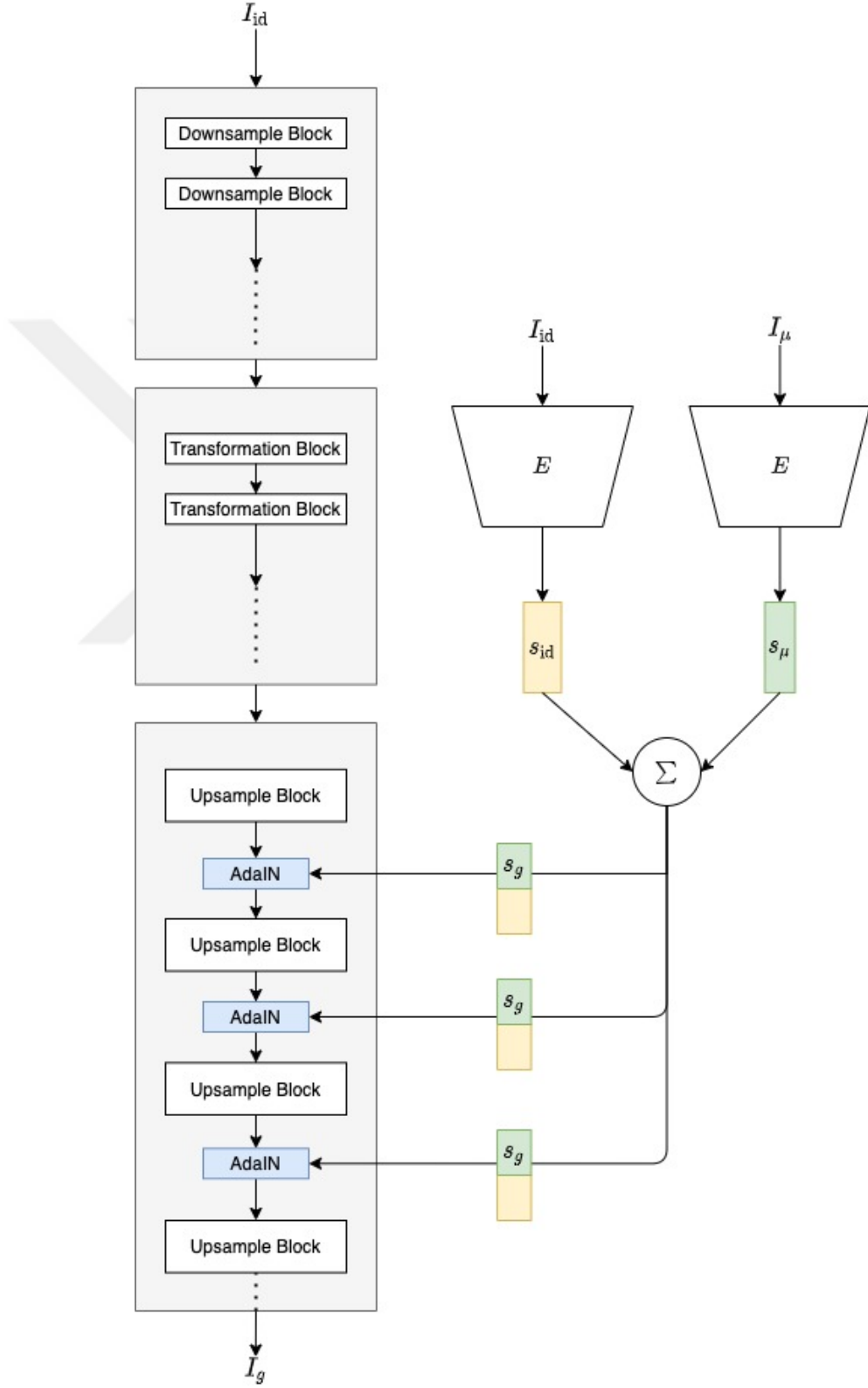
Figure 2.7: Identity-preserved gender normalization by neutral gender style enforcement
