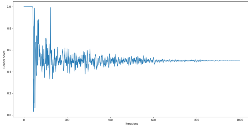
Figure 3.2: Gender score inferred by F_g during the gender normalization process for an example subject
