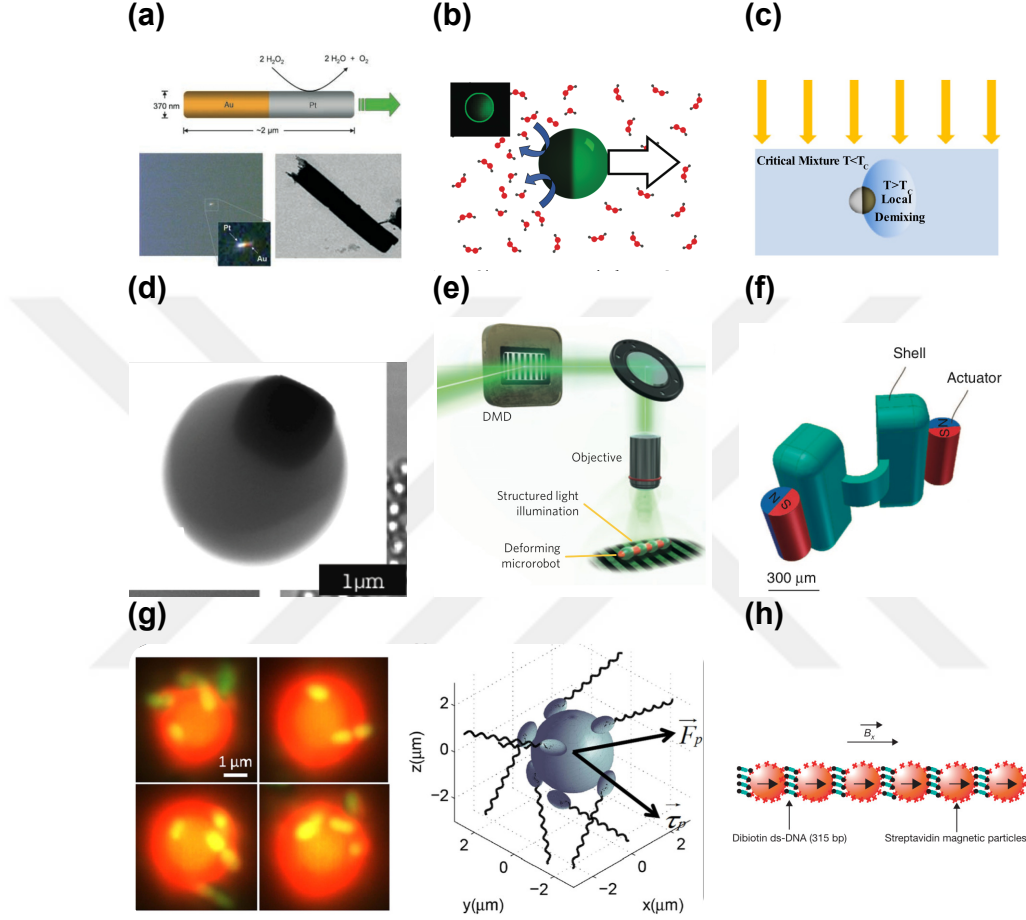
Figure 1.3: Examples to artificially realized microswimmers. (a) Pt and Au coated rod-shaped microswimmers which are activated when exposed to hydrogen peroxide solution due to decomposition of \text{H}_2\text{O}_2 at Pt interface. Reprint from [39]. (b) Pt capped spherical Janus particle that undergoes self-diffusiophoresis due to the concentration gradient around the particle surface. Reprint from [41]. (c) Schematic of the self-propulsion mechanism of gold capped spherical Janus particle which performs a self-phoretic motion due to the local demixing of the critical mixture by the incident light. Reprint from [43]. (d) A Scanning electron microscopy image of polymeric spherical particles enclosing hematite cubes. Reprint from [45]. (e) Activation of deformable cylindrical soft-microrobot. Reprint from [48]. (f) A cartoon of 3D printed PDMS based micro-scallops. Reprint from [49]. (g) Florescent image of E.coli based microswimmers. Spherical PS bead is highlighted in red whereas attached bacterial cells are highlighted in yellow. Reprint from [51]. (h) Schematic of DNA-linked superparamagnetic colloids as an artificial magnetic "flagellum". Reprint from [52].
