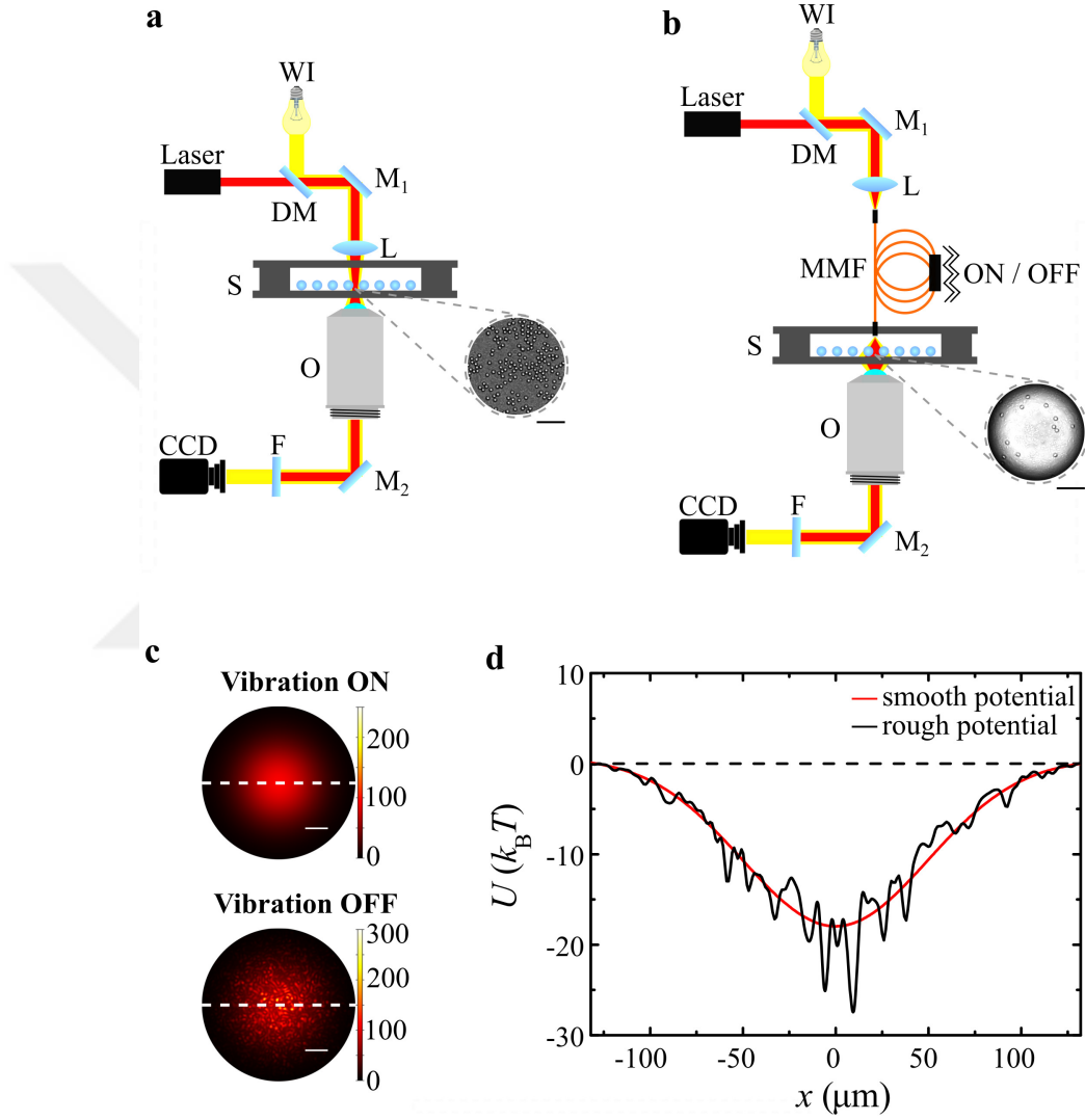
Figure 2.6: Schematics of the setup. Optical setups to generate (a) smooth Gaussian optical potentials and (b) optical potentials with a controllable degree of disorder: WI, white light lamp; DM, dichroic mirror; M_1 and M_2 , mirrors; L, lens; S, sample; O, objective; F, filter; CCD, CCD camera; MMF, multimode optical fiber. (c) The fiber in b is attached to a mechanical oscillator whose vibration frequency can be modulated to change the roughness of the optical potential. (d) The profiles of the optical potentials along the white dashed lines in c both for smooth Gaussian illumination (red line) and disordered illumination (black line). All scale bars correspond to 40 \mu m . Reprint from [104].
