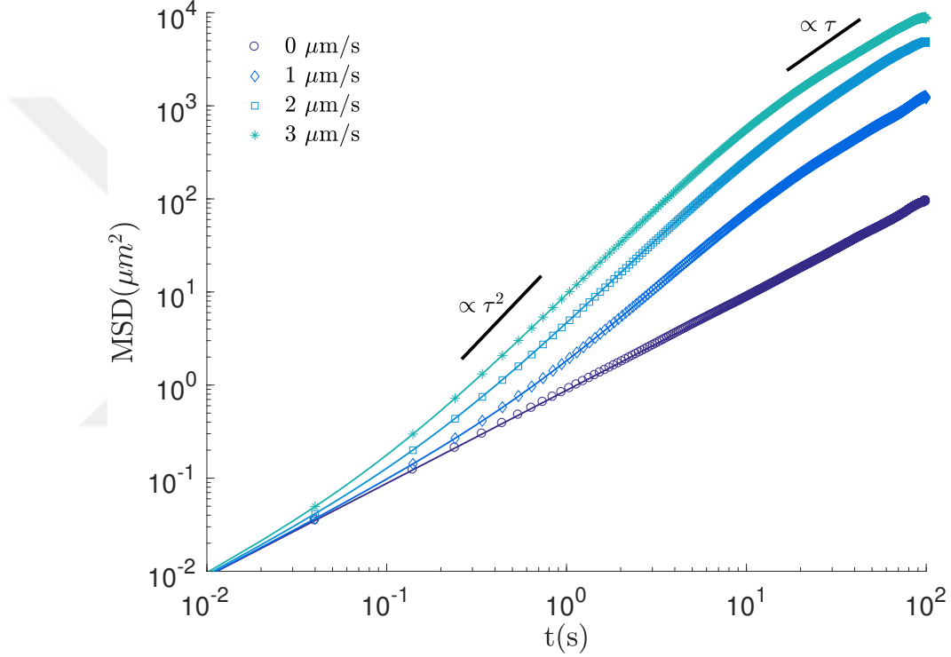
Figure 1.6: The enhanced diffusion and mean square displacement(MSD) of active Brownian particles. The lines show theoretical MSD functions whereas symbols show the MSD values of numerically simulated particles (see eq.(1.22)) with velocities v = 0 \text{ } \mu\text{m s}^{-1} (circles), v = 1 \text{ } \mu\text{m s}^{-1} (diamonds), v = 2 \text{ } \mu\text{m s}^{-1} (squares) and v = 3 \text{ } \mu\text{m s}^{-1} (stars). In the Brownian case ( v = 0 ), the particle is in free diffusion regime ( \text{MSD}(t) \propto t ) whereas in the active Brownian case, particle is in diffusive regime at shorter time scales ( \text{MSD}(t) \propto t where t \ll \tau_R ) renders to superdiffusive regime (i.e. \text{MSD}(t) \propto t^2 for t \approx \tau_R ) and then relaxes back to free diffusion ( \text{MSD}(t) \propto t where t \gg \tau_R ) with an enhanced diffusion coefficient. Reproduced from [4].
