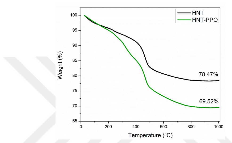
Figure 30. TGA curves for HNT and HNT-PPO under nitrogen atmosphere
