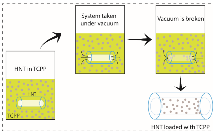
Scheme 1. FR loading of HNTs via vacuum cyclization
