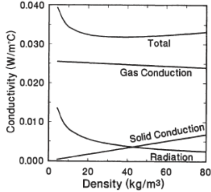
Figure 13. Theoretical change in thermal conductivity for air-filled foam over a range of densities at T=20^{\circ}\text{C} [8]
