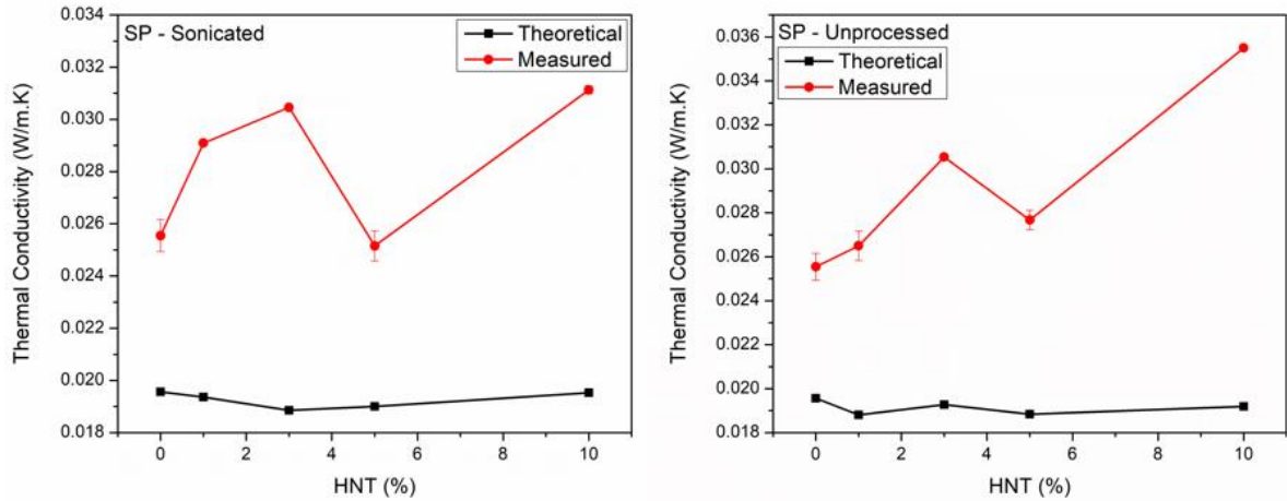
Figure 21. Theoretical and measured thermal conductivity values for SP foams
