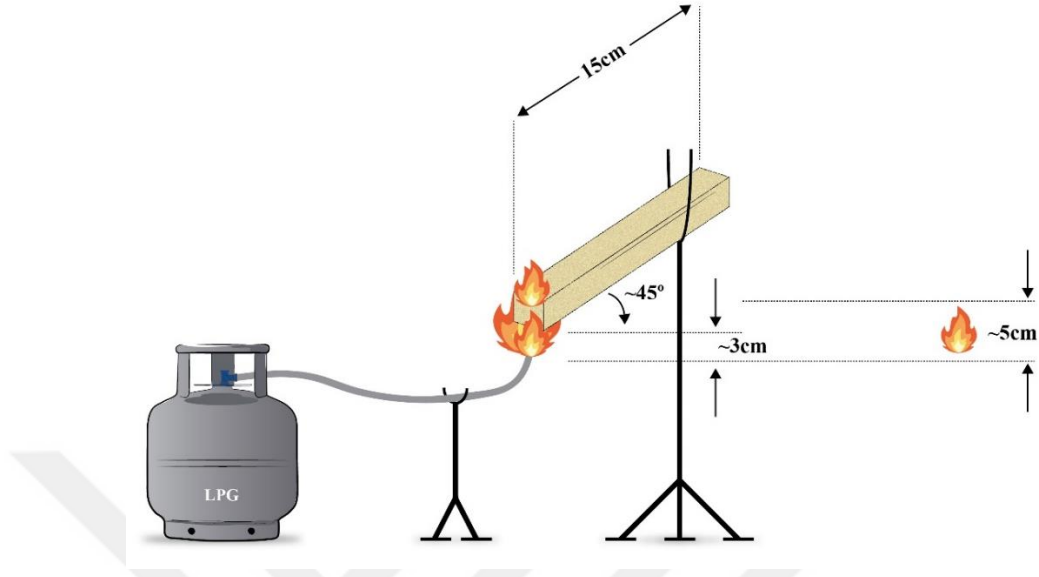
Figure 8. Diagram showing the setup prepared by us
