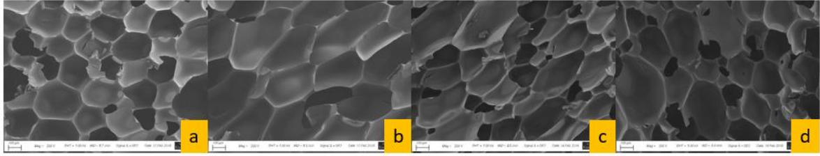
Figure 22. SEM images of B3 foams with HNT-S: (a) reference, (b) 1%, (c) 5%, (d) 10%
