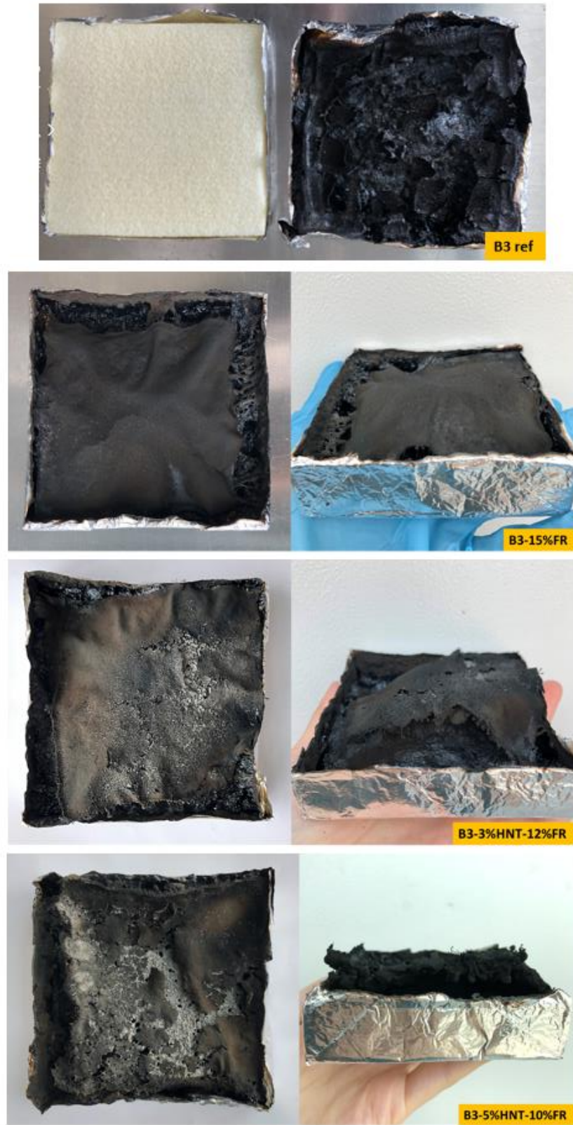
Figure 42. Appearance of some samples after testing with cone calorimeter
