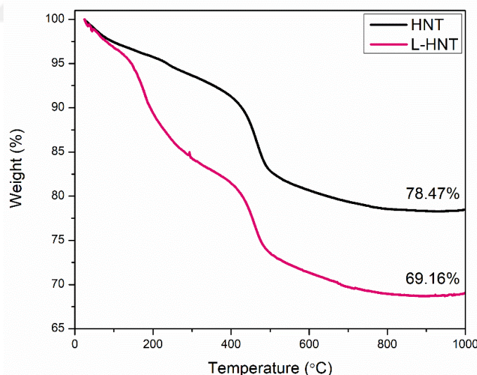
Figure 26. TGA curves for HNT and L-HNT under nitrogen atmosphere
