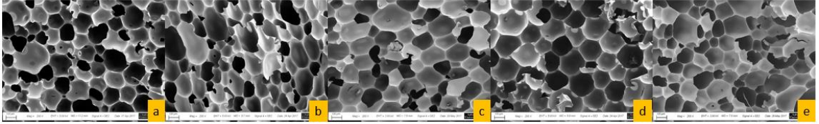
Figure 17. SEM images of DEC foams with sonicated HNT: (a) reference, (b) 1%, (c) 3%, (d) 5%, (e) 10%
