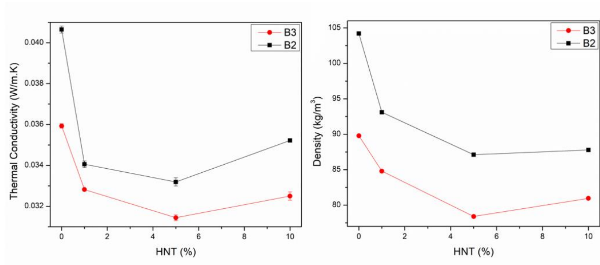
Figure 24. Thermal conductivity and density measurements for B3 and B2 foams
