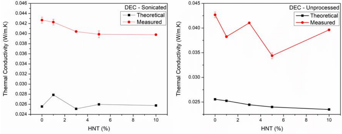
Figure 18. Theoretical and measured thermal conductivity values for DEC foams
