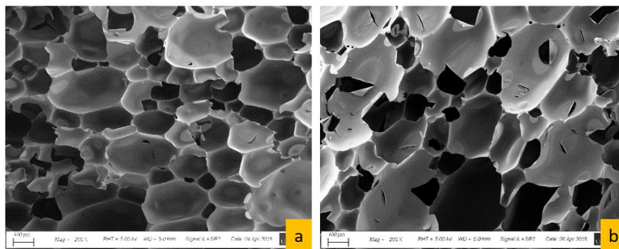
Figure 25. SEM images of B3 and B2 foams with 10% sonicated HNT
