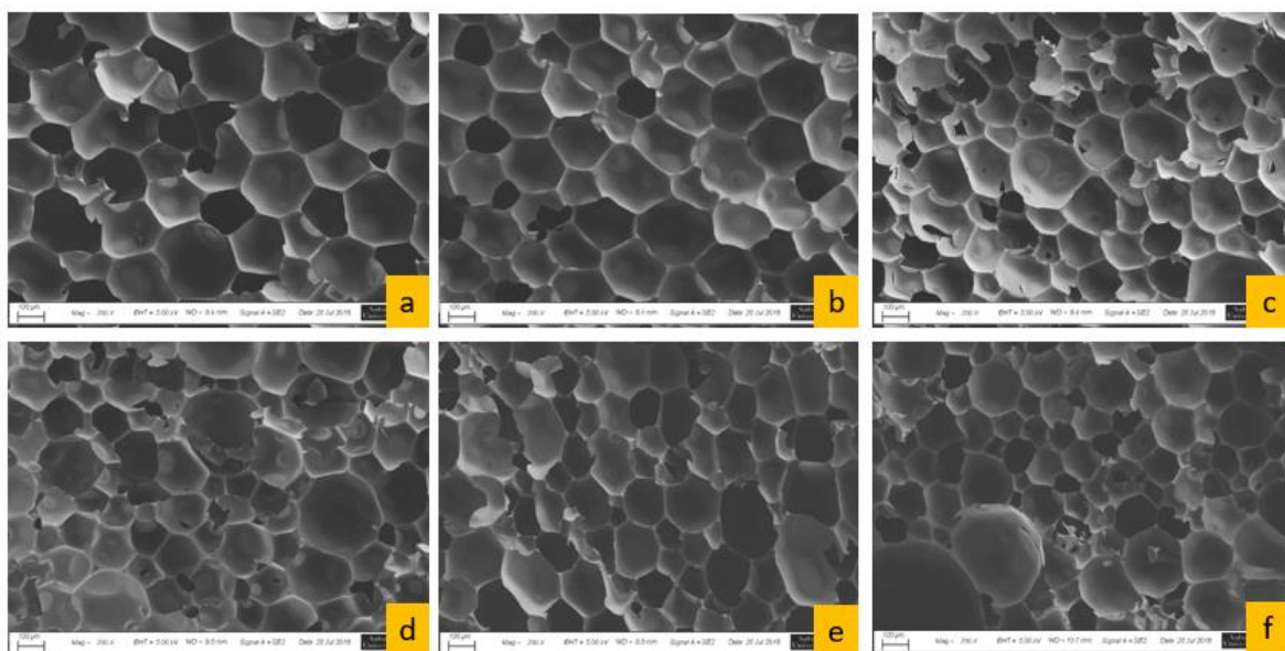
Figure 27. SEM images of B3 foams added with L-HNTs (a) reference (b) 1% (c) 3% (d) 5% (e) 7% (f) 10%
