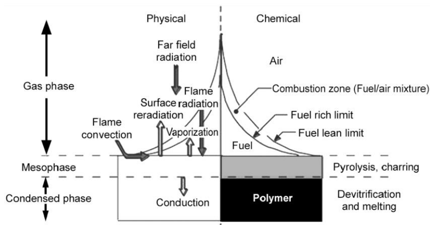
Figure 34. Physical and chemical processes taking place during combustion of polymers [117]
