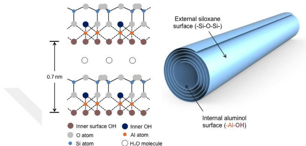
Figure 2. Halloysite nanotube [21]
