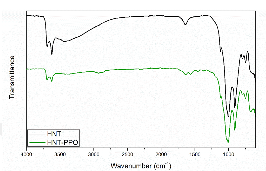
Figure 29. FT-IR spectra of reference HNT and HNT-PPO
