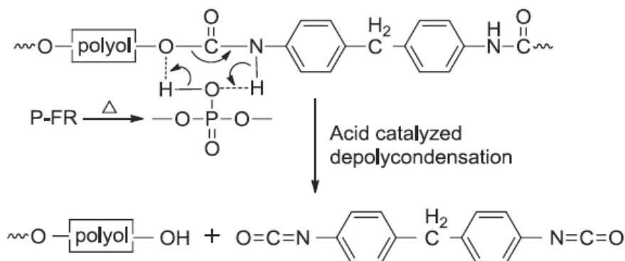
Figure 37. Acid catalysis effect of P-FR on urethane bond degradation [127]
