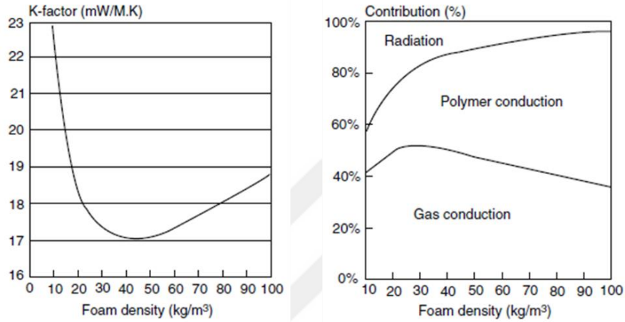
Figure 12. The change in thermal conductivity and percent contributions with density [3]
