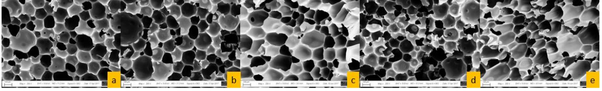
Figure 16. SEM images of DEC foams with unprocessed HNT: (a) reference, (b) 1%, (c) 3%, (d) 5%, (e) 10%
