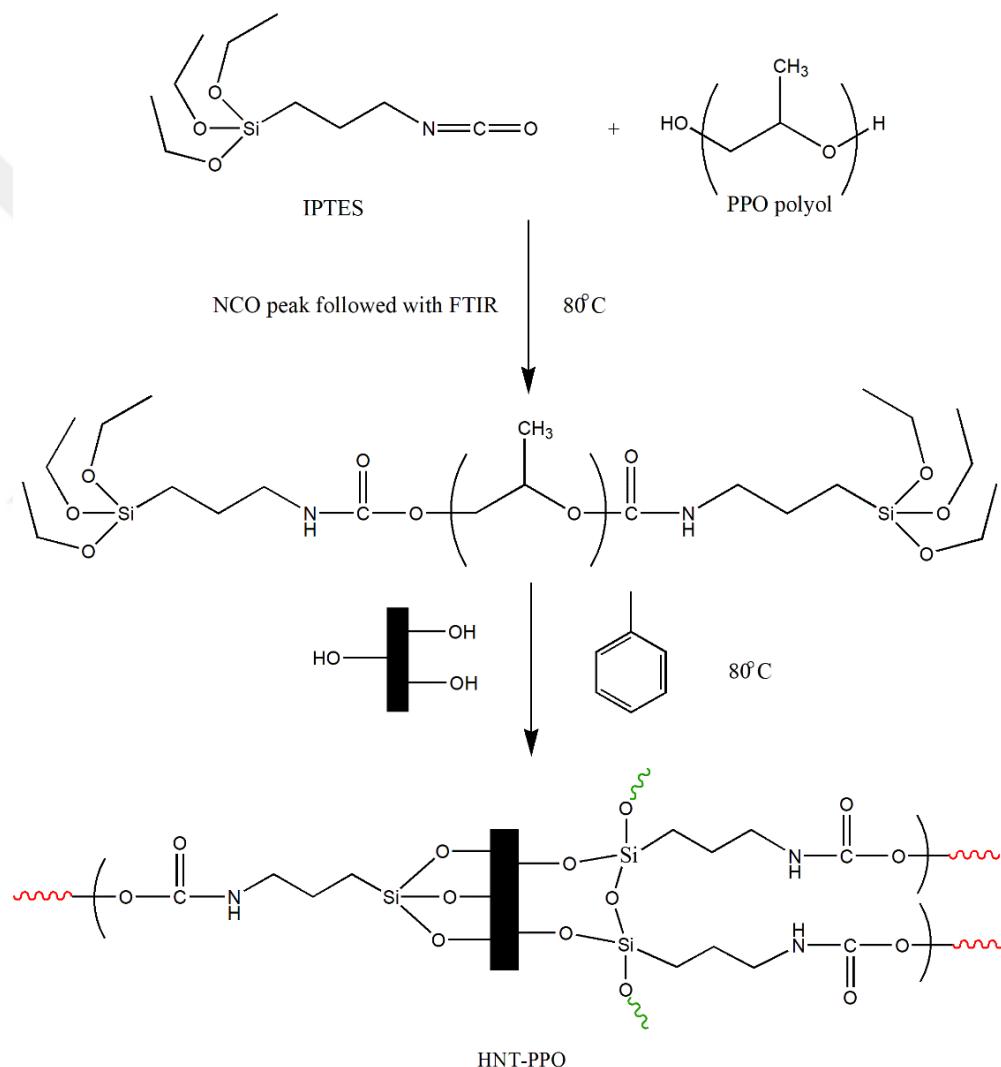
Scheme 2. Surface functionalization of HNTs with PPO using IPTES as coupling agent
