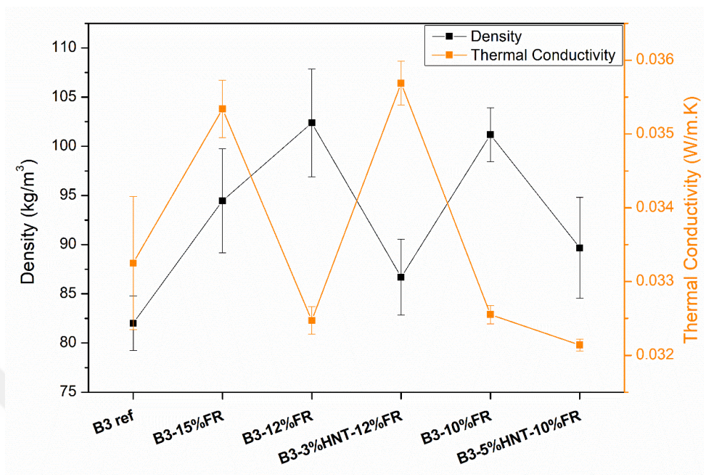
Figure 33. Density and thermal conductivity of samples containing HNT-PPO and FR
