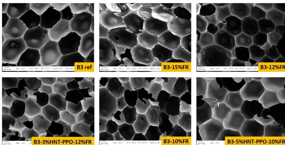
Figure 31. SEM images of B3 foams with HNT-PPO and FR
