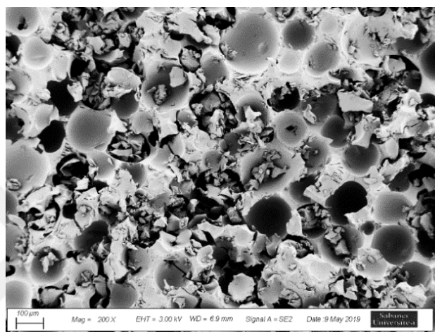
Figure 15. SEM image of foam resin after curing after unsuccessful evaporation of the blowing agent
