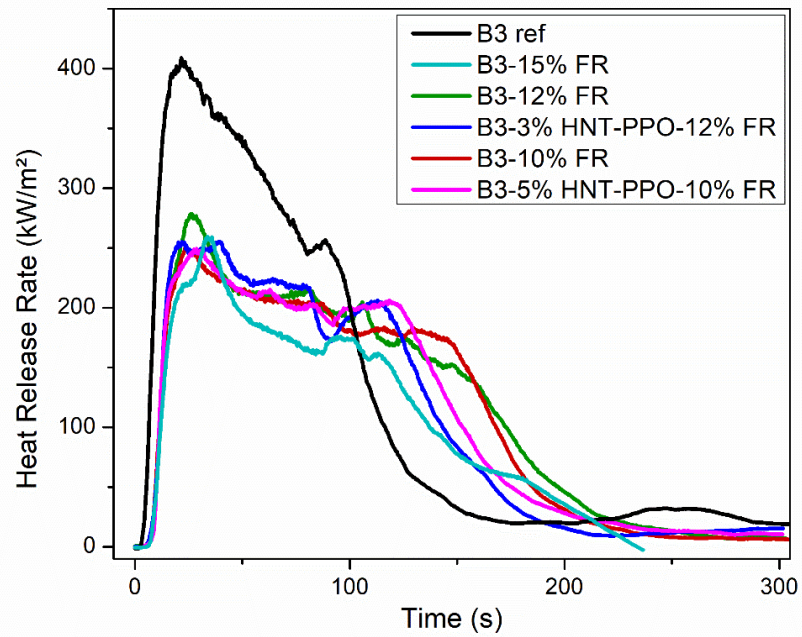
Figure 41. Heat release rate profiles of the samples
