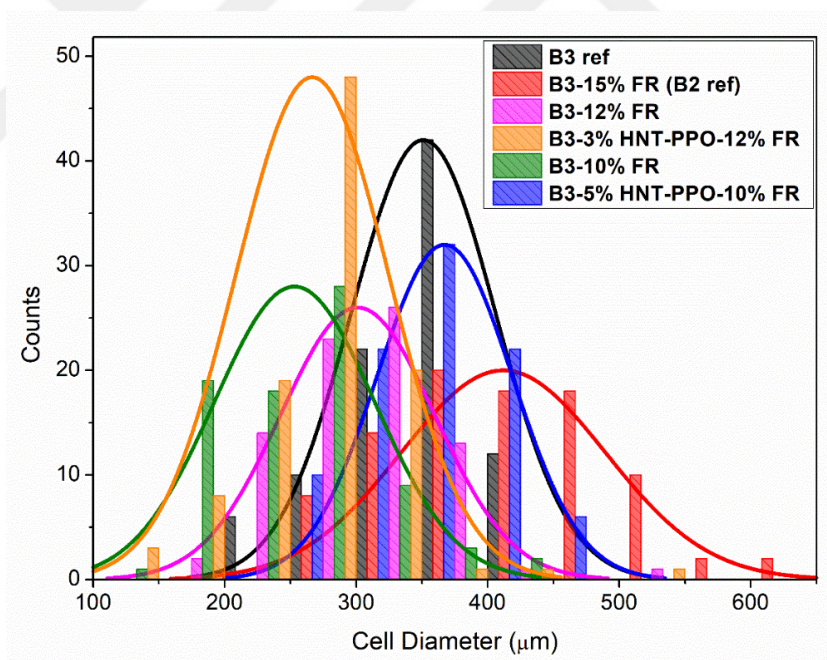
Figure 32. Cell size distribution of B3 foams prepared with HNT-PPO and FR
