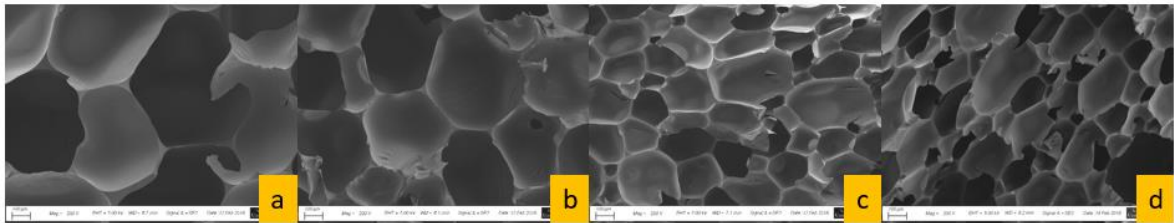
Figure 23. SEM images of B2 foams with HNT-S: (a) reference, (b) 1%, (c) 5%, (d) 10%
