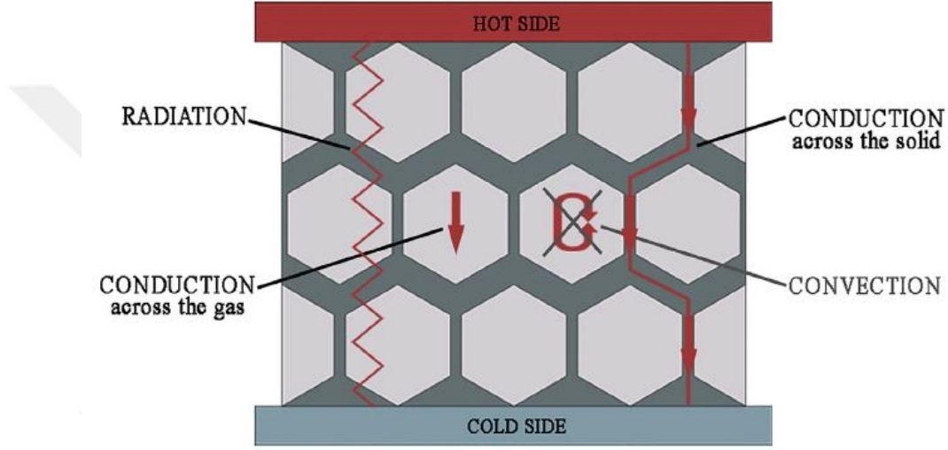
Figure 11. Heat transfer mechanisms in closed-cell polyurethane foams [92]
