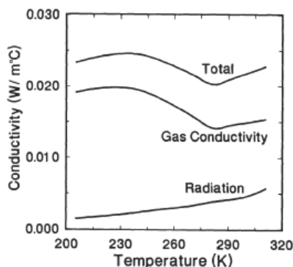
Figure 14. Thermal conductivity versus temperature for foam filled with CFC-11-air mixture at 0.6 atm [8]
