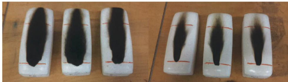
Figure 40. 10% HNT loaded B3 and B2 foam samples after small flame test
