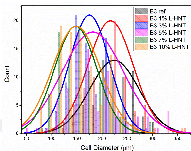
Figure 28. Cell size distribution of B3 foams prepared with L-HNTs
