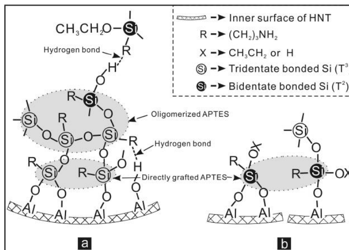
Figure 4. Formation of the crosslinked silane network [62]
