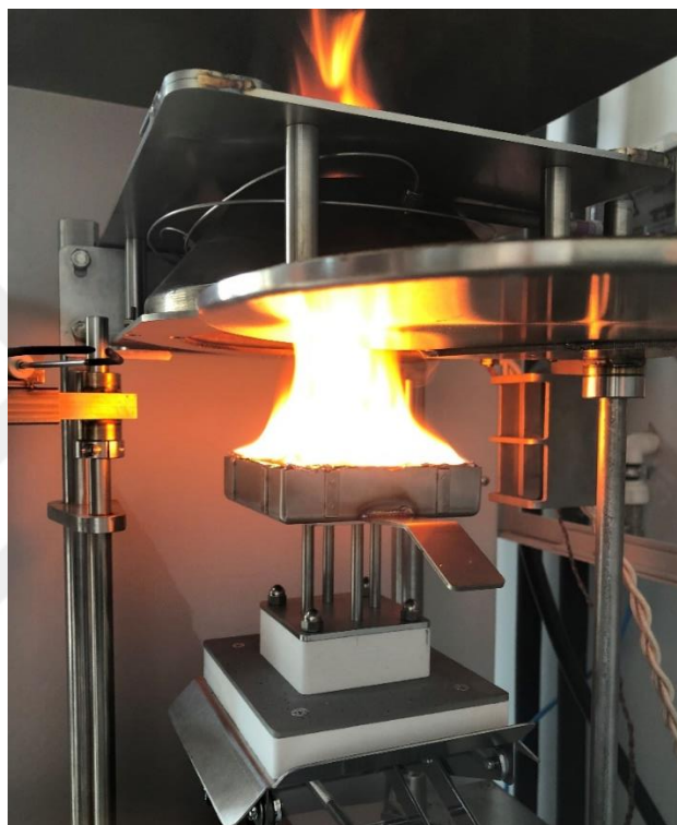
Figure 10. A foam sample being tested with a cone calorimeter
