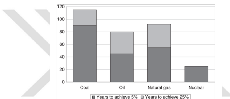
Figure 2.1 Major transitional shifts in global energy supply, 1750–2015
