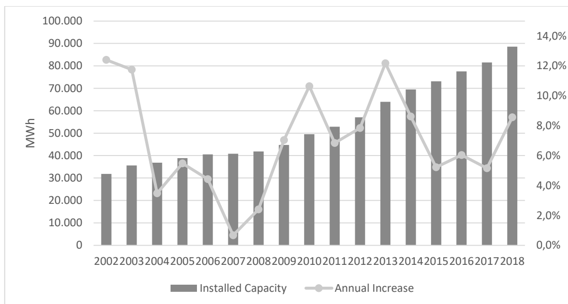
Figure 4.2 Installed Capacity
