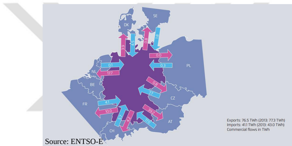
Figure 5.11 Commercial Electricity Exchange between Germany and It's Neighbors (2014)
