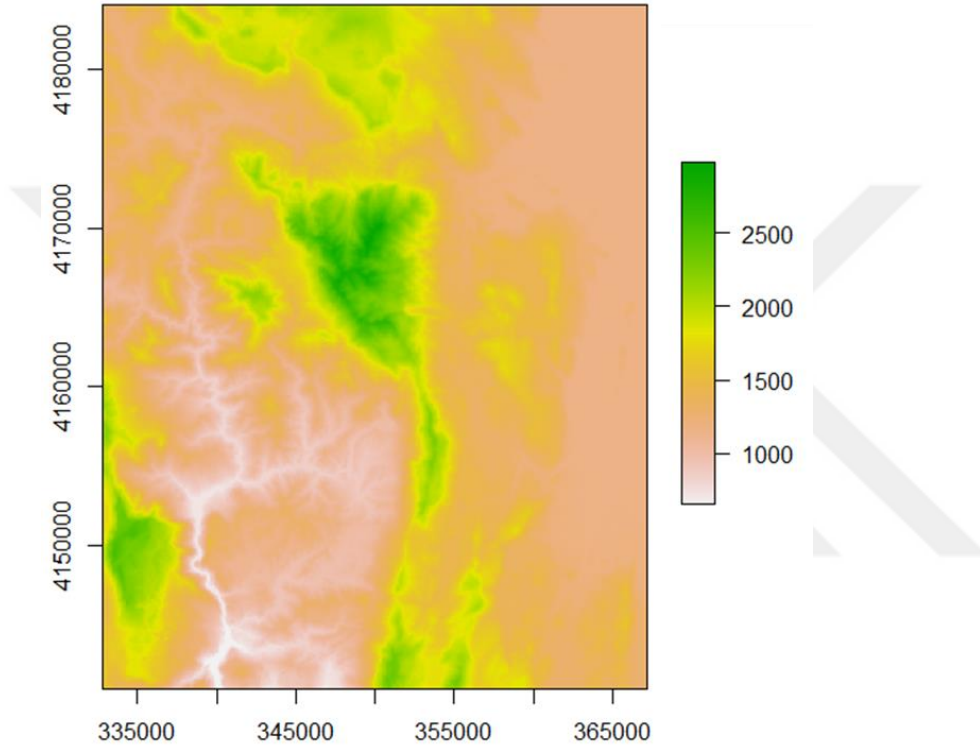
Figure 3.5. Digital elevation model of the Dedegöl Mountain study area
