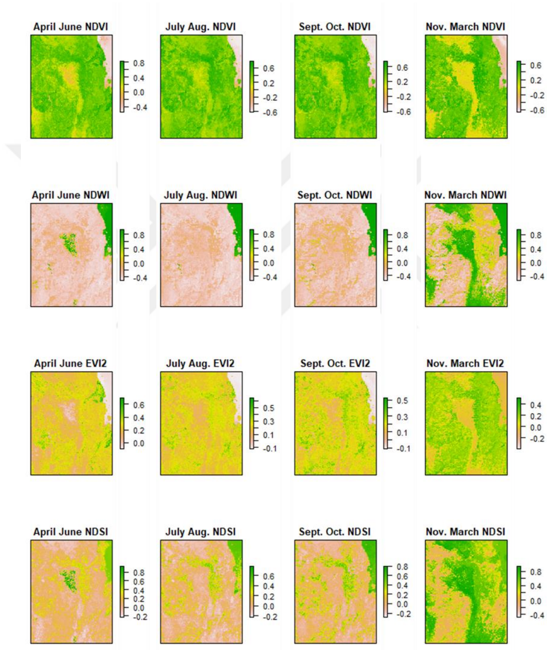
Figure 5.5. Seasonal indices calculated for 2018, Dedegöl Mountain
