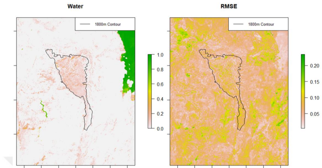
Figure 5.14. Results of unmixing for the endmembers, and the RSME
