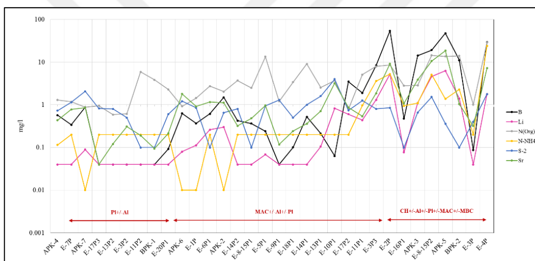
Figure 4.24. B, Li, N (org), N-NH 4 , S -2 and Sr concentrations in well waters.
