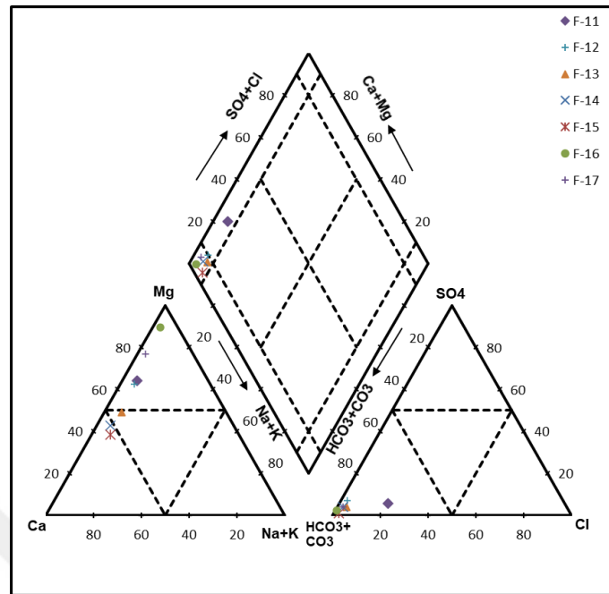
Figure 4.6. Major ion water facies of spring and fountain waters.
