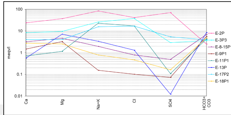
Figure 4.19. The distribution of the major ion concentrations in Pl + MAC well waters.
