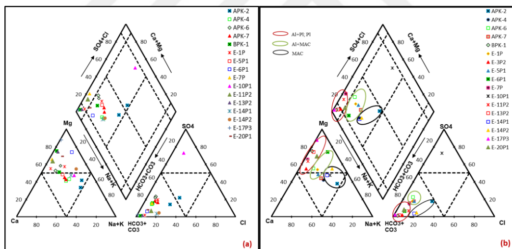
Figure 4.16. Water facies in Al, Al+Pl, Al+MAC, Pl and MAC well waters. (a) all data and (b) average data.
