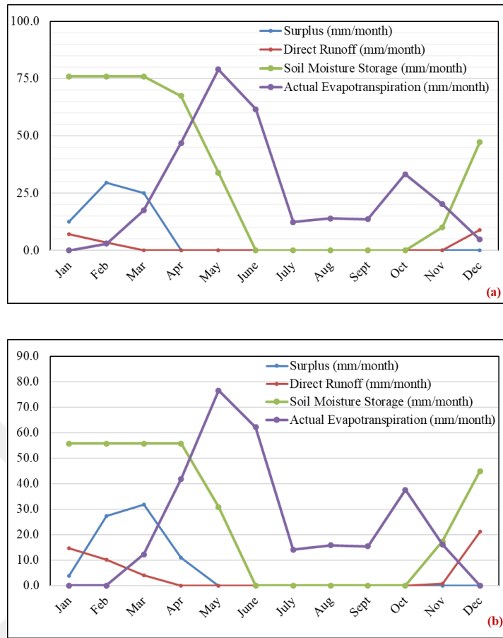
Figure 3.2. Distribution of water budget components for (a) the plain and (b) the mountain areas.
