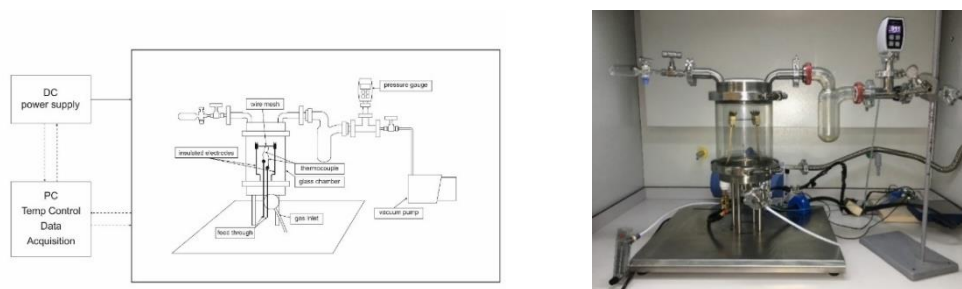
Figure 3.6. Wire mesh reactor at the Clean Combustion Technologies Laboratory of the Middle East Technical University, Turkey. Left-hand side: Schematic representation; right-hand side: Photograph [238].
