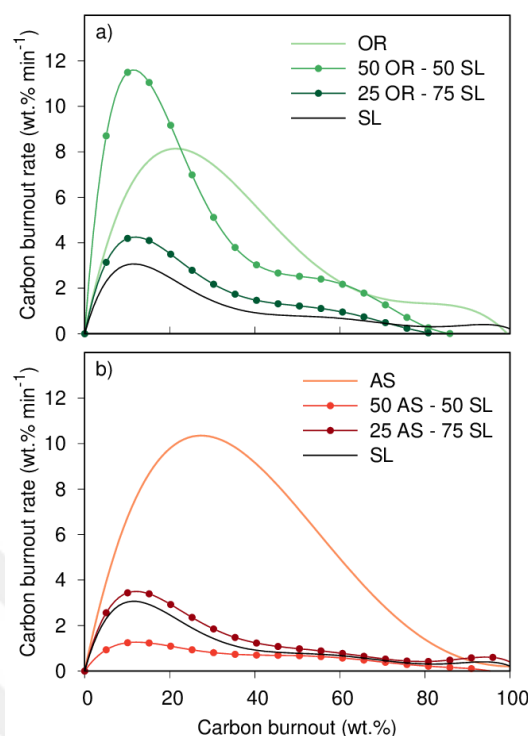
Figure 4.31. Carbon burnout rate vs. burnout for all fuels and respective blends (experimental values). Olive residue (OR) and almond shell (AS) chars were oxidized at 400 °C and all remaining chars were oxidized at 450 °C.
