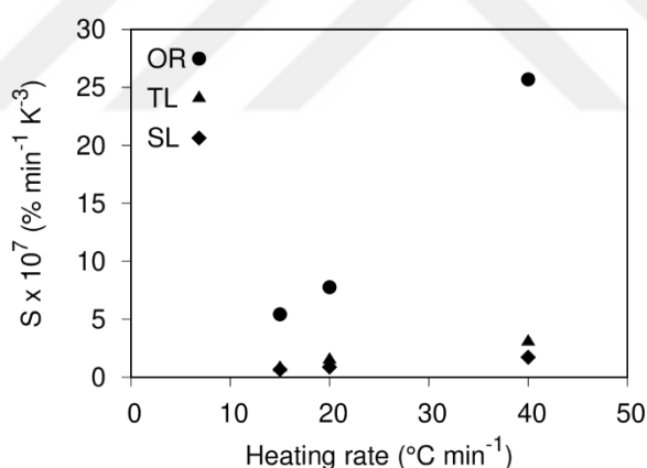
Figure 4.9. Combustibility index – S as a function of the heating rate for all three fuels (OR, TL, and SL) during the major stage of combustion (stage B).
