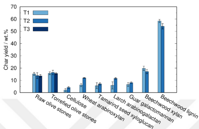
Figure 4.33. Char yields of all commercial samples (T1 and T2), and raw and torrefied olive stones (T1, T2, and T3). Conditions: T1 - 800 °C, 400 °C/s; T2 - 1000 °C, 800 °C/s; and T3 - 1150 °C, 1150 °C/s.
