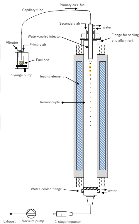
Figure 3.9. Schematic representation of the drop tube furnace at the Clean Combustion Technologies Laboratory of the Middle East Technical University, Turkey, fitted with feeding and collection for total collection. The illustration of a single particle combustion event is not to scale.
