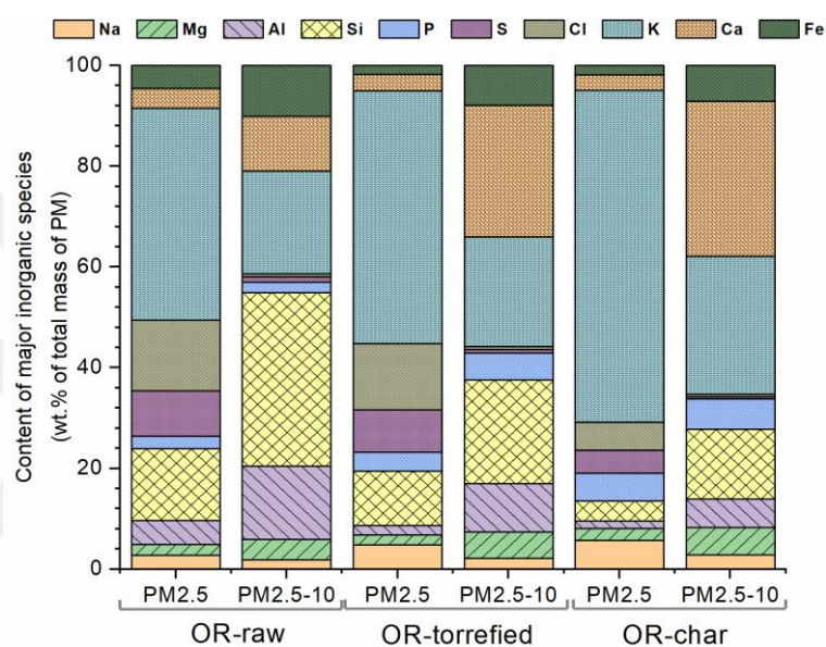
Figure 4.22. Energy dispersive spectroscopy results of concentration of major inorganic species present in PM 2.5 and PM 2.5-10 for raw olive residue, torrefied olive residue, and olive residue char.
