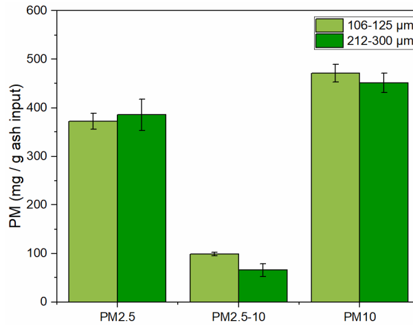
Figure 4.18. PM concentration (mg / g ash input) from the combustion of 106-125 and 212-300 \mu\text{m} size olive residue at 1000 °C in the drop tube furnace. Vertical bars represent 98 % confidence statistical error.
