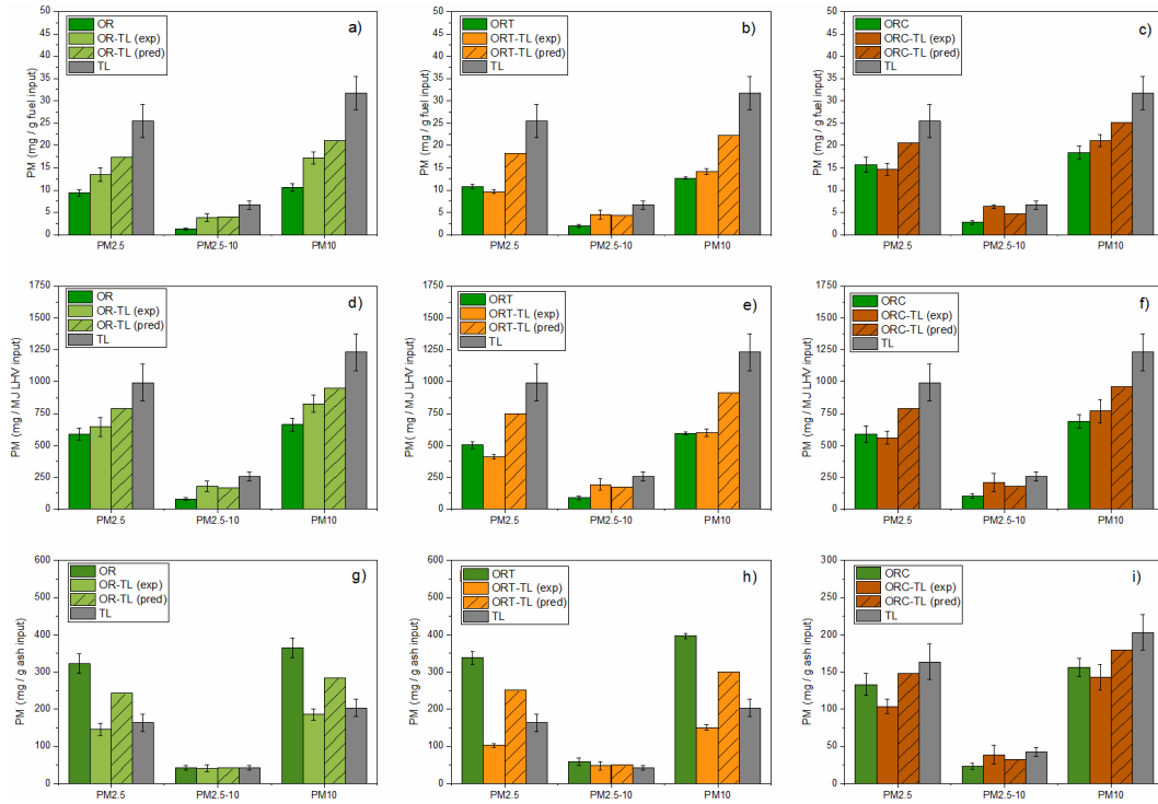
Figure 4.23. PM concentration from combustion of 50:50 blends of 212-300 \mu\text{m} size raw olive residue, torrefied olive residue, and olive residue char with 106-125 \mu\text{m} Tunçbilek lignite at 1200 °C in the drop tube furnace. Vertical bars represent 98 % confidence statistical error. a-c) fuel input basis, d-f) useful energy input basis, g-i) ash input basis.
