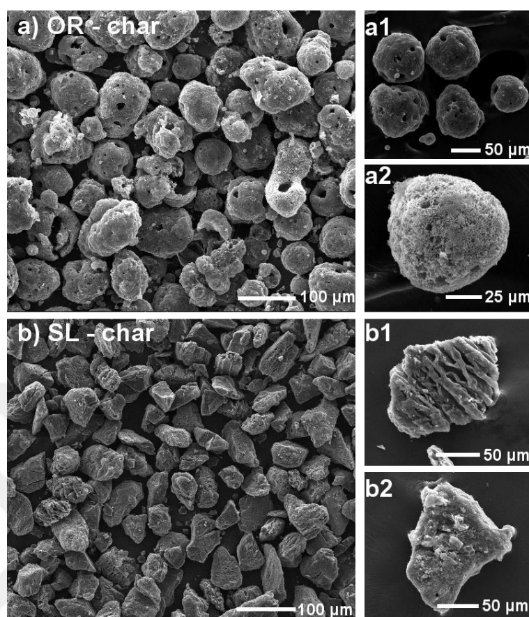
Figure 4.45. Scanning electron microscopy micrographs of chars from (a) olive residue and (b) Soma lignite obtained from fast pyrolysis in the drop tube furnace.
