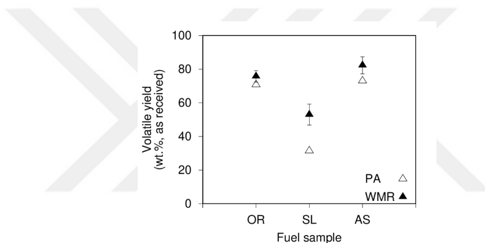
Figure 4.26. Volatile yield of individual fuel samples. PA – proximate analysis, WMR – wire mesh reactor. Vertical bars represent 98% confidence statistical error.
