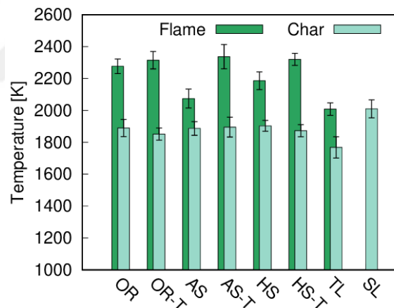
Figure 4.13. Flame (dark green bars) and char (light green bars) temperatures from pyrometry measurements for all studied fuels. Vertical bars represent 98% confidence statistical errors.
