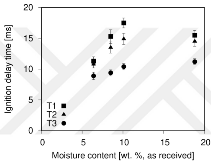
Figure 4.7. Ignition delay time for all solid fuels as a function of moisture content for operating conditions T1-T3. Vertical bars represent 98% confidence statistical error.
