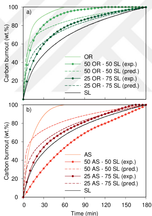
Figure 4.30. Carbon burnout profiles of the blended char samples (experimental and predicted values). a) OR – SL blends; b) AS – SL blends. Individual profiles of SL, OR, and AS are represented for comparison purposes. Olive residue (OR) and almond shell (AS) chars were oxidized at 400 °C and all remaining chars were oxidized at 450 °C.
