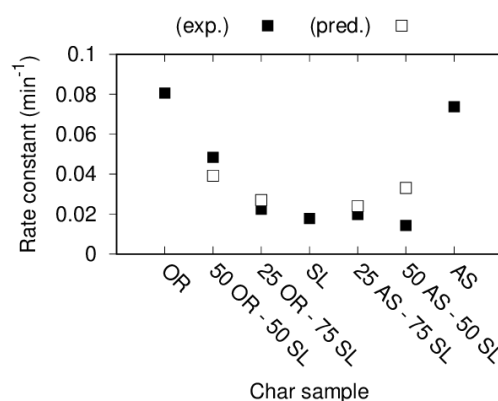
Figure 4.32. First order rate constants of individual chars and corresponding blends (experimental – filled symbols, and predicted – open symbols).
