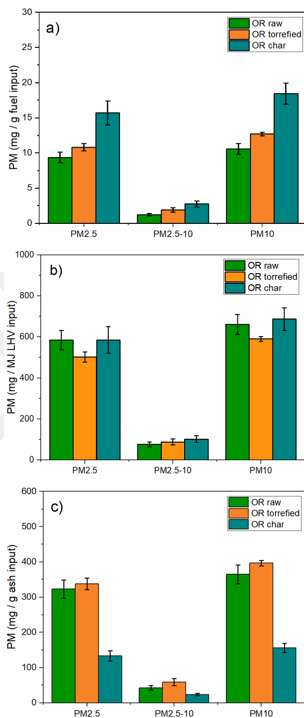
Figure 4.20. PM concentration from combustion of 212-300 \mu\text{m} size raw olive residue, torrefied olive residue, and olive residue char at 1200 ^{\circ}\text{C} in the drop tube furnace. Vertical bars represent 98 % confidence statistical error. a) fuel input basis, b) useful energy (LHV) input basis, c) ash input basis.
