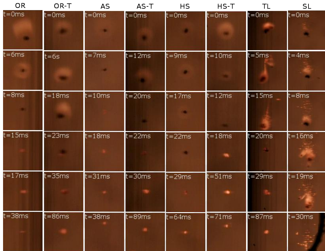
Figure 4.11. High-speed cinematography stills of typical combustion events of single particles of all studied fuels. For sizing purposes the diameter of the wire shown in the last frame of the SL sequence is 240 \mu\text{m} .
