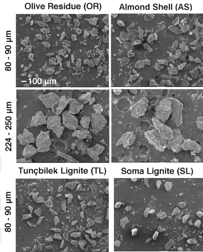
Figure 3.2. Scanning Electron Microscopy images for all fuels used in the ignition study (subsection 4.1). The scale bar represented applies to all images.
