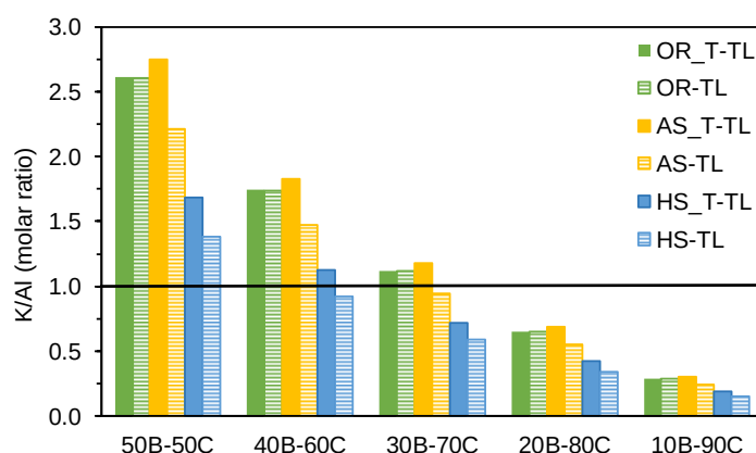
Figure 4.17. K/Al molar ratios for each blend of biomass (B) and Tunçbilek lignite (C). The horizontal line demarks the threshold above which synergistic effects may be observed for biomass-coal mixtures.
