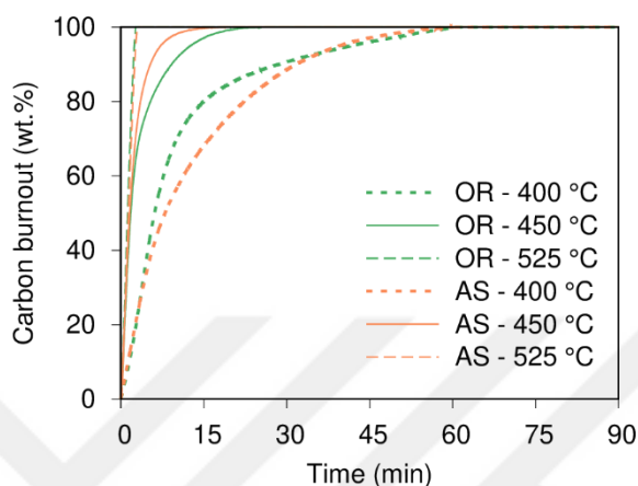
Figure 3.12. Carbon burnout vs time for both biomass fuels (OR – olive residue, and AS – almond shell) for three temperatures (400, 450, and 525 °C).
