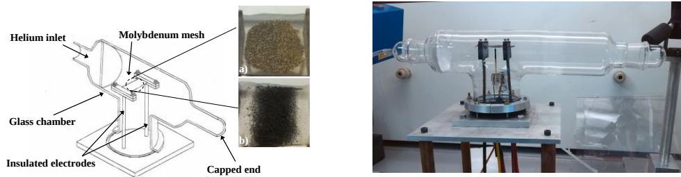
Figure 3.7. Wire mesh reactor at the University of Edinburgh, U.K. Left-hand side: Schematic representation and sample photographs of the bottom mesh, (a) illustration of parent fuel, OR, before pyrolysis, b) illustration of char produced from OR after pyrolysis; right-hand side: Photograph.
