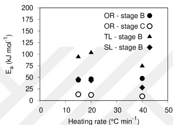
Figure 4.10. Apparent activation energy as a function of the heating rate for all fuels.
