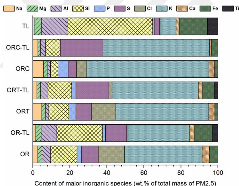
Figure 4.25. Energy dispersive spectroscopy results of concentration of major inorganic species present in PM 2.5 for raw olive residue, torrefied olive residue, olive residue char, Tunçbilek lignite, and respective blends.
