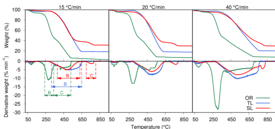
Figure 4.8. TG (top row) and DTG (bottom row) profiles for the studied fuels under: 15 °C/min (left-hand side column); 20 °C/min (center column); and 40 °C/min (right-hand side column), with indication of the weight loss stages for all fuels (excluding moisture release and decomposition) in the 15 °C/min DTG graph.
