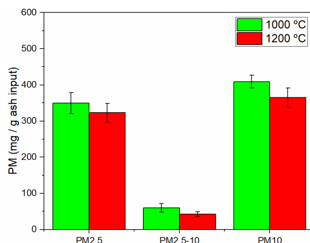
Figure 4.19. PM concentration (mg / g ash input) from combustion of 212-300 \mu\text{m} size olive residue at two distinct temperatures (1000 and 1200 ^{\circ}\text{C} ) in the drop tube furnace. Vertical bars represent 98 % confidence statistical error.
