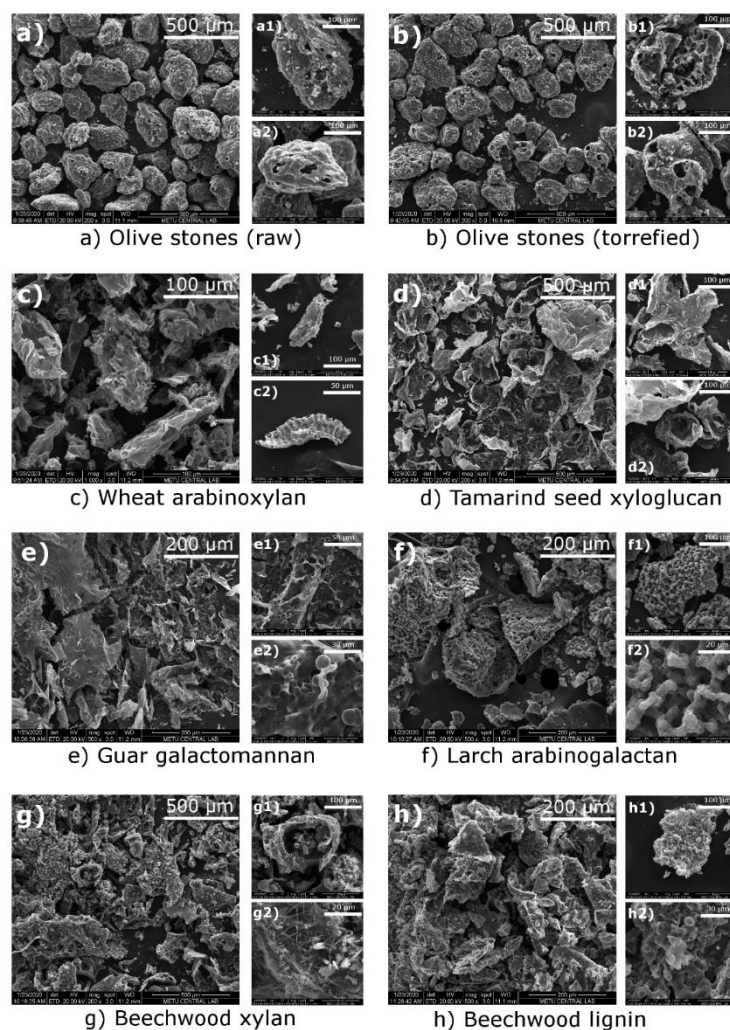
Figure 4.36. Scanning Electron Microscopy images of chars from raw and torrefied olive stones, wheat arabinoxylan, tamarind seed xyloglucan, guar galactomannan, larch arabinogalactan, beechwood xylan, and beechwood lignin.
