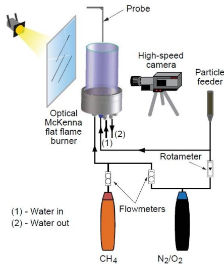
Figure 3.8. Schematic of the entrained flow reactor at IST, University of Lisbon, Portugal.
