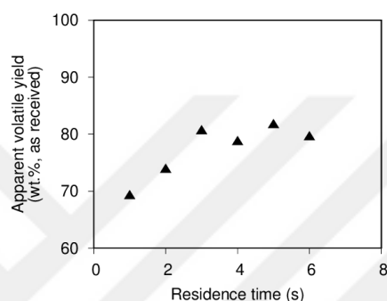
Figure 3.14. Volatile yield as a function of the wire-mesh reactor pyrolysis residence time for almond shell.
