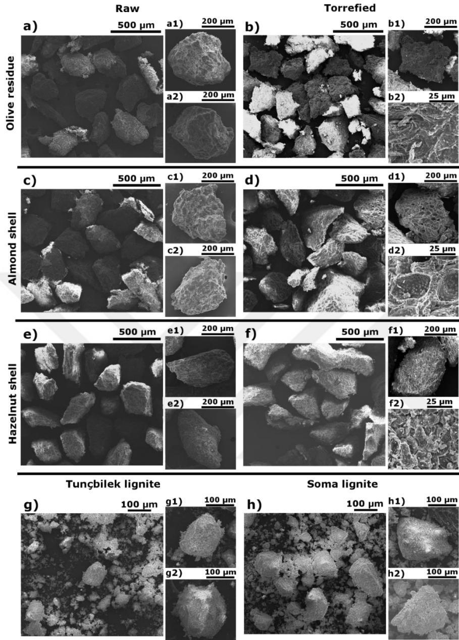
Figure 3.3. Scanning Electron Microscopy images for all fuels used in the combustion study (subsection 4.2). Biomass fuels (raw and torrefied) are in the size range of 212-300 \mu\text{m} , lignites are in the size range of 106-125 \mu\text{m} .
