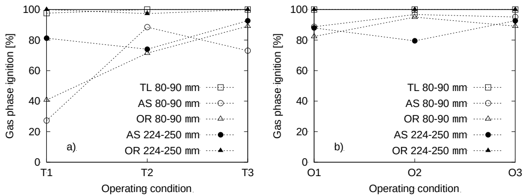
Figure 4.4. Percentage of gas-phase ignition for all solid fuels, except Soma lignite, during the EFR experiments. a) Conditions T1-T3; b) conditions O1-O3.
