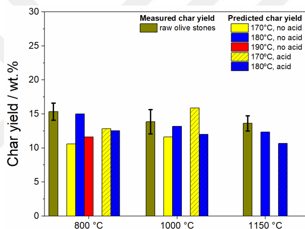
Figure 4.40. Predicted and measured char yields from raw olive stone pyrolysis at 800, 1000, and 1150 °C in the wire mesh reactor based on the additivity law using fractionations of cellulose, hemicellulose, and lignin obtained from organosolv pretreatment.
