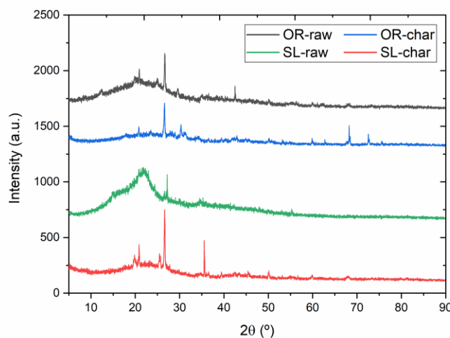
Figure 4.43. X-Ray Diffraction patterns of the chars. Patterns of the raw feedstocks are included for comparison purposes.
