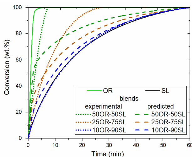
Figure 4.48. Conversion profiles of experimental and predicted (additive) blends during isothermal gasification in TGA at 900 °C. Olive residue and Soma lignite curves are included for comparison purposes.
