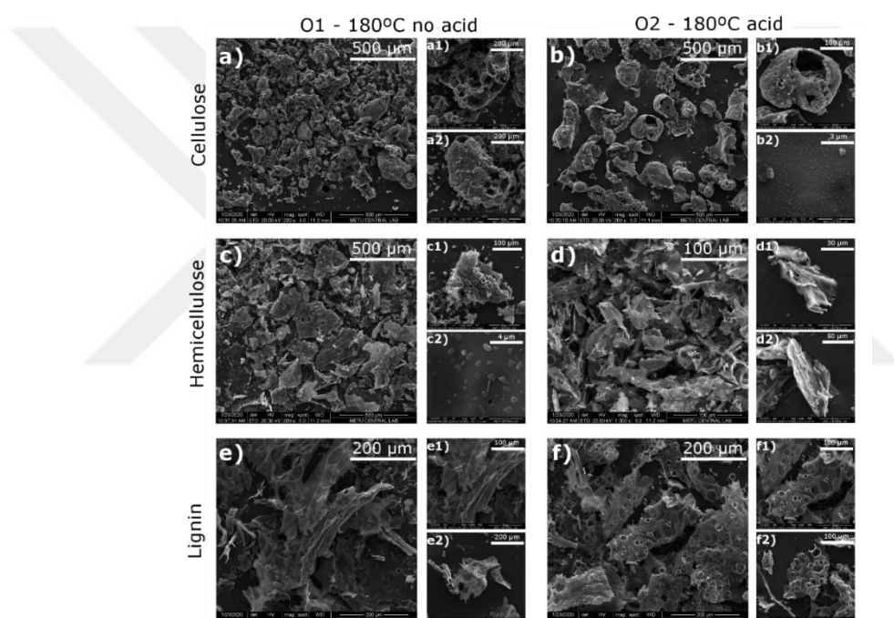
Figure 4.37. Scanning Electron Microscopy (SEM) images of cellulose, hemicellulose, and lignin chars from olive stones fractionated at 180 °C (LHS column: O1, without acid treatment, RHS column: O2, with acid treatment).
