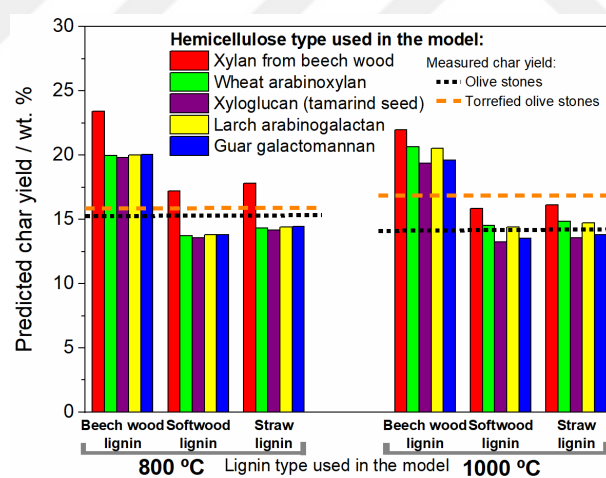
Figure 4.42. Predicted char yields from olive stones and torrefied olive stone pyrolysis at 800 and 1000 °C in the wire mesh reactor based on commercial cellulose, hemicellulose, and lignin.
