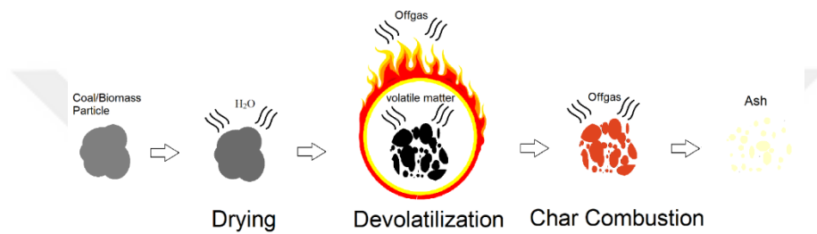
Figure 2.1. Main stages of the combustion of a coal or biomass particle [59].
