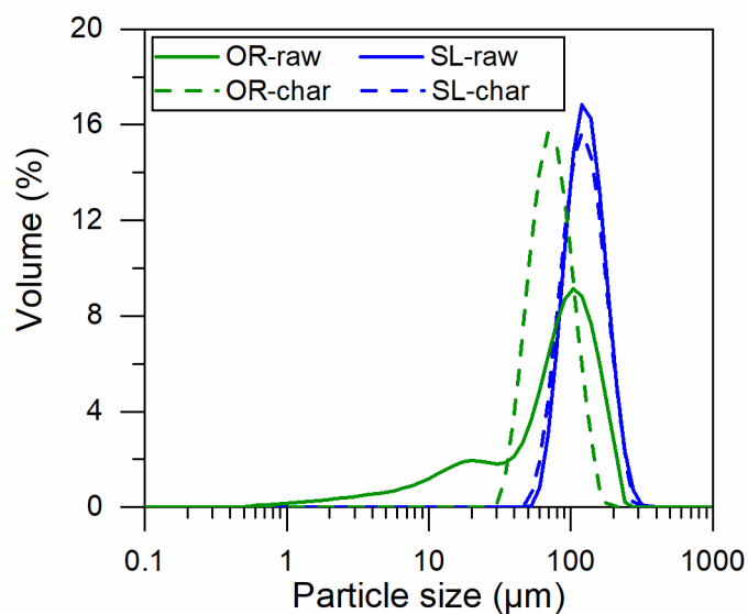
Figure 4.44. Particle size distribution of the raw feedstocks and chars of olive residue and Soma lignite.
