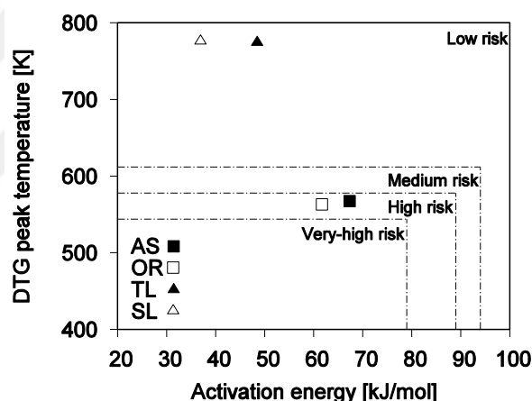
Figure 4.1. Risk of self-ignition map.
