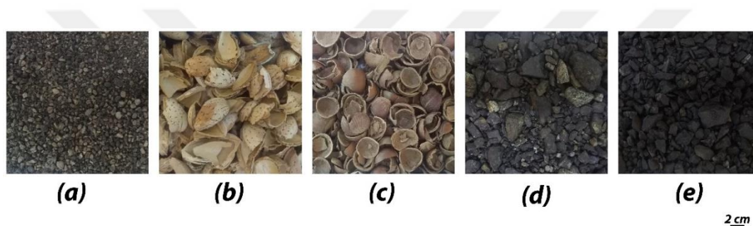
Figure 3.1. Photographs of various fuel samples of this study as received. (a) Olive Residue, (b) Almond Shell, (c) Hazelnut Shell, (d) Tunçbilek lignite, (e) Soma lignite. A size bar is included at the bottom right of this figure.
