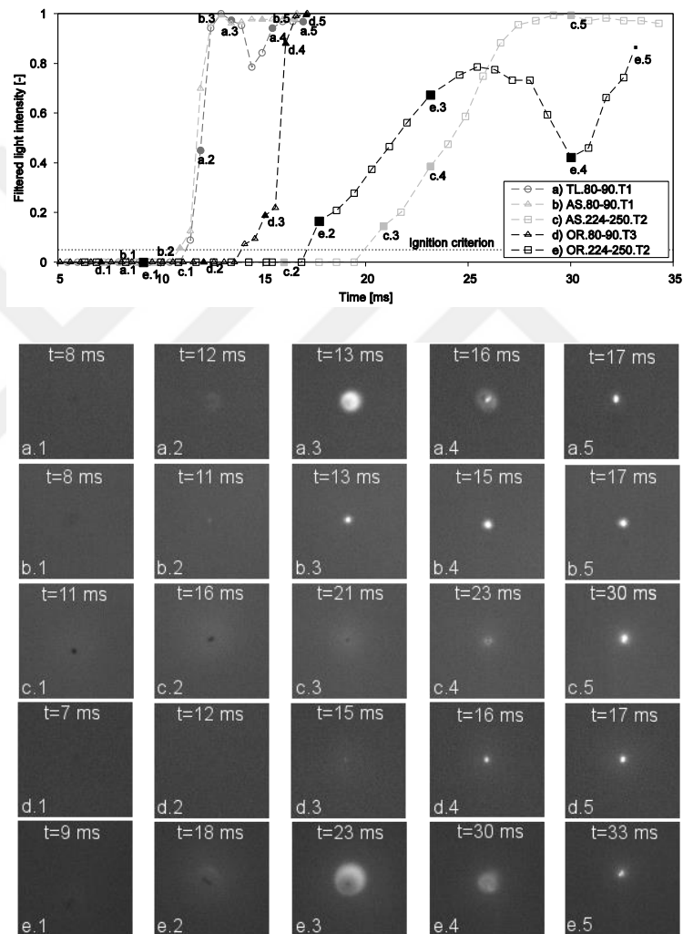
Figure 4.3. Typical ignition events of individual particles during the EFR experiments: (top) filtered and normalized light intensity and the ignition criterion; (bottom) recorded frames for selected events.
