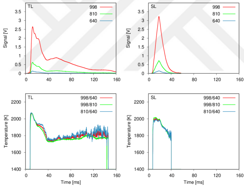
Figure 4.14. Three-color pyrometric intensity signals at wavelengths of 998, 810, 640 nm and derived temperature profiles of Tunçbilek lignite (TL) and Soma lignite (SL), based on the wavelength ratios of 998/640, 998/810 and 810/640.
