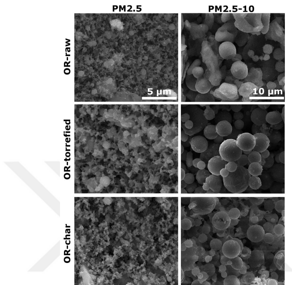
Figure 4.21. Scanning electron microscopy micrographs from PM2.5 and PM2.5-10 resulting from the combustion at 1200 °C in the drop tube furnace of olive residue (raw, torrefied, and char).
