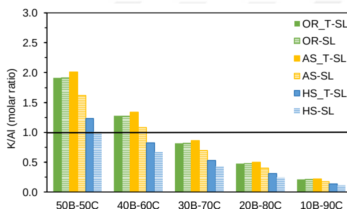
Figure 4.16. K/Al molar ratios for each blend of biomass (B) and Soma lignite (C). The horizontal line demarks the threshold above which synergistic effects may be observed for biomass-coal mixtures.
