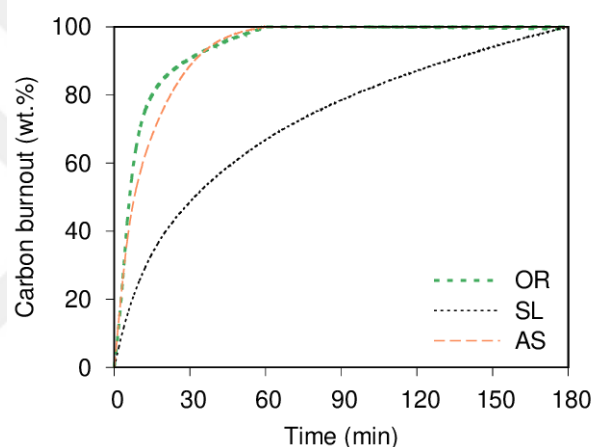
Figure 4.28. Carbon burnout as a function of time for the individual chars. Olive residue (OR) and almond shell (AS) chars were oxidized at 400 °C and Soma lignite (SL) char was oxidized at 450 °C.
