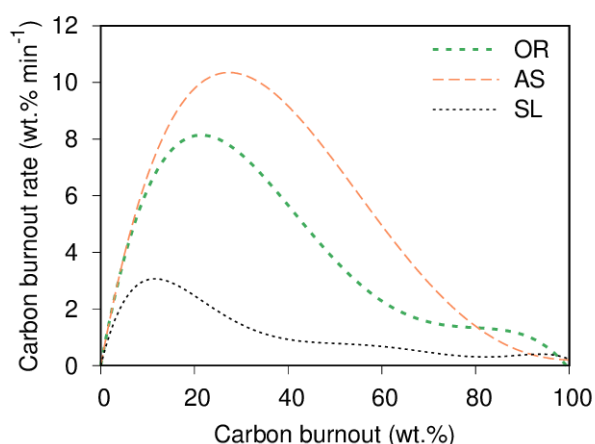
Figure 4.29. Carbon burnout rate as a function of burnout for the individual chars. Olive residue (OR) and almond shell (AS) chars were oxidized at 400 °C and Soma lignite (SL) char was oxidized at 450 °C.
