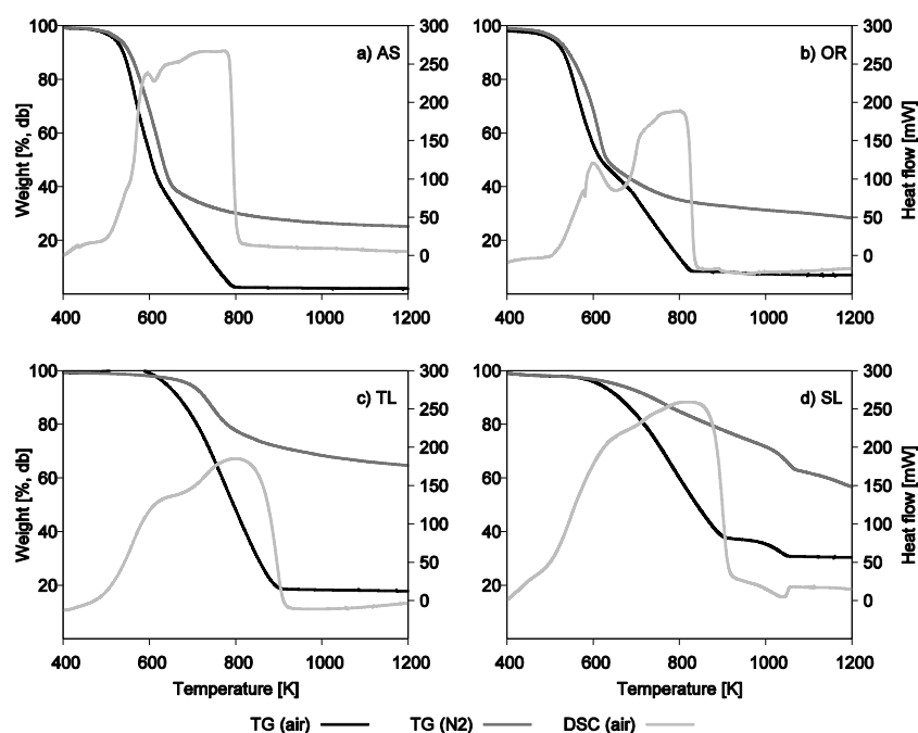
Figure 4.2. TG – combustion (black lines); TG – pyrolysis (dark grey lines); and DSC – air (light grey lines) profiles for all studied fuels under 20 K/min. a) AS; b) OR; c) TL; d) SL.
