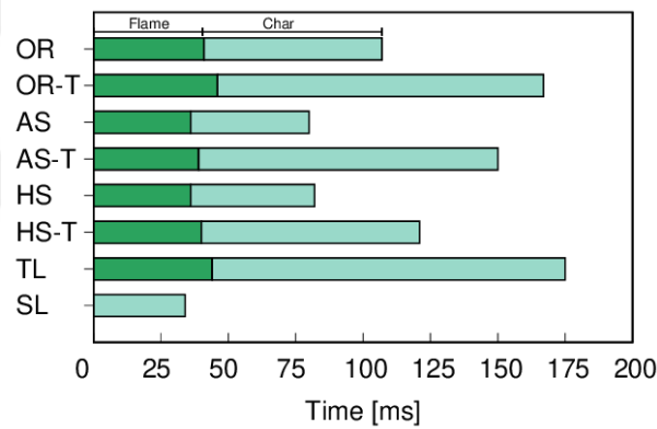
Figure 4.12. Flame (dark green bars) and char (light green bars) burnout times for all studied fuels, as measured by pyrometry.
