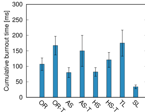
Figure 4.15. Cumulative burnout times from pyrometry measurements for all studied fuels. Vertical bars represent 98% confidence statistical errors.
