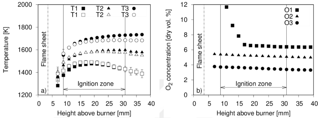
Figure 3.11. a) Measured (open symbols) and corrected gas temperatures (solid symbols) for conditions T1-T3. Vertical bars represent 98% confidence statistical errors. b) Measured oxygen concentrations for conditions O1-O3.
