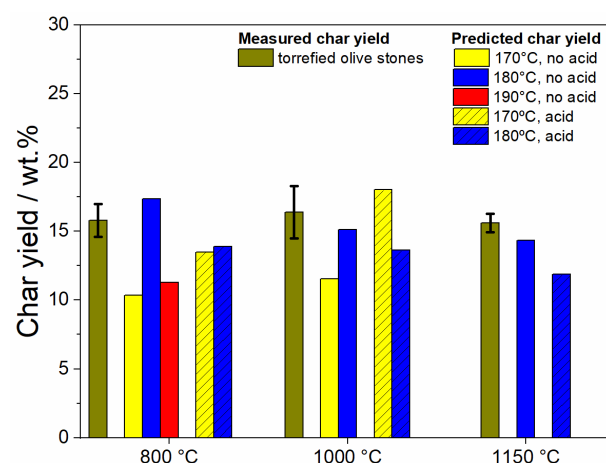
Figure 4.41. Predicted and measured char yields from torrefied olive stone pyrolysis at 800, 1000, and 1150 °C in the wire mesh reactor based on the additivity law using fractionations of cellulose, hemicellulose, and lignin obtained from organosolv pretreatment.
