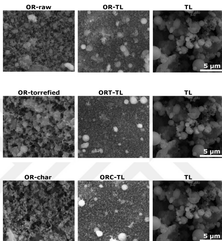
Figure 4.24. Scanning electron microscopy micrographs from PM 2.5 resulting from the combustion at 1200 °C in the drop tube furnace of olive residue (raw, torrefied, and char) and 50:50 blends with Tunçbilek lignite.
