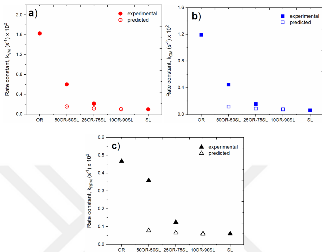
Figure 4.51. Rate constants of the blends from fitting of a) the volumetric model, b) the grain model, and c) the random pore model from isothermal gasification at 900 °C.
