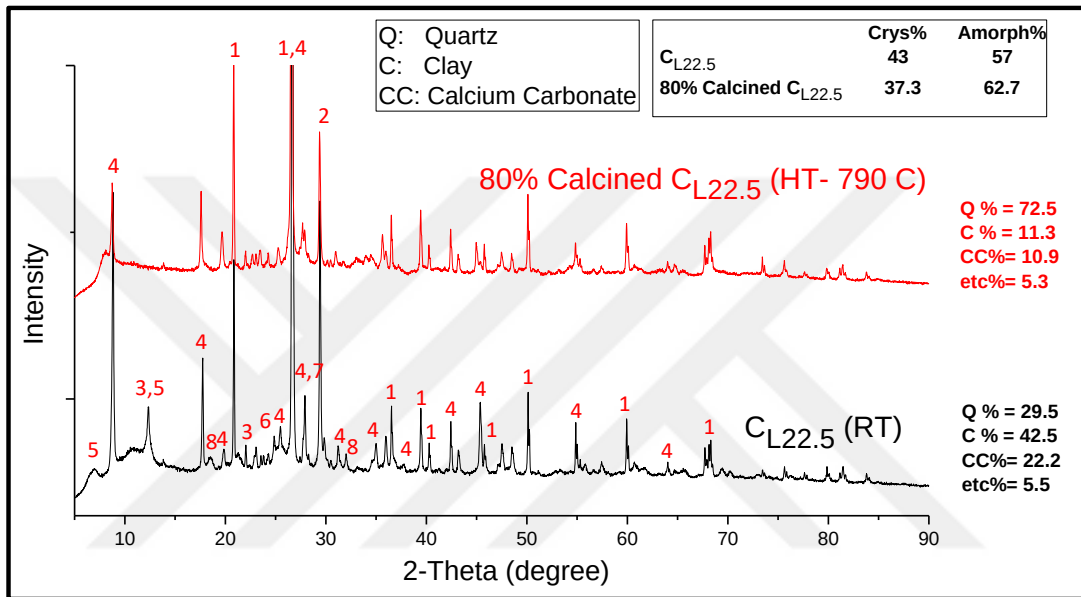
Figure 37. X-ray spectrum of untreated vs. 80% calcined C_{L22.5} schist powder (C schist with 22.5 wt% C\bar{C} addition). The numbers at the peaks correspond to phases listed in table 19.
