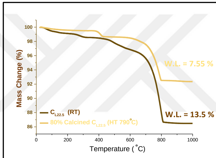
Figure 54. Thermo-gravimetric analysis of untreated vs. 80% calcined C_{L22.5} schist powders (C schist with 22.5 wt% CC addition).
