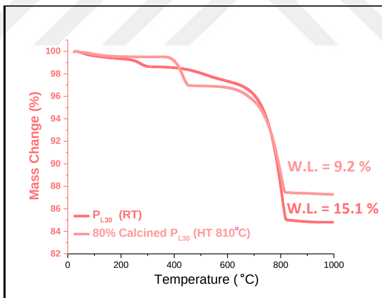
Figure 59. Thermo-gravimetric analysis of untreated vs. 80% calcined P_{L30} schist powders (P schist with 30 wt% CC addition).
