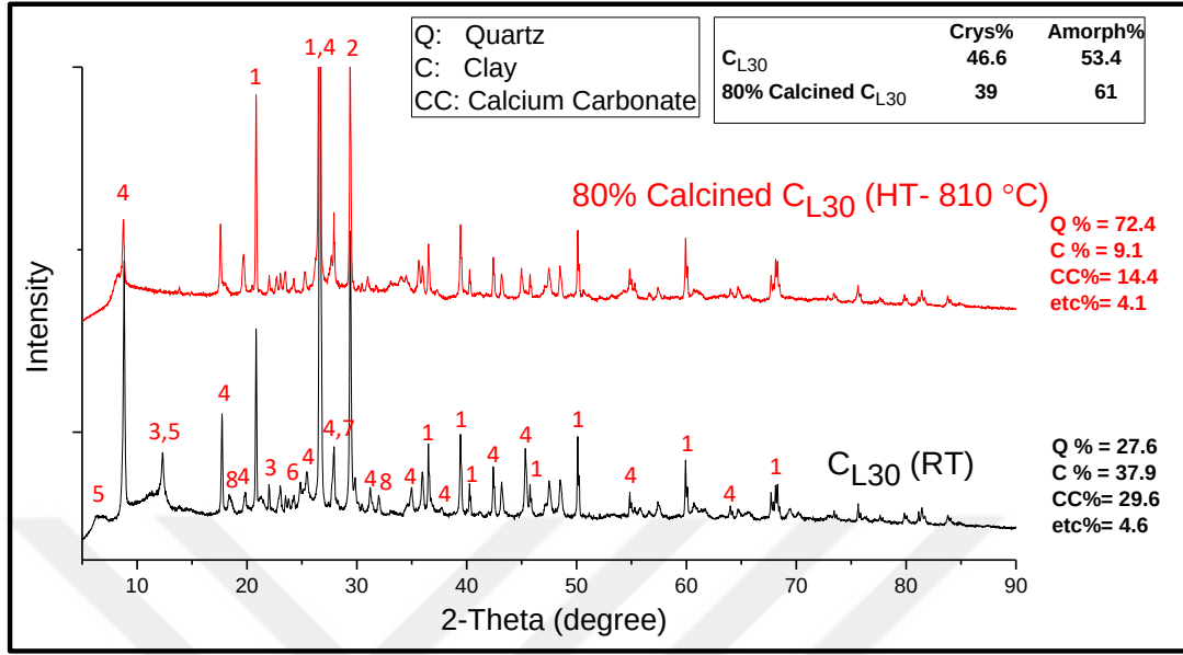
Figure 38. X-ray spectrum of untreated vs. 80% calcined CL30 schist powder (C schist with 30 wt% CC addition). The numbers at the peaks correspond to phases listed in table 19.
