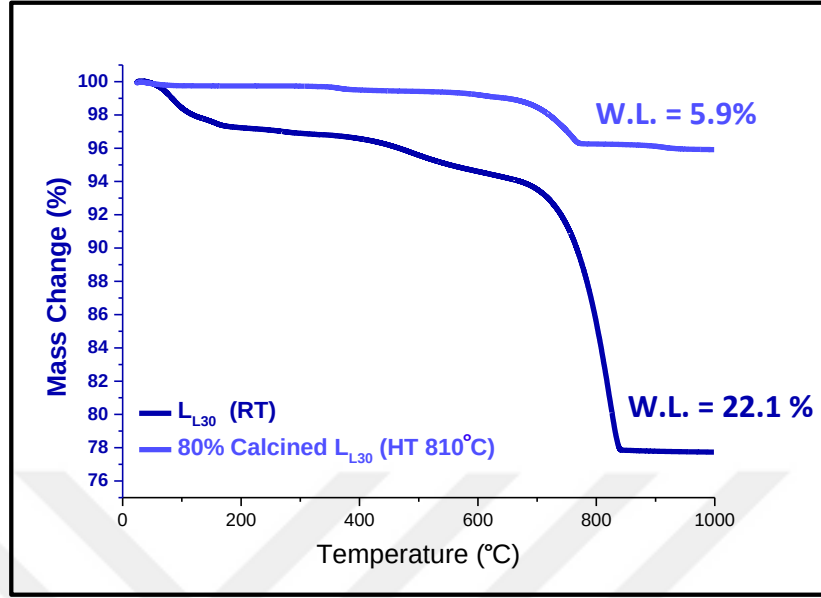
Figure 64. Thermo-gravimetric analysis of untreated vs. 80% calcined L_{L30} schist powders (L schist with 30 wt% CC addition).
