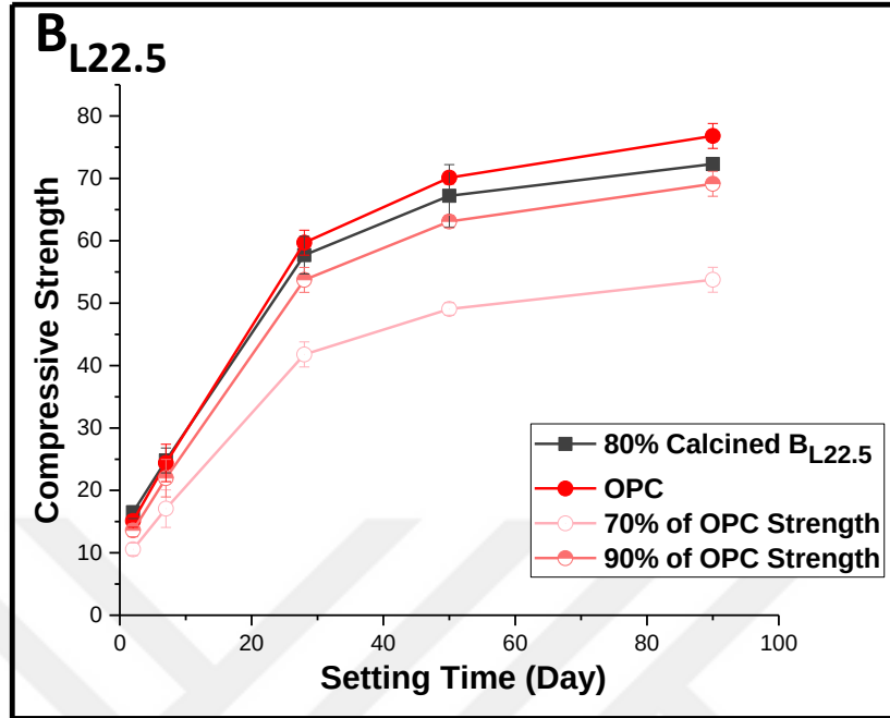
Figure 87. Compressive strength of OP cement blended with 30 wt% of calcined B L22.5 schist (B schist with 22.5 wt% \bar{C}\bar{C} addition), compared to pure cement
