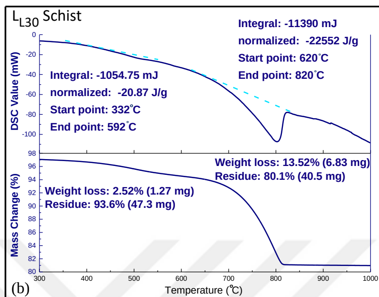
Figure 73. DSC/TGA curve of L 30 schist sample in the temperature range of (a) 25-300°C and (b) 300-1000°C
