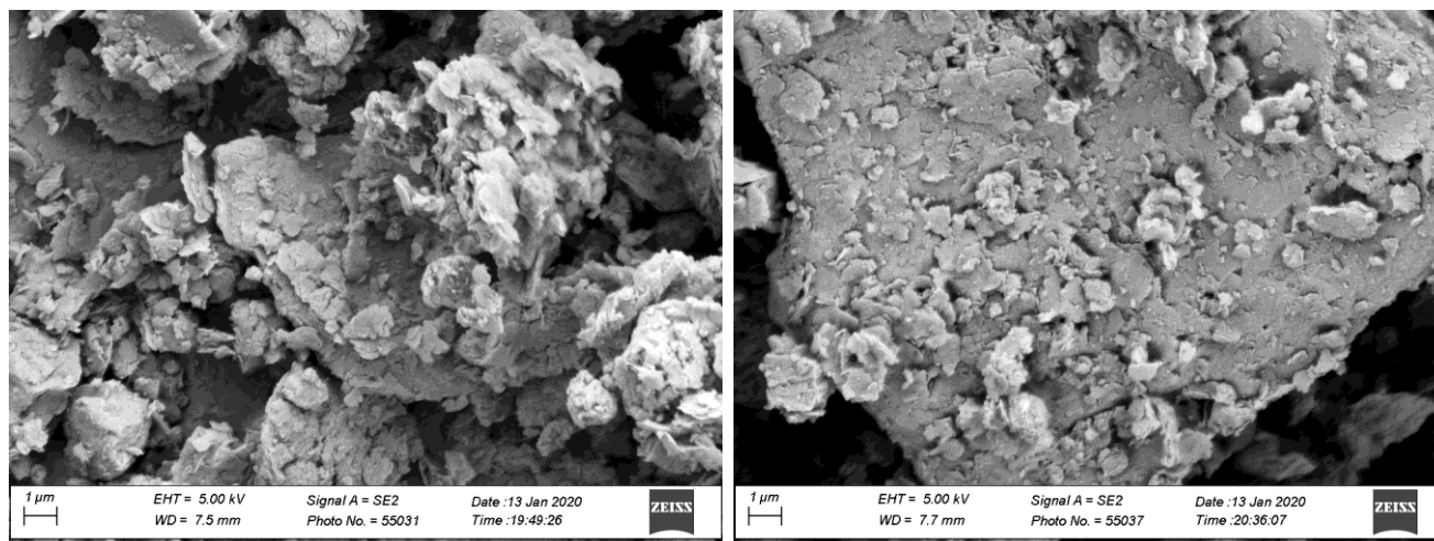
Figure 69. L schist micrographs for Virgin (Left) and Calcined (Right) Powders at the same magnification. First row: mag. = 1KX, second row: mag = 5KX, and third row: mag = 10KX
