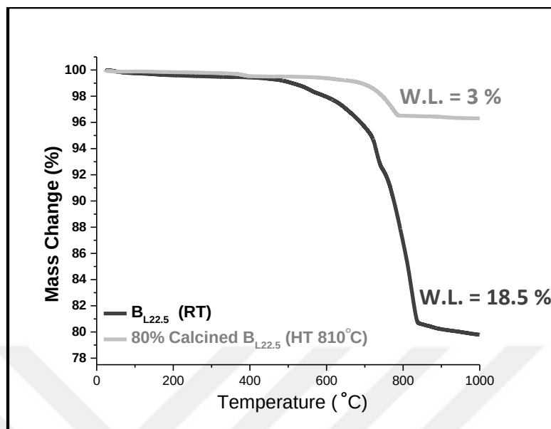
Figure 61. Thermo-gravimetric analysis of untreated vs. 80% calcined B L22.5 schist powders (B schist with 22.5 wt% \text{CC} addition).
