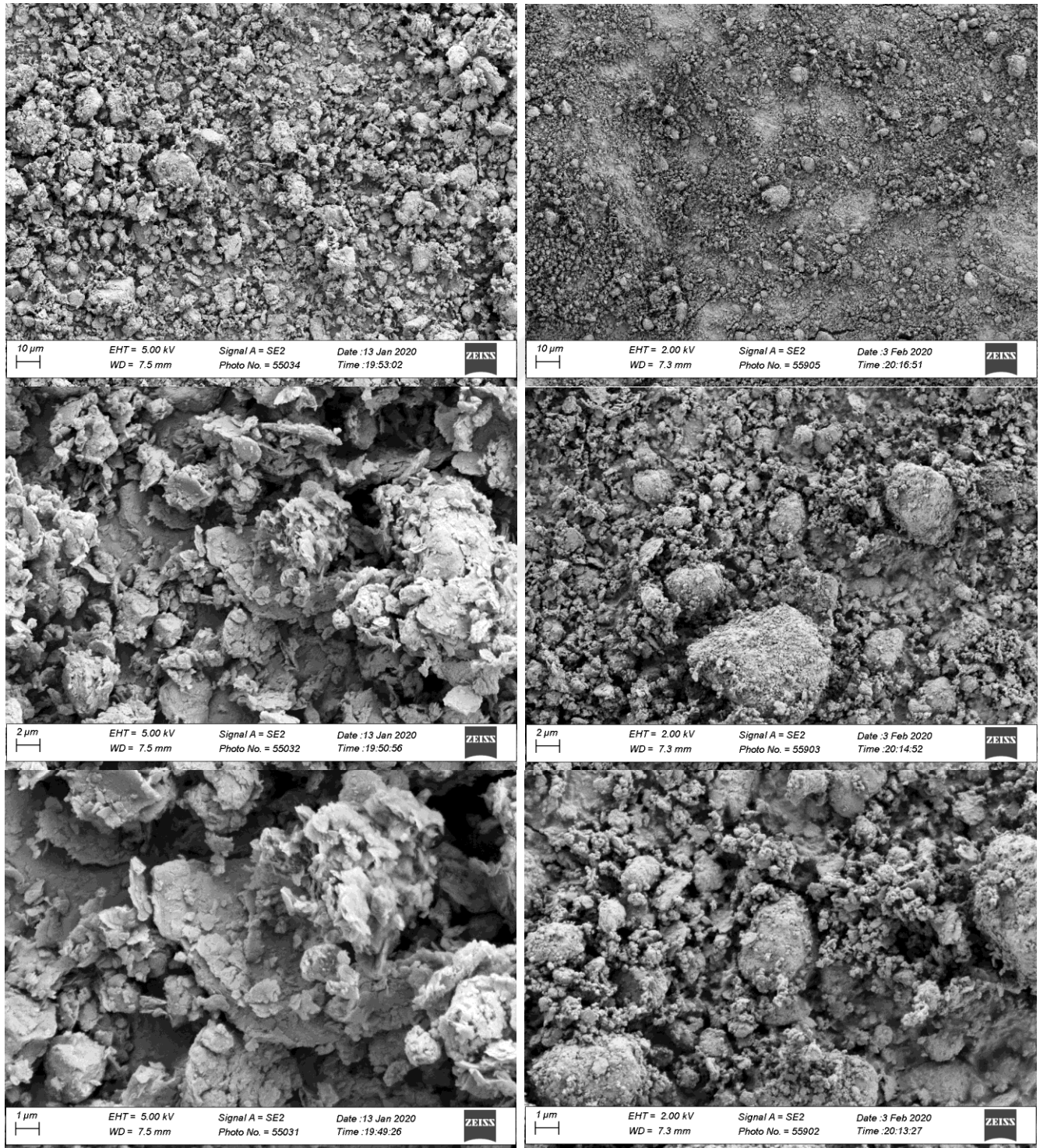
Figure 99. L schist micrographs for Virgin (Left) and ball milled (Right) Powders at the same magnification. First row: mag. = 1KX, second row: mag = 5KX, and third row: mag = 10KX
