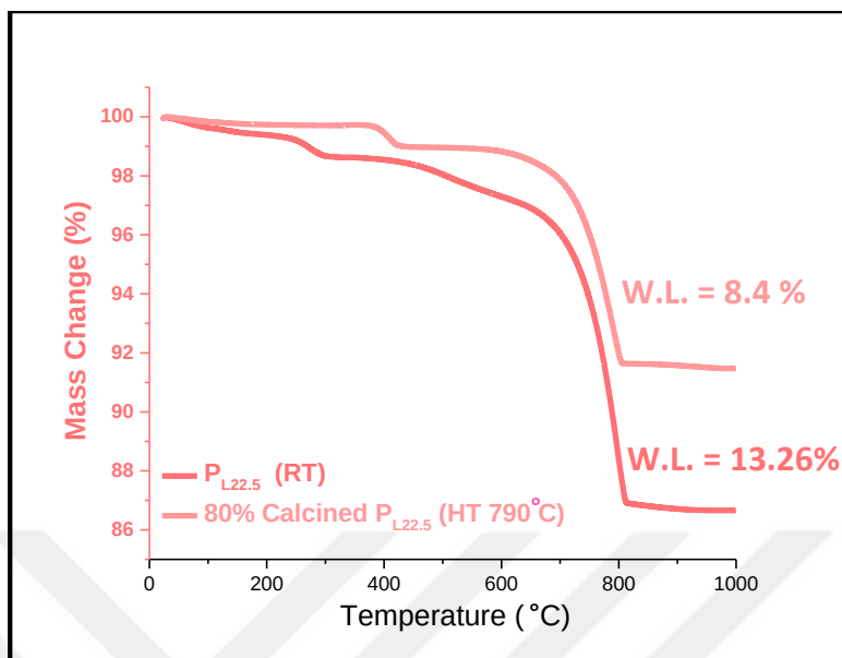
Figure 58. Thermo-gravimetric analysis of untreated vs. 80% calcined P_{L22.5} schist powders (P schist with 22.5 wt% CC addition).
