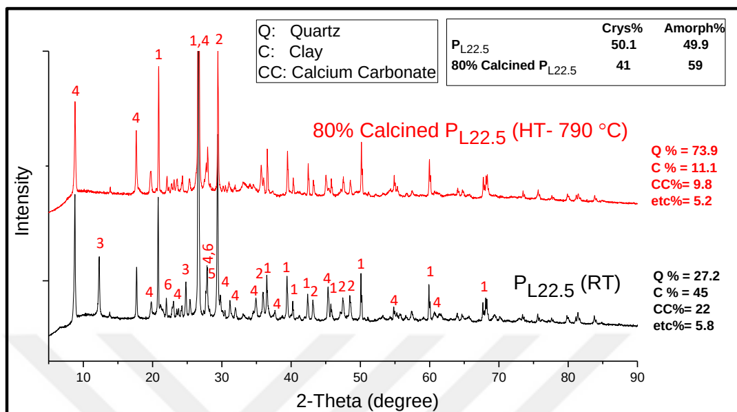
Figure 41. X-ray spectrum of untreated vs. 80% calcined P_{L22.5} schist powder (P schist with 22.5 wt% CC addition). The numbers at the peaks correspond to phases listed in table 20.
