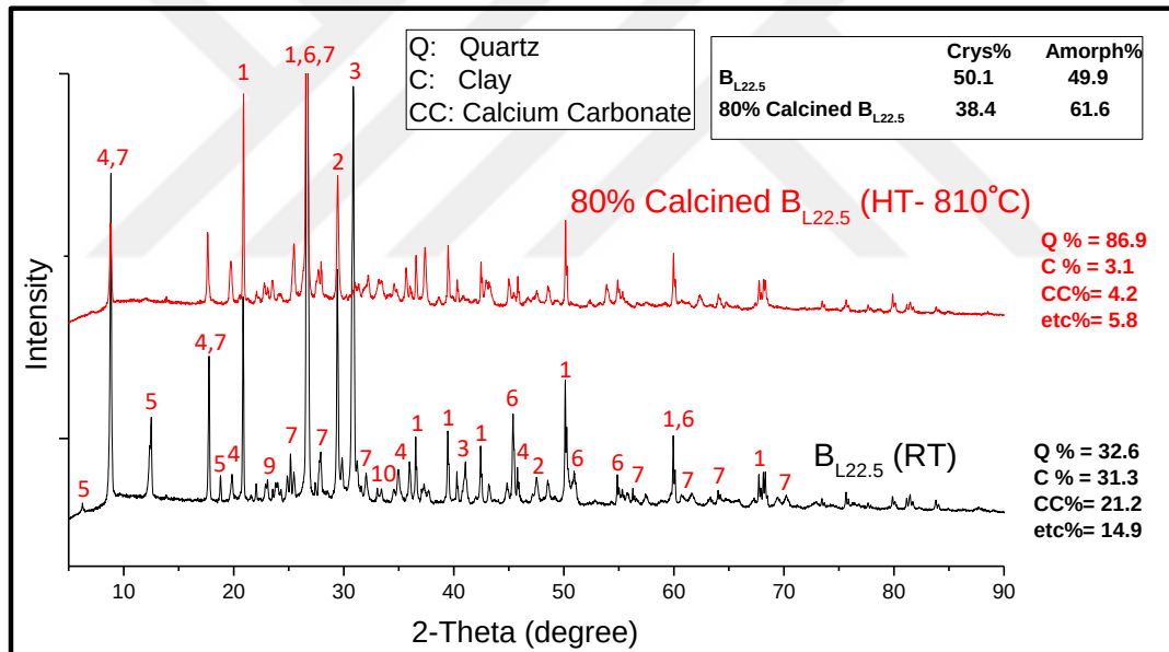
Figure 44. X-ray spectrum of untreated vs. 80% calcined \text{B}_{\text{L22.5}} schist powder (B schist with 22.5 wt% \text{CC} addition). The numbers at the peaks correspond to phases listed in table 21.
