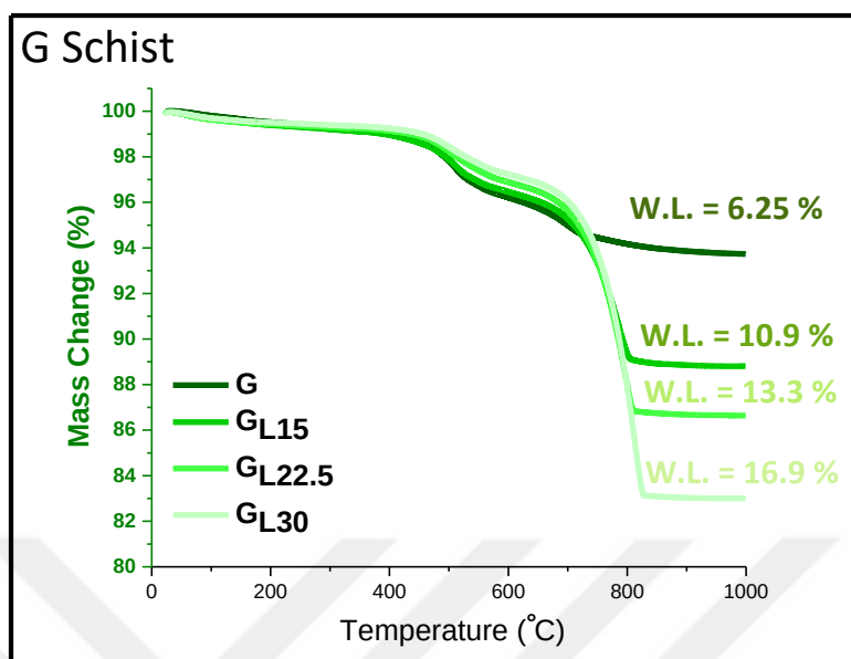
Figure 16. TGA diagram of G: G schist (as-received), G_{L15} : G schist with 15 wt% CC addition, G_{L22.5} : G schist with 22.5 wt% CC addition, and G_{L30} : G schist with 30 wt% CC addition
