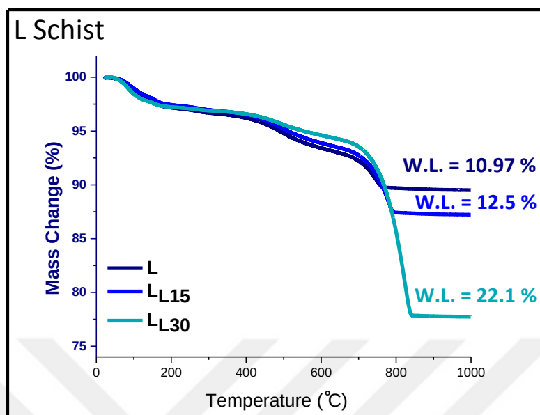
Figure 24. TGA diagram of L: L schist (as-received), L L15 : L schist with 15 wt% CC addition, and L L30 : L schist with 30 wt% CC addition
