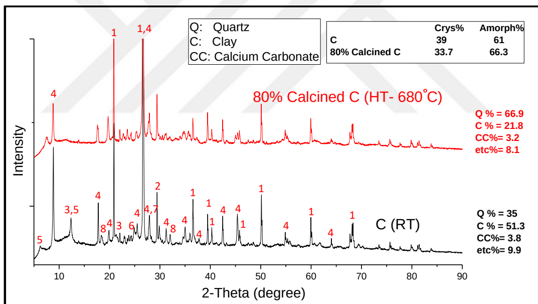
Figure 35. X-ray spectrum of virgin vs. 80% calcined C schist powder. The numbers at the peaks correspond to phases listed in table 19.
