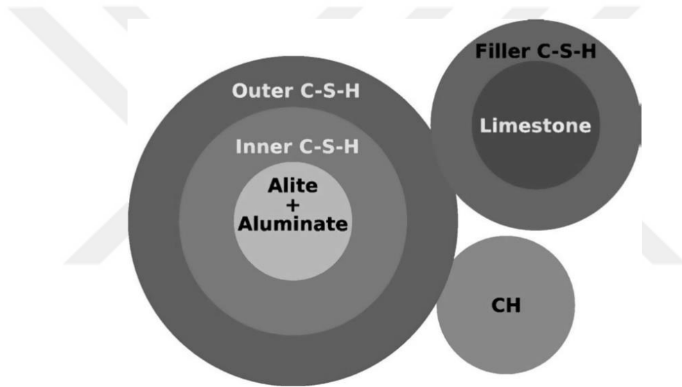
Figure 6. Example of different materials and particle types defined in a simulation [92]
