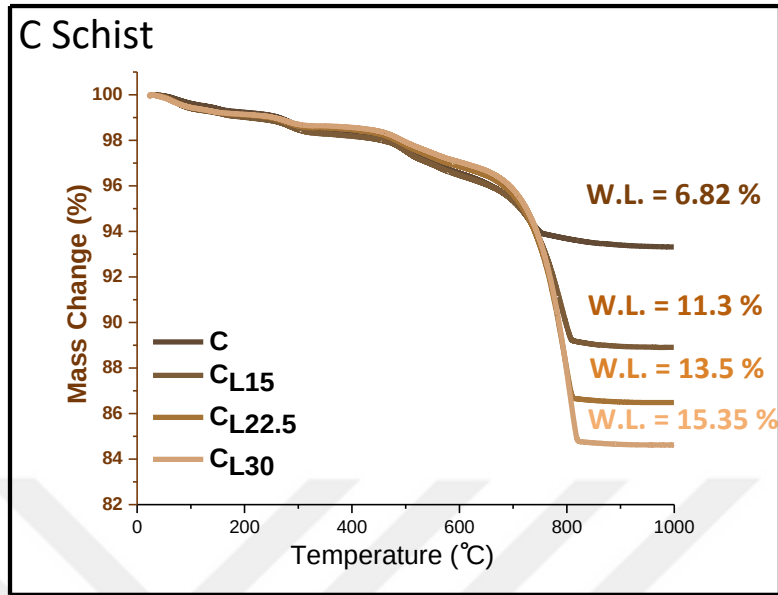
Figure 18. TGA diagram of C: C schist (as-received), CL15: C schist with 15 wt% \text{CC} addition, CL22.5: C schist with 22.5 wt% \text{CC} addition, and CL30: C schist with 30 wt% \text{CC} addition
