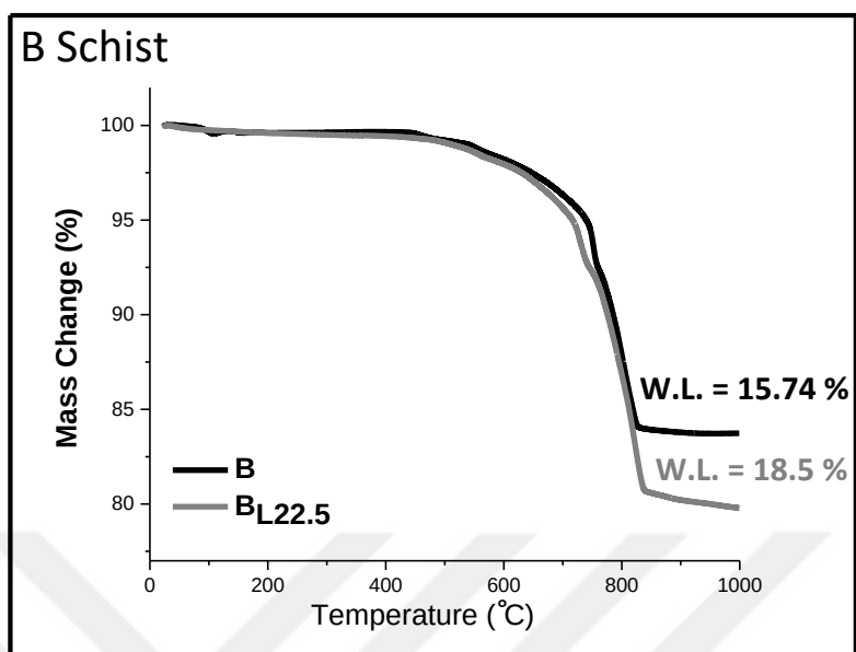
Figure 22. TGA diagram of B: B schist (as-received), and B_{L22.5} : B schist with 22.5 wt% CC addition
