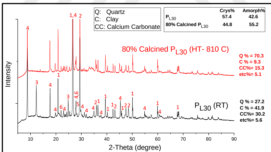
Figure 42. X-ray spectrum of untreated vs. 80% calcined P_{L30} schist powder (P schist with 30 wt% CC addition). The numbers at the peaks correspond to phases listed in table 20.
