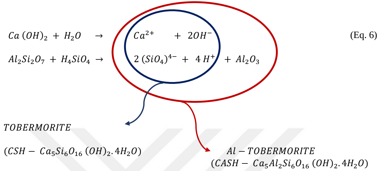
Equation 6. Pozzolanic Reaction of Kaolinite and CH
