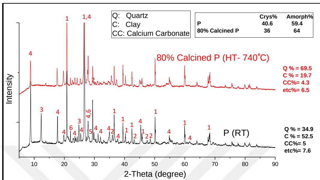
Figure 39. X-ray spectrum of virgin vs. 80% calcined P schist powder. The numbers at the peaks correspond to phases listed in table 20.
