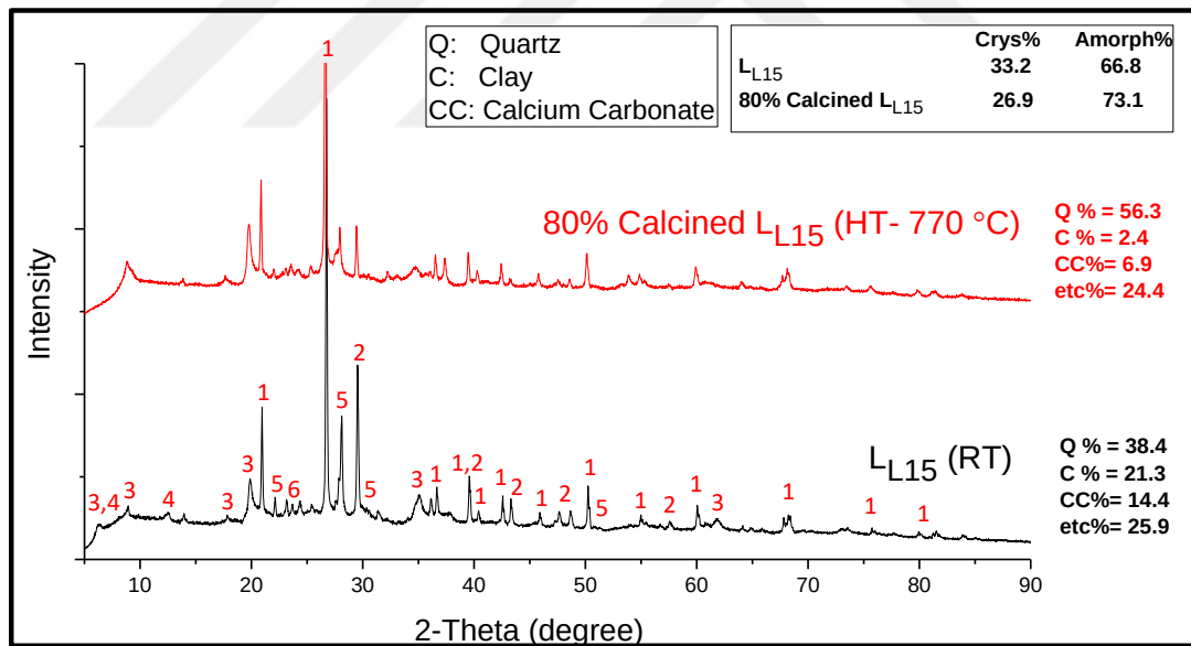
Figure 46. X-ray spectrum of untreated vs. 80% calcined \text{L}_{\text{L15}} schist powder (L schist with 15 wt% \text{CC} addition).
