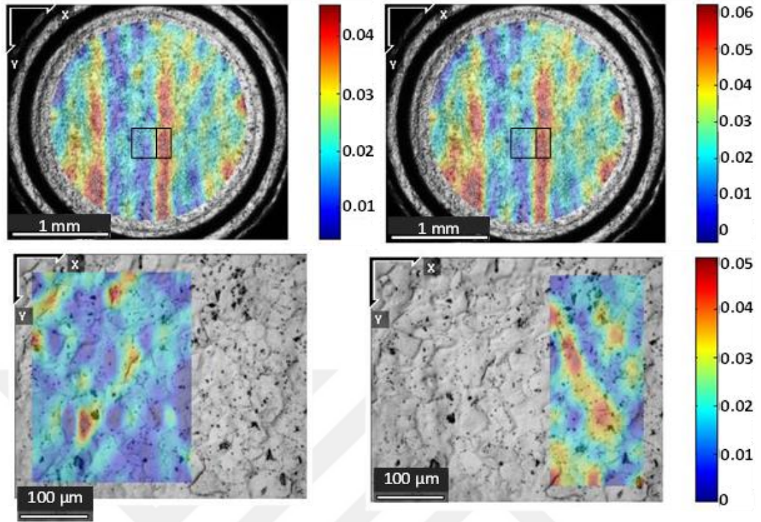
Figure 4.3. Multi-scale DIC results of Bi-1 sample under equibiaxial tension. Upper left image is the strain analysis at the meso-scale for the Step I. The sub-regions are separated by a line in the rectangular box. Upper right image is the strain analysis at the meso-scale for Step V. Lower images are the strain analysis at the micro-scale for Step III.
