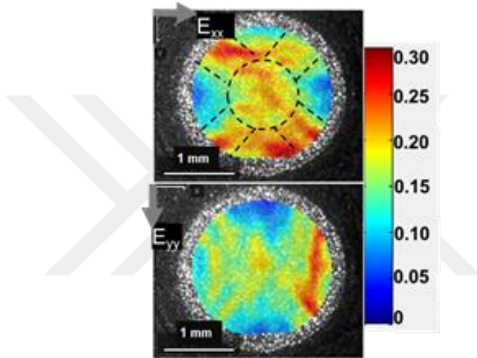
Figure 2.7. DIC Results of Al 6061-T6 up to fracture. The upper results for E_{xx} while the below for E_{yy} . The strain bands are shown as dashed lines.
