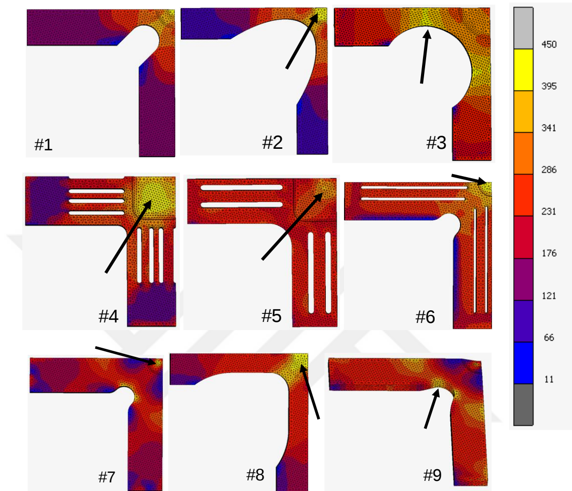
Figure 2.3. FEA results of various cruciform design. The numbers correspond to sample design numbers in Table 2.2.
