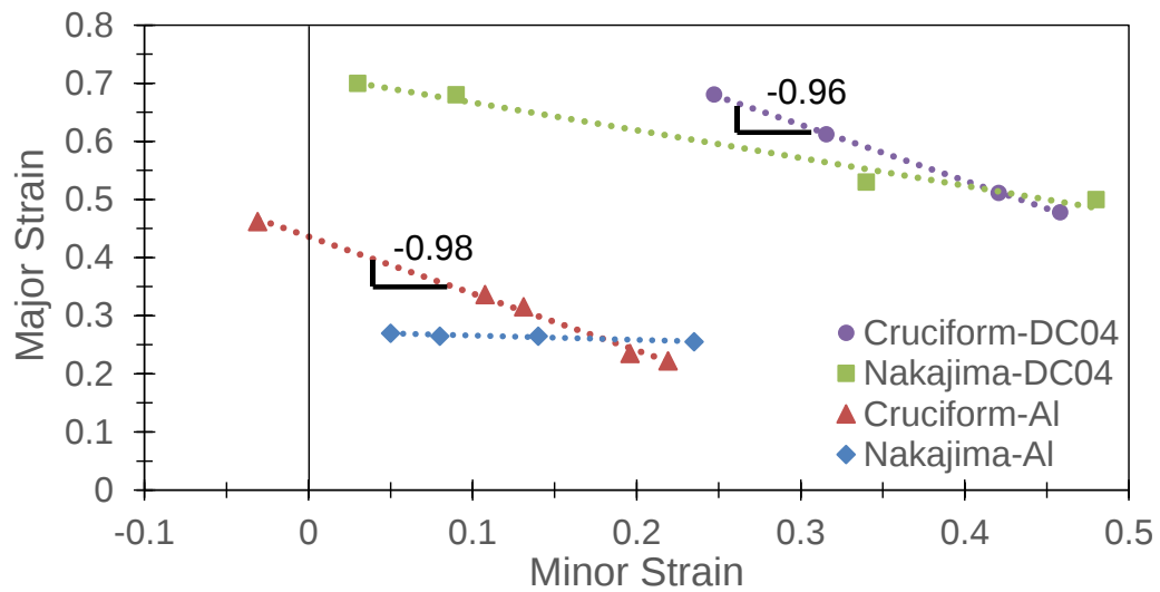
Figure 3.8. Comparison of fracture limit curves of Al 6061-T6 and DC-04 steel with regards to Cruciform and Nakajima tests.
