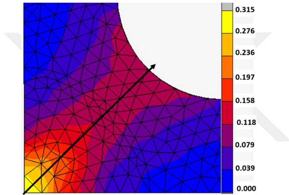
Figure 2.4. FEA result of the cruciform sample with respect to the total equivalent plastic strain.
