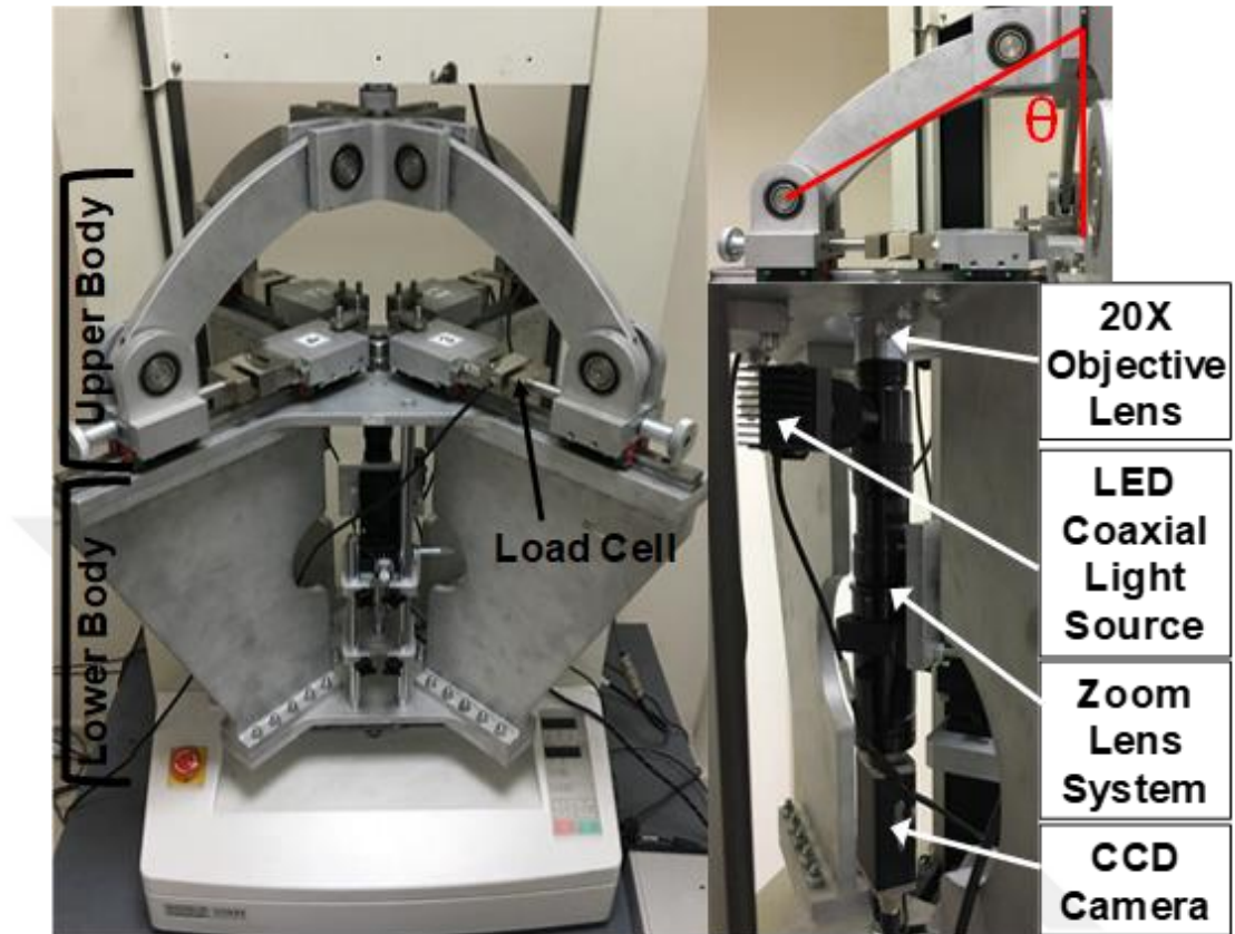
Figure 2.1. Biaxial test setup.
