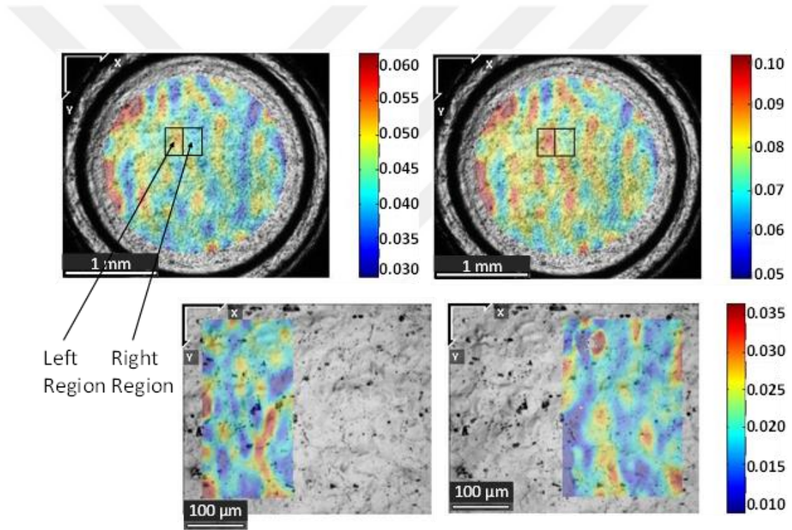
Figure 4.2. Multi-scale DIC results of Uni-1 sample under uniaxial tension. Upper left image is the strain analysis at the meso-scale for the Step I. The sub-regions are separated by a line in the rectangular box. Upper right image is the strain analysis at the meso-scale for Step V. Lower images are the strain analysis at the micro-scale for Step III.
