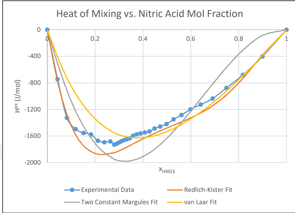
Figure 5.2 Comparison of experimental and fitted heat of mixing data for oxidizer - water mixture
