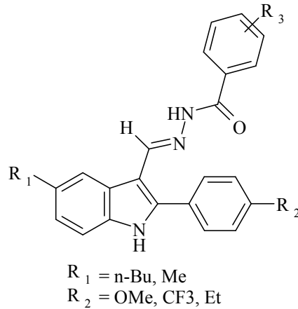
2-fenilindol-3-karbaldehit benzoilhidrazon
