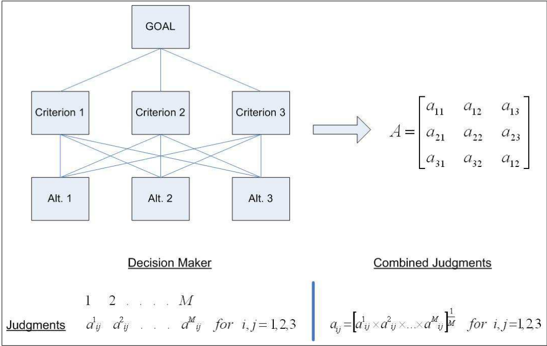
Figure 2.1: Combined Judgments
