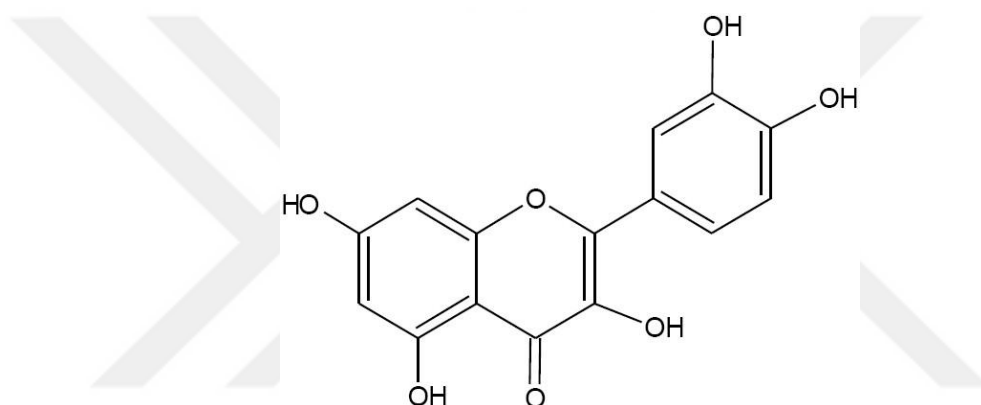
Figure 2.4. Chemical structure of quercetin.
