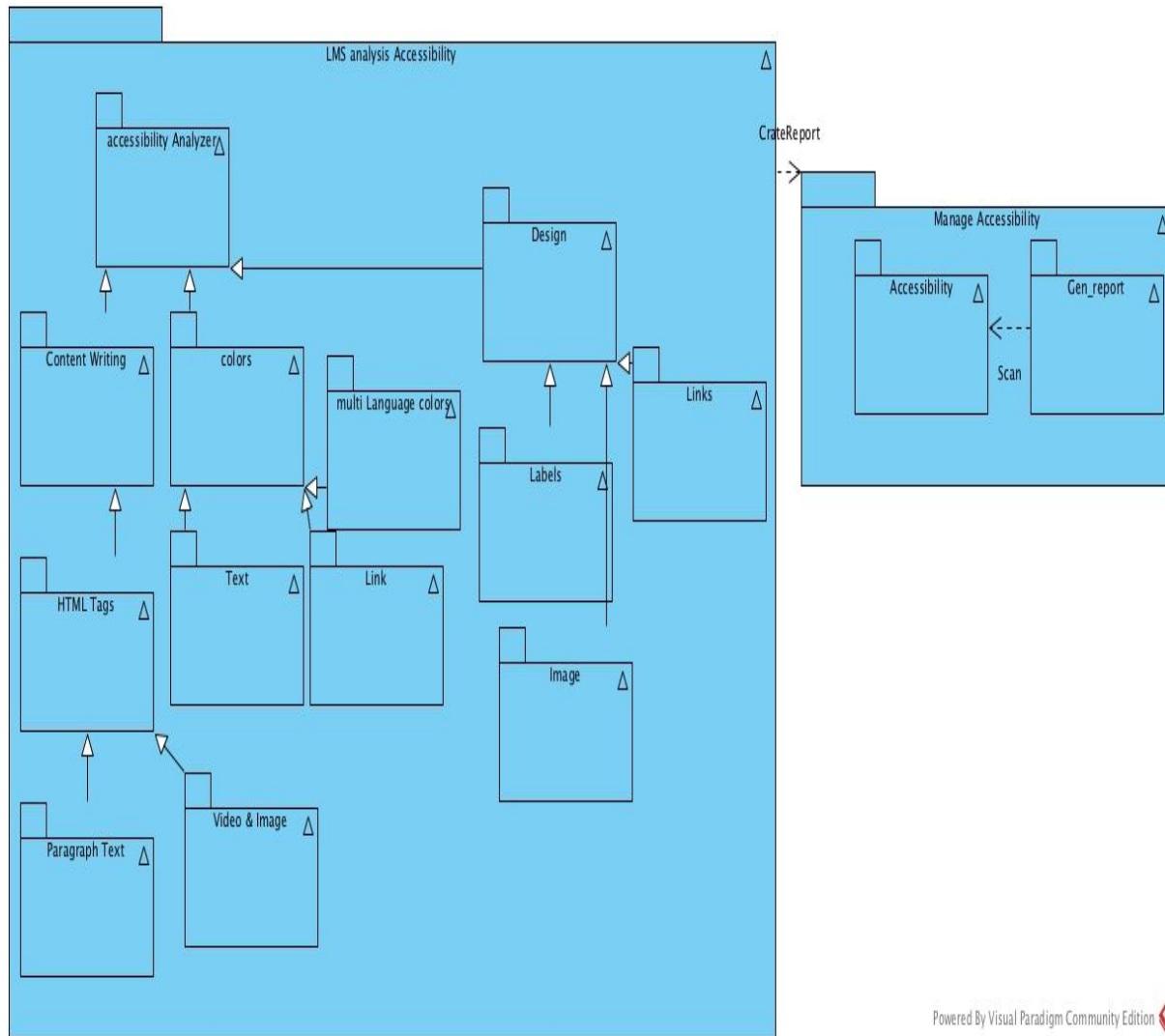
Figure 5.3: LMS Analysis Accessibility Module
