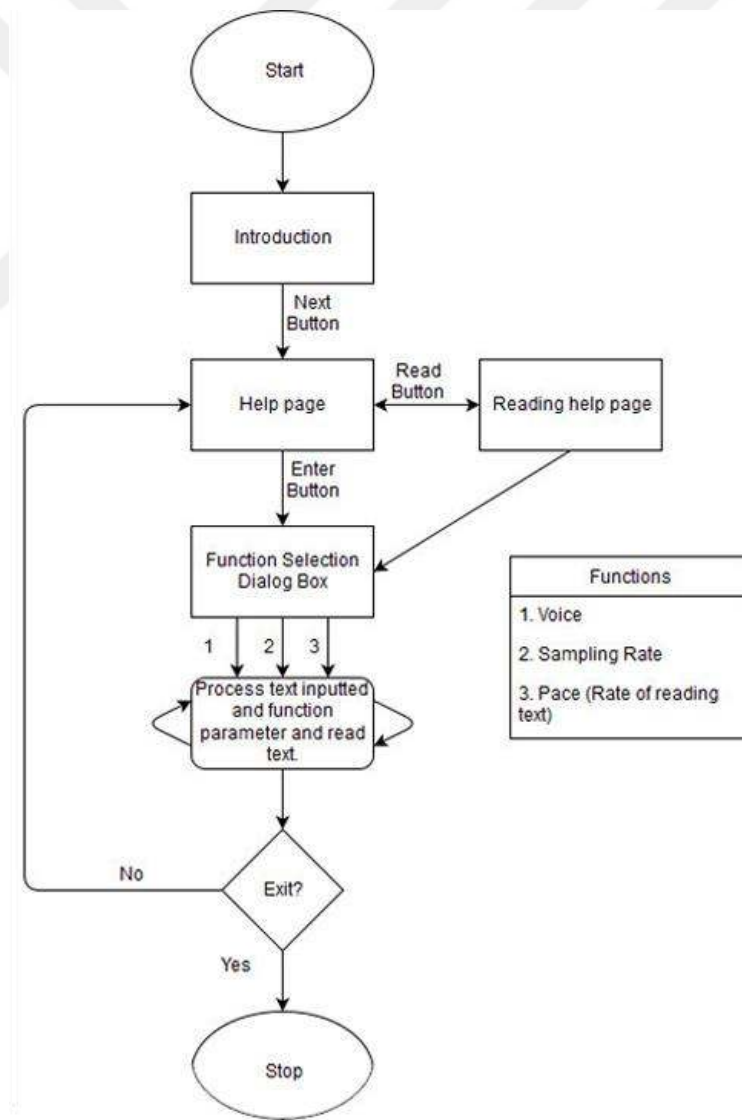
Figure 6.18: Speech Algorithm
