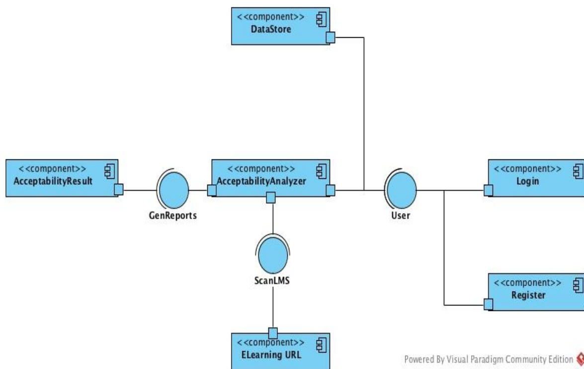
Figure 5.5: UML Component Diagram.
