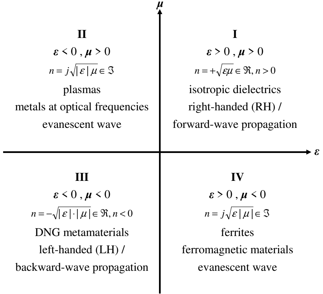
Figure 2.2: Permittivity and permeability ( \epsilon - \mu ) diagram.
