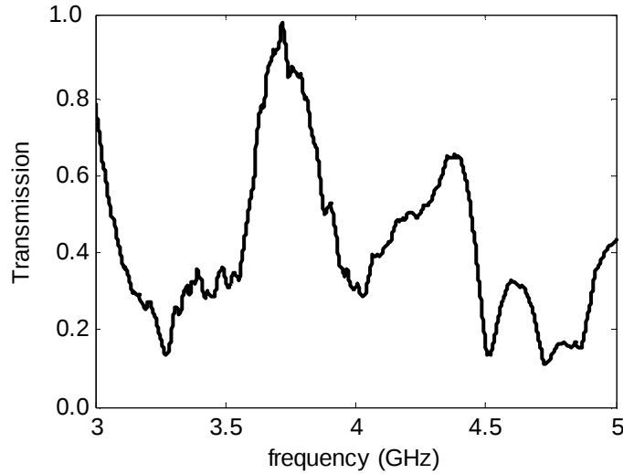
Figure 6.25: Measured transmission spectrum for five layered configuration comprised of three metamaterial slabs and two dielectric (air) layers.
