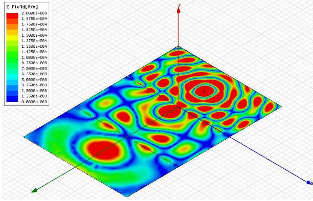
Figure 4.27: Magnitude of the electric field for DNS simulation without using effective medium approach. ( \epsilon_r = 9.0, \mu_r = 1.0 for DPS-I, \epsilon_r = -3.5032, \mu_r = -1.0014 . for DNG medium, and \epsilon_r = 1.0, \mu_r = 1.0 for DPS-II.)
