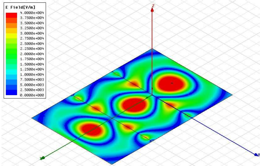
Figure 4.28: Magnitude of the electric field for DNS simulation with using effective medium approach. ( \epsilon_r = 9.0, \mu_r = 1.0 for DPS-I, \epsilon_r = -3.5032, \mu_r = -1.0014 . for DNG medium, and \epsilon_r = 1.0, \mu_r = 1.0 for DPS-II.)
