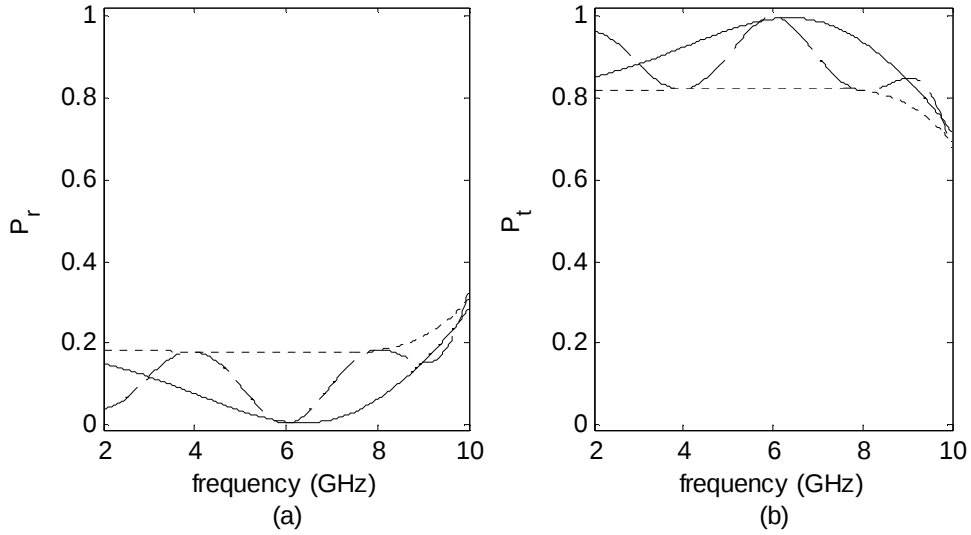
Figure 5.25: Reflected and transmitted powers against the frequency for Structure I. Solid lines represent c_1 = c_2 = 1/4 , dashed lines c_1 = 1/2 and c_2 = 1/4 , and dotted lines c_1 = 1/4 and c_2 = 1/2 .
