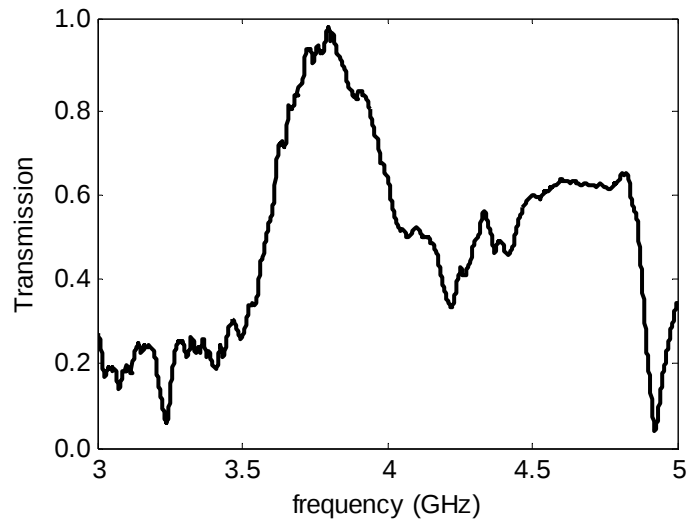
Figure 6.20: Measured transmission characteristic versus the frequency for one metamaterial slab with two columns consists of 16 unit cells.
