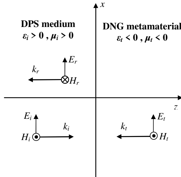
Figure 4.1: Reflection and transmission at normal incidence by two planar semi infinite DPS and DNG media.
