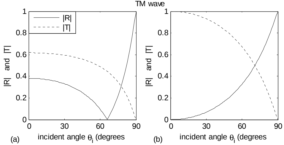
Figure 4.6: Magnitude of reflection and transmission coefficients versus incident angle for hypothetical DNG metamaterial. \{\epsilon_i = \epsilon_o, \mu_i = \mu_o ; (a) \epsilon_t = -5\epsilon_o, \mu_t = -\mu_o ; (b) \epsilon_t = -5\epsilon_o, \mu_t = -5\mu_o\} .
